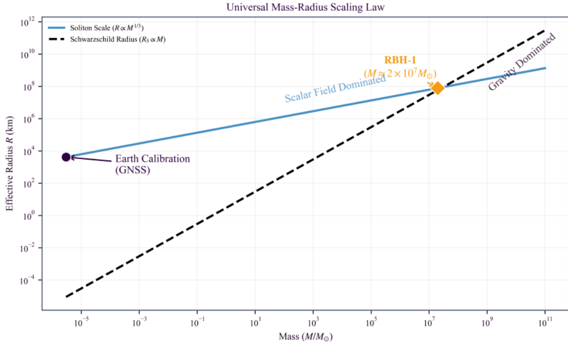
Figure D.1: The Universal Scaling Plot. The trajectory represents the saturation scaling law ( R \propto M^{1/3} ), calibrated via terrestrial GNSS data ( L_e \approx 4200 \text{ km} ). This sets the scaling used in the SPARC comparison (Appendix D.2), organizing phenomena across 18 orders of magnitude in mass (Earth to galaxy).
