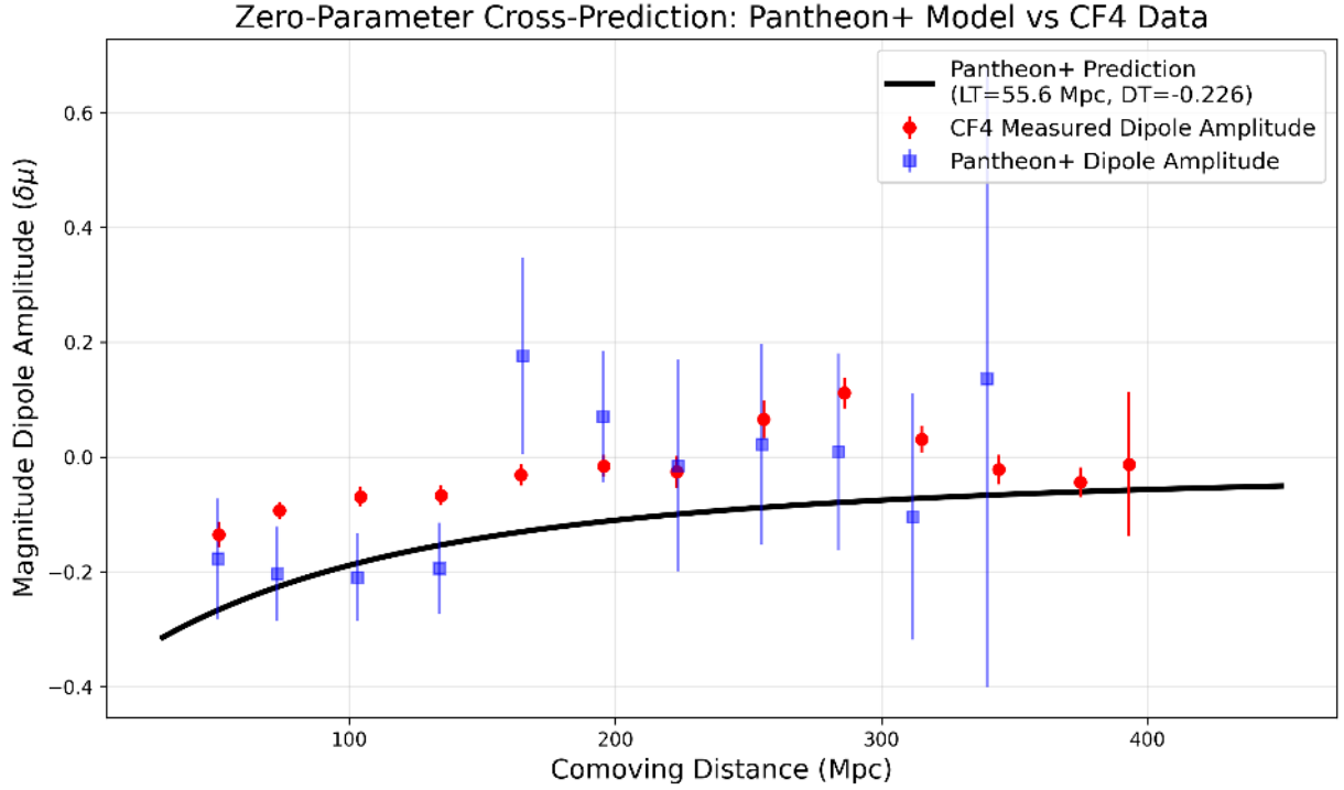
Figure 6: Zero-parameter cross-prediction. The Pantheon+ derived finite-coherence temporal model ( L_T = 55.6 Mpc, DT = -0.226 ) projected onto the distance-binned CF4 dipole amplitude (red circles) and Pantheon+ dipole amplitude (blue squares).
