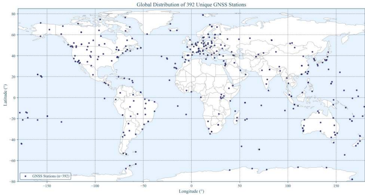
Figure 1b. GNSS Station Coverage Map: Global distribution showing substantial overlap between analysis centers and geographic coverage essential for intercontinental correlation analysis.
