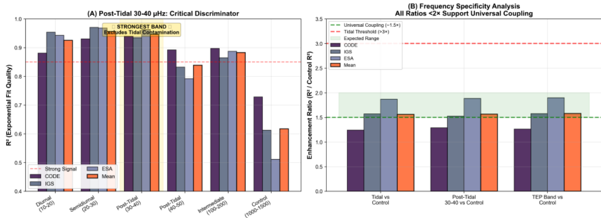
Figure 10. Comprehensive Post-Tidal Discriminator Analysis. (A) Post-tidal 30–40 \mu\text{Hz} prominence: Strongest band excludes classical tidal contamination while maintaining high correlation quality across all analysis centers (mean R^2 = 0.946 , equal to tidal bands). (B) Frequency specificity validation: All enhancement ratios < 2\times support universal coupling interpretation (classical tidal contamination would require > 3\times ratios), distinguishing TEP from tidal artifacts and demonstrating universal broadband coupling extending beyond tidal frequencies.
