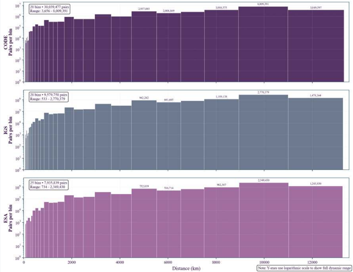
Figure 3. Logarithmic Distance Binning Strategy: Three-panel visualization showing how correlation analysis is binned by distance for each analysis center (CODE, IGS, ESA). Each bin shows statistical power (pairs per bin) with TEP correlation length range highlighted. Logarithmic Y-axis reveals full dynamic range from ~10 to 100,000+ pairs per bin.
