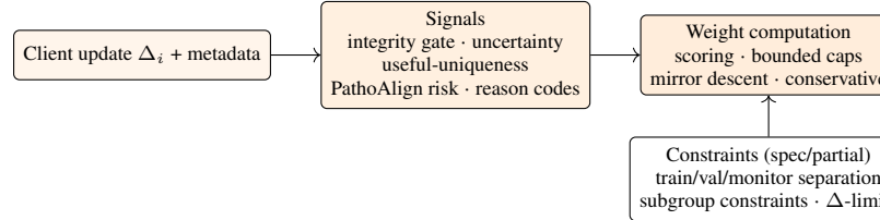
Figure 9: FAIR-WEIGHTS-H signal and constraint flow. Implemented: integrity gate, uncertainty penalty, useful-uniqueness, bounded weights, PathoAlign audit bridge, conservative mode. Specification-only or partial: training/validation/ monitoring weight separation, difficulty adjustment, Shapley-style contribution, subgroup constraints, weight-change limits. No established performance or fairness superiority (see Section 7).
