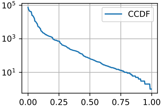
CCDF of function verification times
