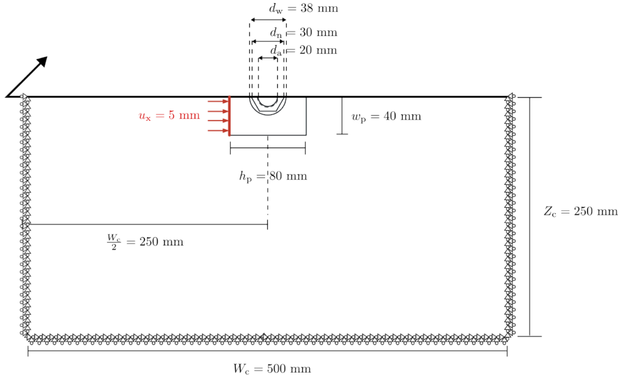
Figure 2: Top view of the model including the plane of symmetry z = 0 , across which the model and the loading are symmetric. The prescribed displacement u_x = 5 mm is distributed over the eleven nodes of the plate edge set plate_left_loading .
