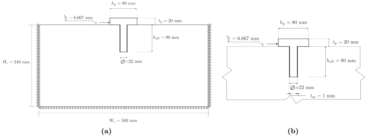
Figure 5: Bonded anchor model with the merged anchor-plate connection. a Section on the symmetry plane z = 0 , together with the boundary conditions of the concrete slab; the horizontal displacement u_x is introduced on the negative- x edge of the steel plate, at the height t_p/3 = 6.667 mm above the concrete surface, and the shaft terminates flush with the plate top at y = t_p . b Detail near the anchor: mortar thickness t_m , borehole diameter d_h = d_a + 2t_m and plate thickness t_p ; the plate hole is coincident with the shaft.
