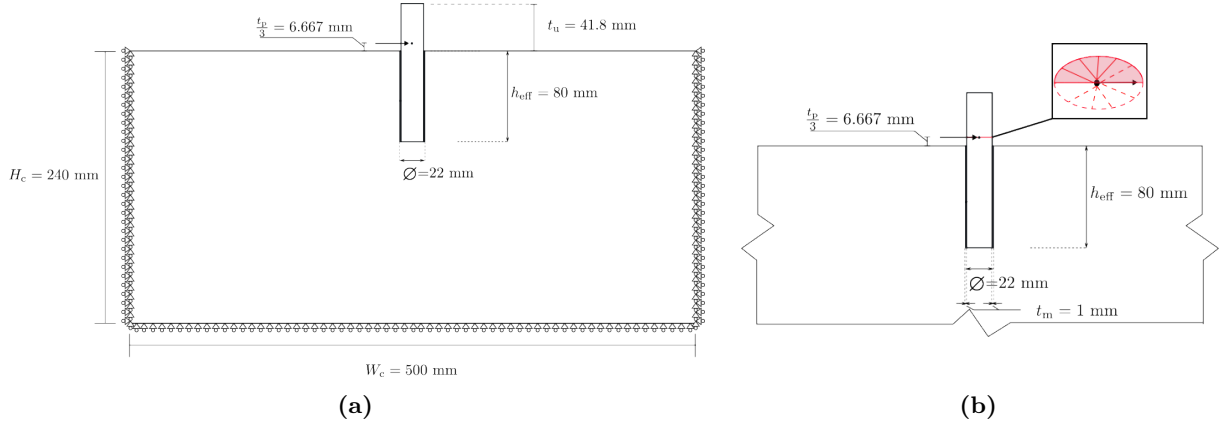
Figure 3: Bare bonded-anchor model. a Section on the symmetry plane z = 0 , together with the boundary conditions of the concrete slab; the dot marks the reference node of the rigid cross-section, on the anchor axis at t_p/3 = 6.667 mm above the concrete surface, where the horizontal displacement is prescribed. b Detail near the anchor: mortar thickness t_m , borehole diameter d_h = d_a + 2t_m , and the plane t_p/3 on which the displacement is prescribed. The inset shows the complete shaft cross-section at this plane: the central reference node lies on the anchor axis, and the dashed red spokes indicate the kinematic coupling of the section nodes to this node.
