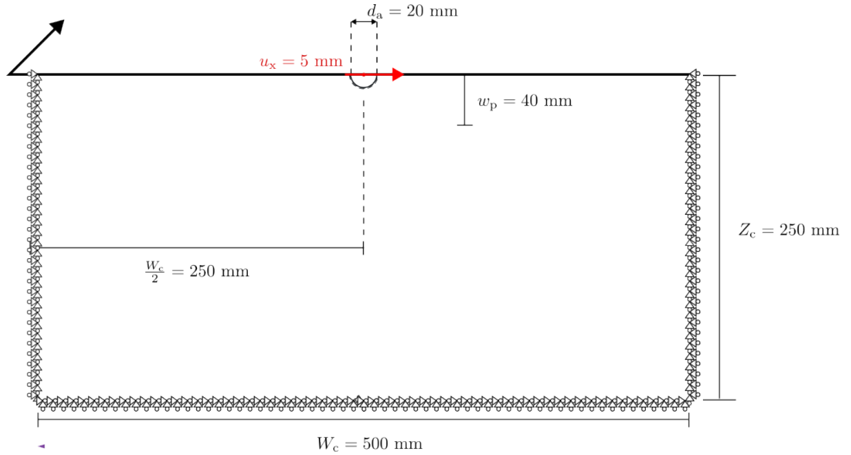
Figure 4: Top view of the model including the plane of symmetry z = 0 , across which the model and the loading are symmetric. The prescribed displacement u_x = 5 mm is applied at the single reference node of the rigid cross-section, which lies on the anchor axis.
