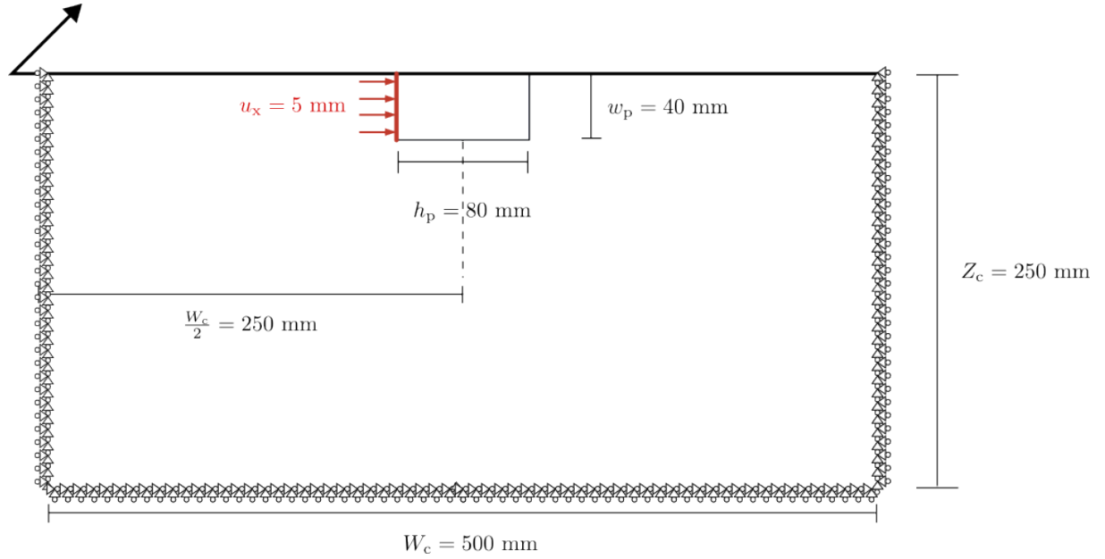
Figure 6: Top view of the model including the plane of symmetry z = 0 , across which the model and the loading are symmetric. The prescribed displacement u_x = 5 mm is distributed over the twelve nodes of the plate edge set plate_left_loading .
