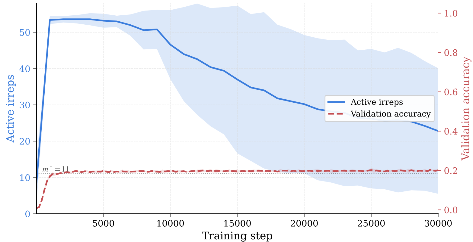
Irreps vs. \ generalisation ( p=113 , f_{\text{train}}=0.2 )
