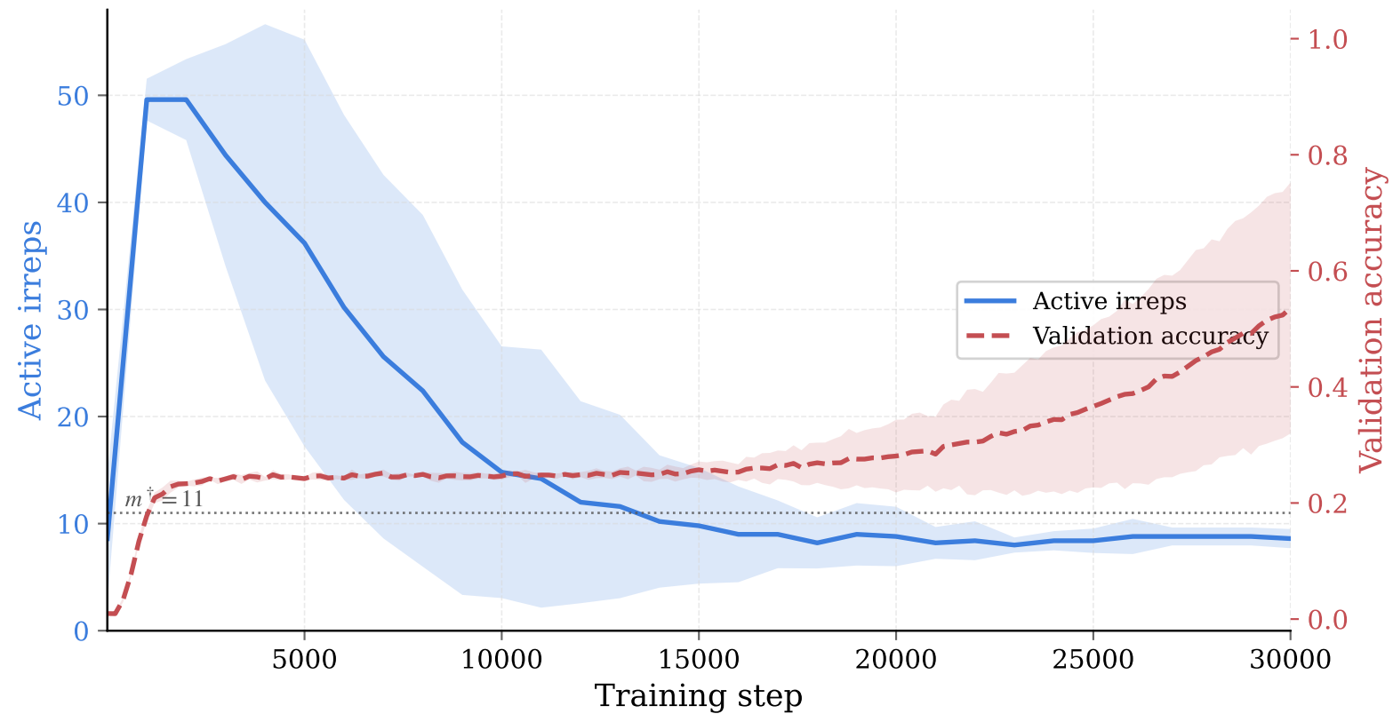
Irreps vs. \ generalisation ( p = 113 , f_{\text{train}} = 0.25 )
