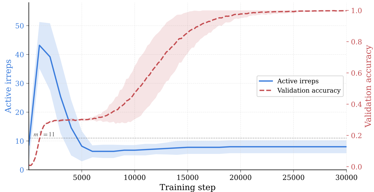
Irreps vs. \ generalisation ( p=113 , f_{\text{train}}=0.3 )
