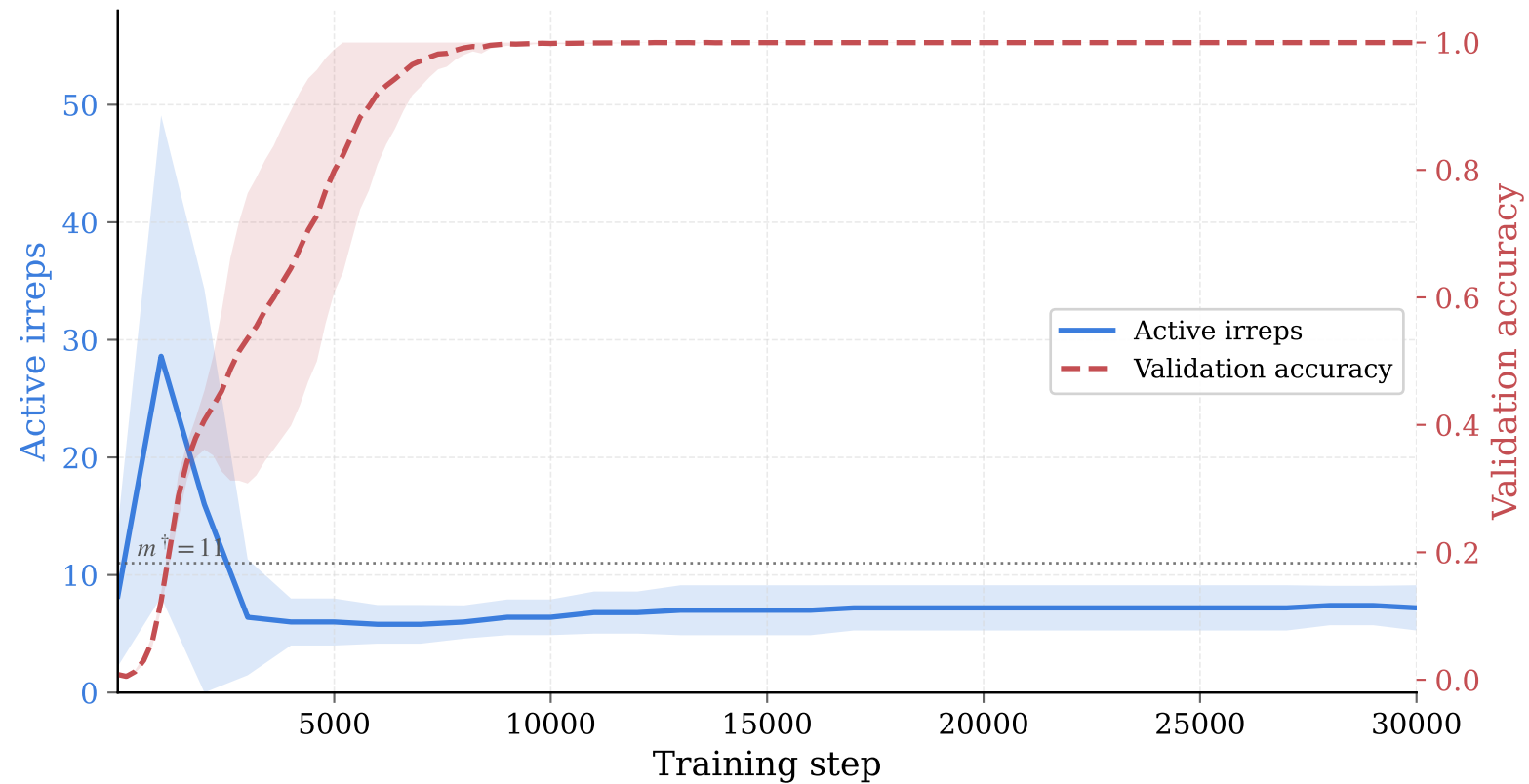
Irreps vs. \ generalisation ( p=113 , f_{\text{train}}=0.4 )
