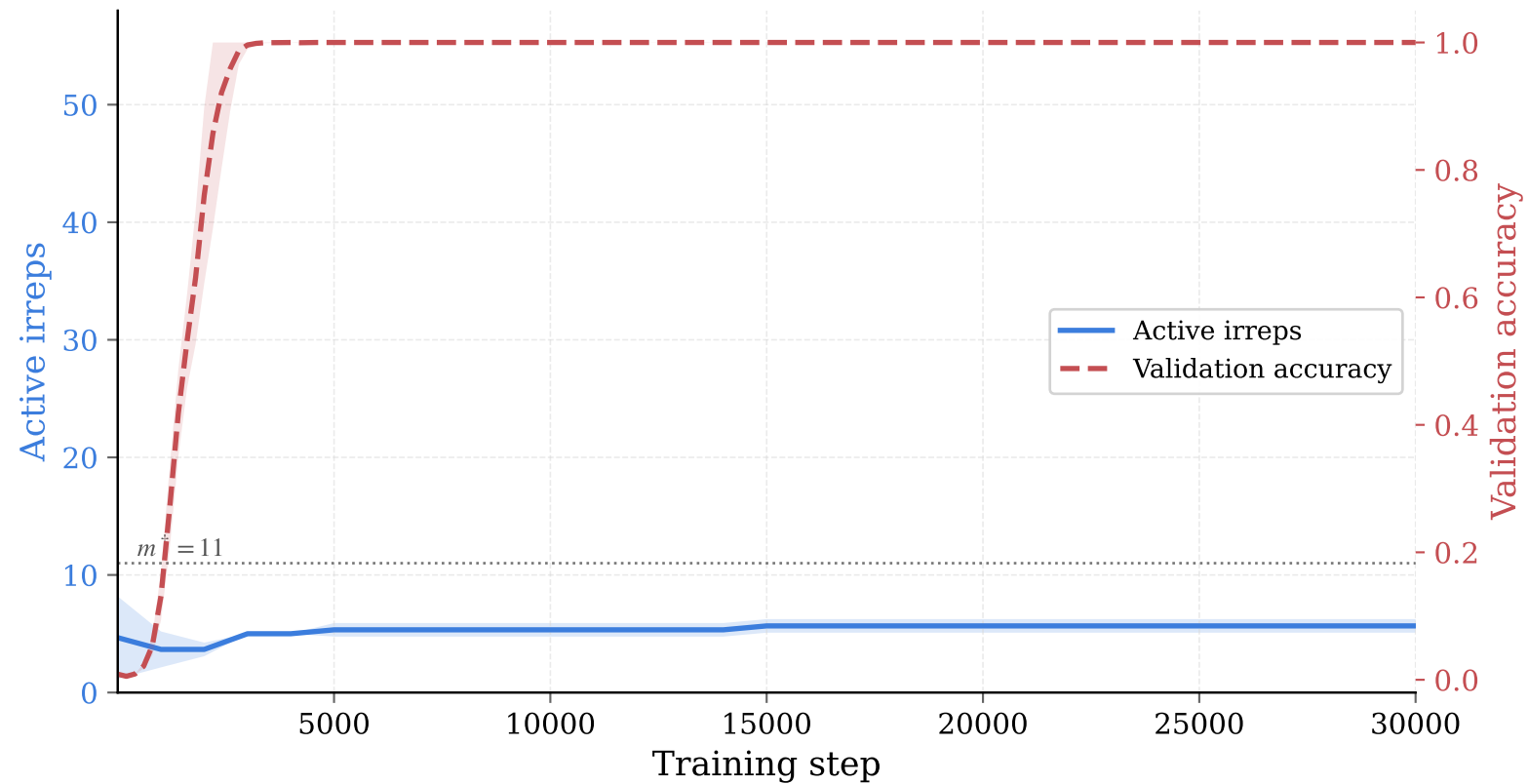
Irreps vs. \ generalisation ( p=113 , f_{\text{train}}=0.5 )
