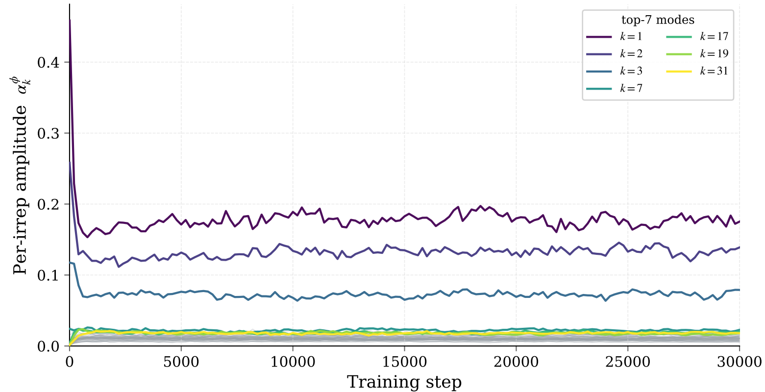
Spectrum collapse on V^* : top-7 modes survive ( f_{\text{train}}=0.1 , seed = 2)
