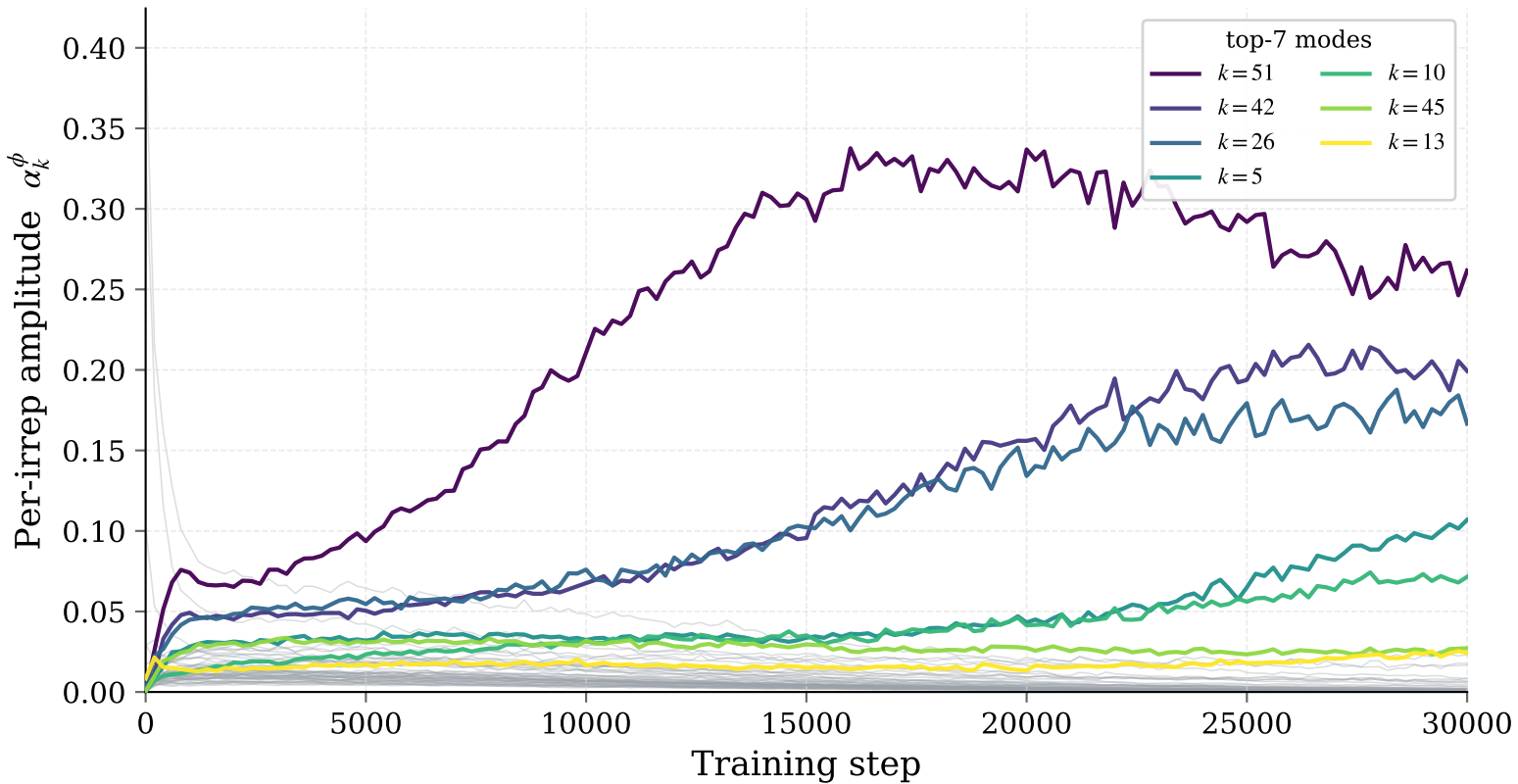
Spectrum collapse on V^* : top-7 modes survive ( f_{\text{train}}=0.25 , seed =4)
