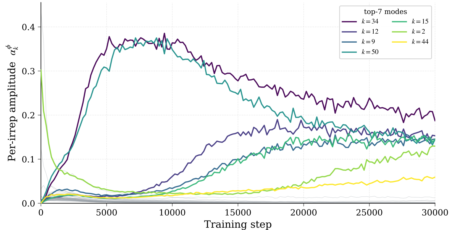
Spectrum collapse on V^* : top-7 modes survive ( f_{\text{train}}=0.3 , seed = 1)
