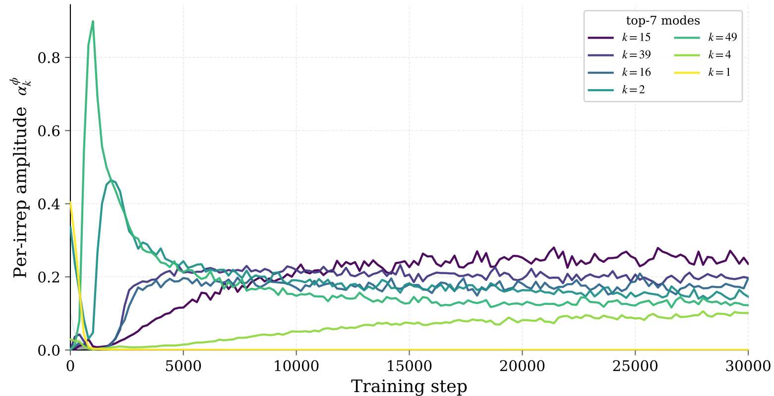
Spectrum collapse on V^* : top-7 modes survive ( f_{\text{train}}=0.5 , seed = 4)
