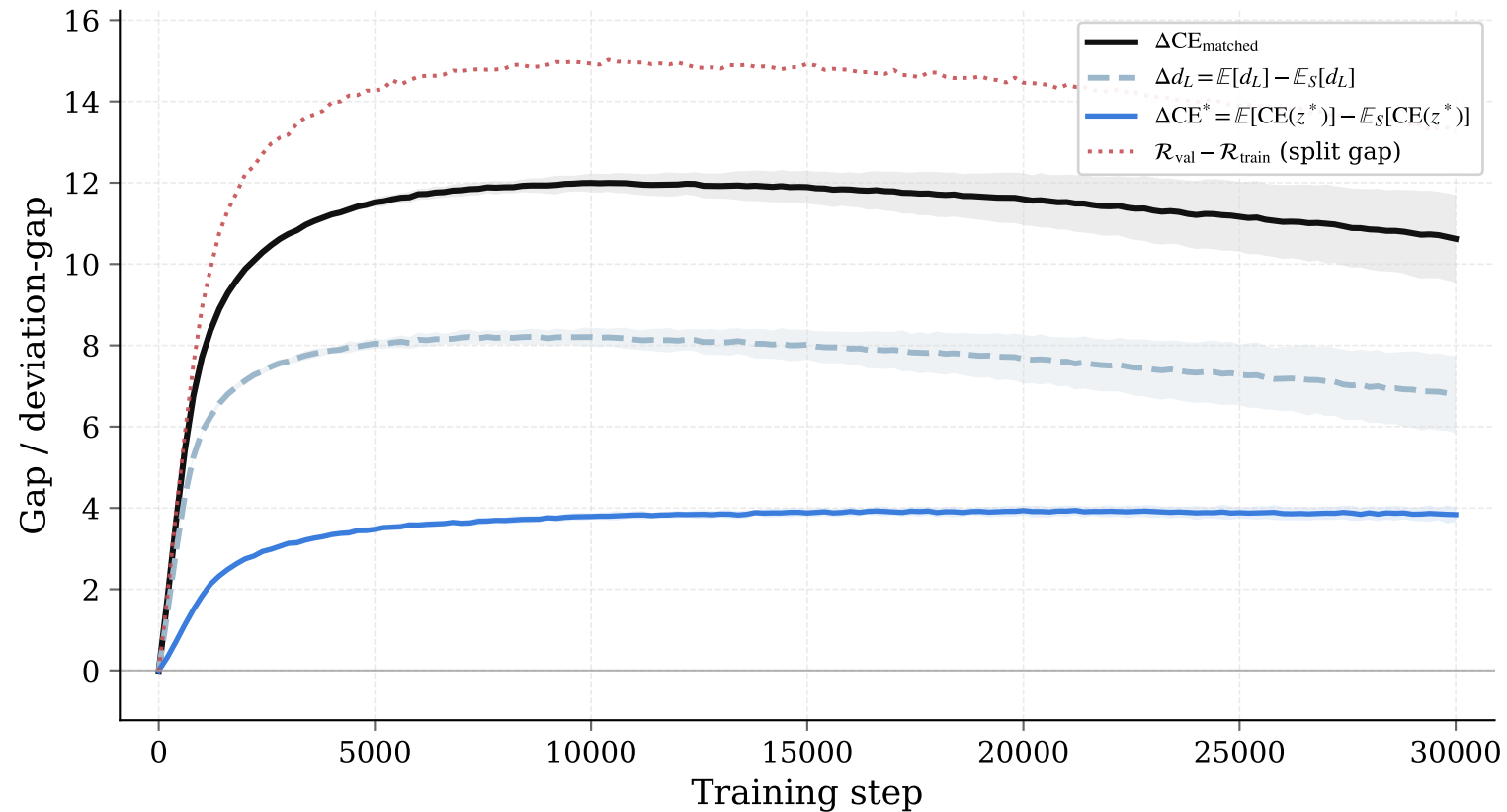
Theorem 3 decomposition ( f_{\text{train}}=0.2 , runs=5)
