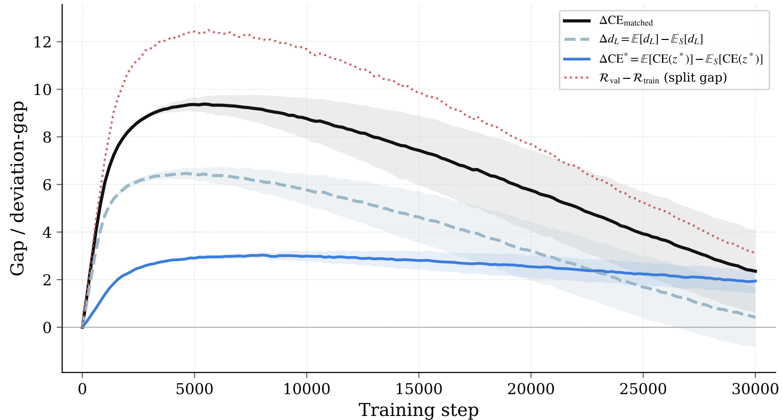
Theorem 3 decomposition ( f_{\text{train}}=0.25 , runs=5)
