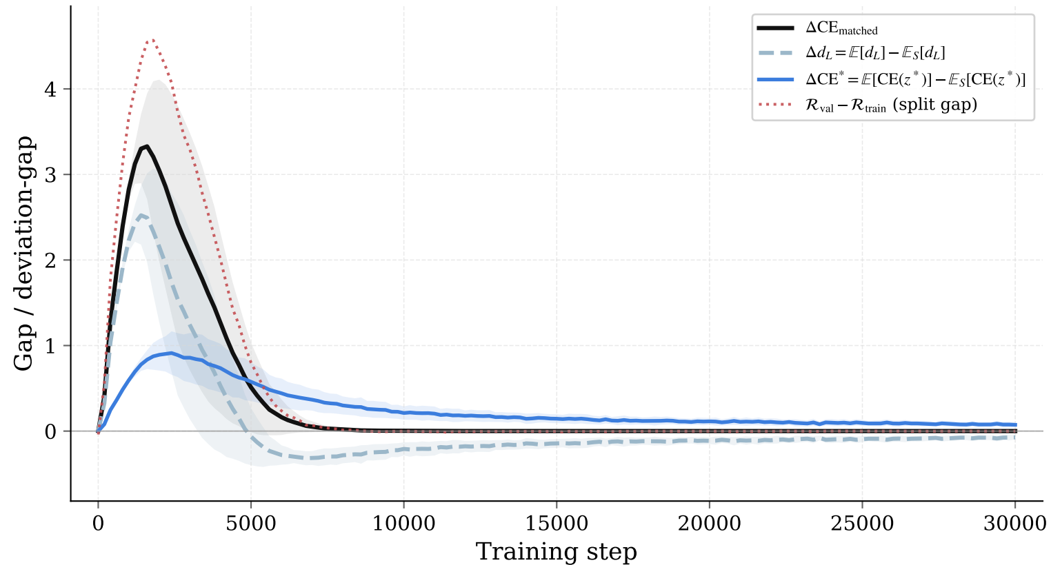
Theorem 3 decomposition ( f_{\text{train}}=0.4 , runs=5)
