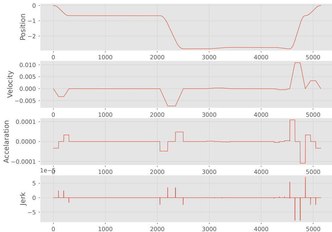
Trajectory profiles of joint 0boxwithPIP trapez
