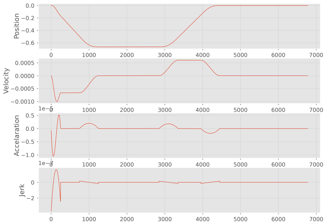
Trajectory profiles of joint 0box
