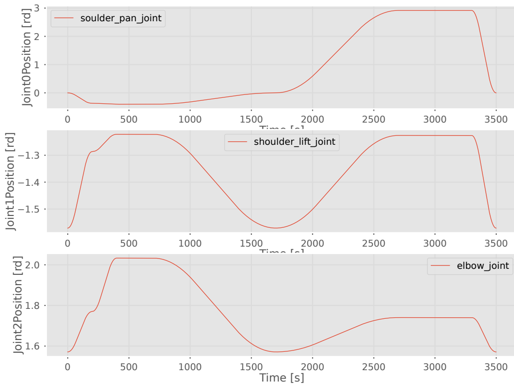
Trajectory joint profiles of duck with PIP_trapezoidal
