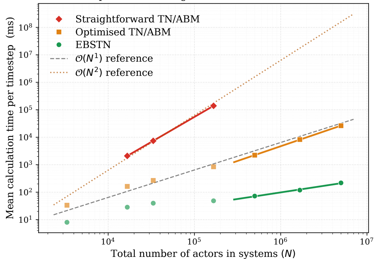
Computational scaling: EBSTN vs TN/ABM variants
