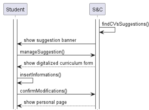
Figure 25: Sequence diagram of "Apply a suggestion to the digitalized curriculum vitae" use case.
