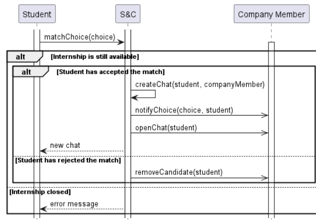
Figure 29: Sequence diagram of "Student responds to company's match proposal" use case.
