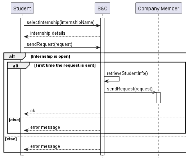
Figure 27: Sequence diagram of "Student sends a match proposal" use case.
