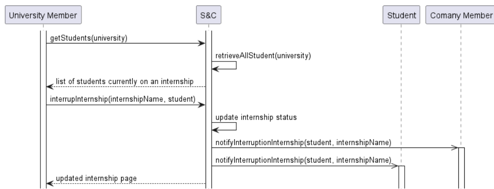
Figure 38: Sequence diagram of " University member interrupts an internship " use case.
