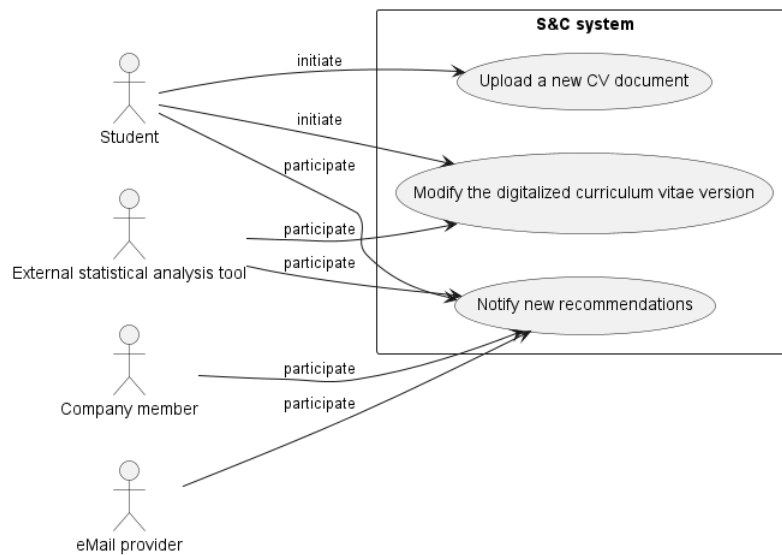
Figure 7: Use cases from UC11 to UC13.
