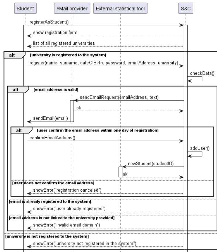
Figure 14: Sequence diagram of "Registration of a student" use case.
