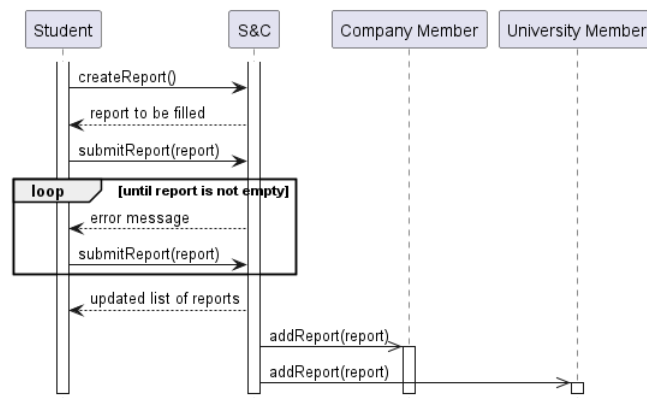
Figure 35: Sequence diagram of "Student writes a report" use case.
