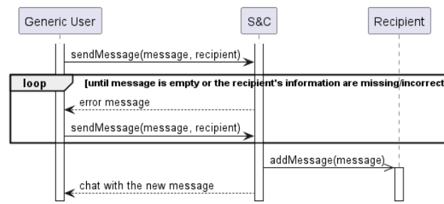
Figure 34: Sequence diagram of "User writes a message" use case.
