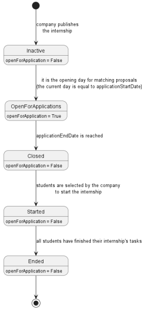
Figure 2: State diagram of Internship class.
