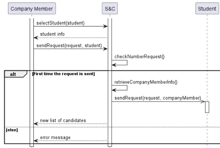
Figure 28: Sequence diagram of "Company member sends a match proposal" use case.
