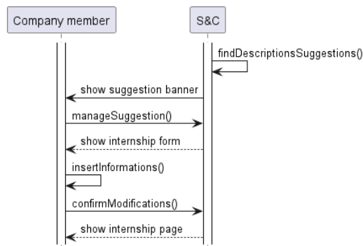
Figure 26: Sequence diagram of "Apply a suggestion to the internship description" use case.
