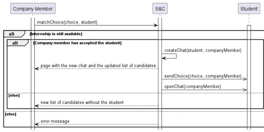
Figure 30: Sequence diagram of "Company member responds to student's match proposal" use case.
