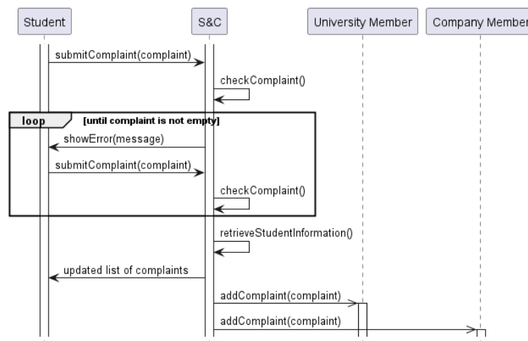
Figure 37: Sequence diagram of "Student writes a complaint" use case.
