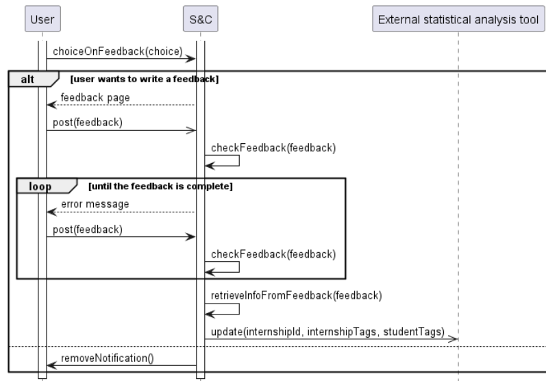
Figure 39: Sequence diagram of "Student or company member posts a feedback" use case.
