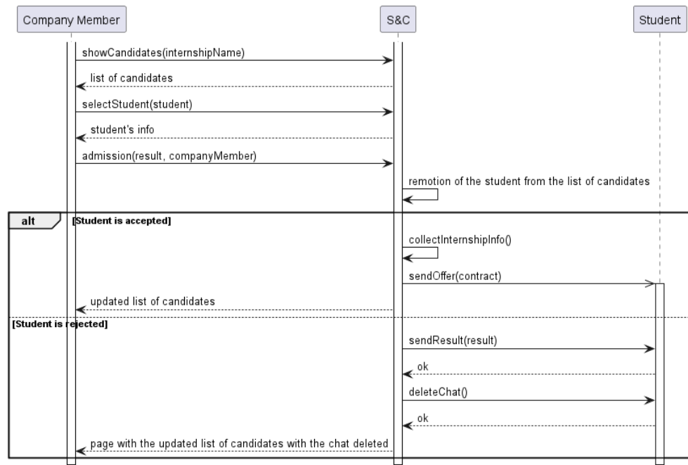
Figure 32: Sequence diagram of "Company member communicates the result of the interview" use case.
