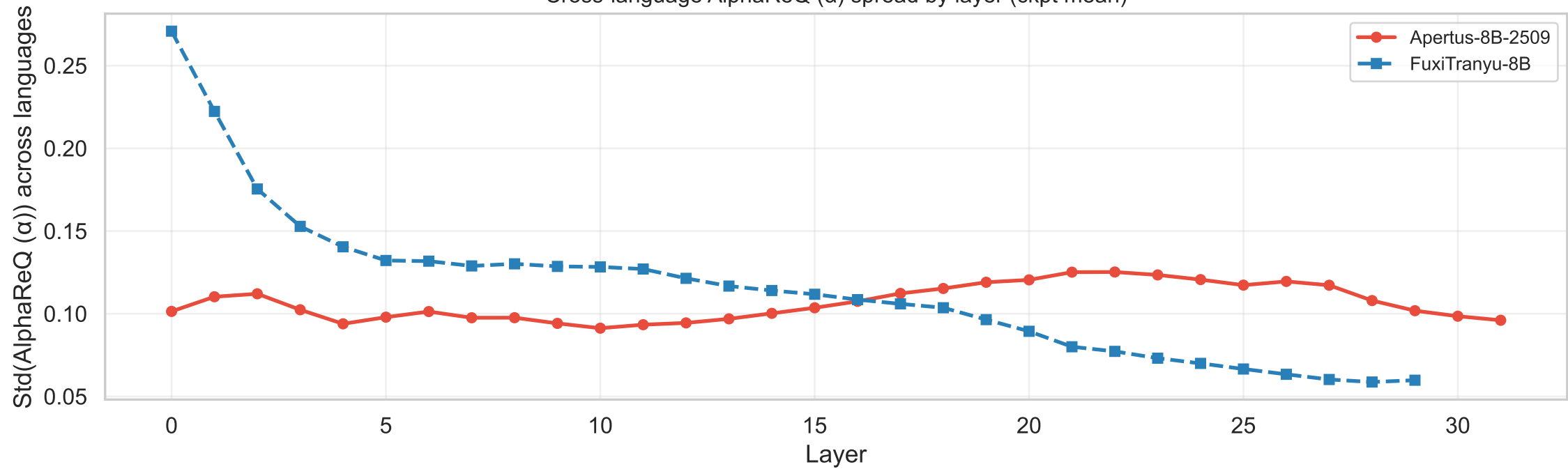
Cross-language AlphaReQ ( \alpha ) spread by layer (ckpt mean)
