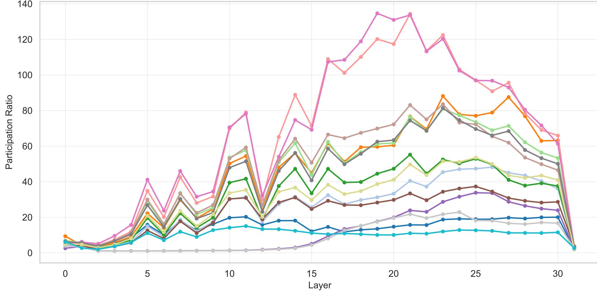
Participation Ratio by layer — all languages (ckpt mean) | agg=last [Apertus-8B-2509]
