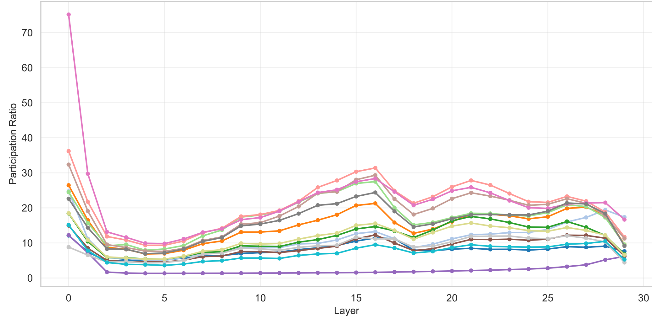
Participation Ratio by layer — all languages (ckpt mean) | agg=last [FuxiTranyu-8B]
