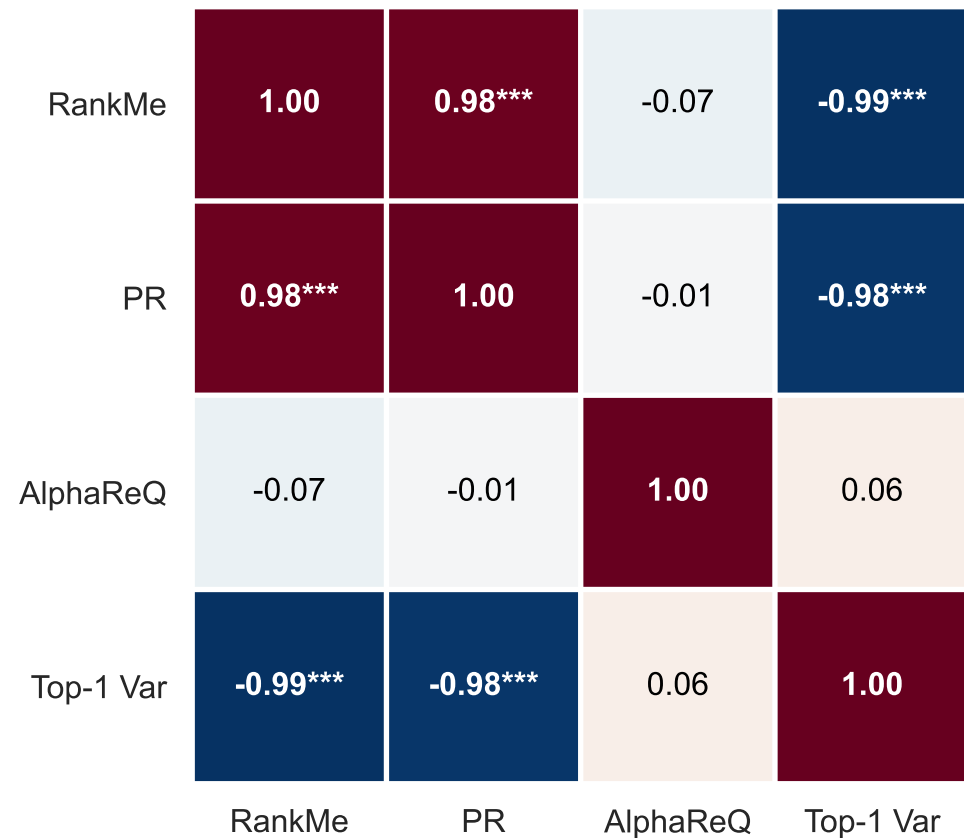
Apertus-8B-2509 (n = 32 layers)
