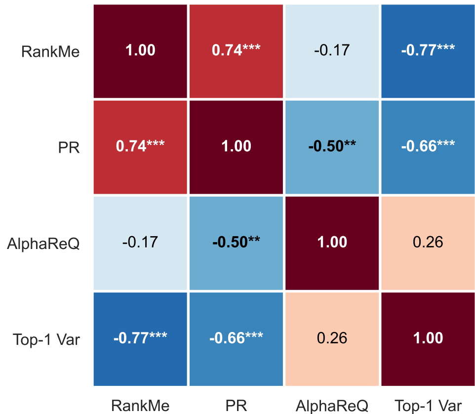
FuxiTranyu-8B (n = 30 layers)
