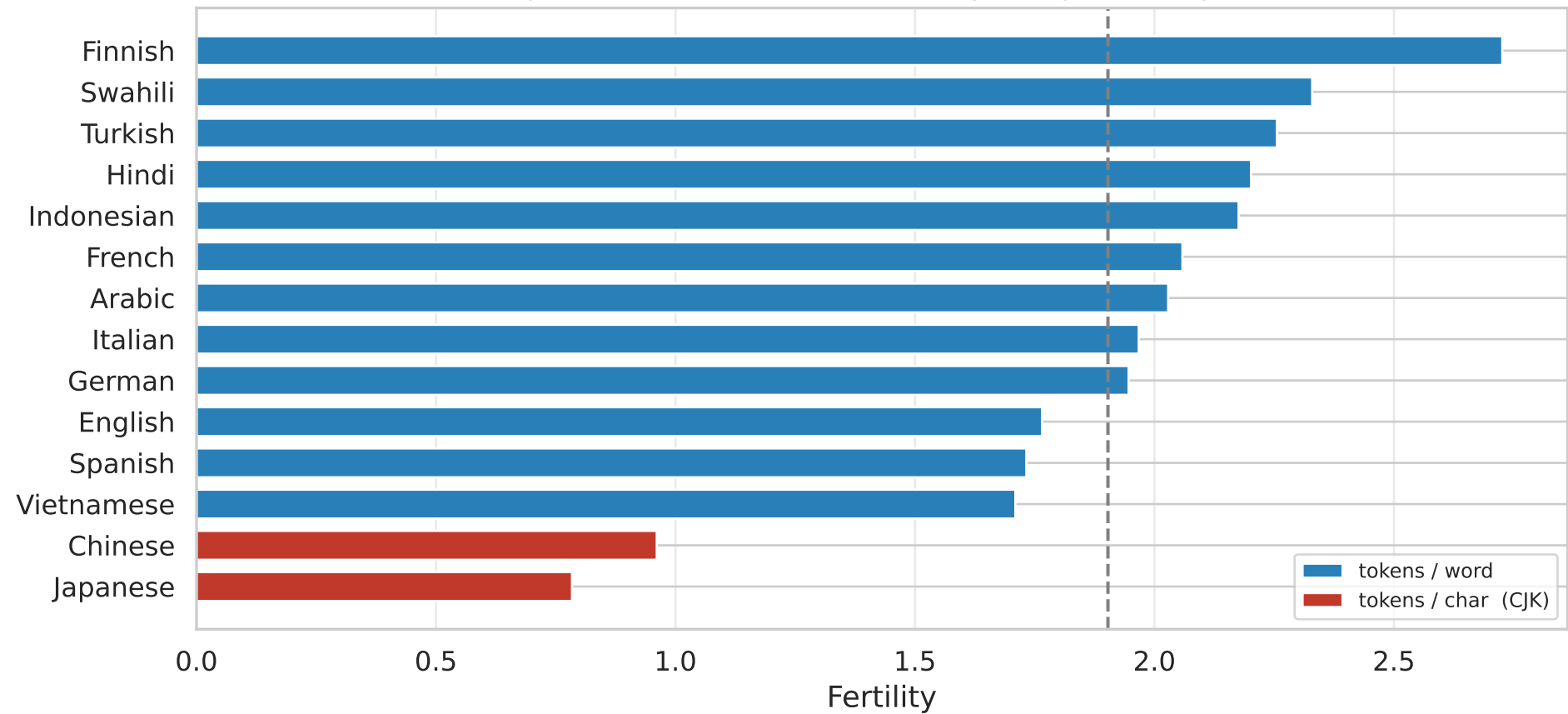
[Apertus-8B-2509] Tokenizer Fertility (Wikipedia samples)
