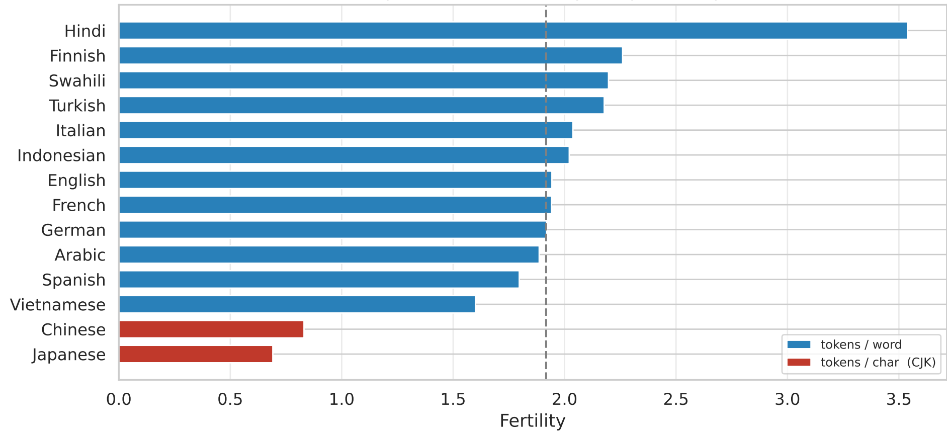
[FuxiTranyu-8B] Tokenizer Fertility (Wikipedia samples)
