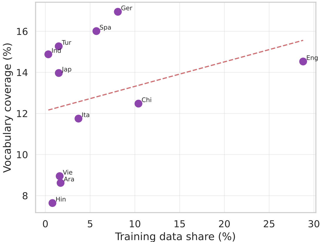
[FuxiTranyu-8B] Training Distribution vs. Vocabulary Coverage Pearson r=0.31 ( p=0.356 ) | Spearman \rho=0.24 ( p=0.484 )
