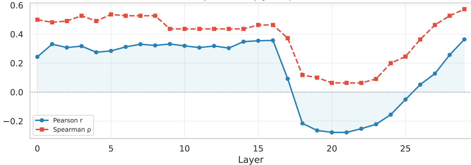
[FuxiTranyu-8B] Training Distribution vs. RankMe — Correlation Profile
