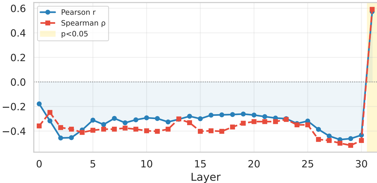
[Apertus-8B-2509] Fertility-RankMe Correlation Profile main | last-token | gold = p < 0.05
