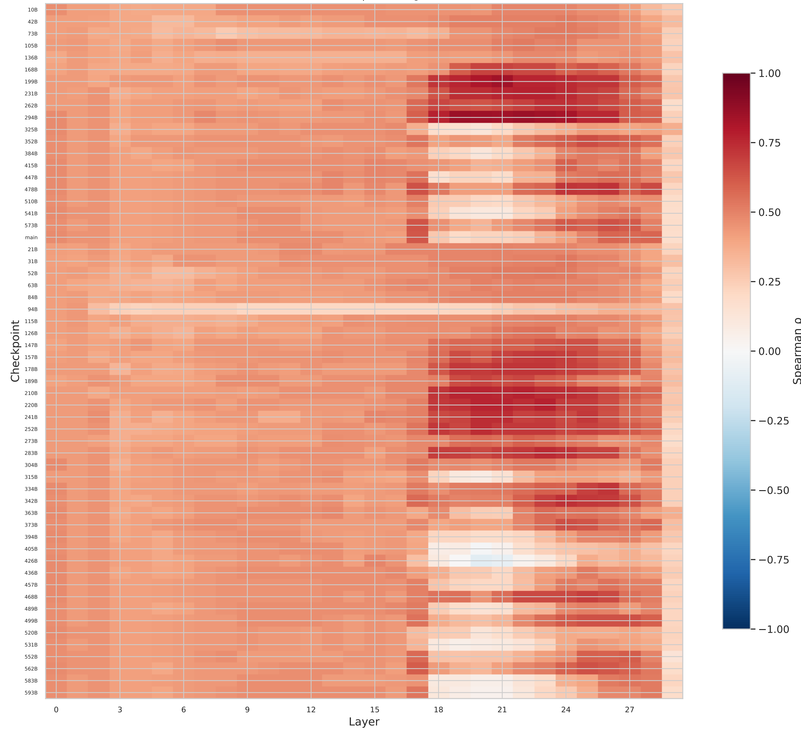
[FuxiTranyu-8B] Spearman \rho — Coverage vs. RankMe Blue: → lower RankMe | Red: → higher RankMe
