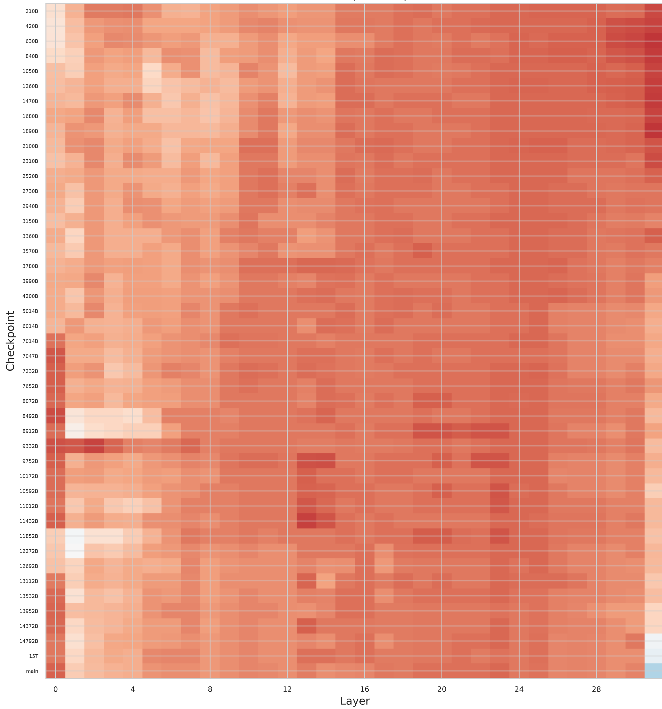
[Apertus-8B-2509] Spearman \rho — Coverage vs. RankMe Blue: → lower RankMe | Red: → higher RankMe
