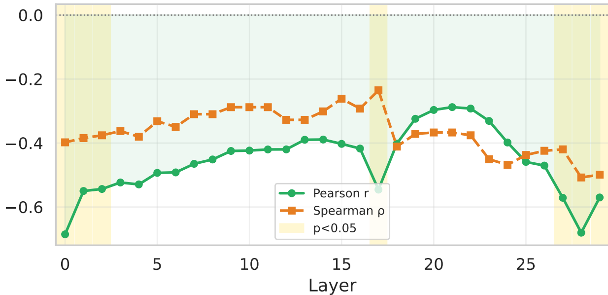
[FuxiTranyu-8B] Fertility-RankMe Correlation Profile (All languages) main | last-token | gold = p < 0.05
