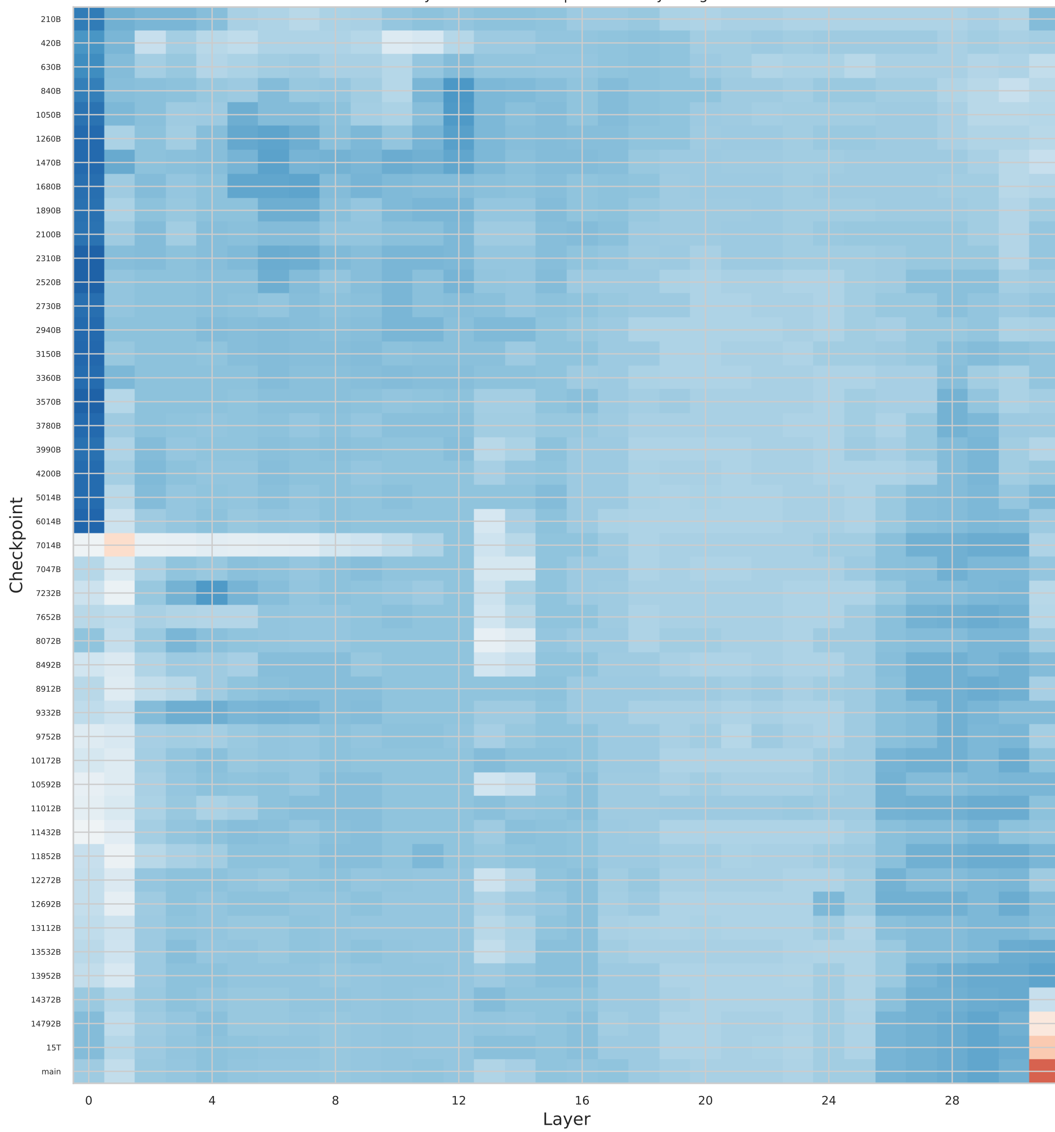
[Apertus-8B-2509] Spearman \rho — Fertility vs. RankMe Blue: fertility \rightarrow lower RankMe | Red: fertility \rightarrow higher RankMe
