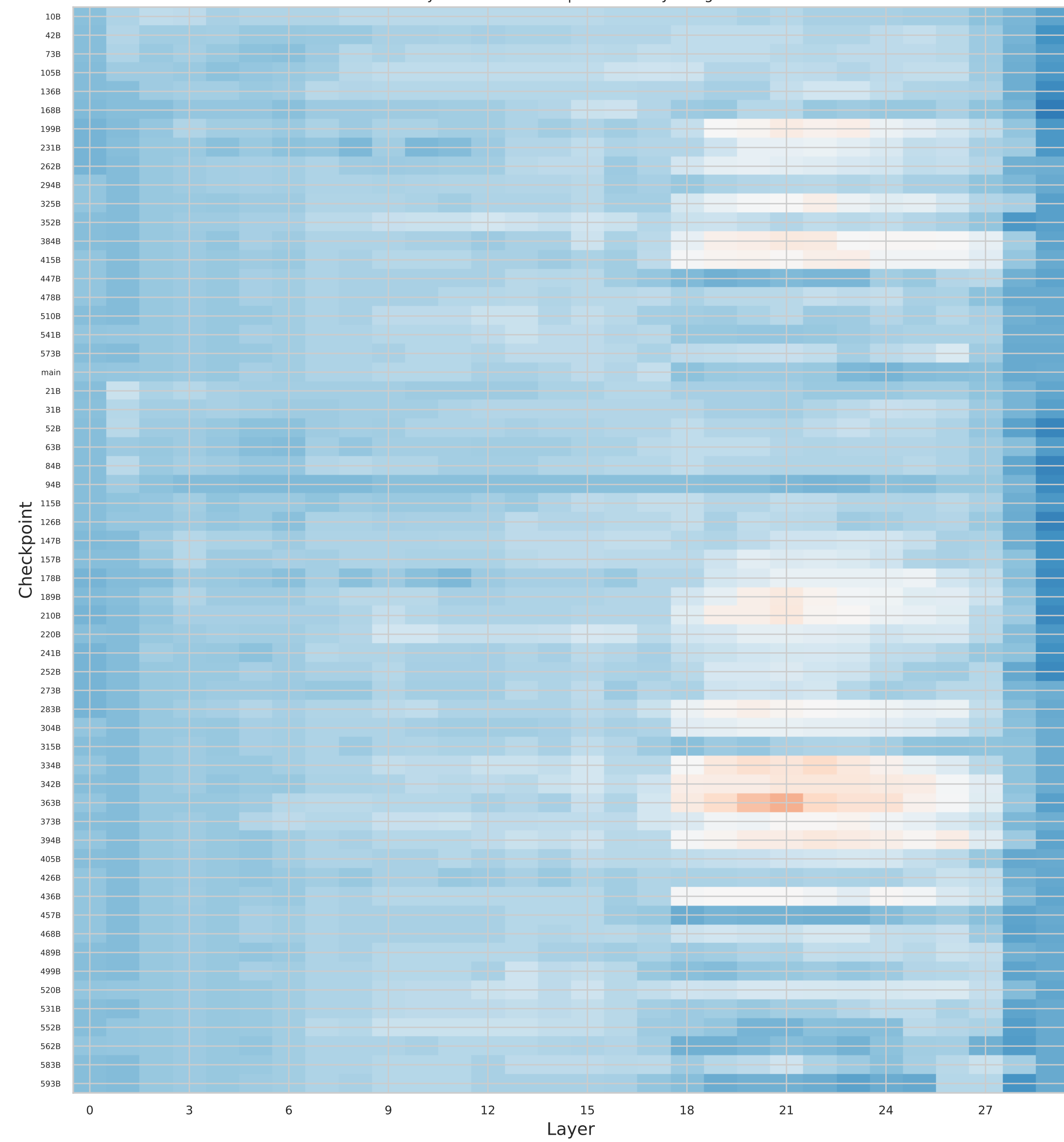
[FuxiTranyu-8B] Spearman \rho — Fertility vs. RankMe Blue: fertility \rightarrow lower RankMe | Red: fertility \rightarrow higher RankMe
