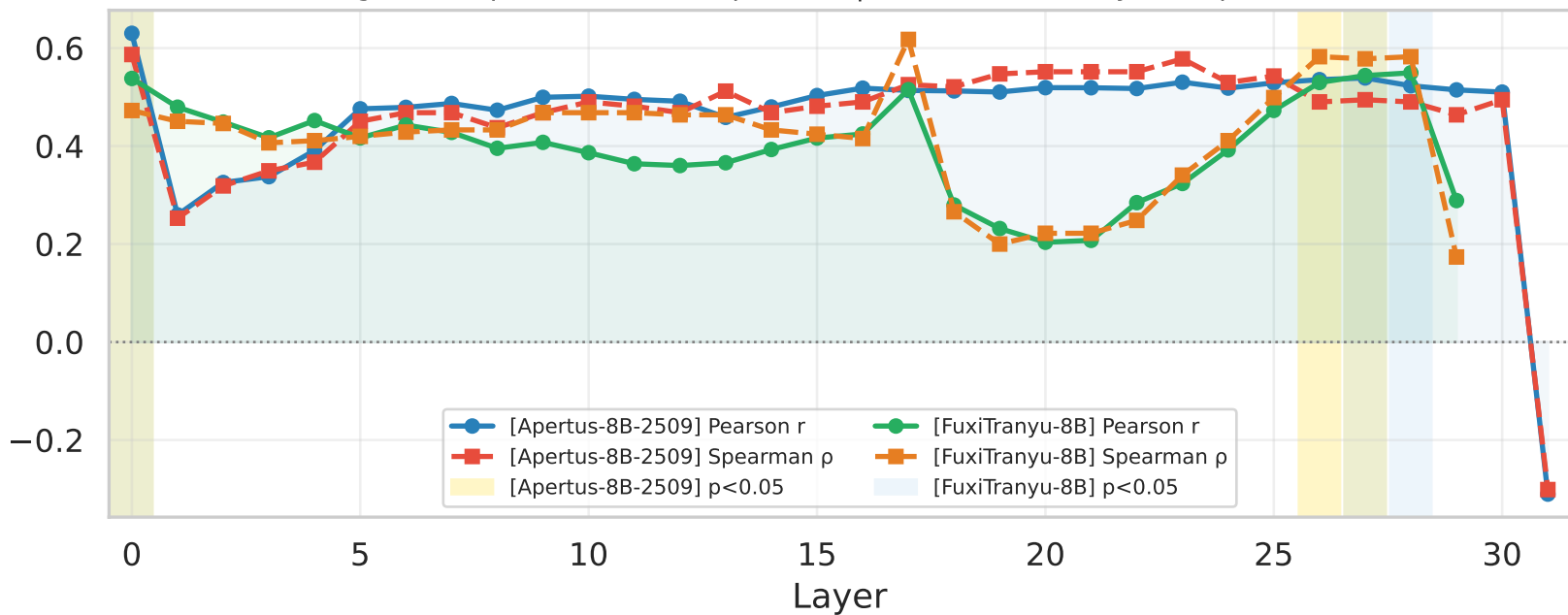
Coverage-RankMe Correlation Profile (All languages) gold = [Apertus-8B-2509] p < 0.05 | blue = [FuxiTranyu-8B] p < 0.05
