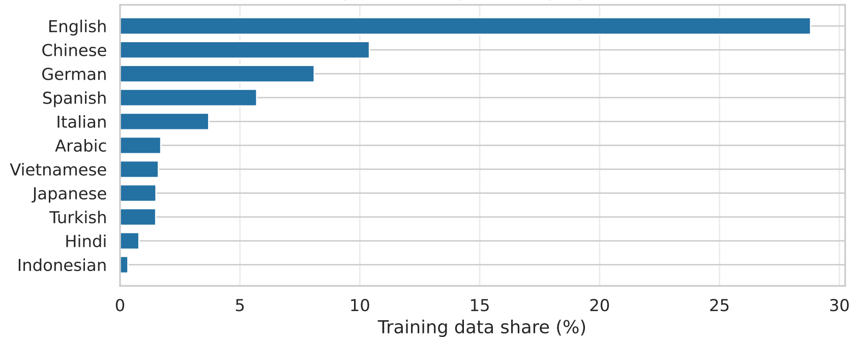
[FuxiTranyu-8B] Training Data Language Distribution
