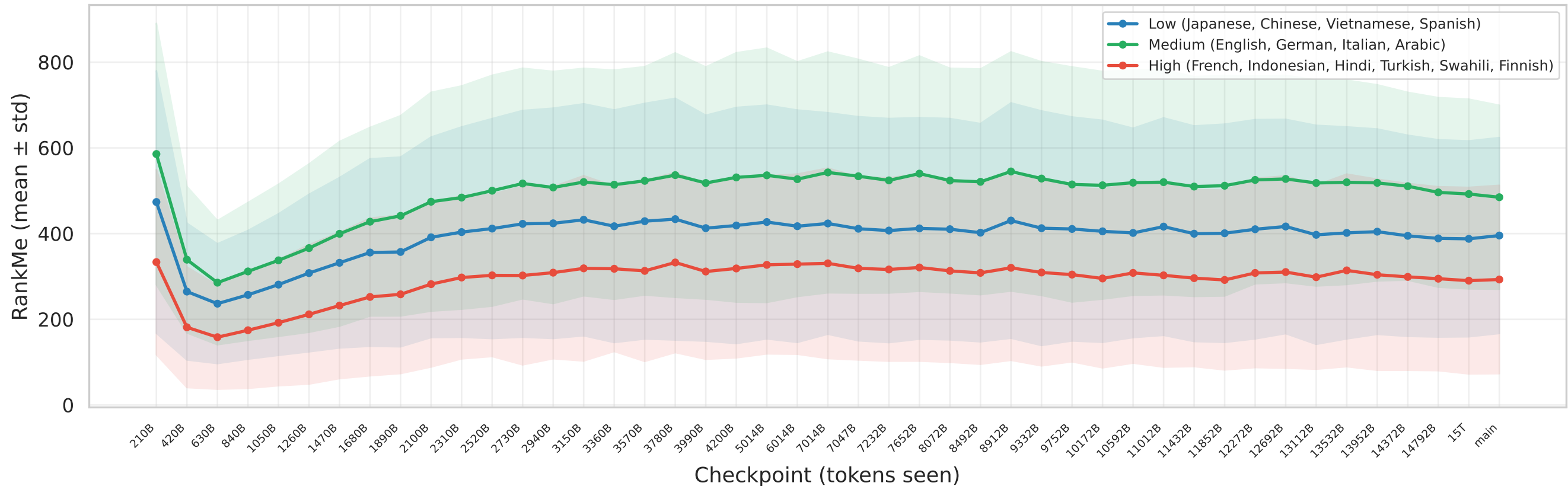
[Apertus-8B-2509] Training Dynamics by Fertility Tier layer 16 | last-token
