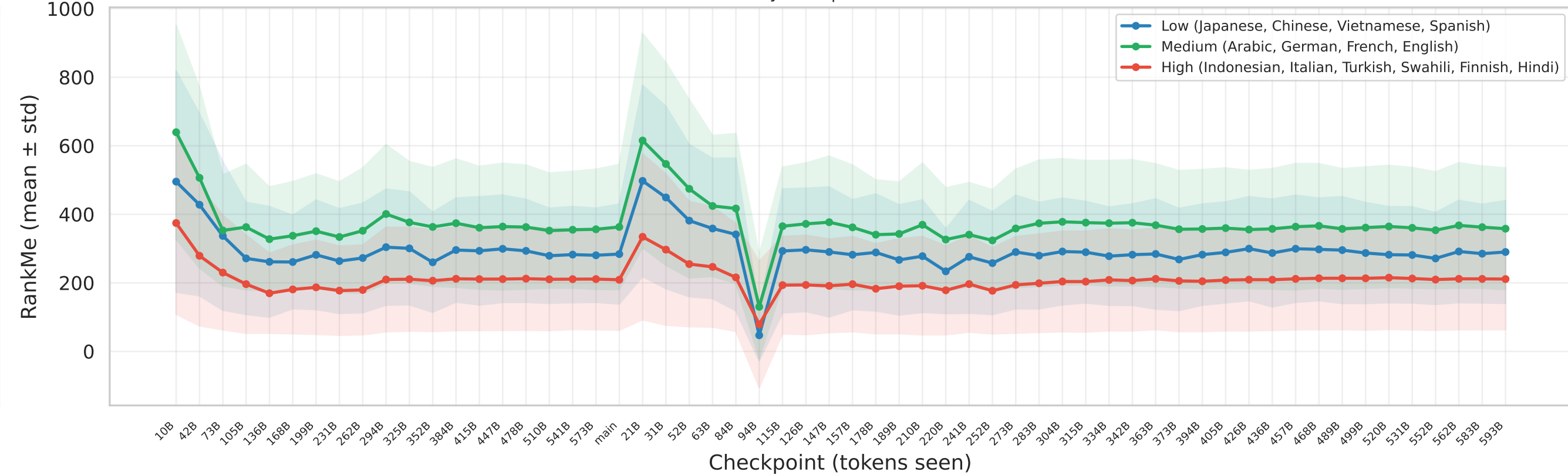
[FuxiTranyu-8B] Training Dynamics by Fertility Tier layer 15 | last-token
