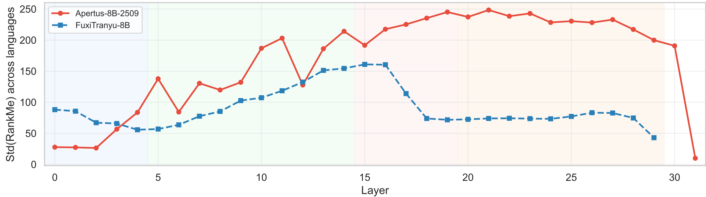
Cross-language RankMe spread by layer (checkpoint mean) Higher = languages more stratified at this depth
