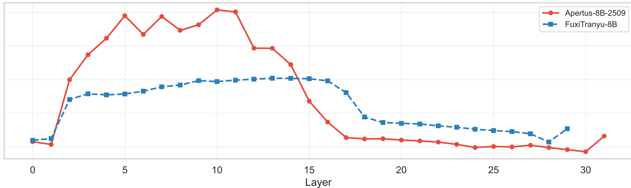
Cross-language Top-1 Variance spread by layer (ckpt mean) Higher = languages differ more in how spiked their representation is at this depth
