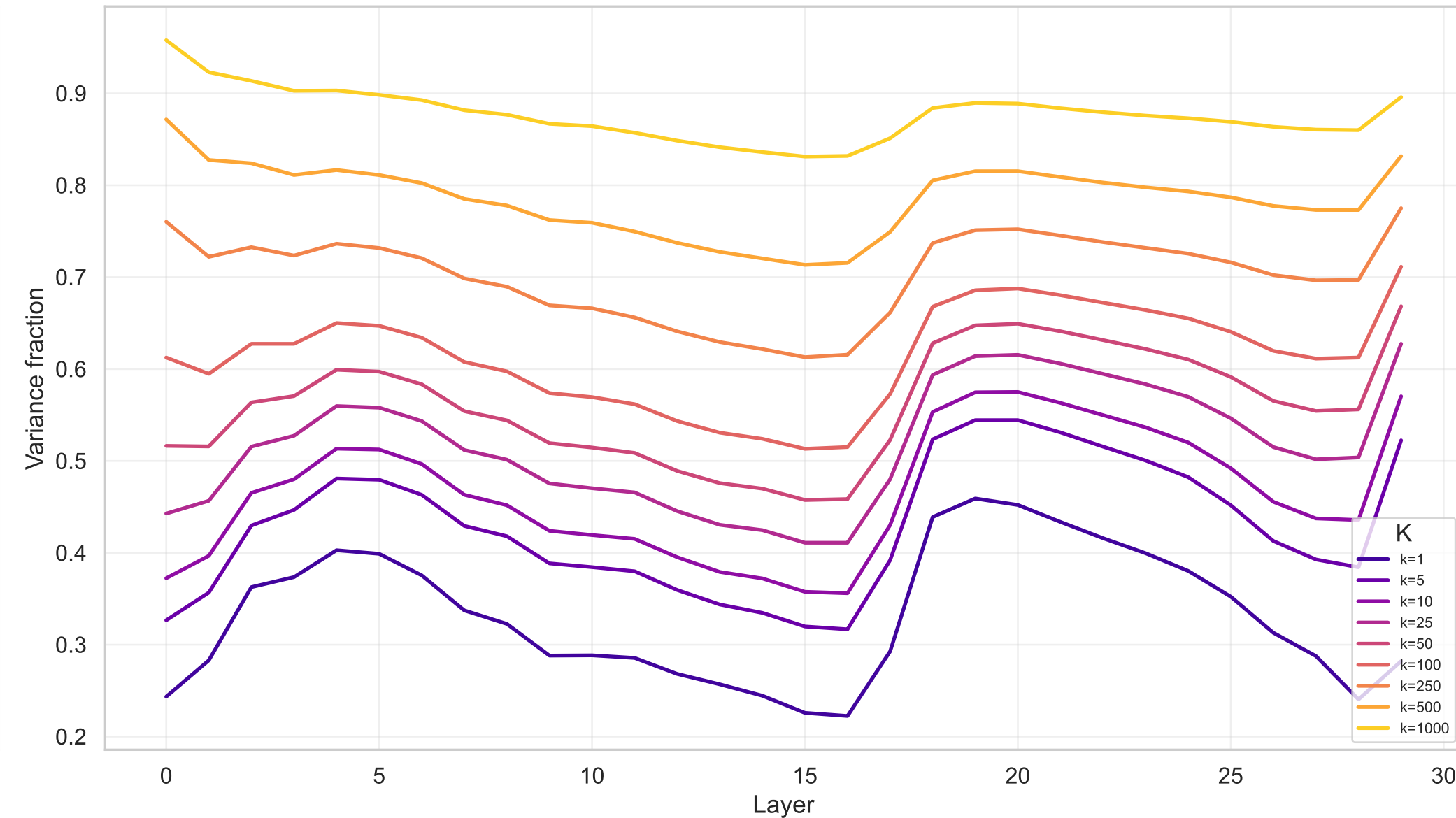
[FuxiTranyu-8B] Top-K variance by layer — English (ckpt mean)
