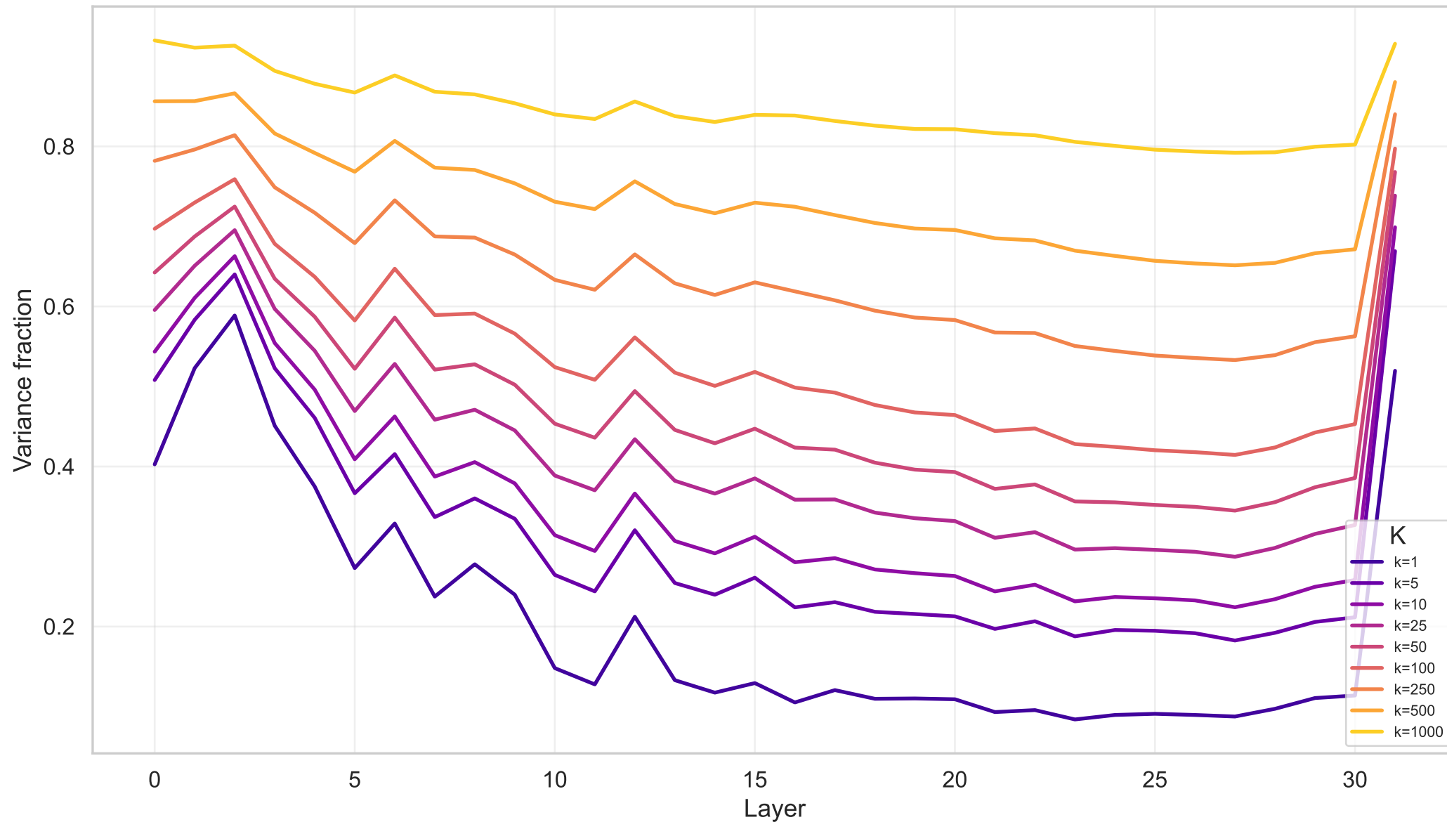
[Apertus-8B-2509] Top-K variance by layer — English (ckpt mean)
