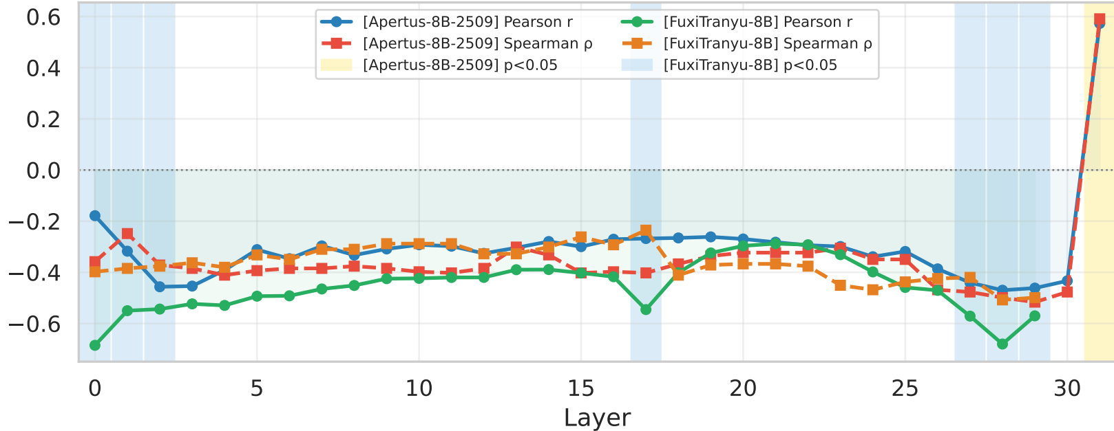
Fertility-RankMe Correlation Profile (All languages) gold = [Apertus-8B-2509] p < 0.05 | blue = [FuxiTranyu-8B] p < 0.05
