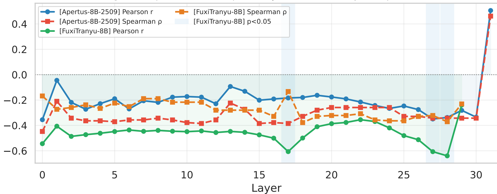
Fertility-RankMe Correlation Profile (Excluding Chinese & Japanese) gold = [Apertus-8B-2509] p < 0.05 | blue = [FuxiTranyu-8B] p < 0.05
