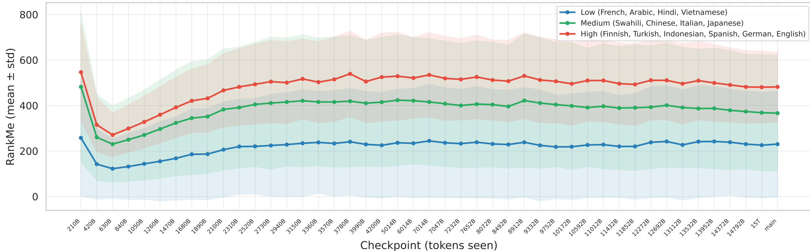
[Apertus-8B-2509] Training Dynamics by Coverage Tier layer 16 | last-token
