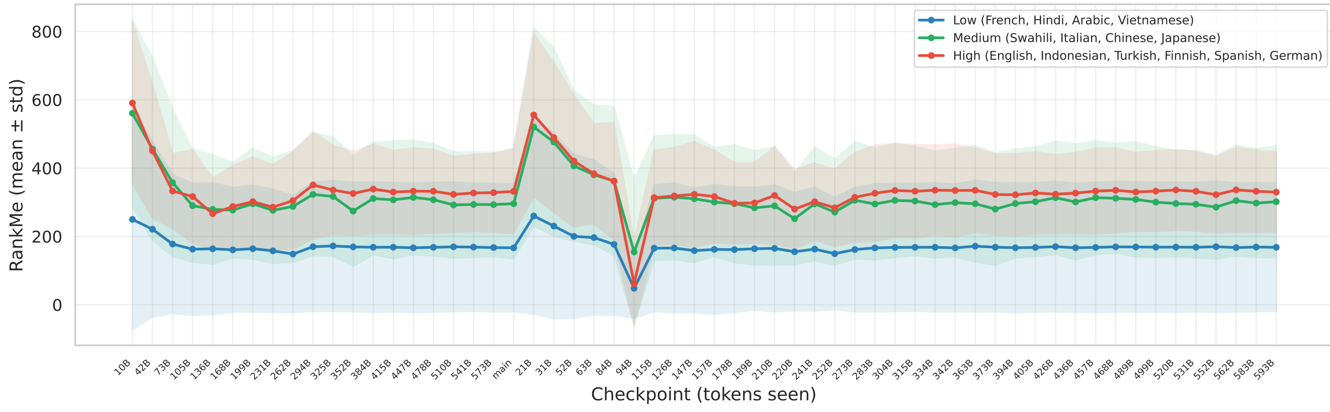
[FuxiTranyu-8B] Training Dynamics by Coverage Tier layer 15 | last-token
