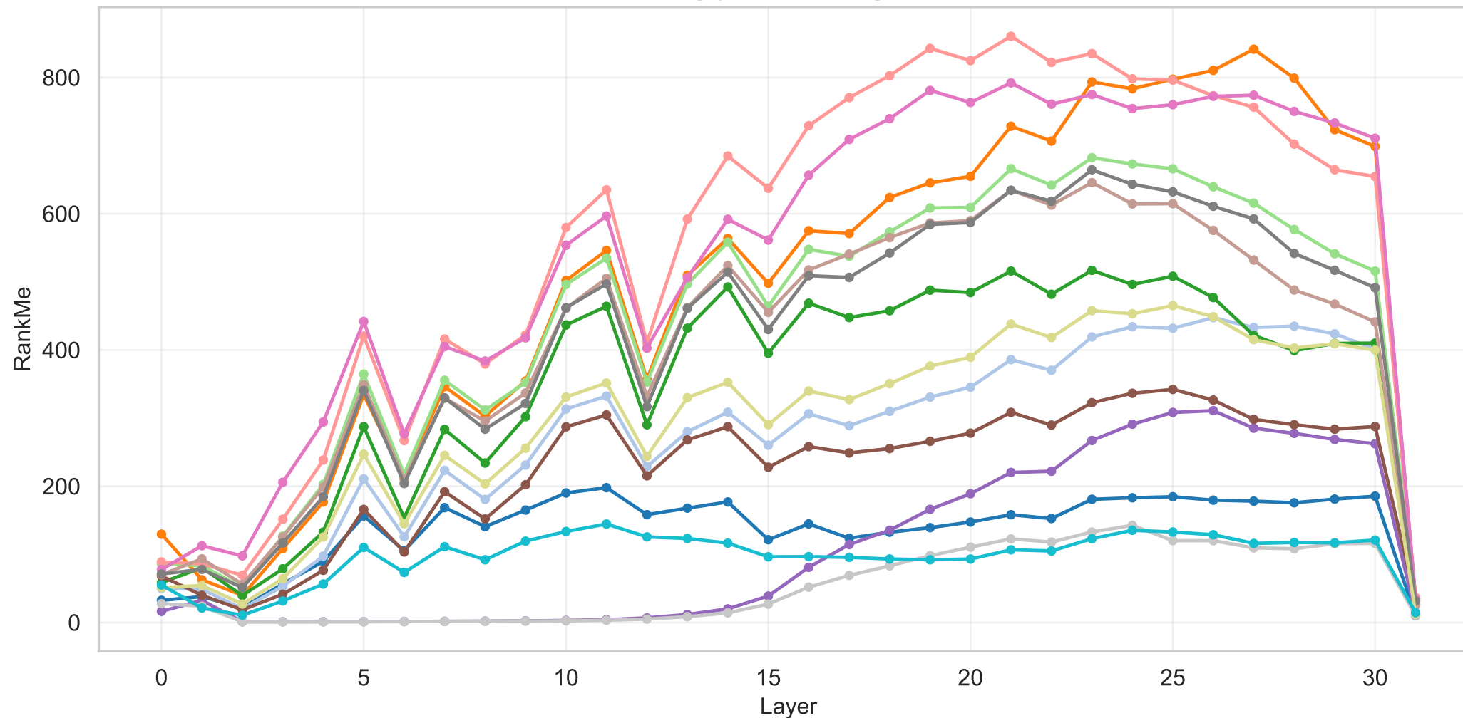
RankMe by layer — all languages (checkpoint mean) | agg=last [Apertus-8B-2509]
