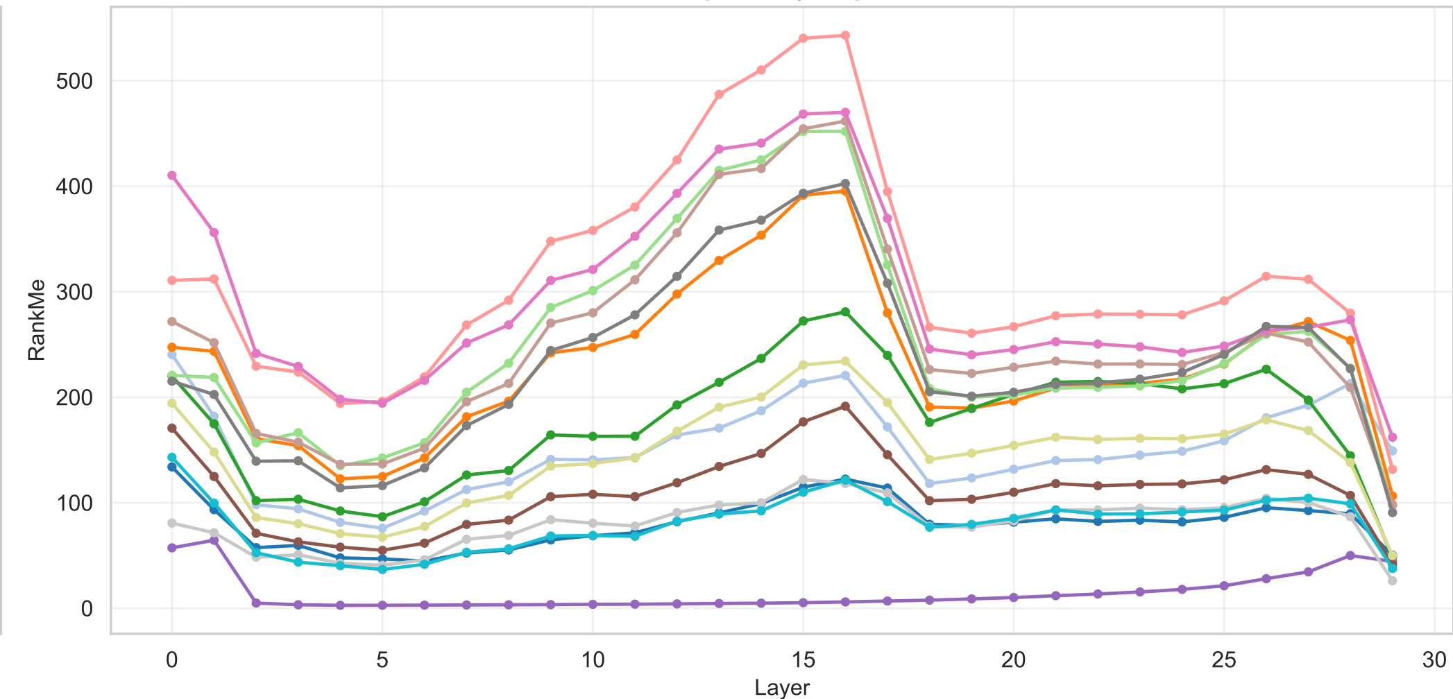
RankMe by layer — all languages (checkpoint mean) | agg=last [FuxiTranyu-8B]
