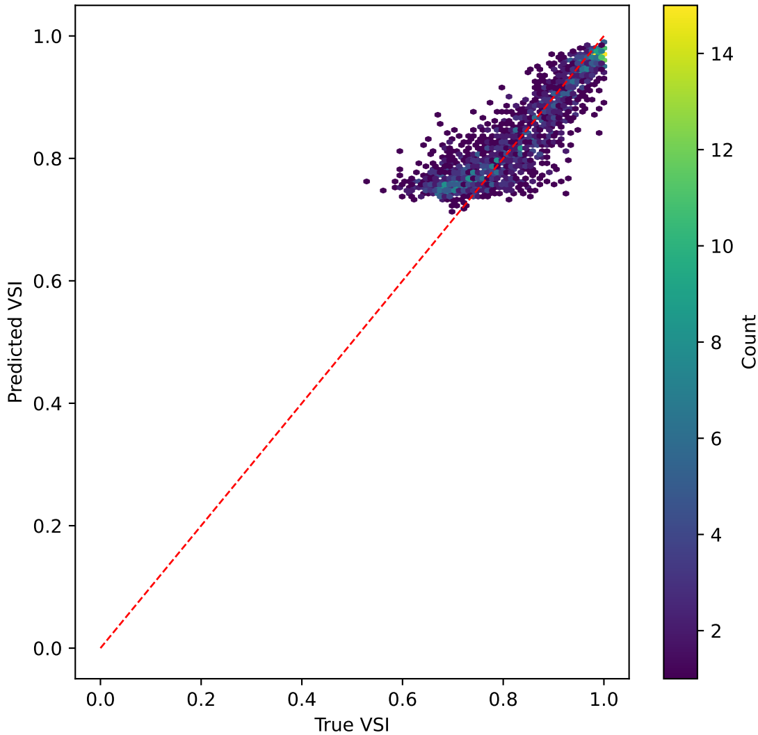
mobilenetv3 on VSI | R^2=0.615
