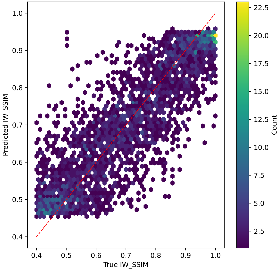
tinyvit on IW_SSIM | R^2=0.760
