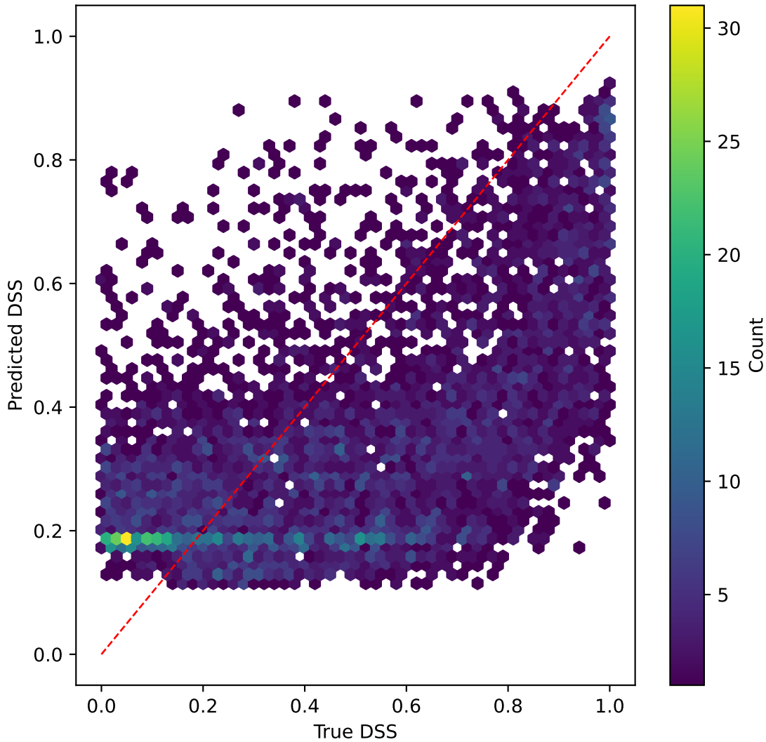
mobilevitv2 on DSS | R^2=0.188
