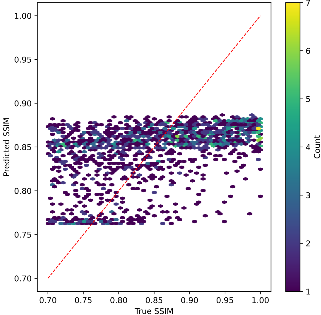
tinyvit on SSIM | R^2=0.161
