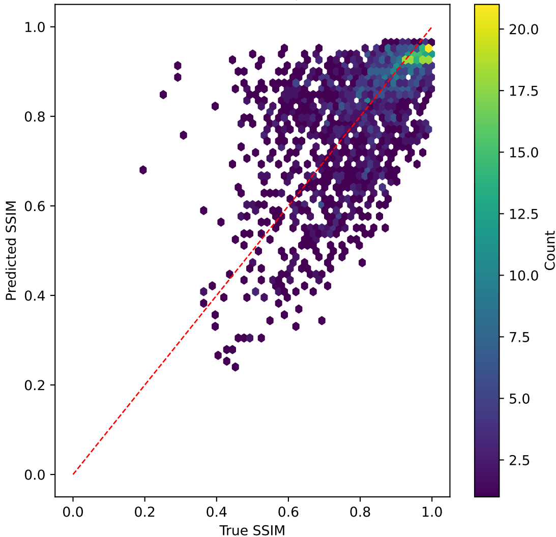
mobilevitv2 on SSIM | R^2=0.349
