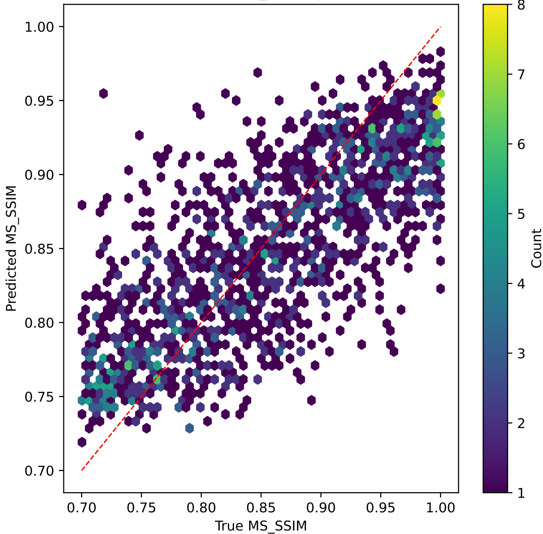
resnet50v2 on MS_SSIM | R^2=0.583
