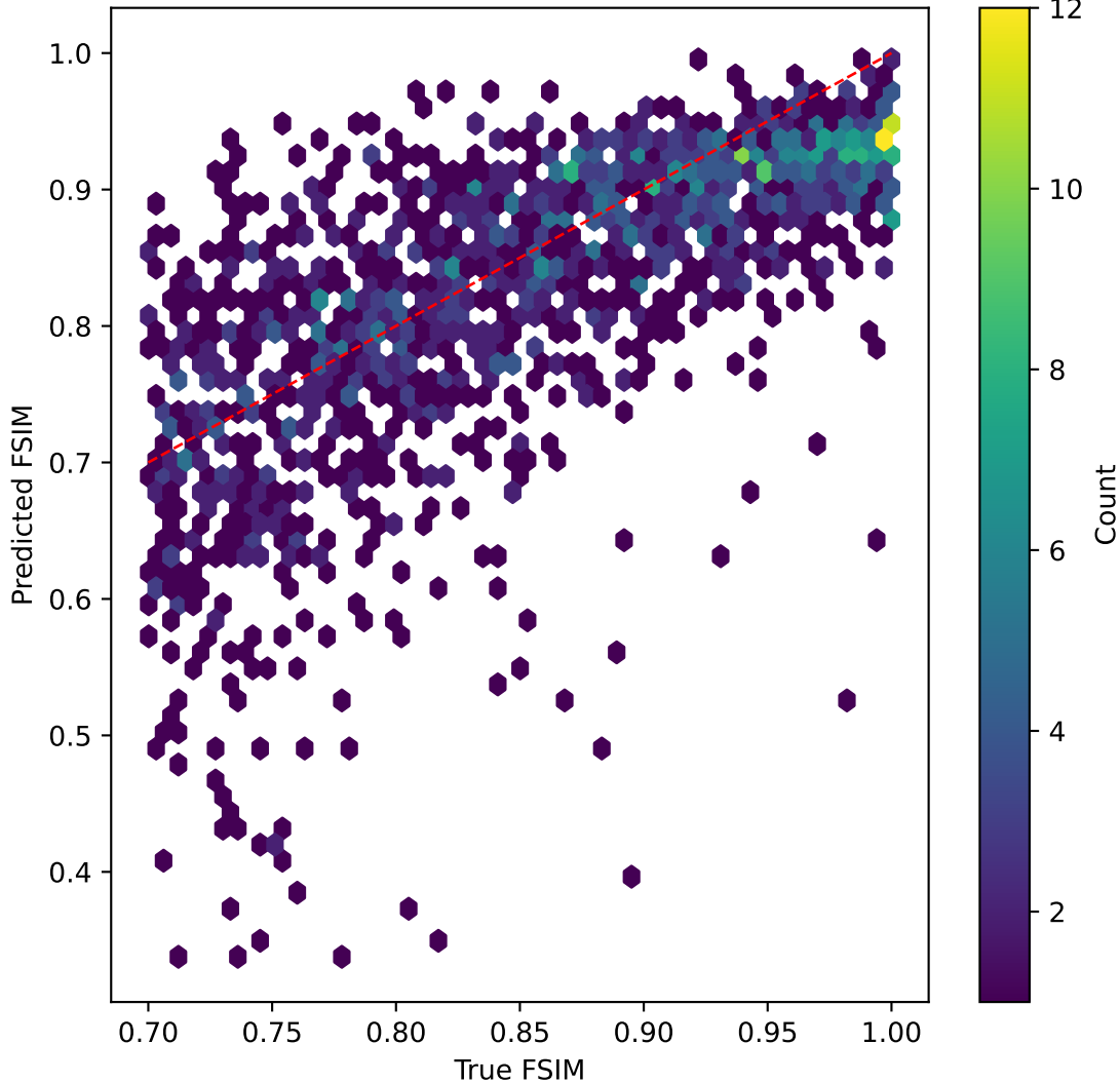
mobilenetv3 on FSIM | R^2=-0.055
