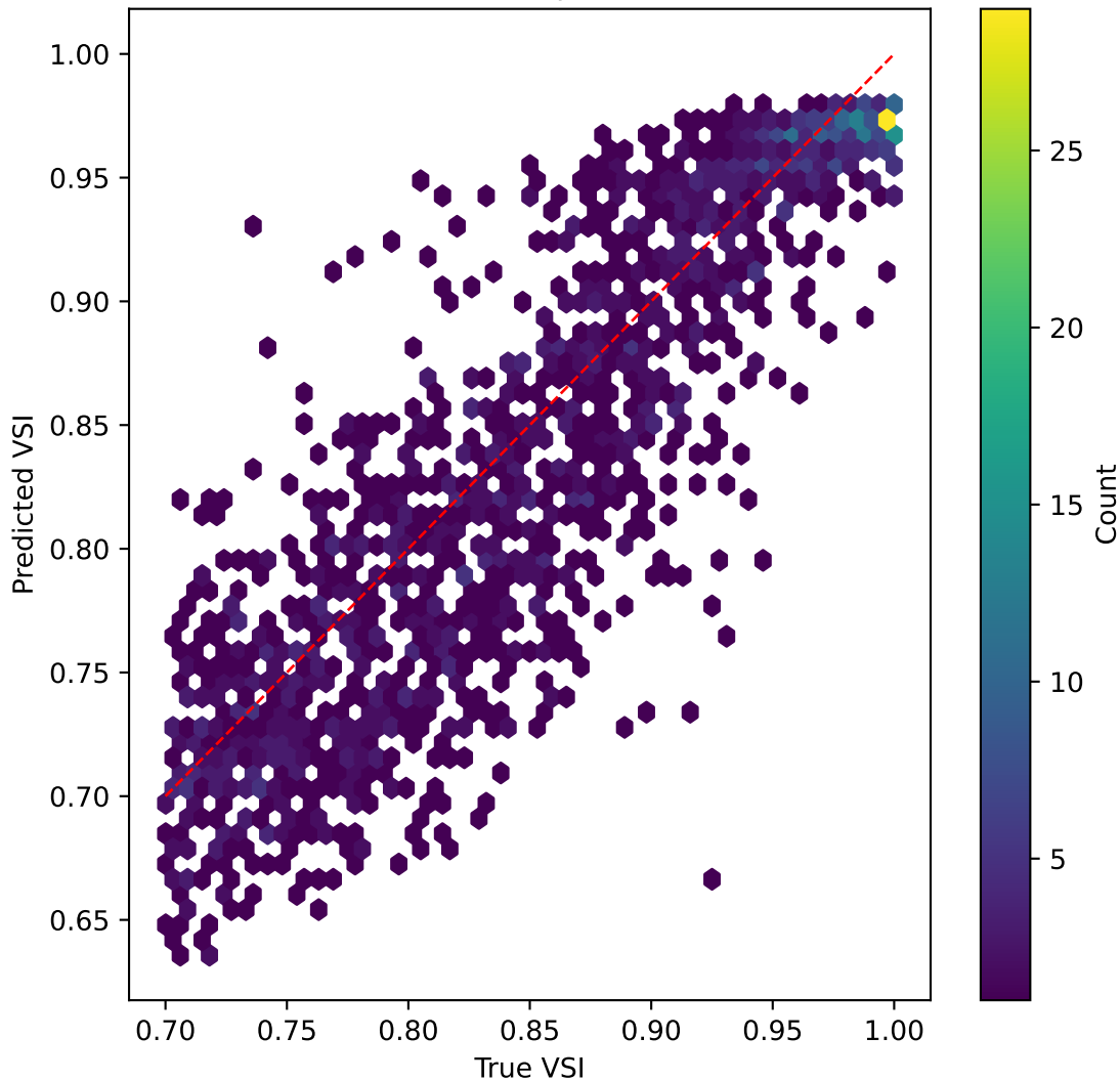
tinyvit on VSI | R^2=0.337
