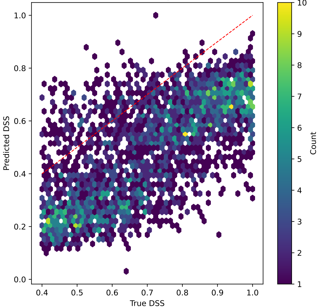
efficientnet on DSS | R^2=-0.811
