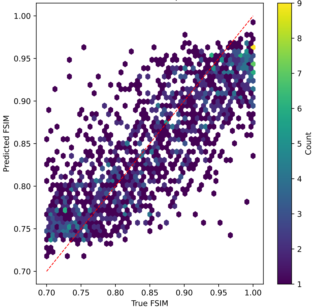
mobilenetv3 on FSIM | R^2=0.624
