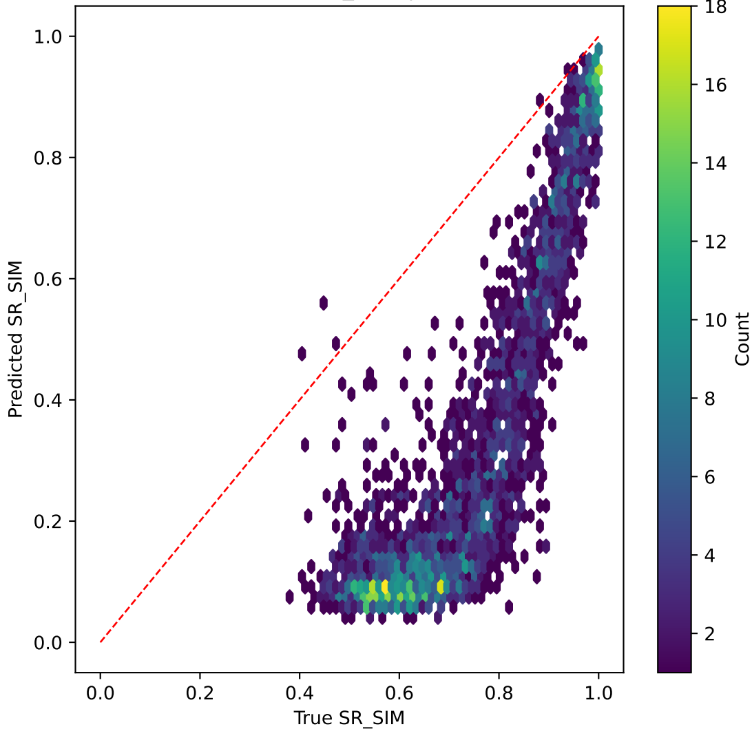
mobilevitv2 on SR_SIM | R^2=-17.350
