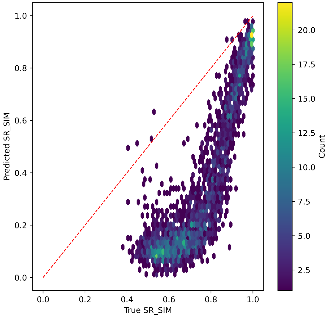
resnet50v2 on SR_SIM | R^2=-16.921
