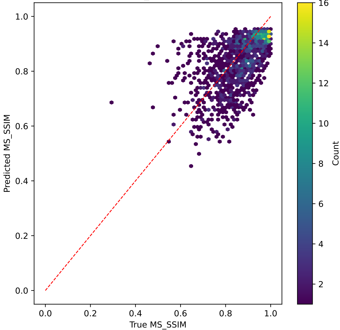
tinyvit on MS_SSIM | R^2=0.051
