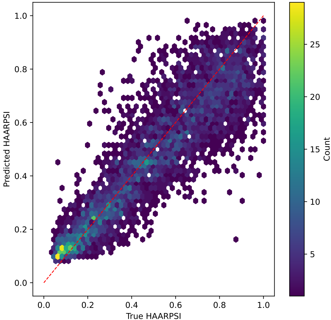
mobilevitv2 on HAARPSI | R^2=0.740
