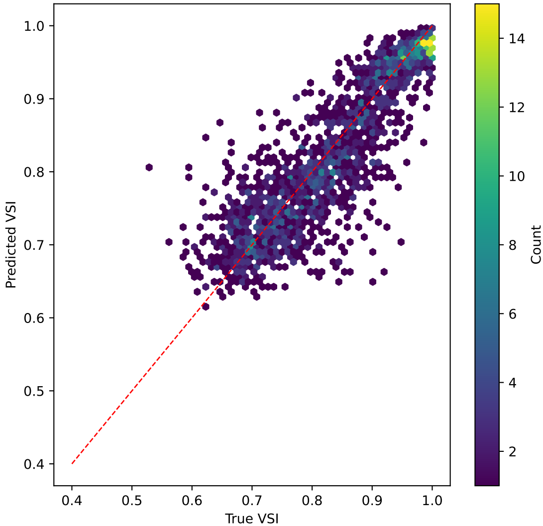
resnet50v2 on VSI | R^2=0.370
