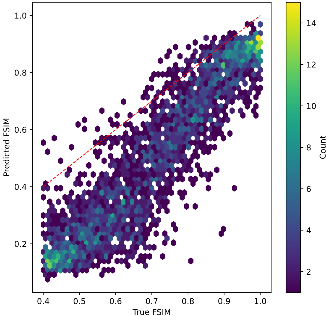
mobilenetv3 on FSIM | R^2=-2.506
