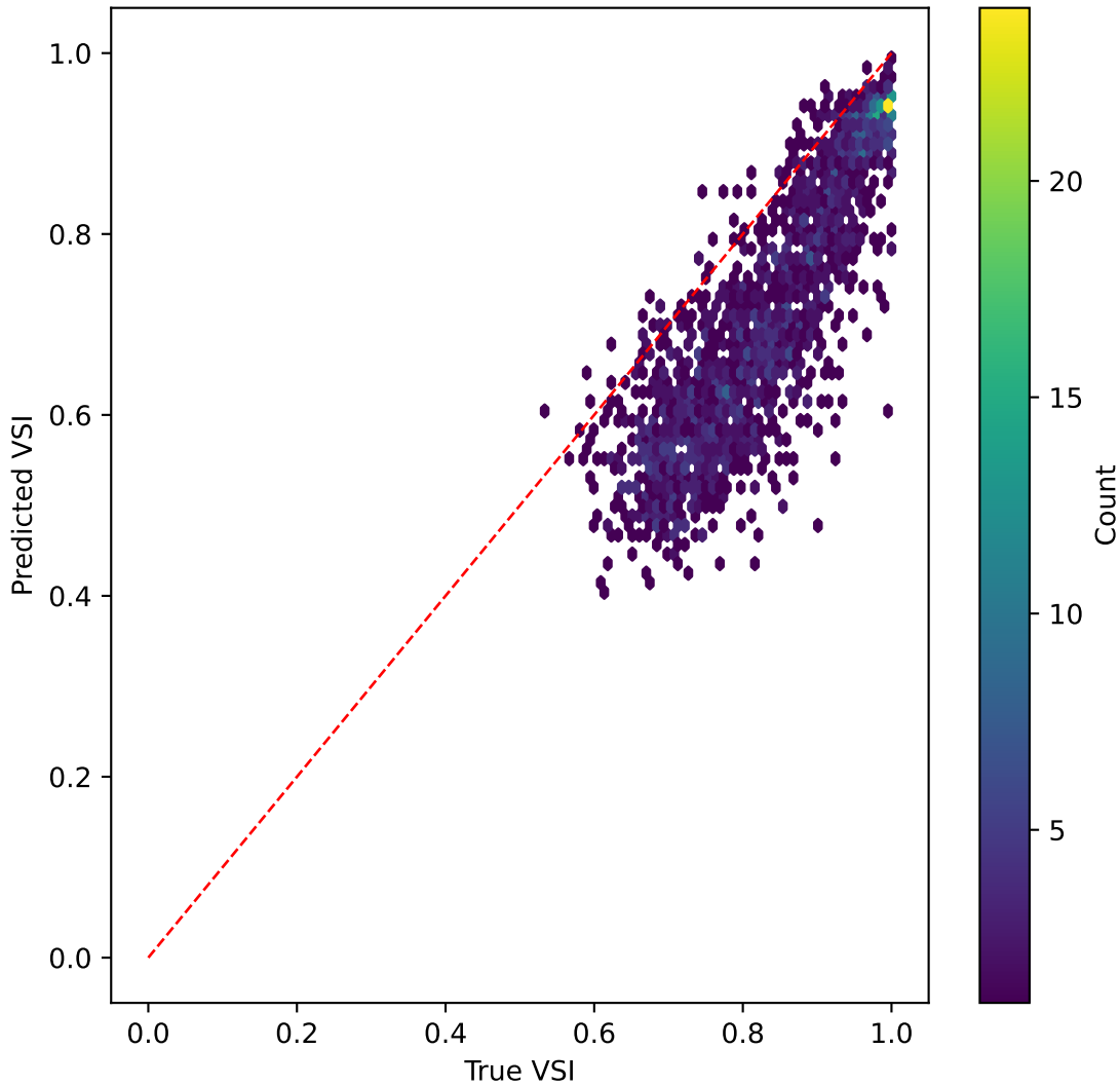
mobilenetv3 on VSI | R^2=-3.630
