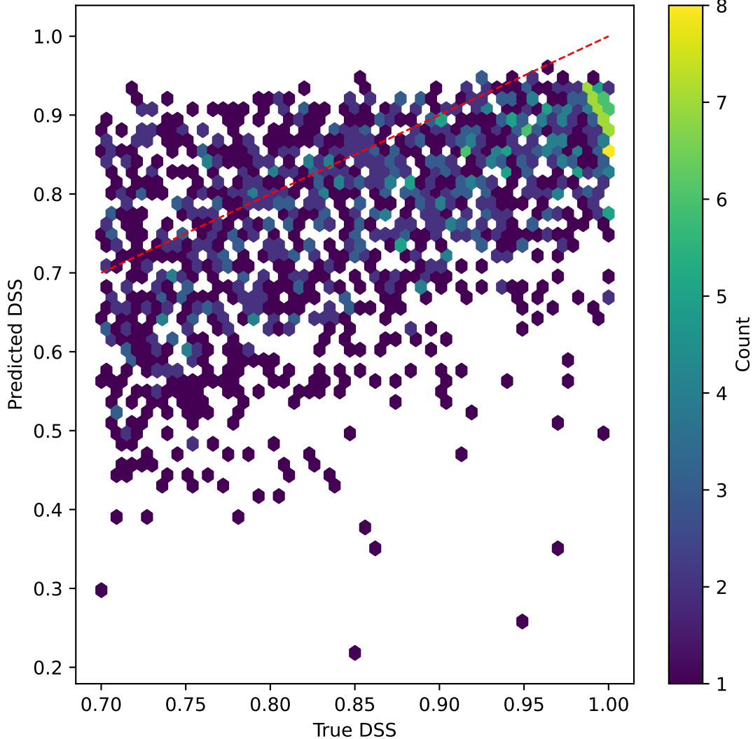
mobilevitv2 on DSS | R^2=-1.247
