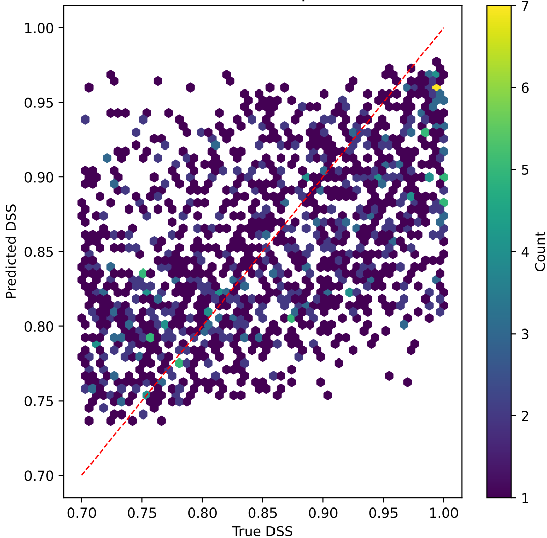
mobilevitv2 on DSS | R^2=0.215
