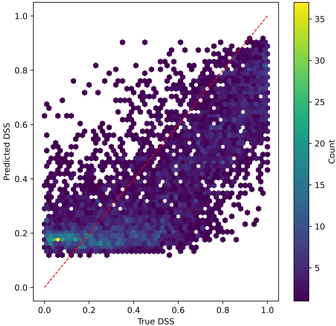
mobilevitv2 on DSS | R^2=0.461
