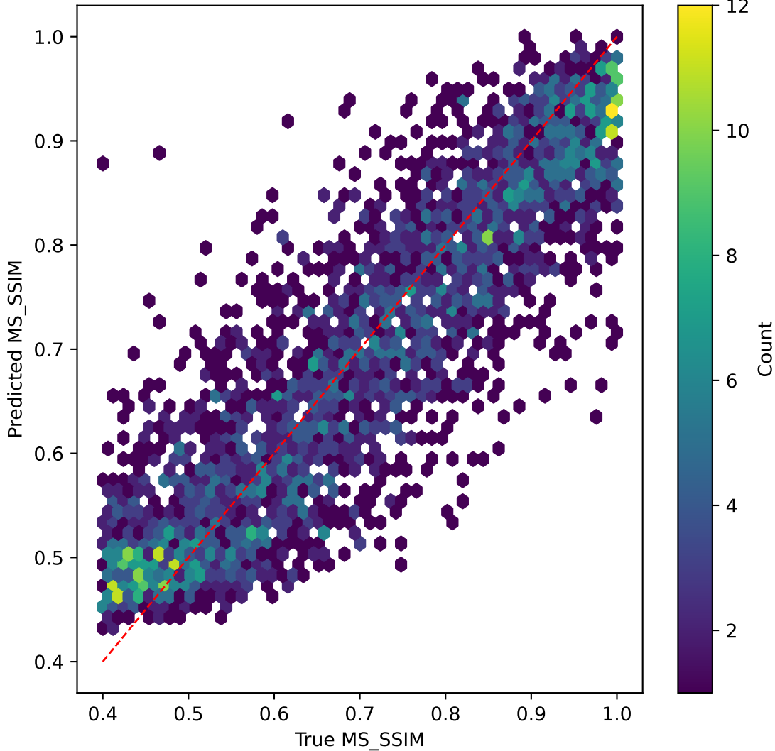
efficientnet on MS_SSIM | R^2=0.757
