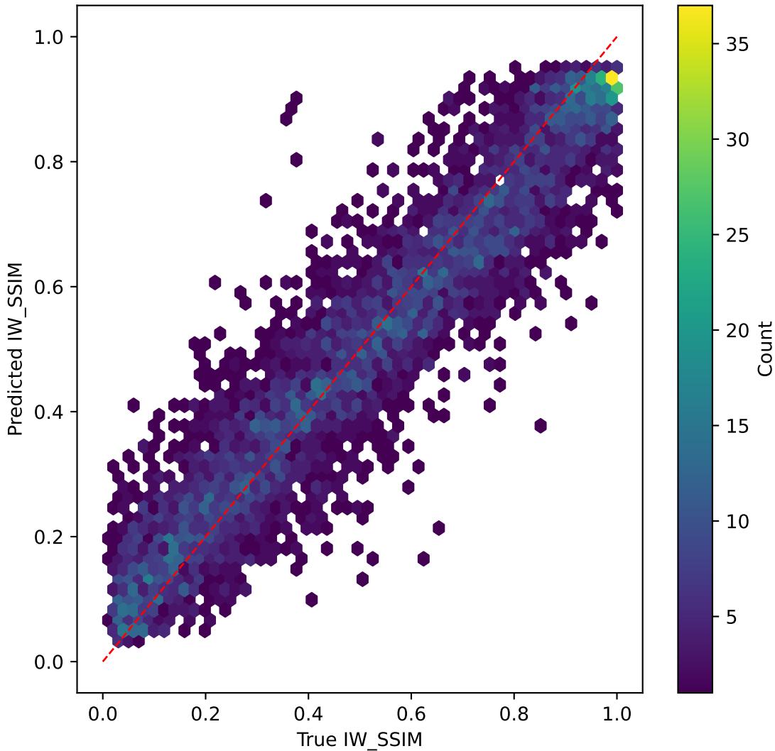
tinyvit on IW_SSIM | R^2=0.870
