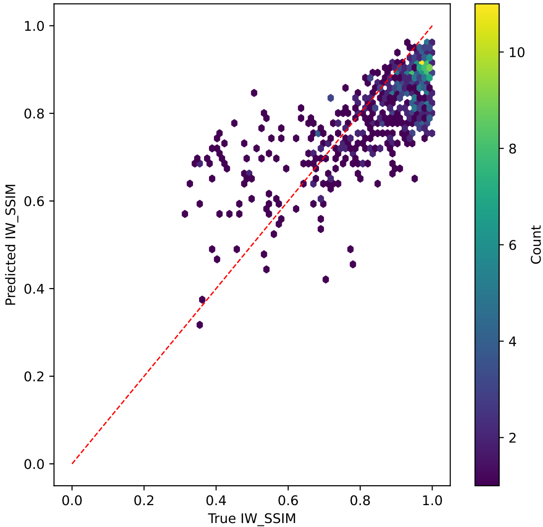
resnet50v2 on IW_SSIM | R^2=0.354
