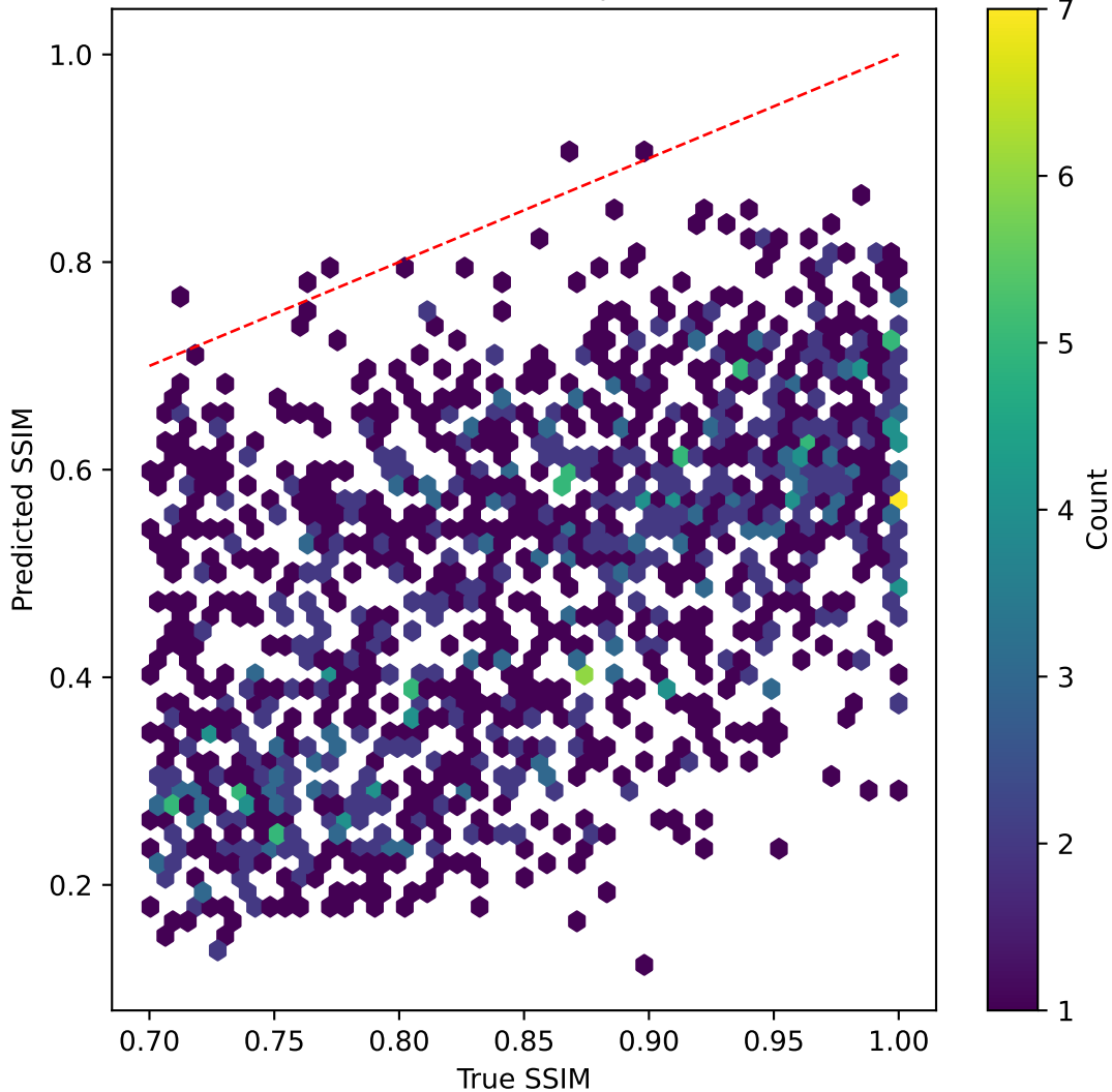
mobilenetv3 on SSIM | R^2=-18.754
