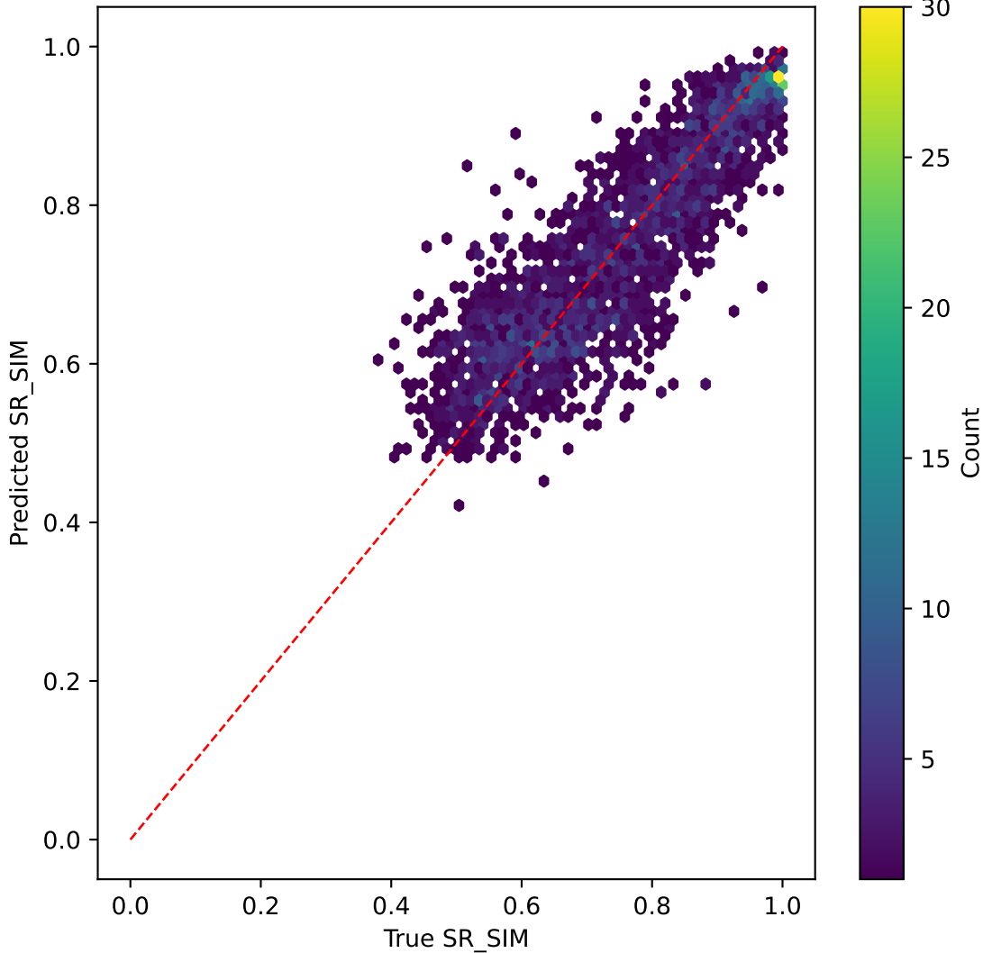
mobilenetv3 on SR_SIM | R^2=0.584
