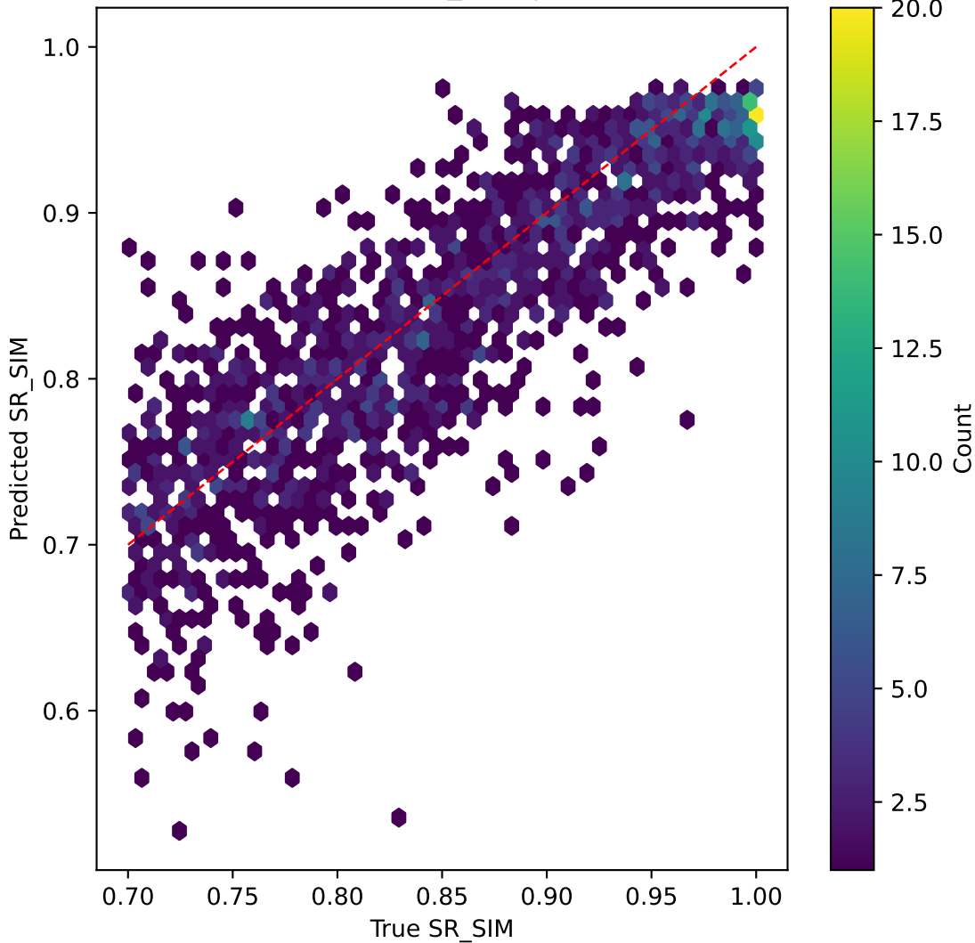
mobilevitv2 on SR_SIM | R^2=0.599
