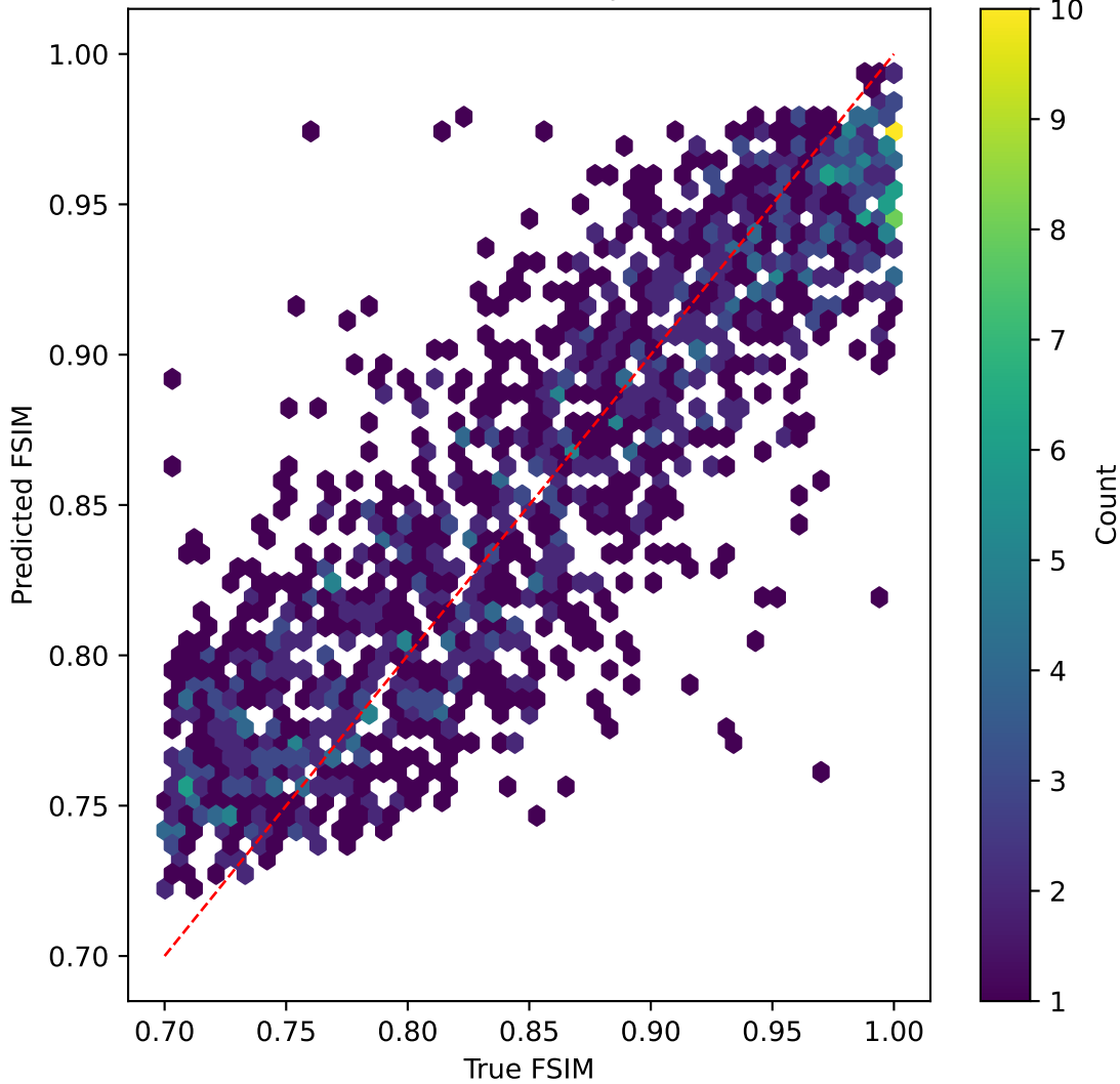
resnet50v2 on FSIM | R^2=0.715
