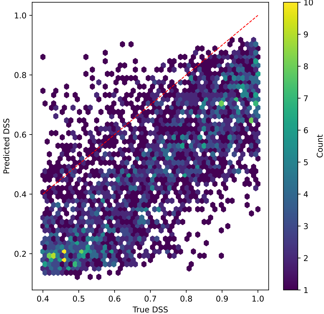
mobilevitv2 on DSS | R^2=-0.858
