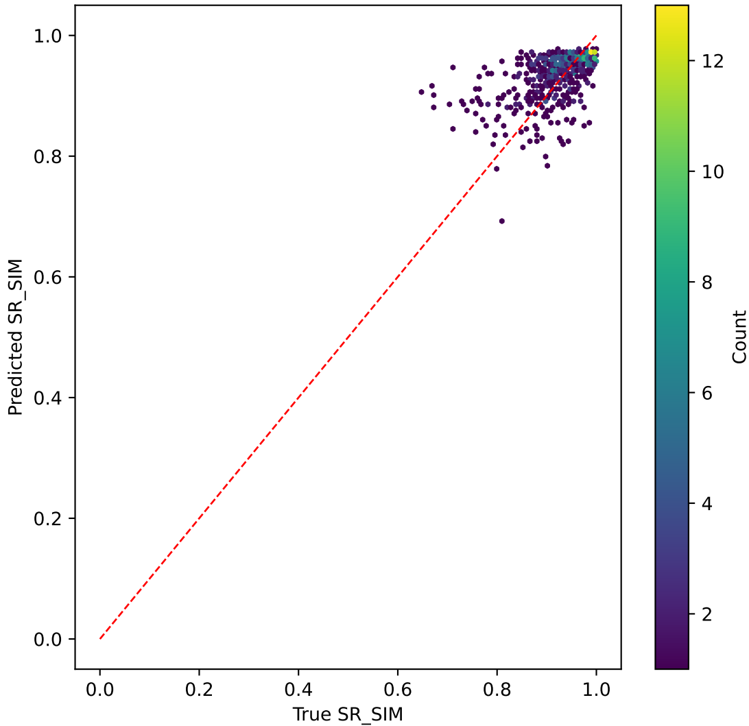
mobilevitv2 on SR_SIM | R^2=0.022
