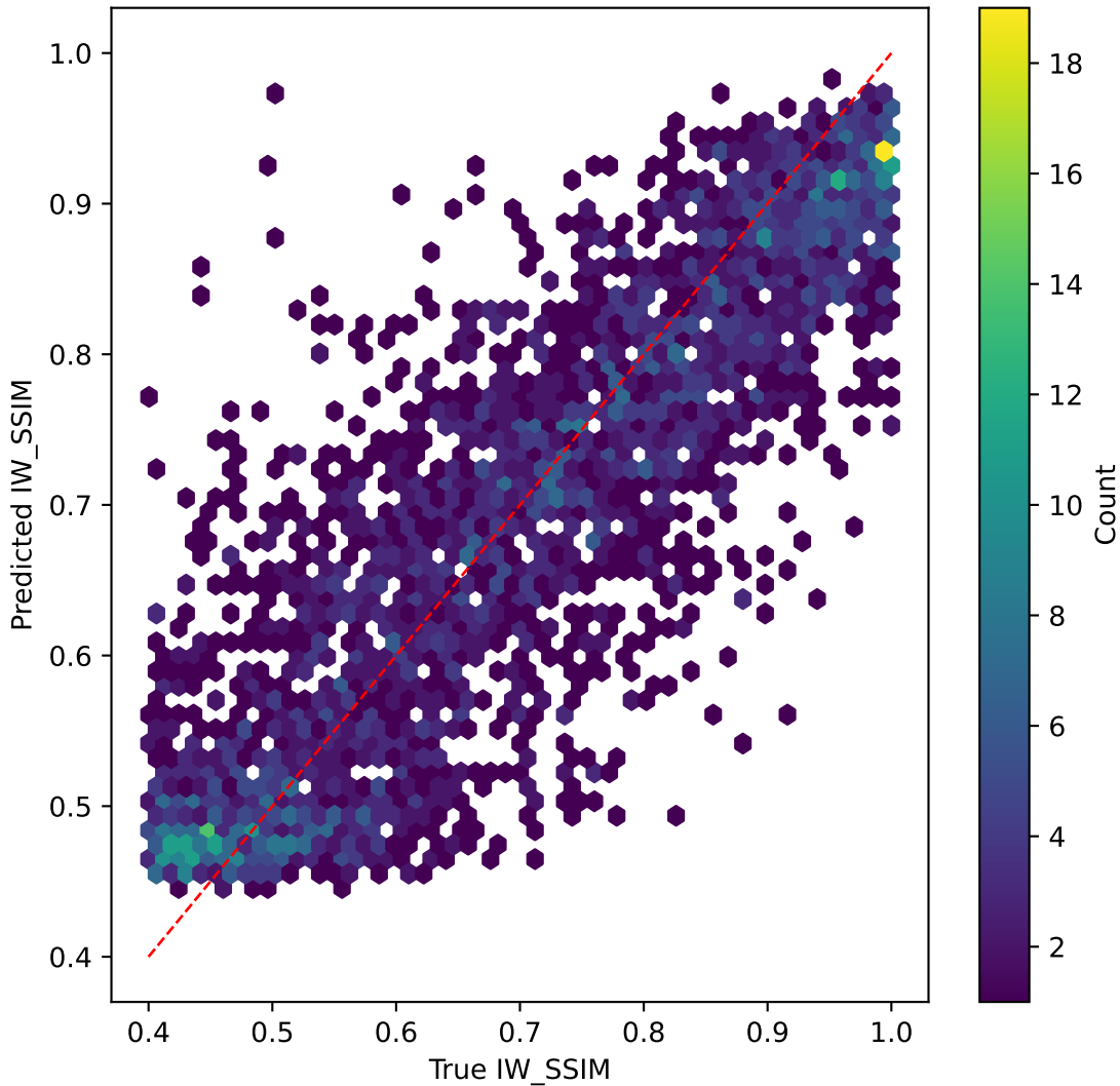
mobilevitv2 on IW_SSIM | R^2=0.758
