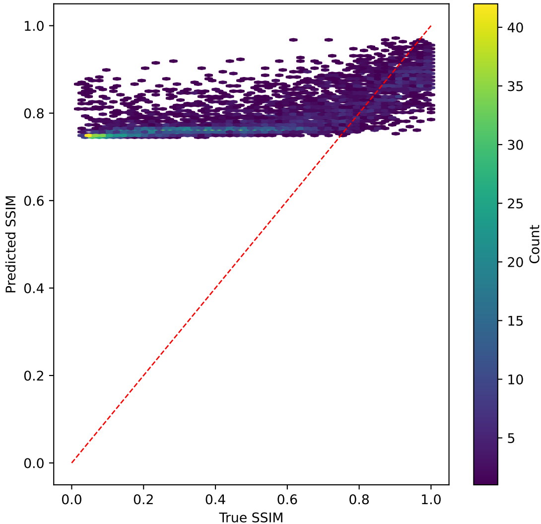
mobilevitv2 on SSIM | R^2=-2.076
