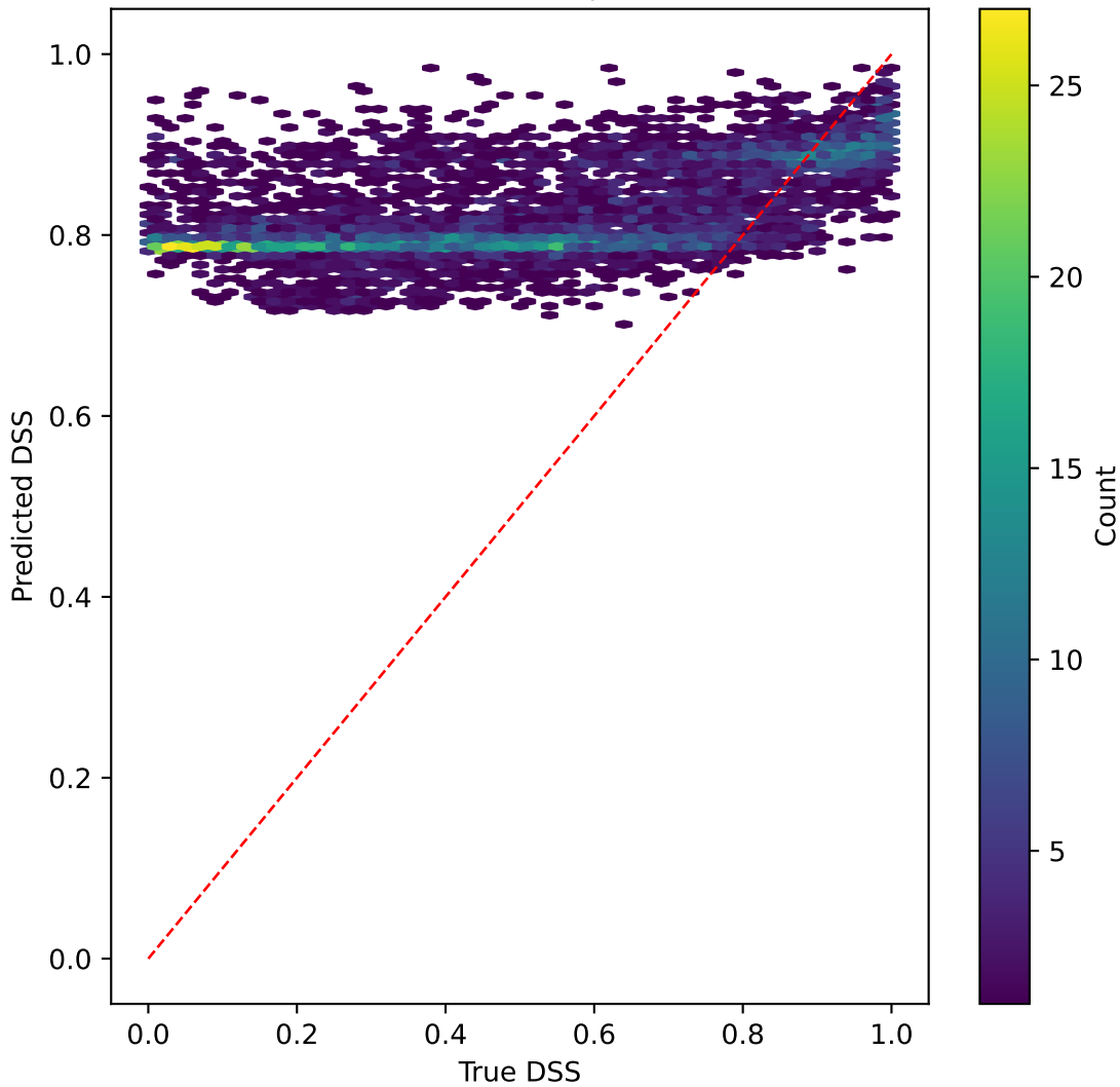
resnet50v2 on DSS | R^2=-4.674
