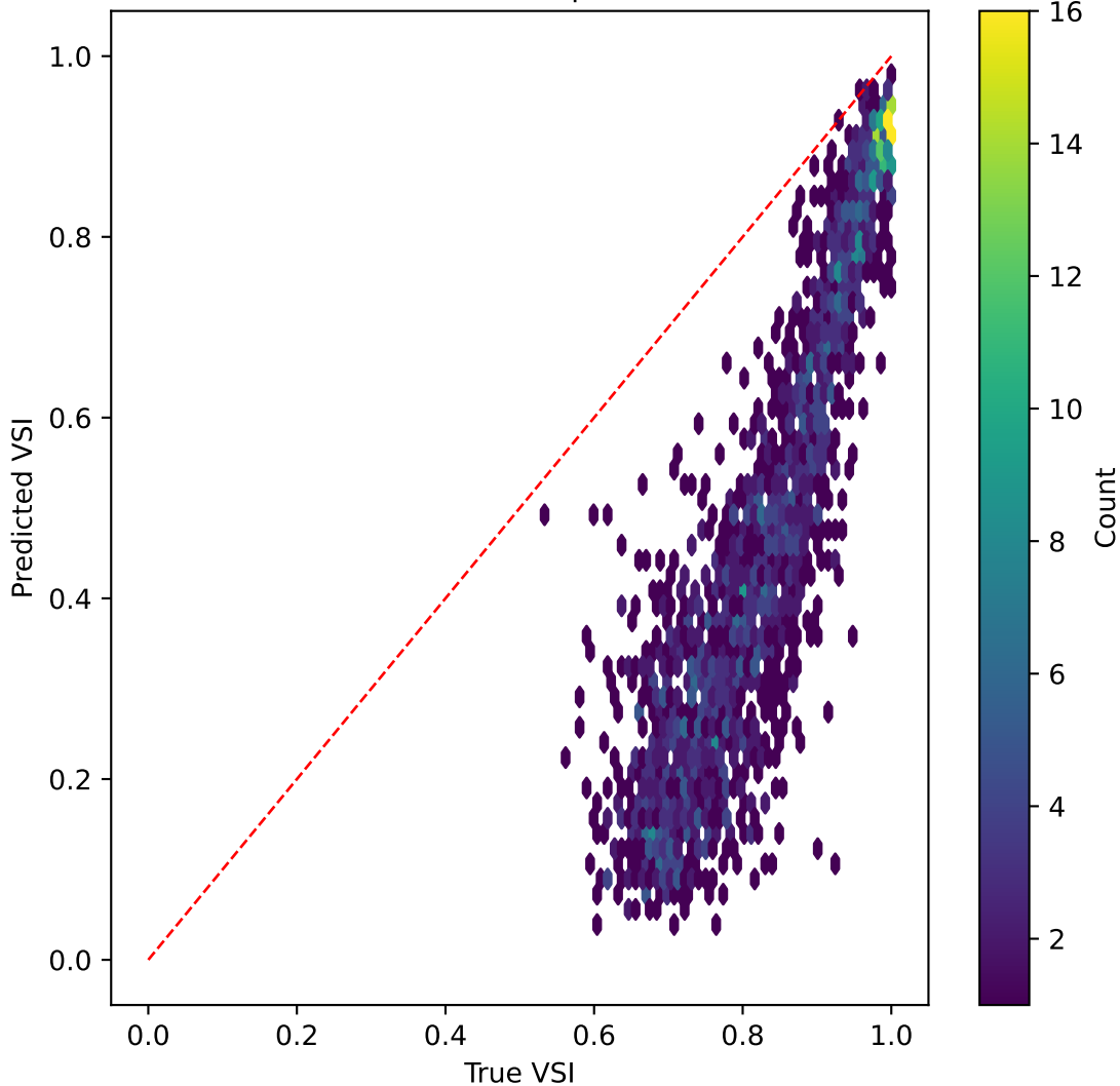
resnet50v2 on VSI | R^2=-28.161
