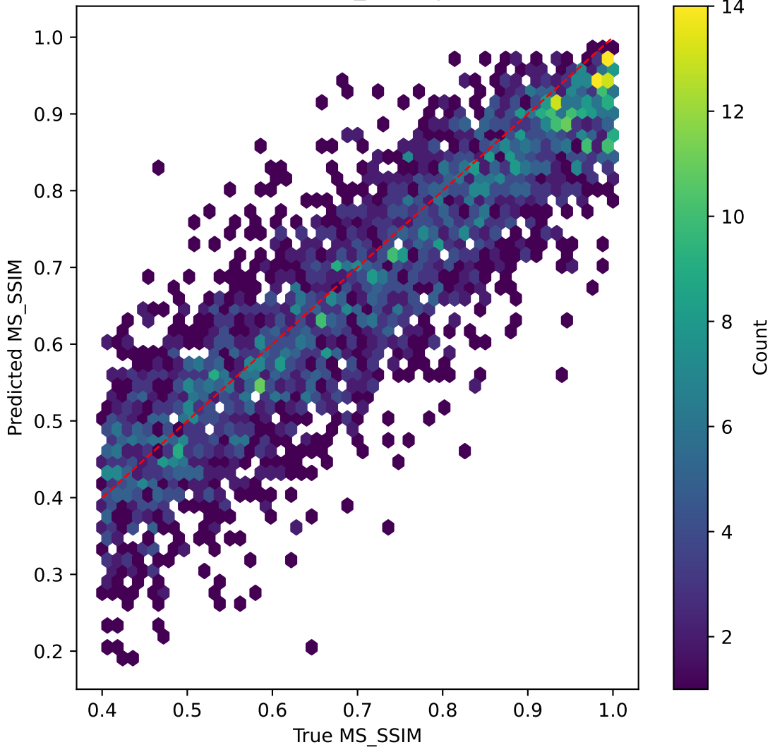
resnet50v2 on MS_SSIM | R^2=0.726
