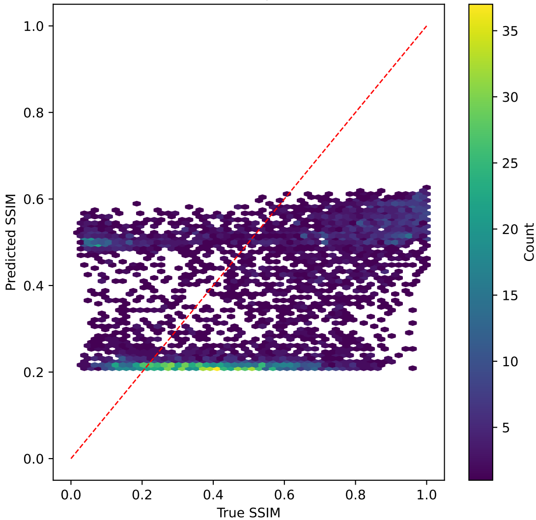
tinyvit on SSIM | R^2=-0.081
