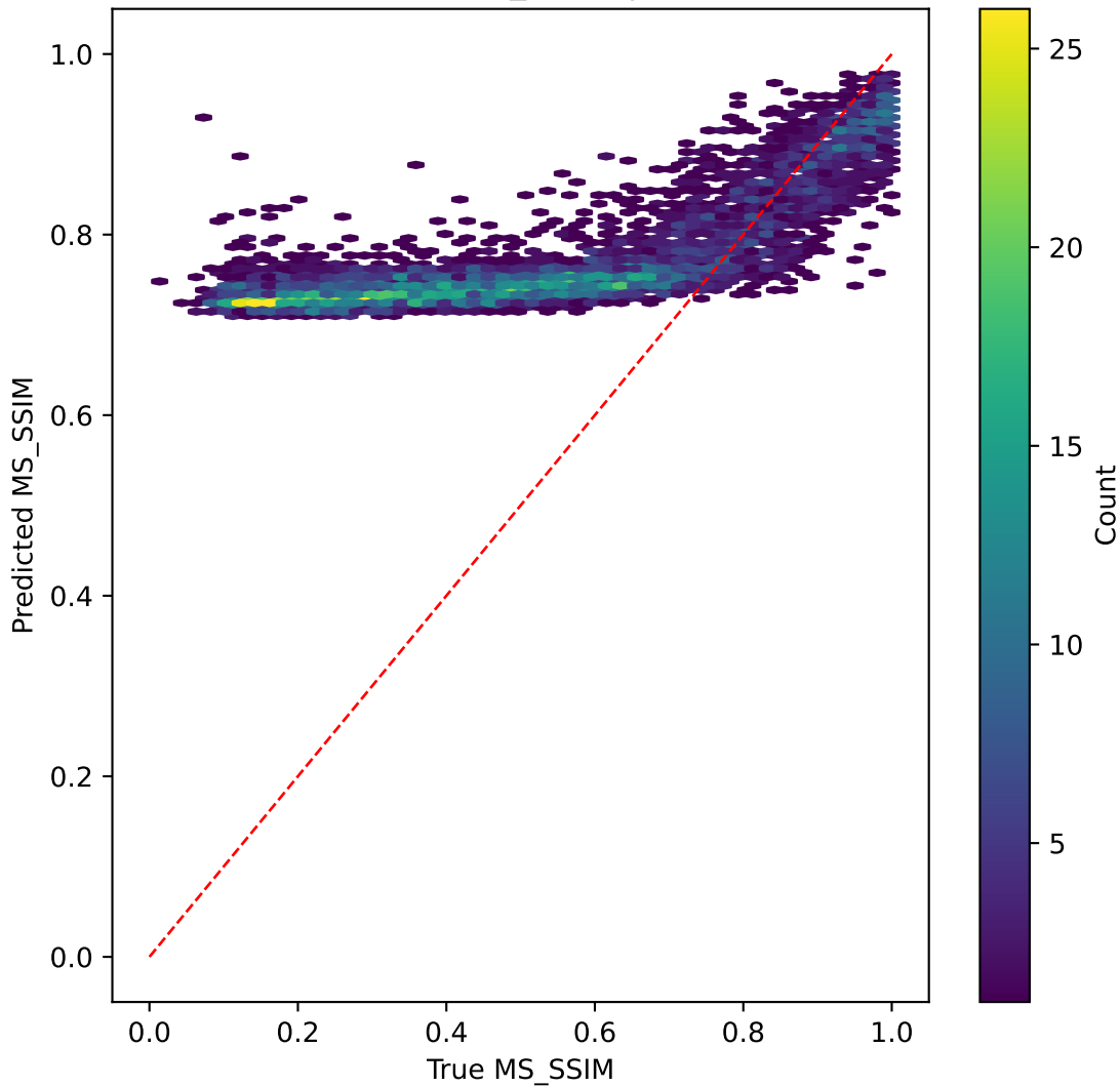
resnet50v2 on MS_SSIM | R^2=-0.847
