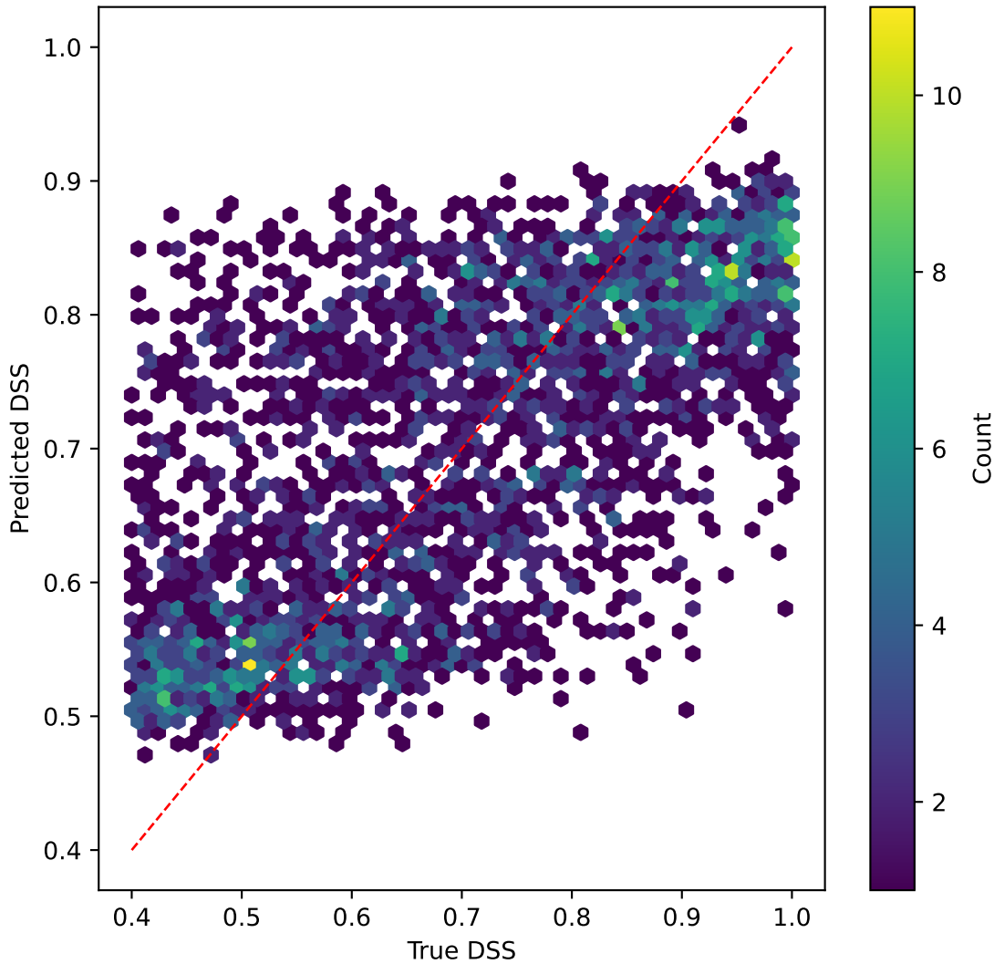
mobilenetv3 on DSS | R^2=0.421
