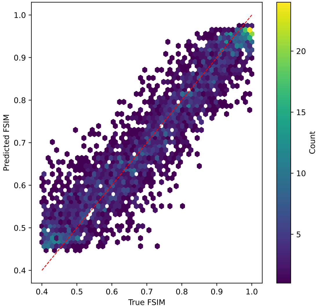
tinyvit on FSIM | R^2=0.785
