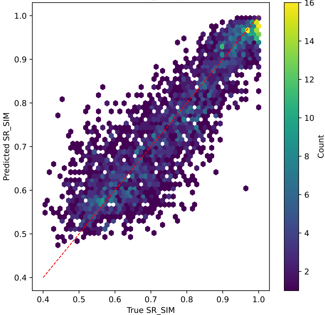
resnet50v2 on SR_SIM | R^2=0.544
