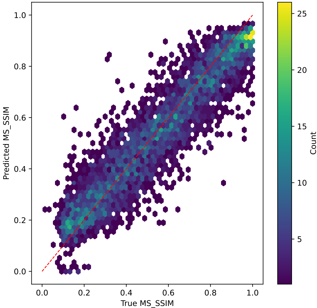
efficientnet on MS_SSIM | R^2=0.802
