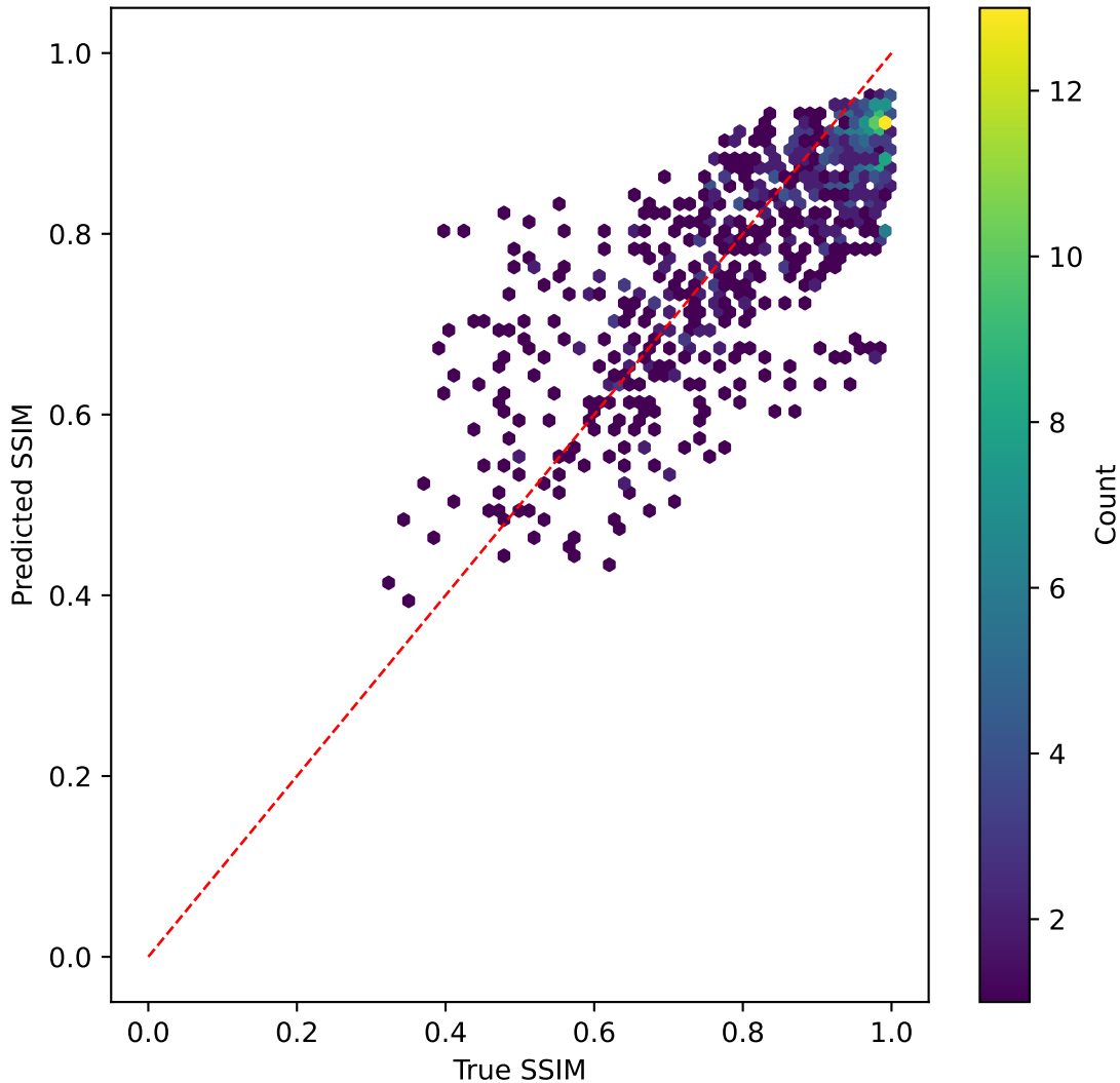
resnet50v2 on SSIM | R^2=0.553
