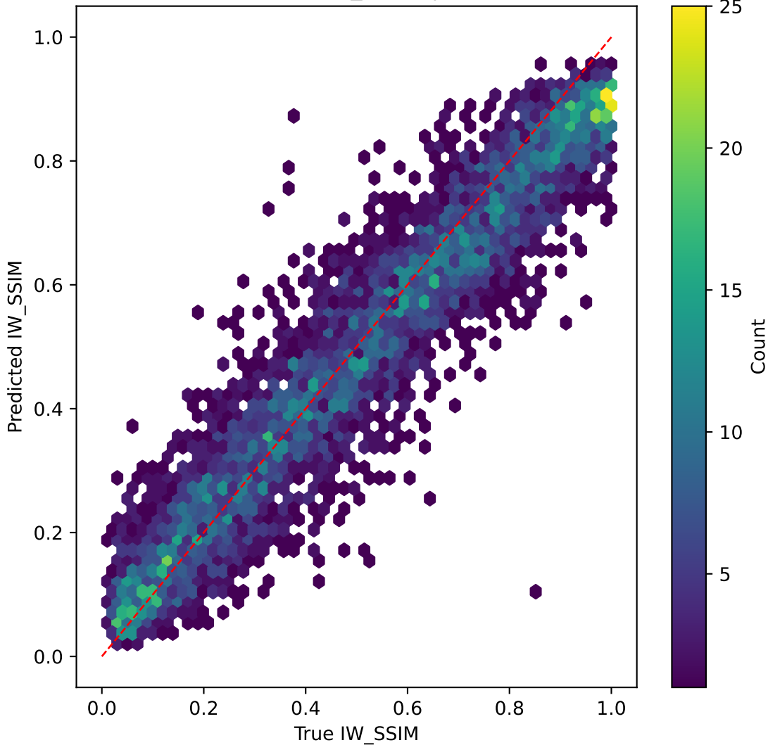
resnet50v2 on IW_SSIM | R^2=0.884
