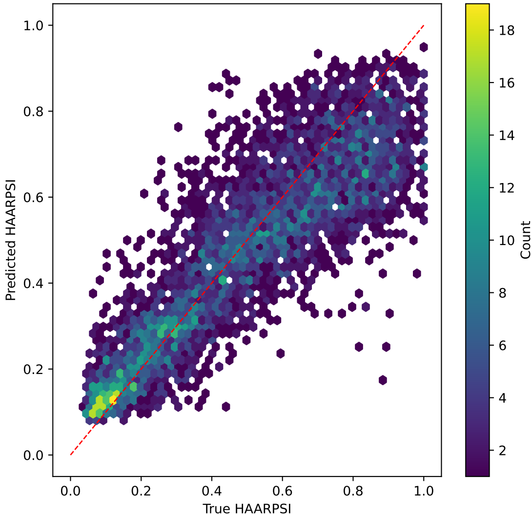
efficientnet on HAARPSI | R^2=0.635
