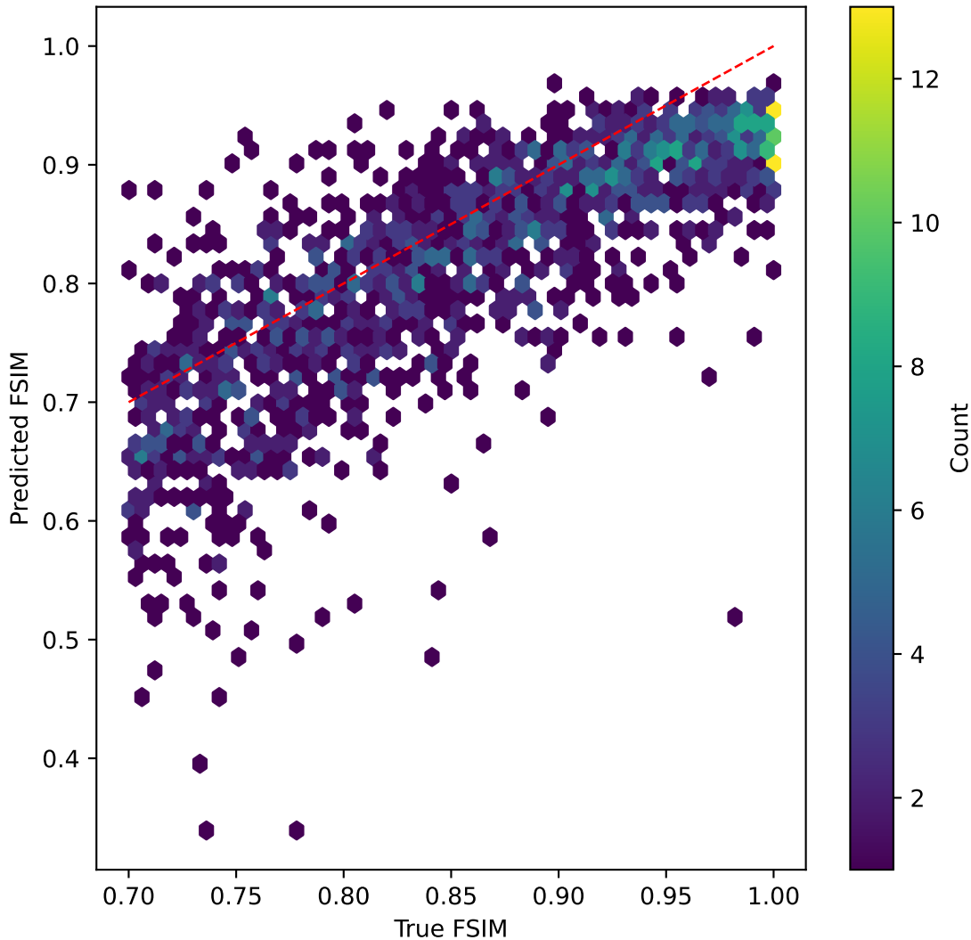
resnet50v2 on FSIM | R^2=0.257
