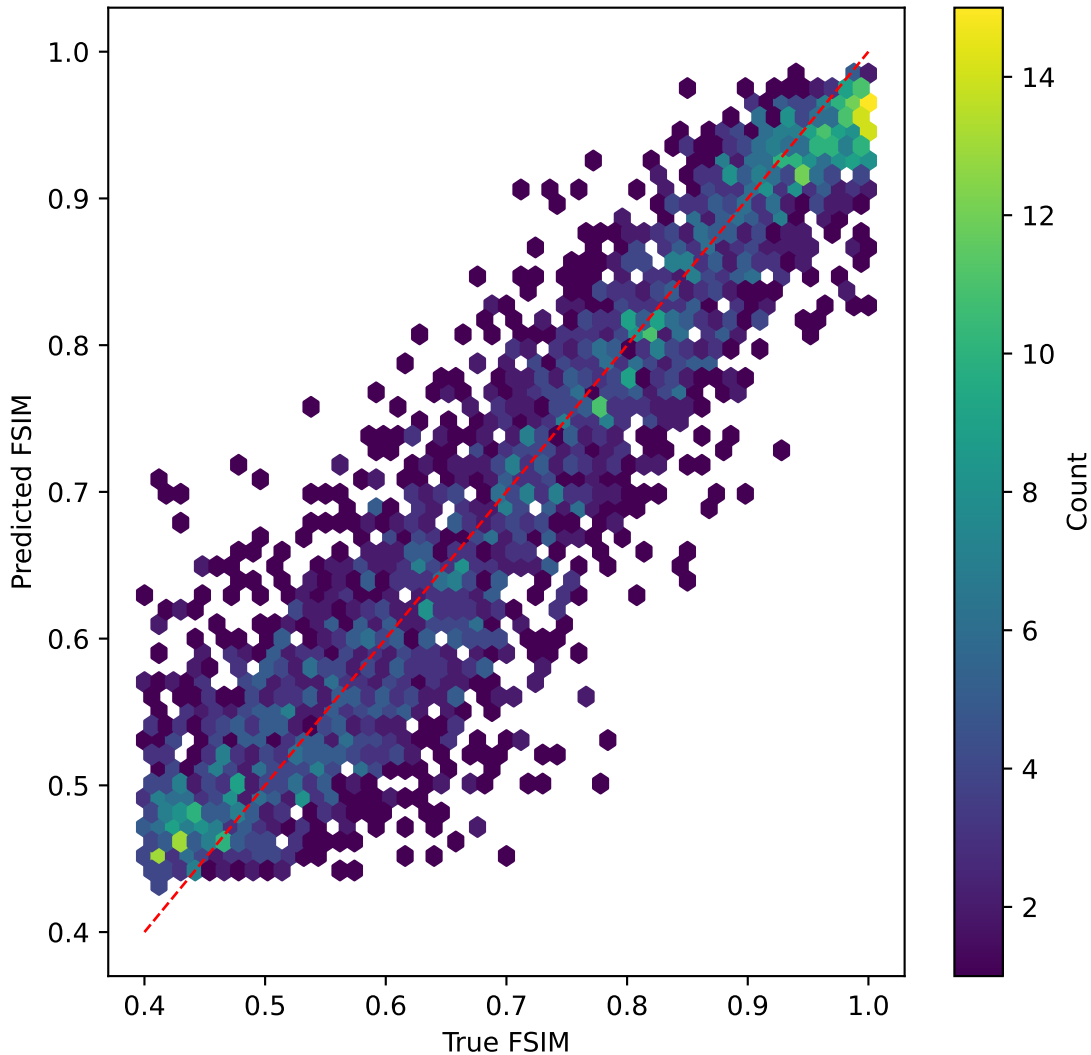
mobilevitv2 on FSIM | R^2=0.779
