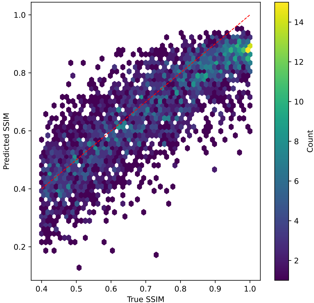
efficientnet on SSIM | R^2=0.558
