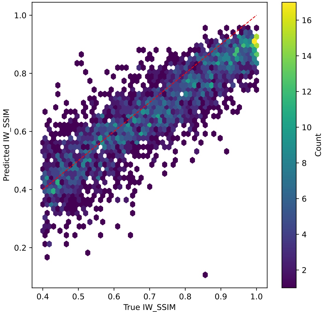
resnet50v2 on IW_SSIM | R^2=0.739
