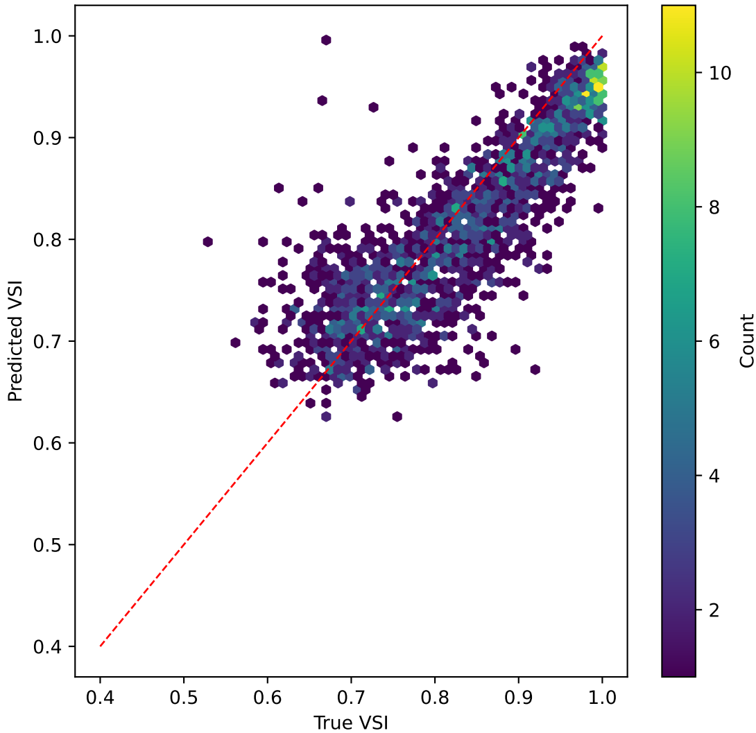
efficientnet on VSI | R^2=0.340
