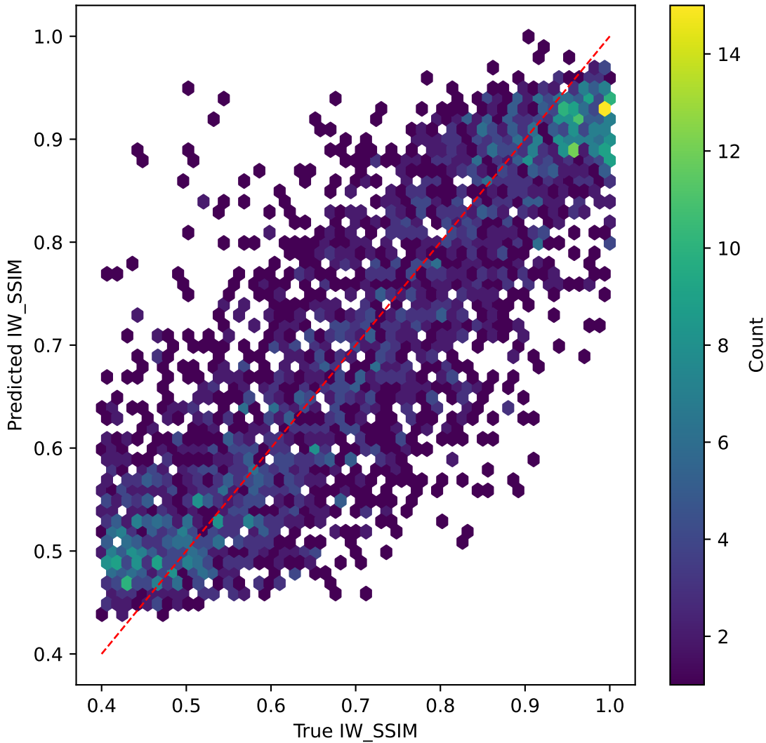
efficientnet on IW_SSIM | R^2=0.731
