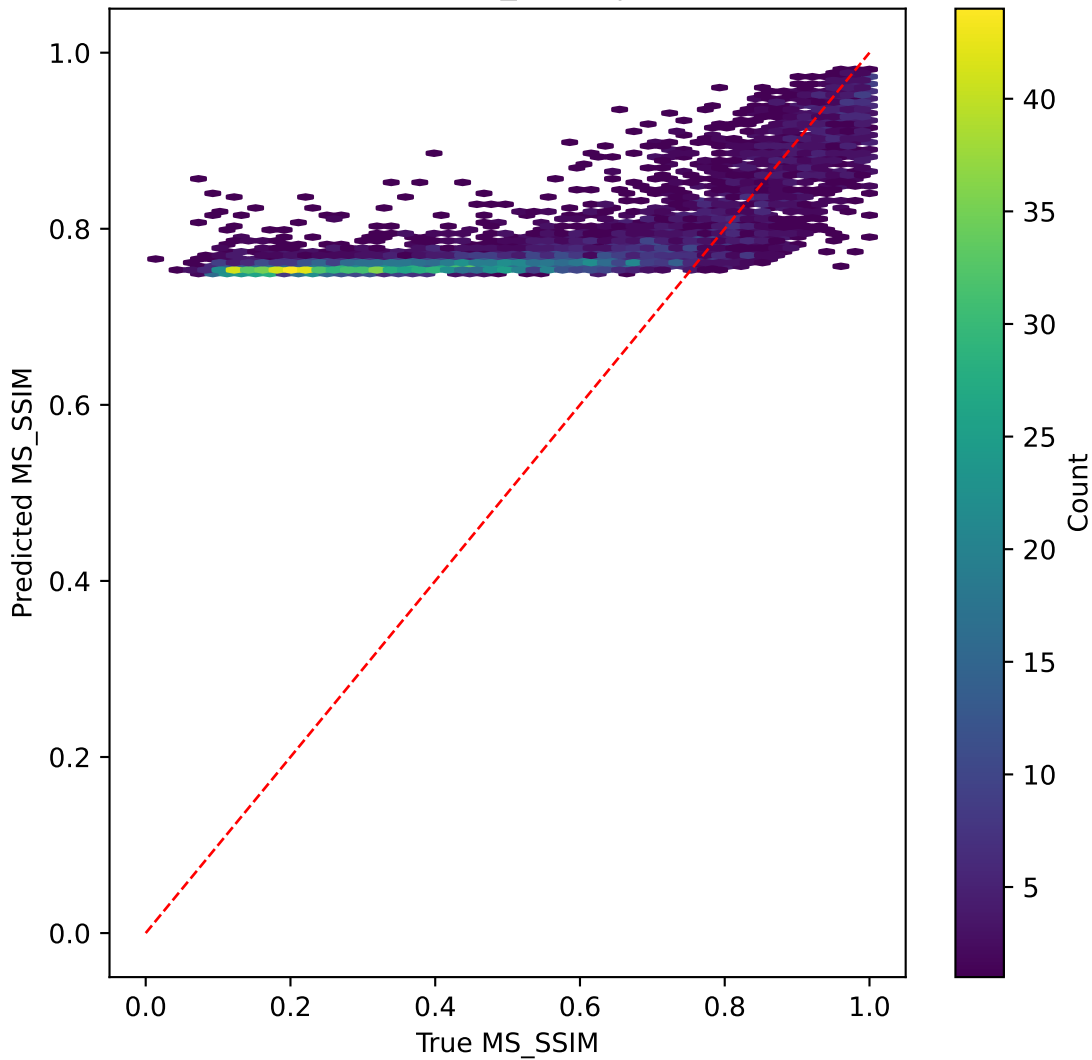
mobilevitv2 on MS_SSIM | R^2=-1.061
