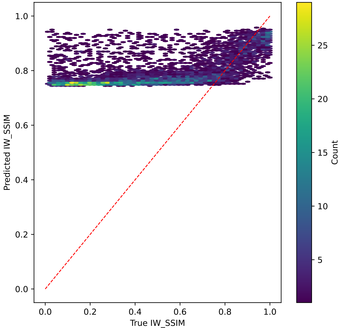
mobilevitv2 on IW_SSIM | R^2=-1.890
