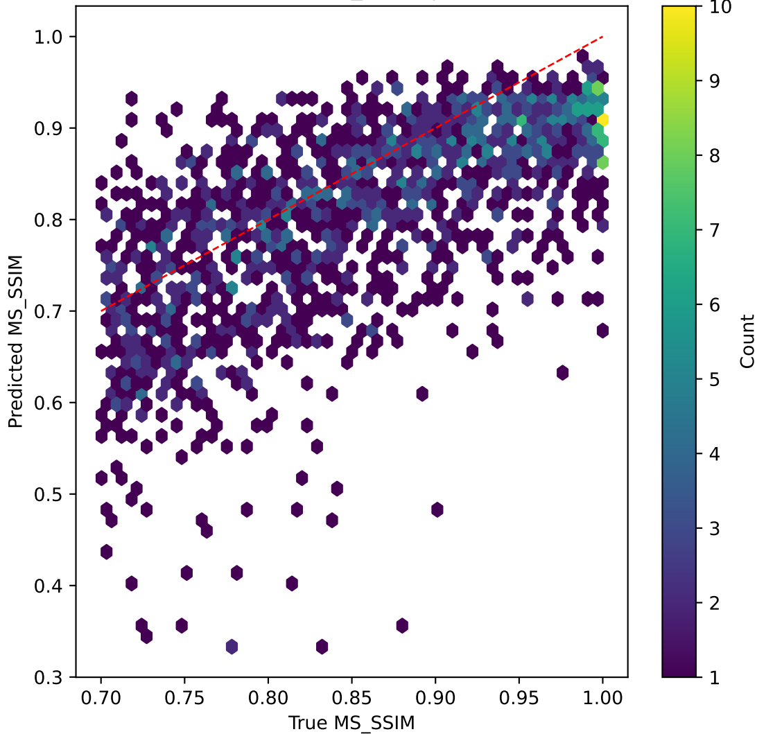
mobilenetv3 on MS_SSIM | R^2=-0.238
