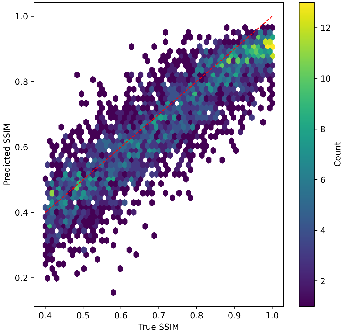
resnet50v2 on SSIM | R^2=0.676
