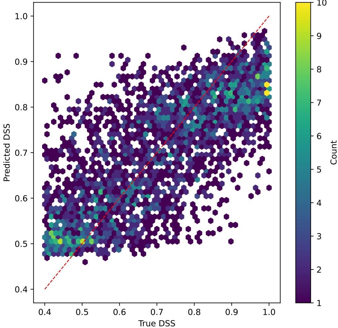
resnet50v2 on DSS | R^2=0.538
