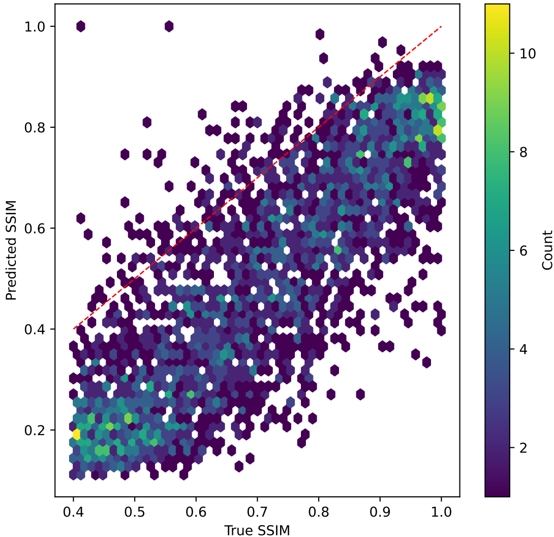
efficientnet on SSIM | R^2=-1.182
