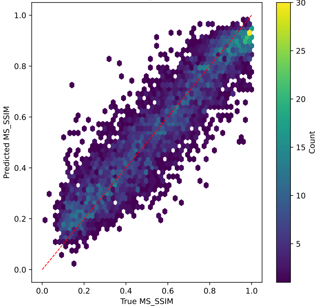
mobilenetv3 on MS_SSIM | R^2=0.777
