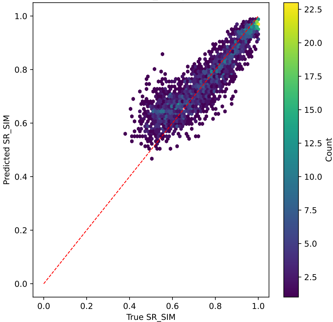
mobilevitv2 on SR_SIM | R^2=0.745
