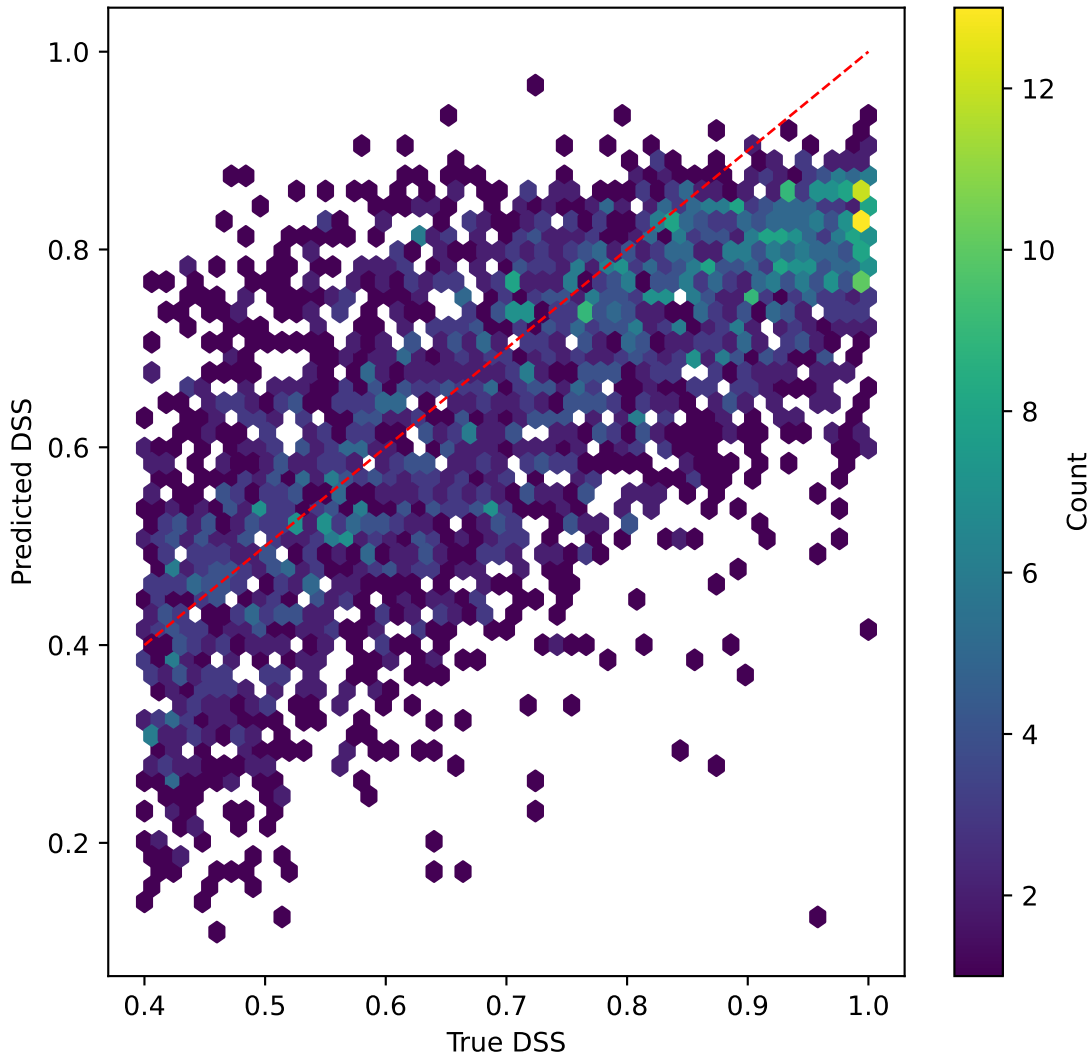
efficientnet on DSS | R^2=0.365
