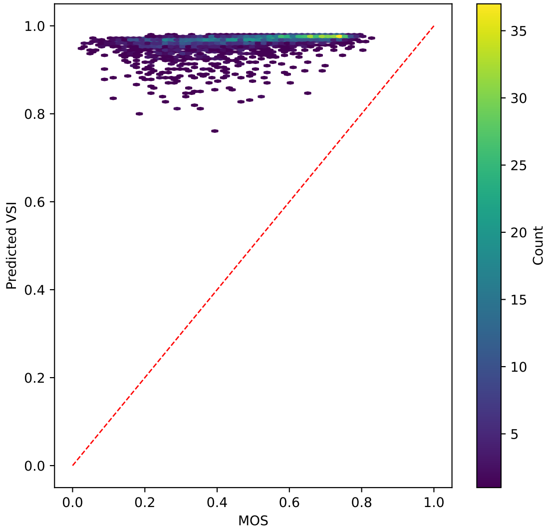
tinyvit on VSI AGAINST MOS | R^2=-9.395
