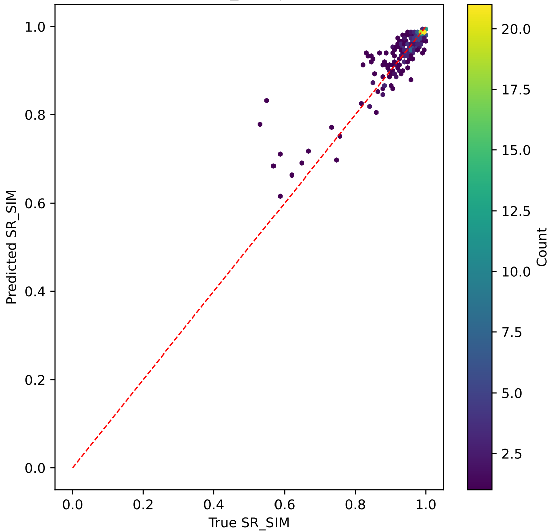
tinyvit on SR_SIM | R^2=0.814
