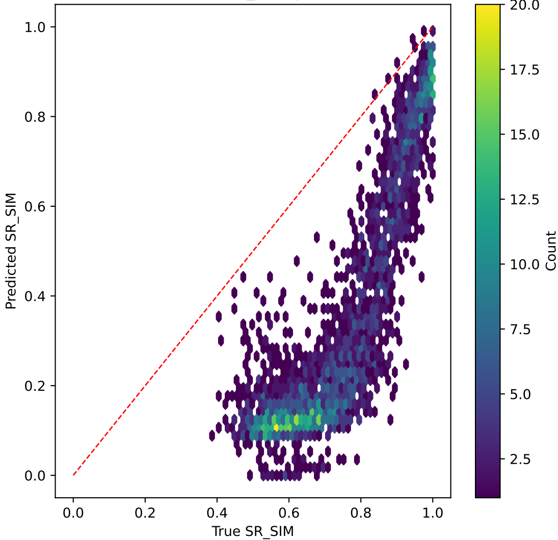
efficientnet on SR_SIM | R^2=-17.055
