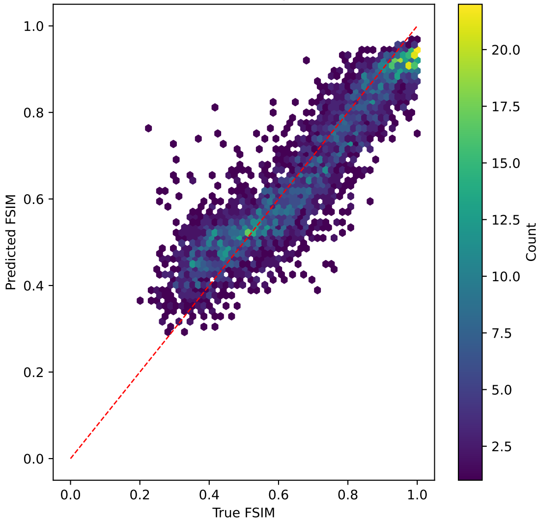
resnet50v2 on FSIM | R^2=0.732
