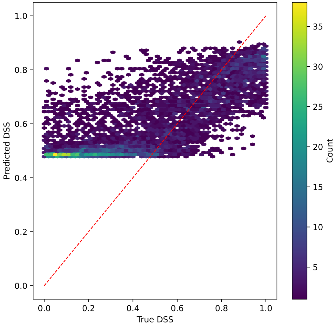
tinyvit on DSS | R^2=-0.946
