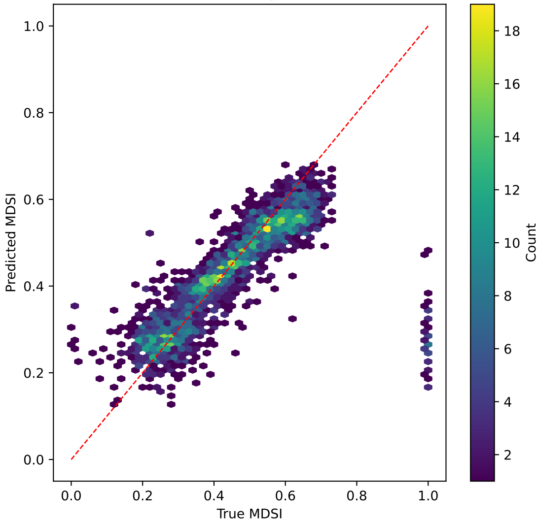
tinyvit on MDSI | R^2=0.300
