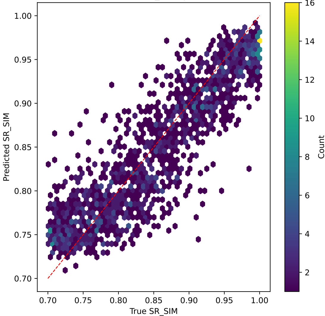
efficientnet on SR_SIM | R^2=0.774
