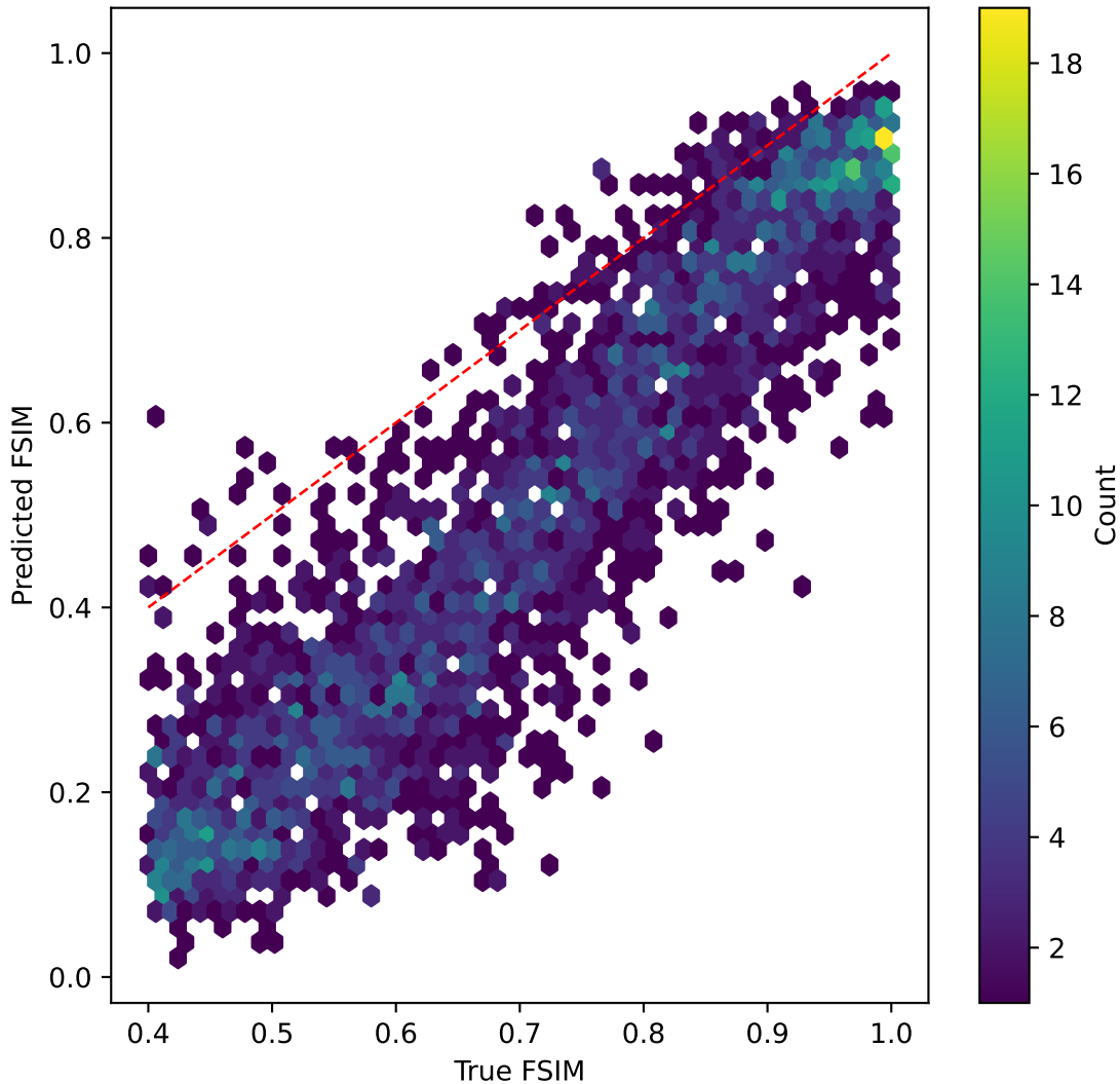
efficientnet on FSIM | R^2=-2.518
