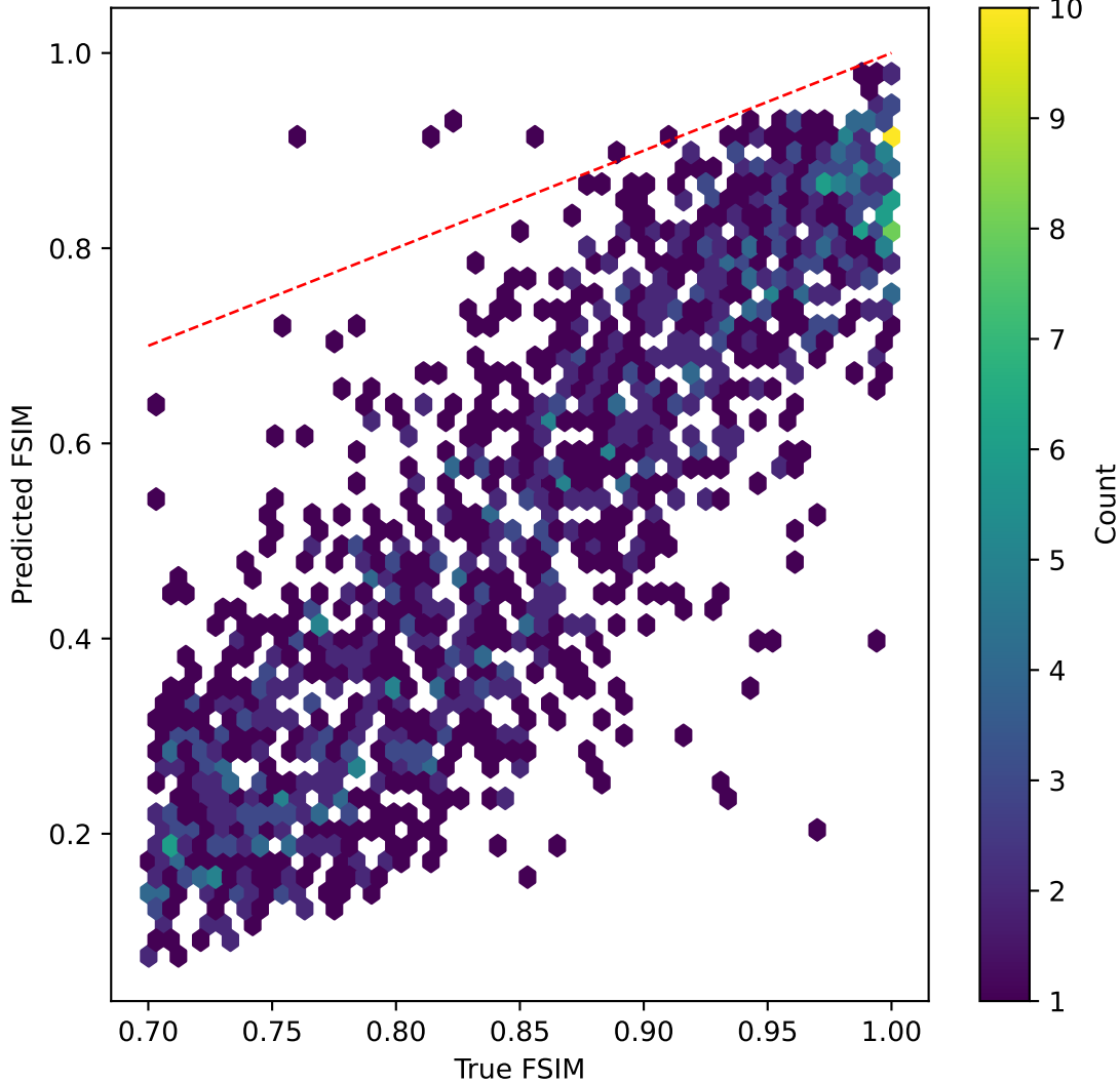
resnet50v2 on FSIM | R^2=-21.009
