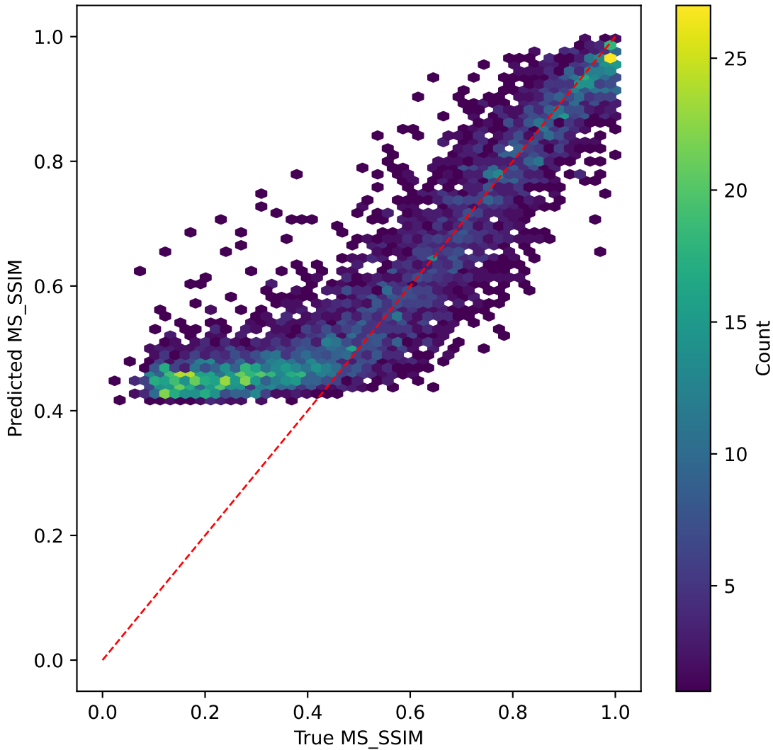
mobilevitv2 on MS_SSIM | R^2=0.660
