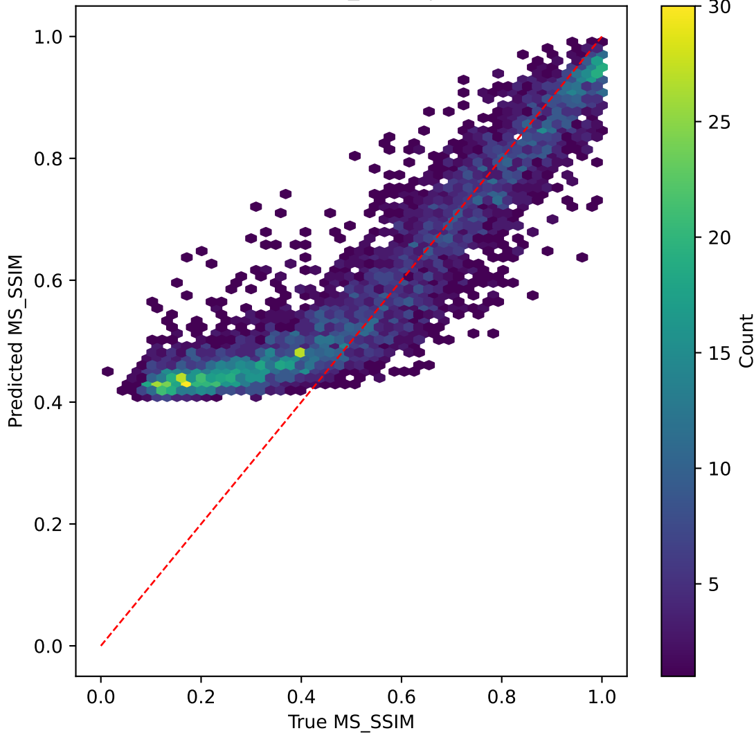
resnet50v2 on MS_SSIM | R^2=0.685
