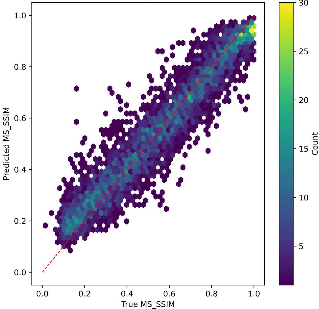
mobilevitv2 on MS_SSIM | R^2=0.863
