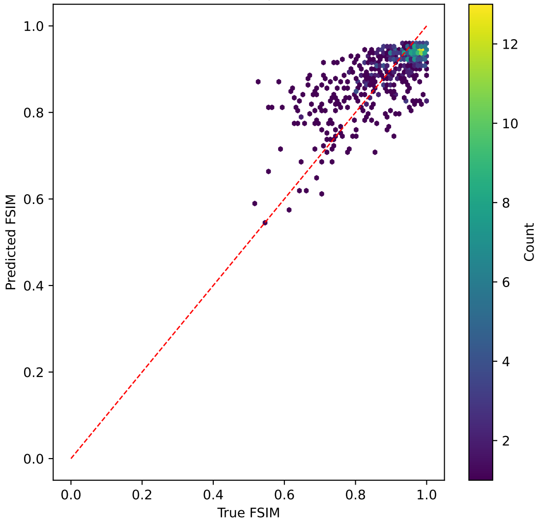
tinyvit on FSIM | R^2=0.496
