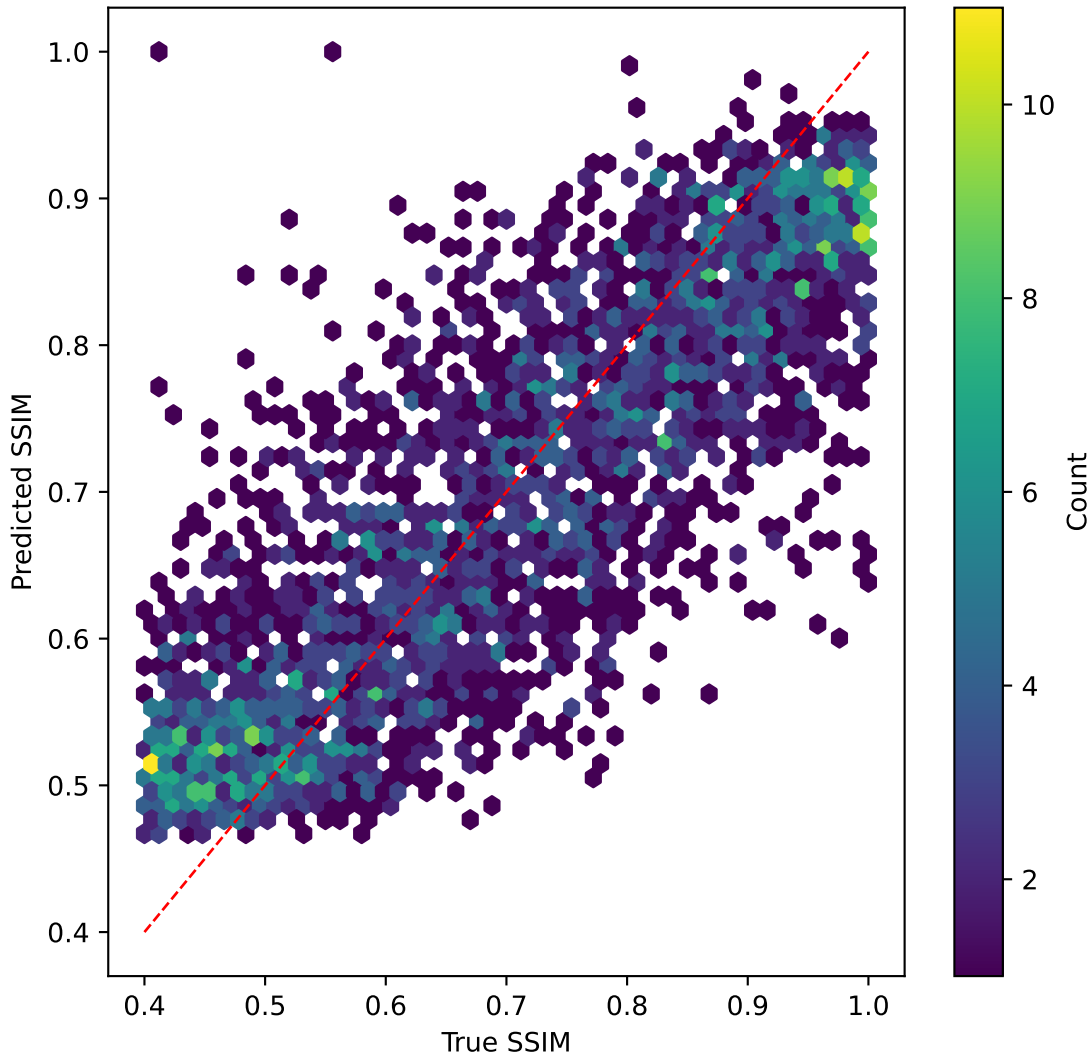
efficientnet on SSIM | R^2=0.646
