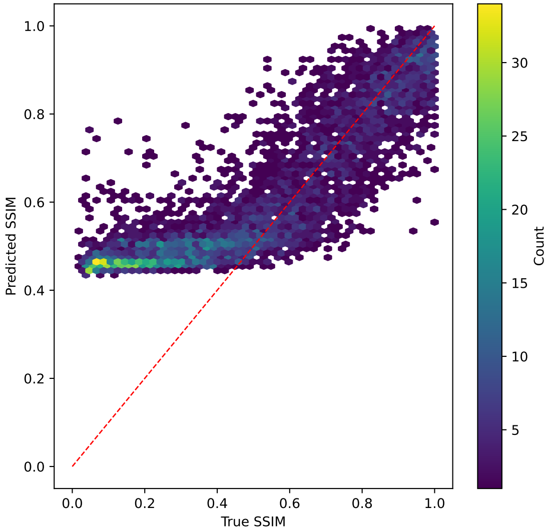
resnet50v2 on SSIM | R^2=0.253
