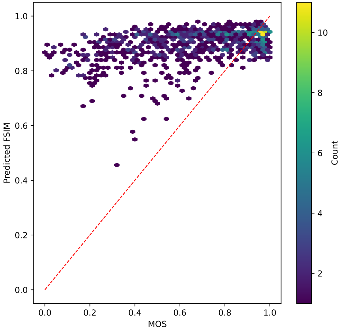
mobilenetv3 on FSIM AGAINST MOS | R^2=-0.746
