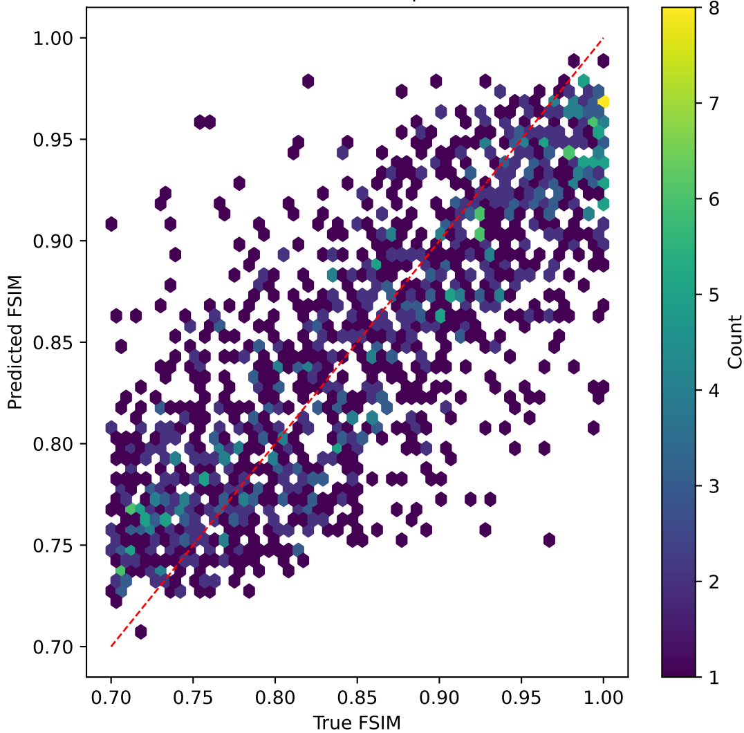
efficientnet on FSIM | R^2=0.628
