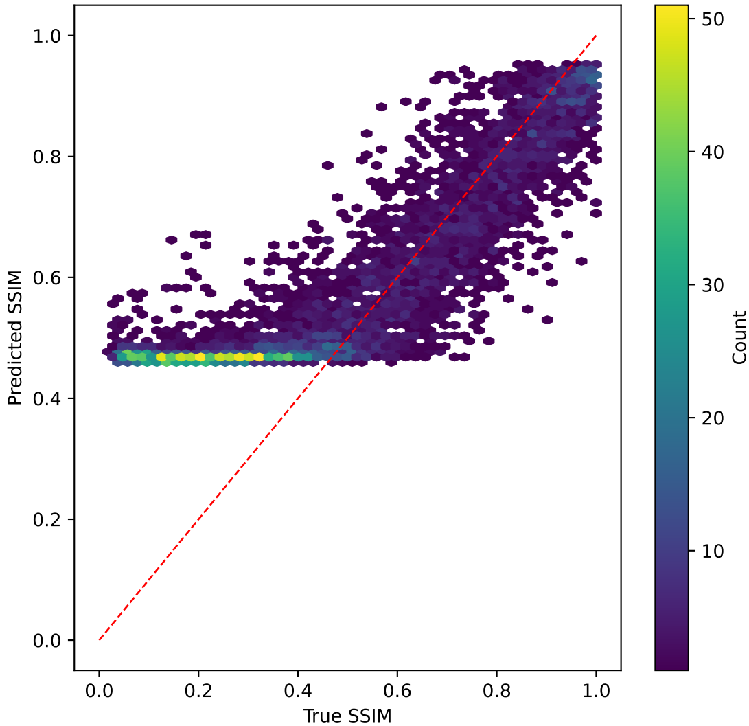
tinyvit on SSIM | R^2=0.343
