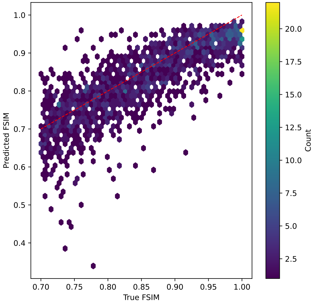
mobilevitv2 on FSIM | R^2=0.443
