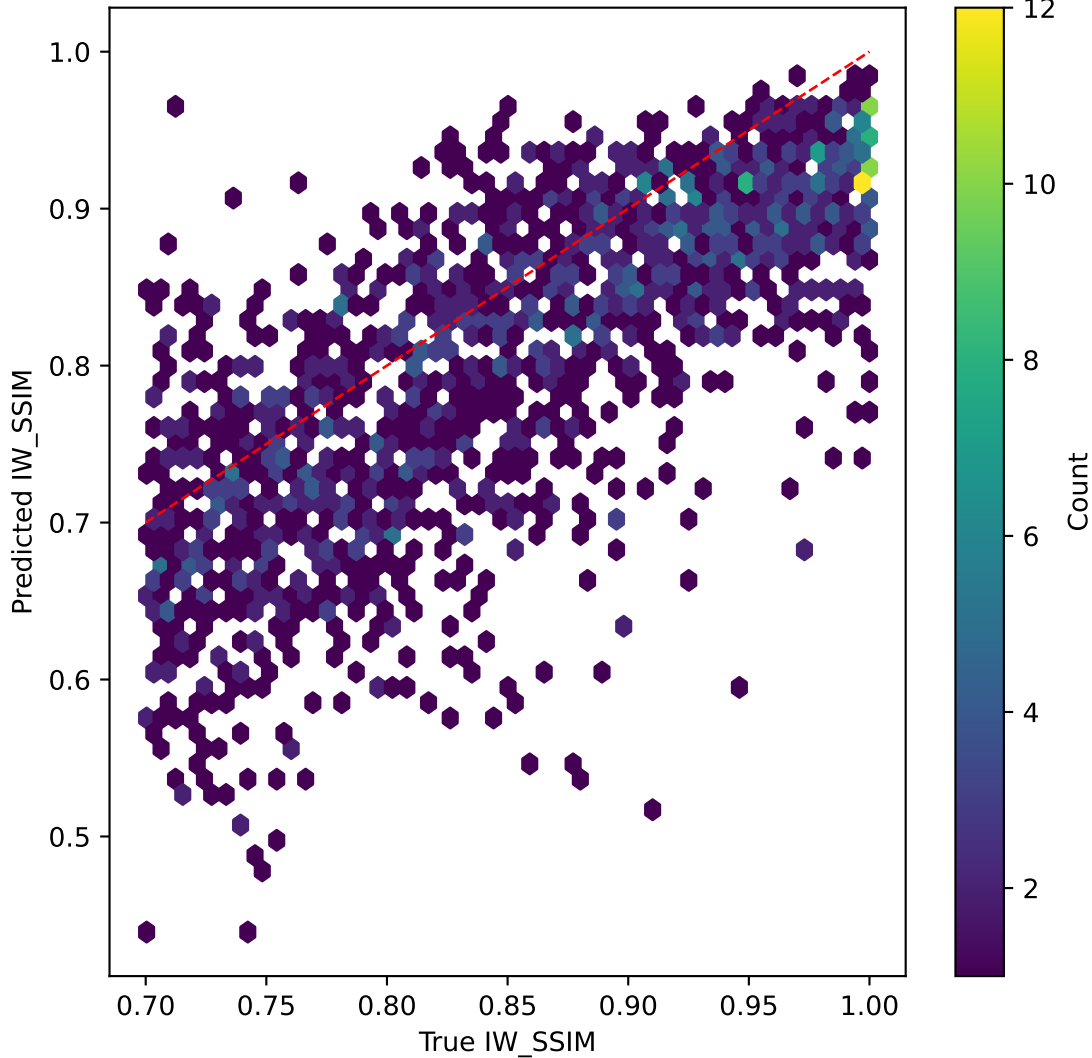
mobilevitv2 on IW_SSIM | R^2=0.114
