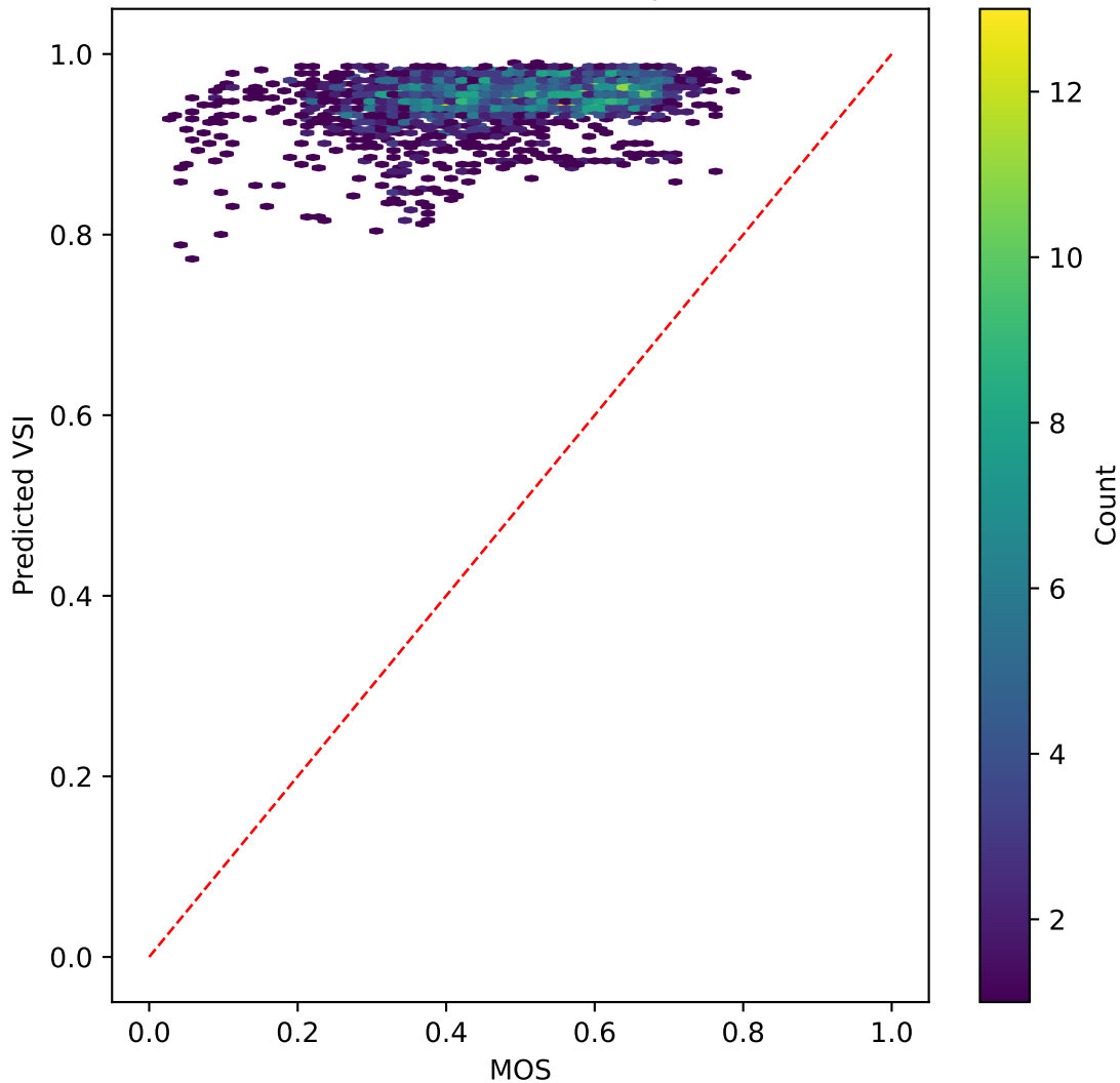
tinyvit on VSI AGAINST MOS | R^2=-10.699
