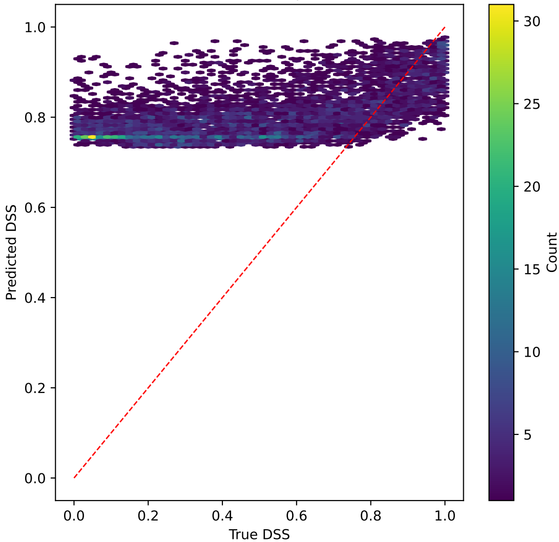
mobilevitv2 on DSS | R^2=-4.321
