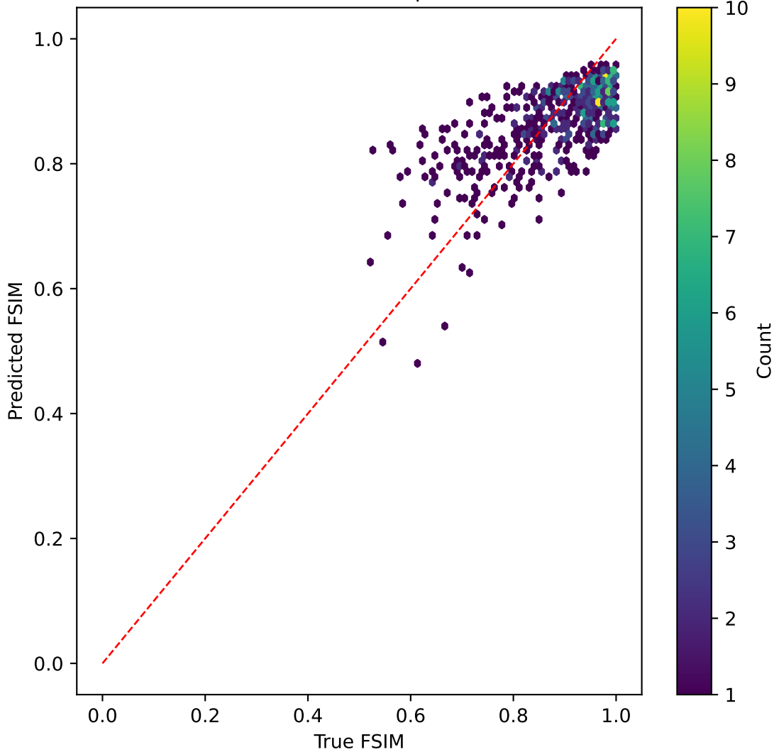
efficientnet on FSIM | R^2=0.331
