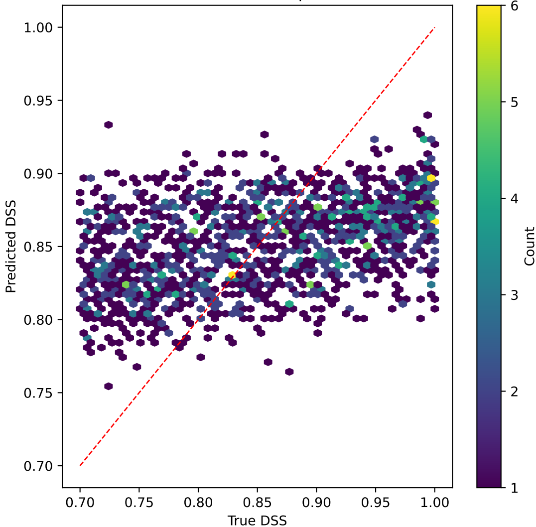
mobilenetv3 on DSS | R^2=0.155
