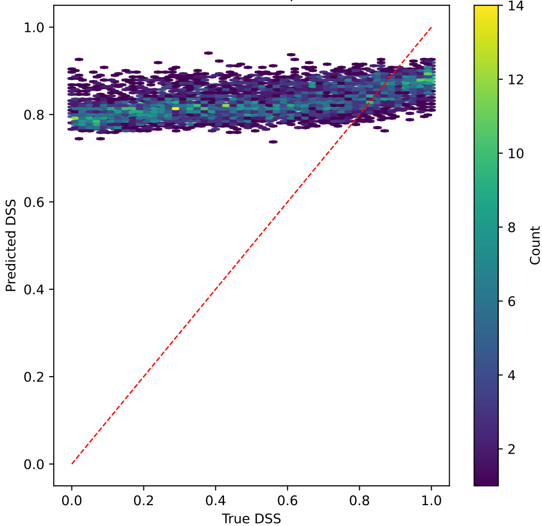
mobilenetv3 on DSS | R^2=-4.832
