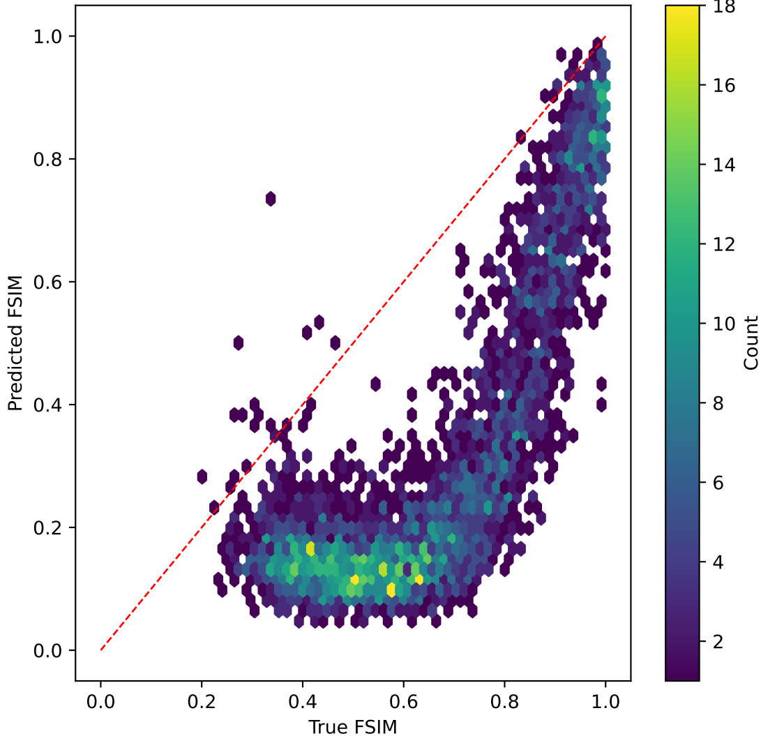
resnet50v2 on FSIM | R^2=-7.874
