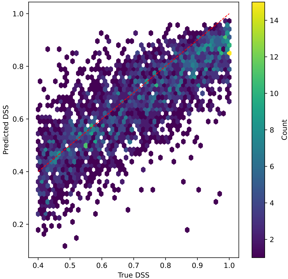
resnet50v2 on DSS | R^2=0.569
