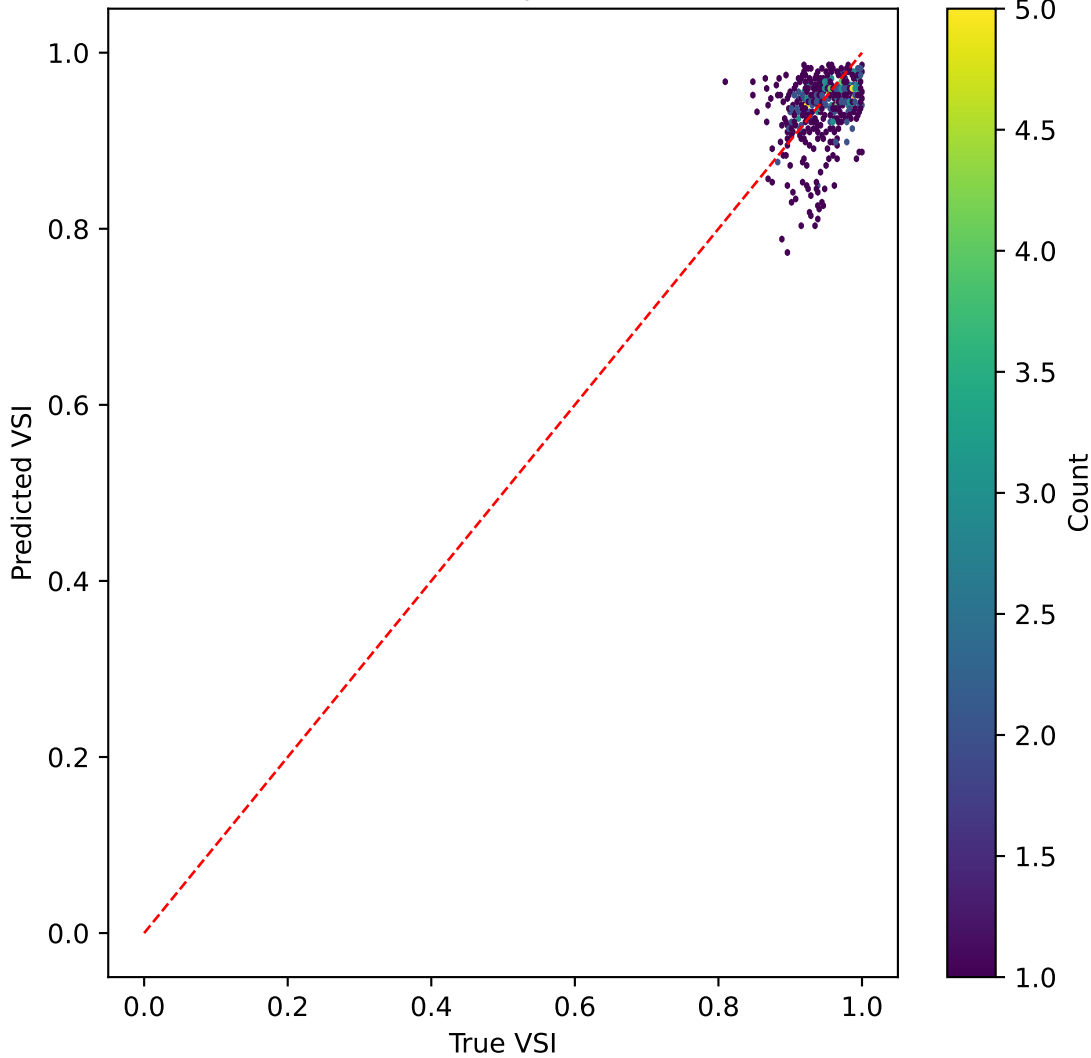
tinyvit on VSI | R^2=-2.246
