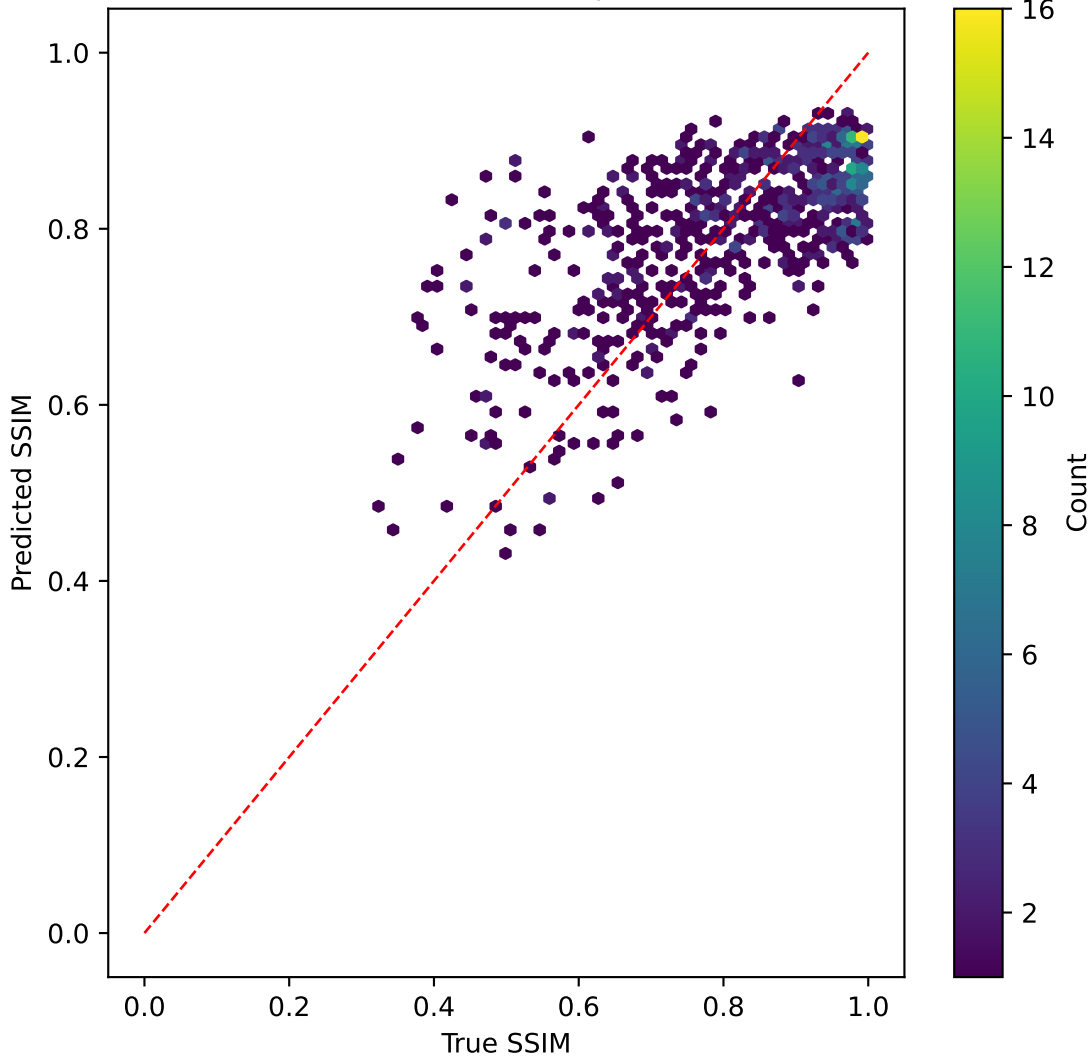
mobilenetv3 on SSIM | R^2=0.417
