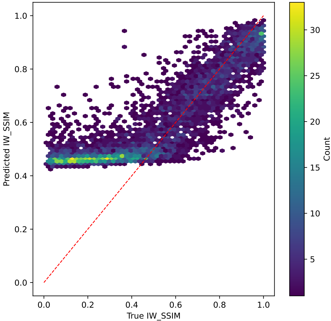
mobilevitv2 on IW_SSIM | R^2=0.329
