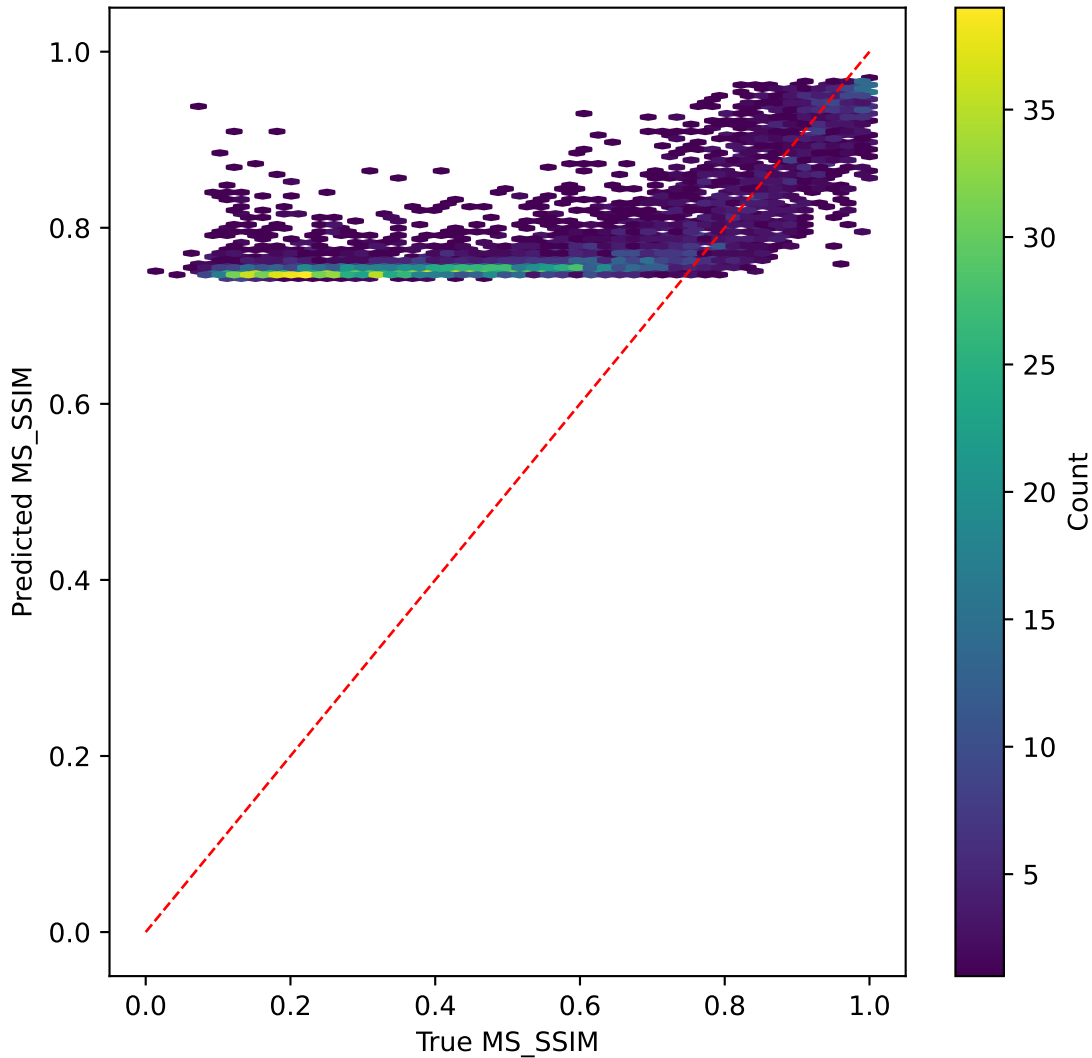
tinyvit on MS_SSIM | R^2=-1.018
