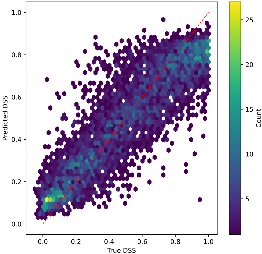
efficientnet on DSS | R^2=0.704
