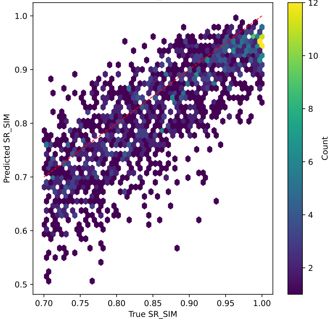
mobilenetv3 on SR_SIM | R^2=0.178
