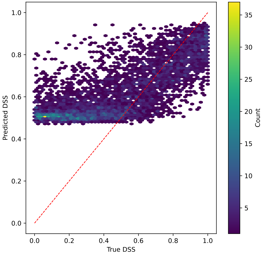
mobilevitv2 on DSS | R^2=-1.095
