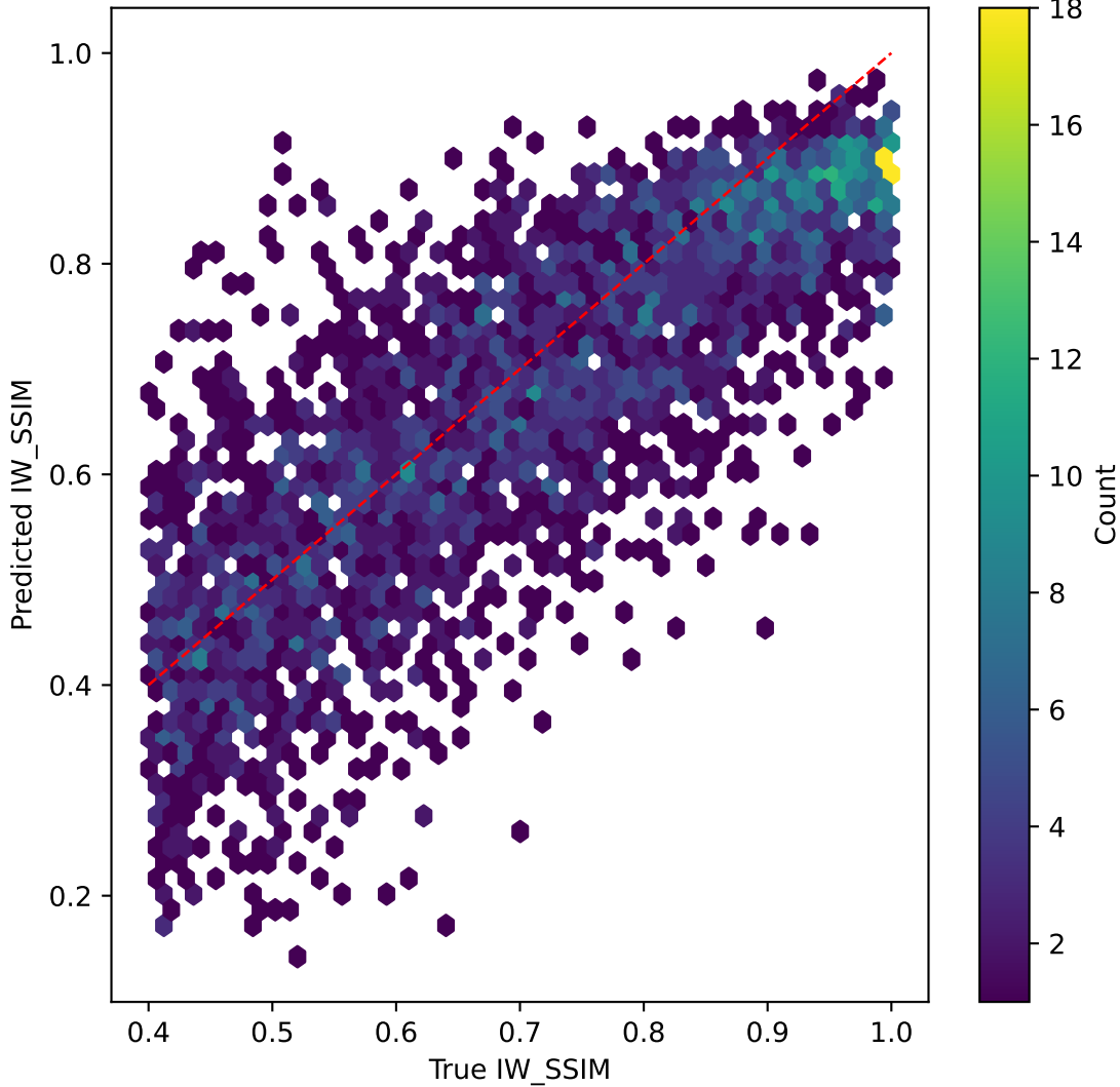
mobilenetv3 on IW_SSIM | R^2=0.602
