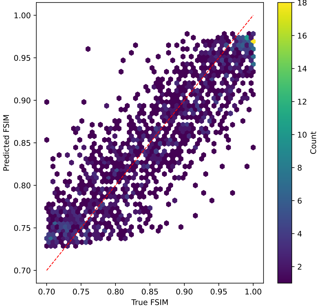
tinyvit on FSIM | R^2=0.740
