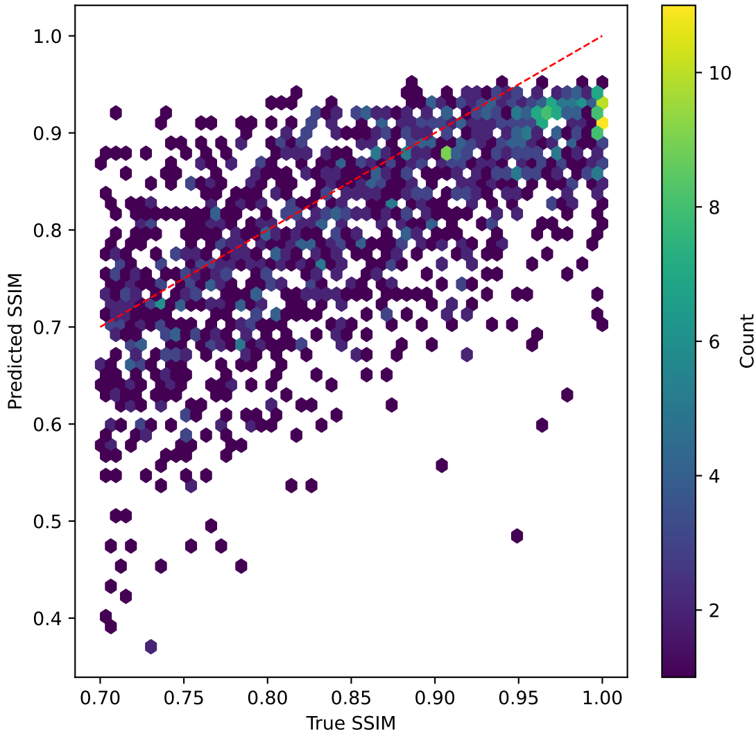
tinyvit on SSIM | R^2=-0.158
