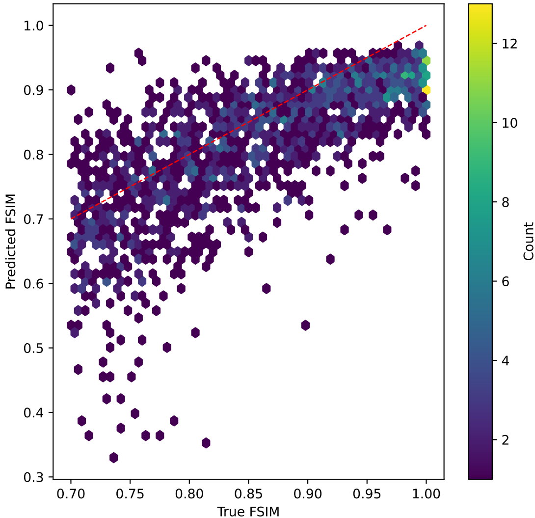
efficientnet on FSIM | R^2=0.004
