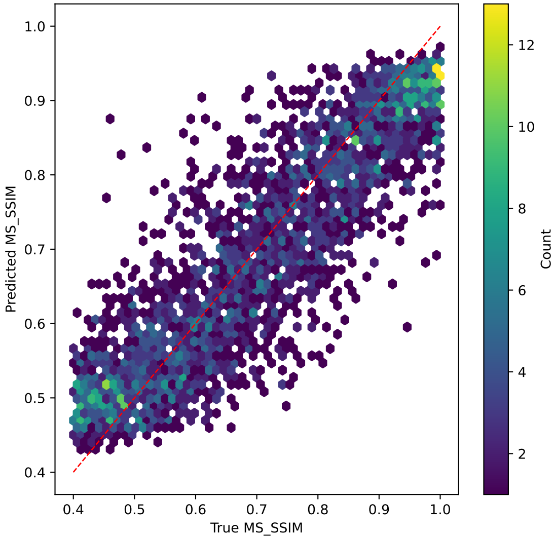
mobilenetv3 on MS_SSIM | R^2=0.750
