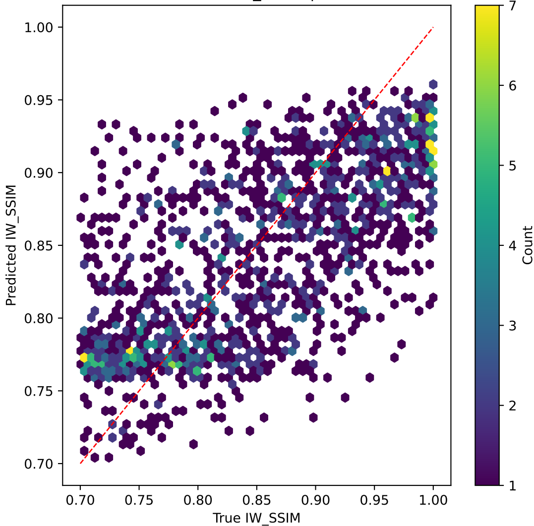
efficientnet on IW_SSIM | R^2=0.434
