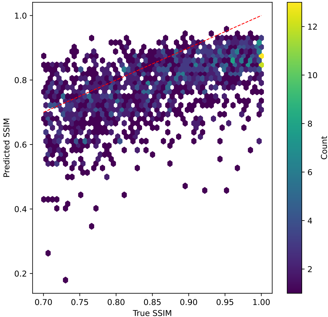
efficientnet on SSIM | R^2=-0.780
