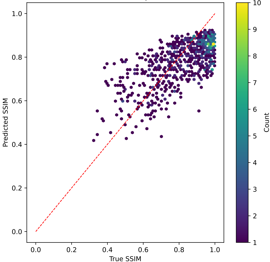
efficientnet on SSIM | R^2=0.353
