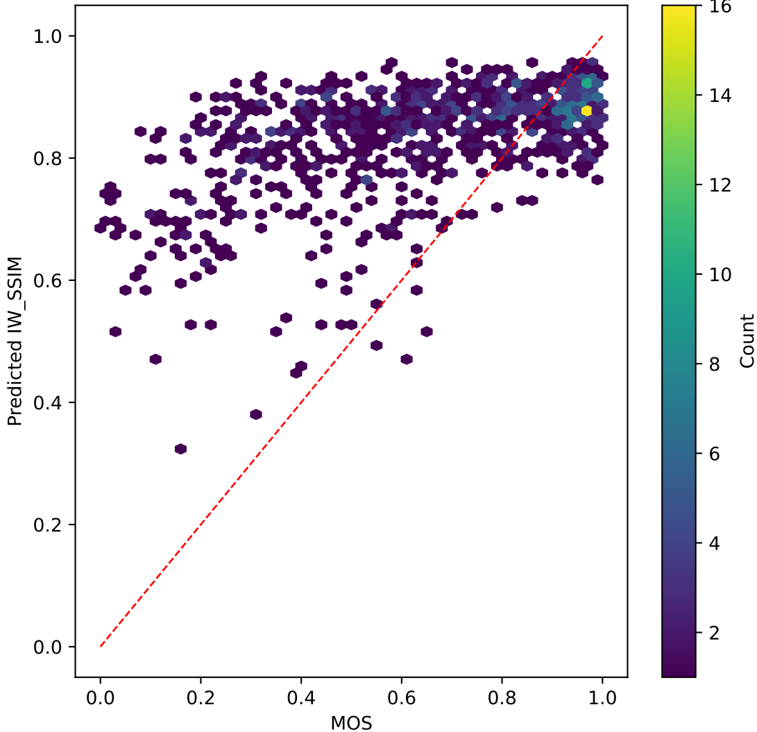
mobilenetv3 on IW_SSIM AGAINST MOS | R^2=-0.269
