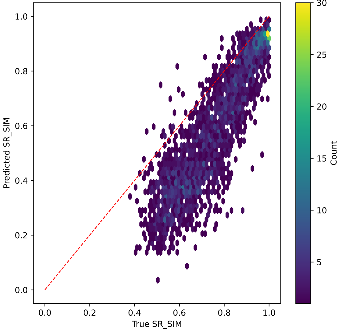
mobilenetv3 on SR_SIM | R^2=-2.757
