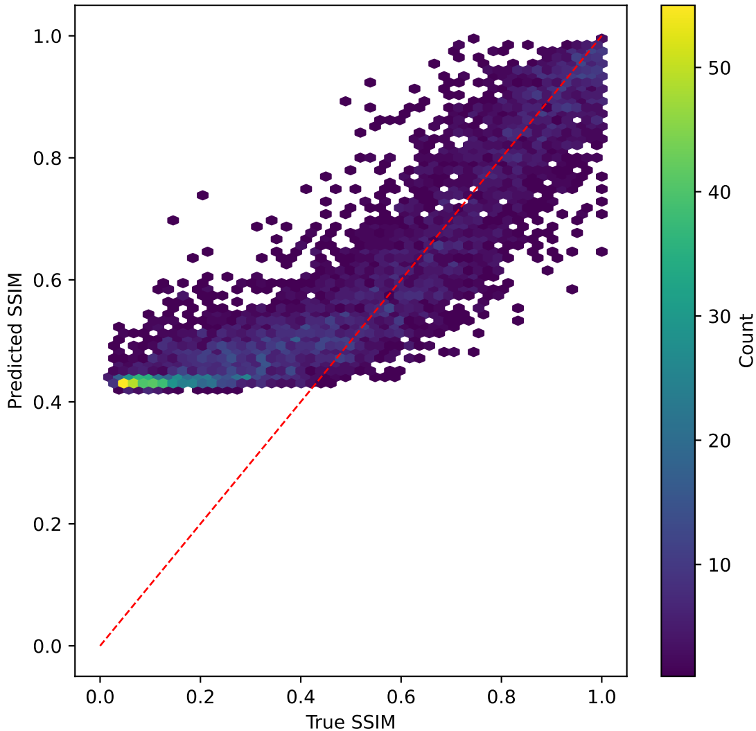
resnet50v2 on SSIM | R^2=0.363
