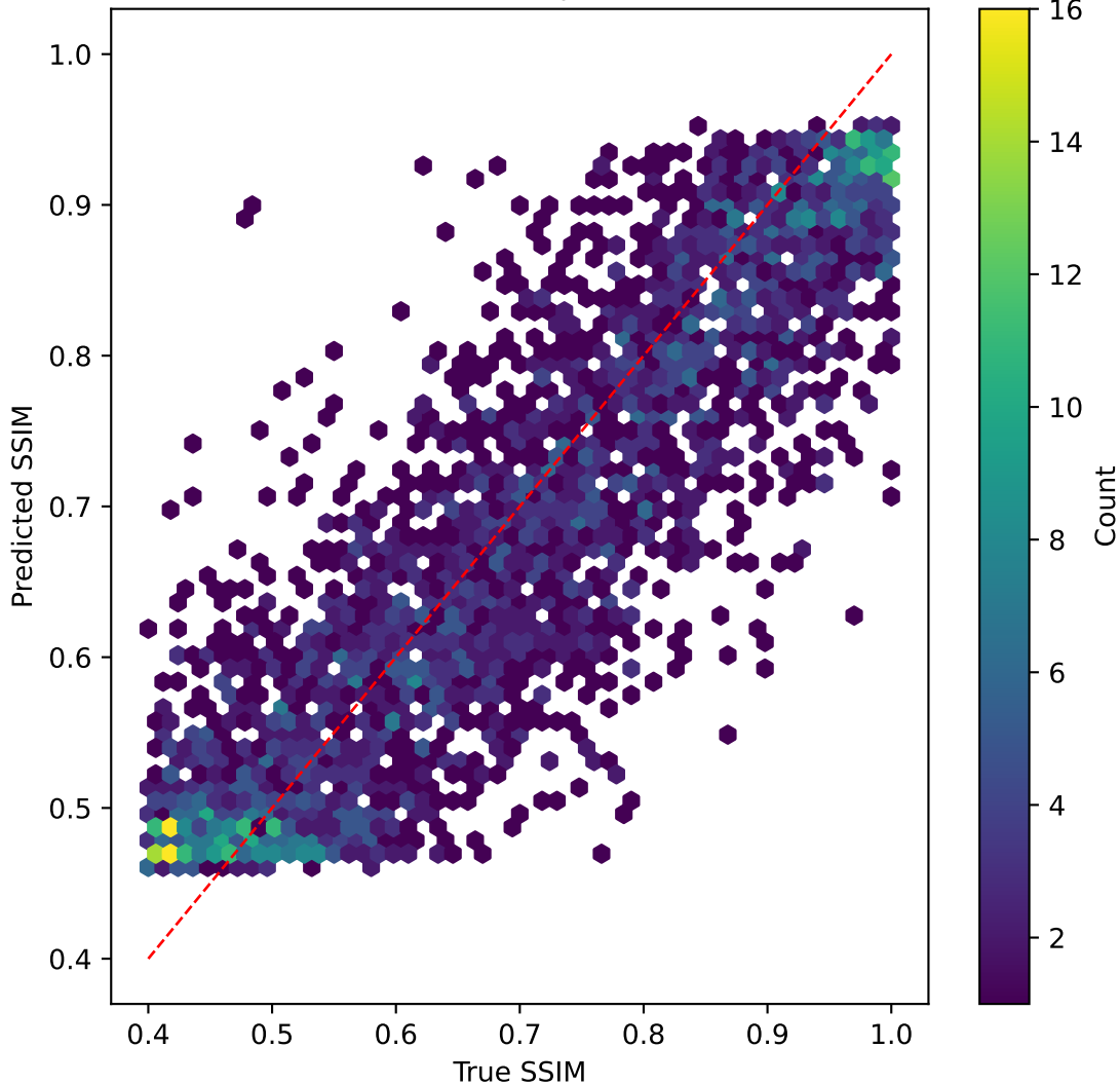
tinyvit on SSIM | R^2=0.751
