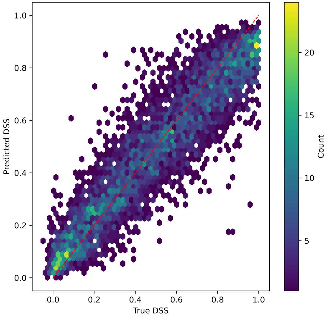
resnet50v2 on DSS | R^2=0.829
