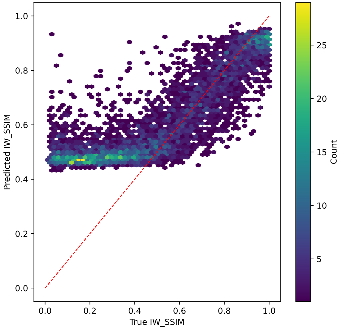
mobilenetv3 on IW_SSIM | R^2=0.216
