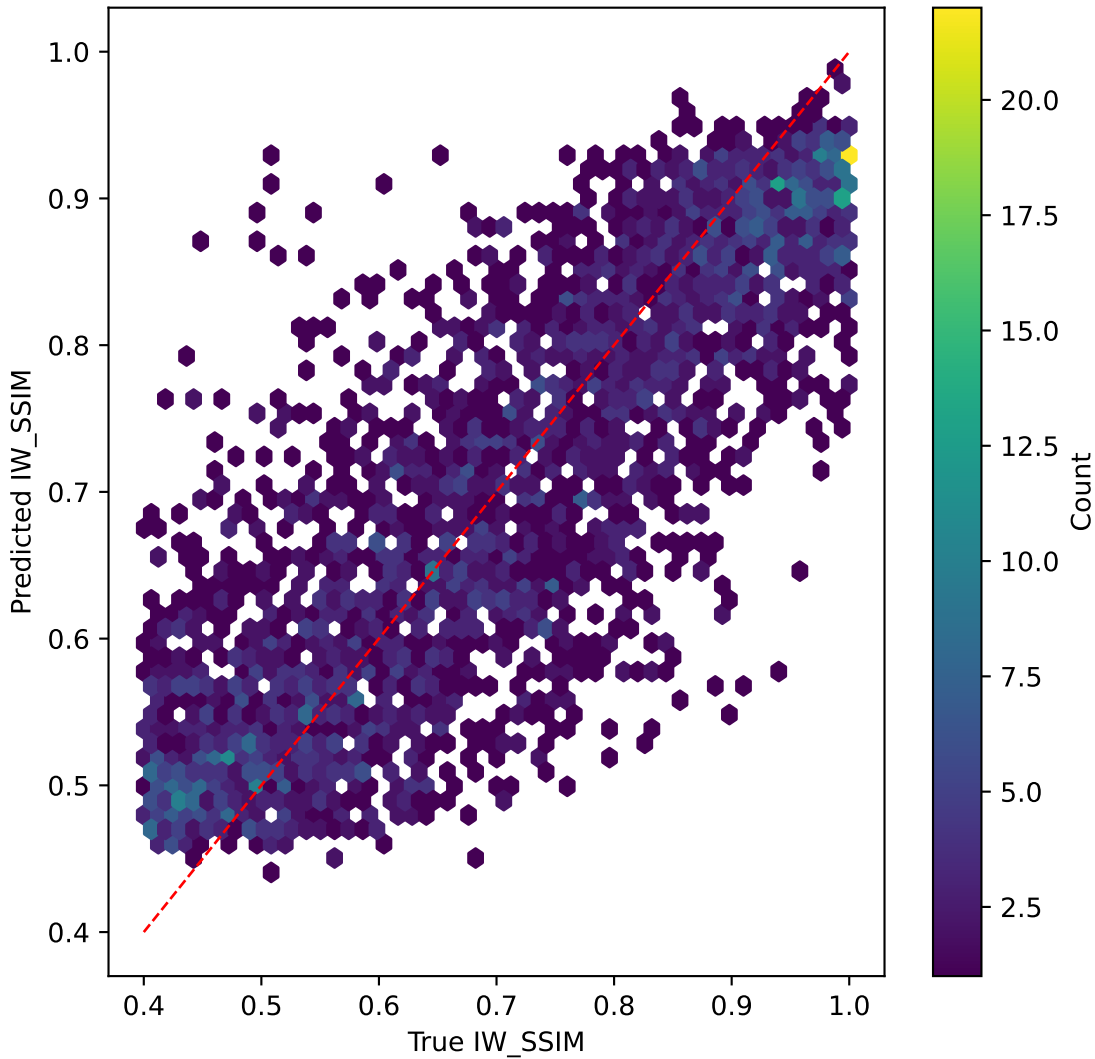
mobilenetv3 on IW_SSIM | R^2=0.719
