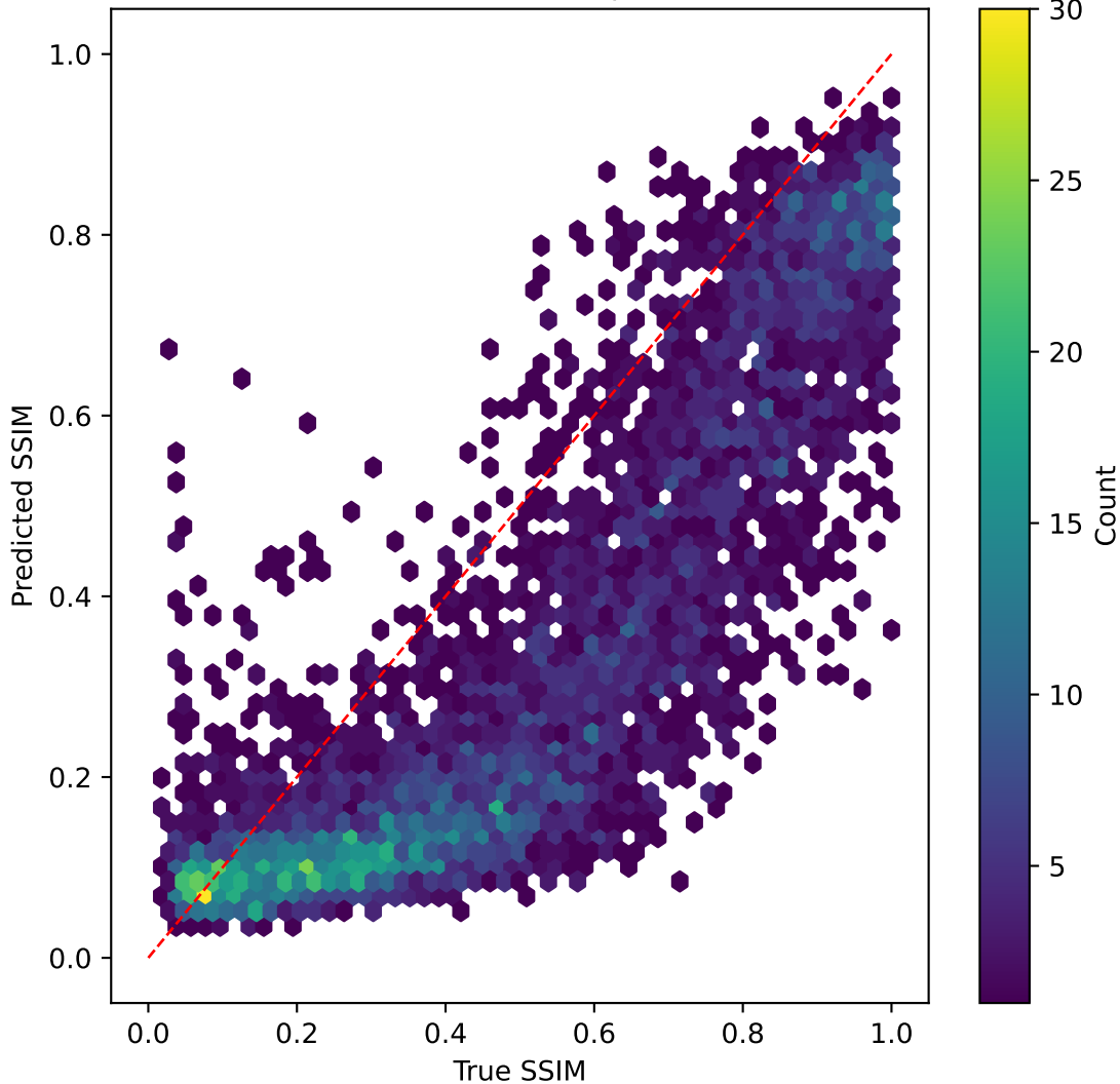
mobilenetv3 on SSIM | R^2=0.157
