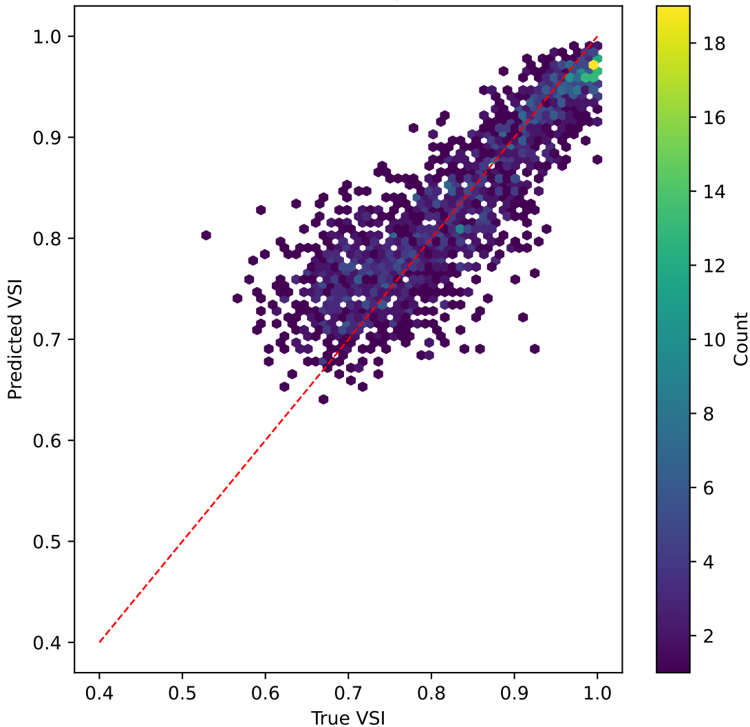
efficientnet on VSI | R^2=0.578
