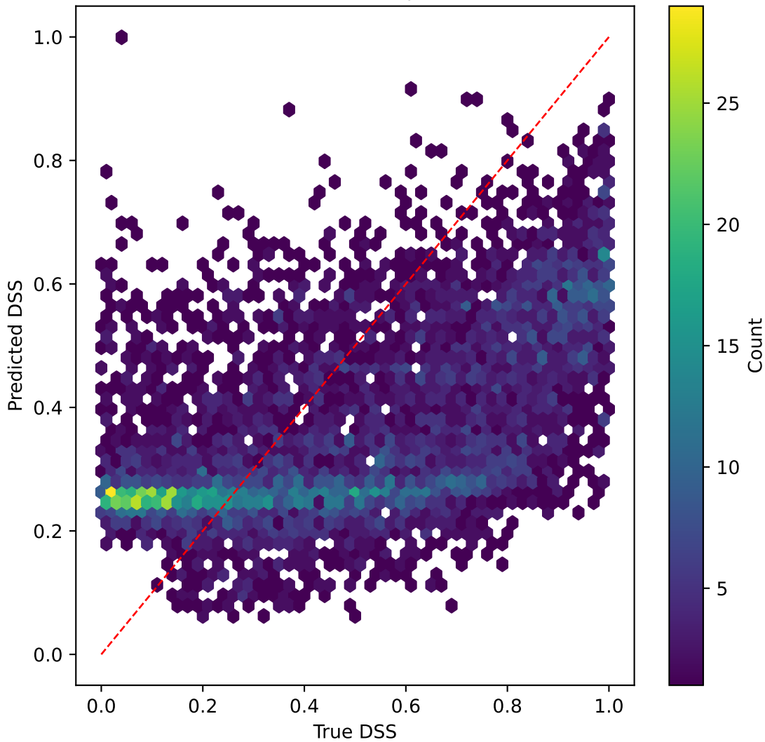
efficientnet on DSS | R^2=0.115
