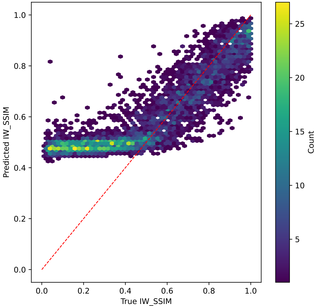
resnet50v2 on IW_SSIM | R^2=0.294
