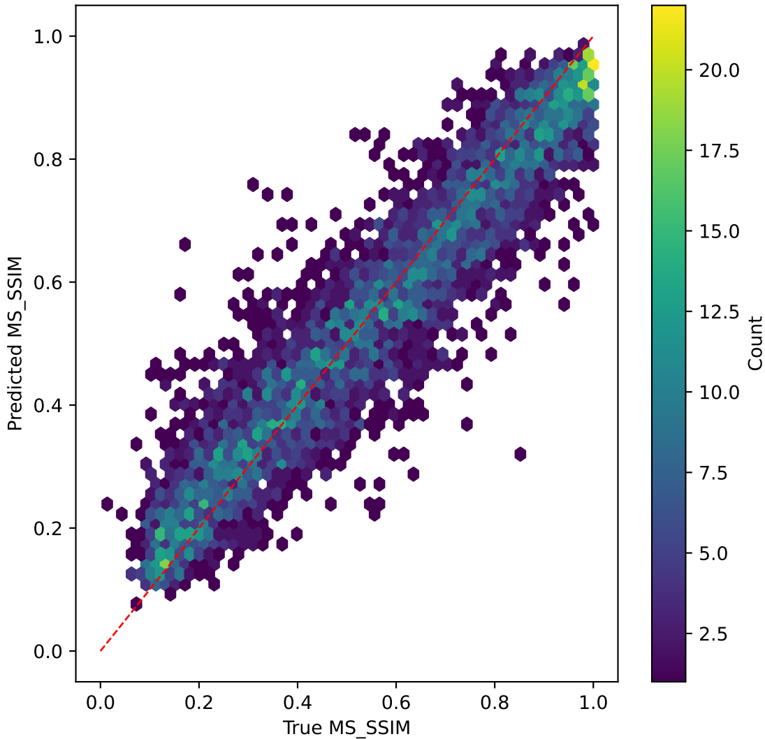
resnet50v2 on MS_SSIM | R^2=0.836
