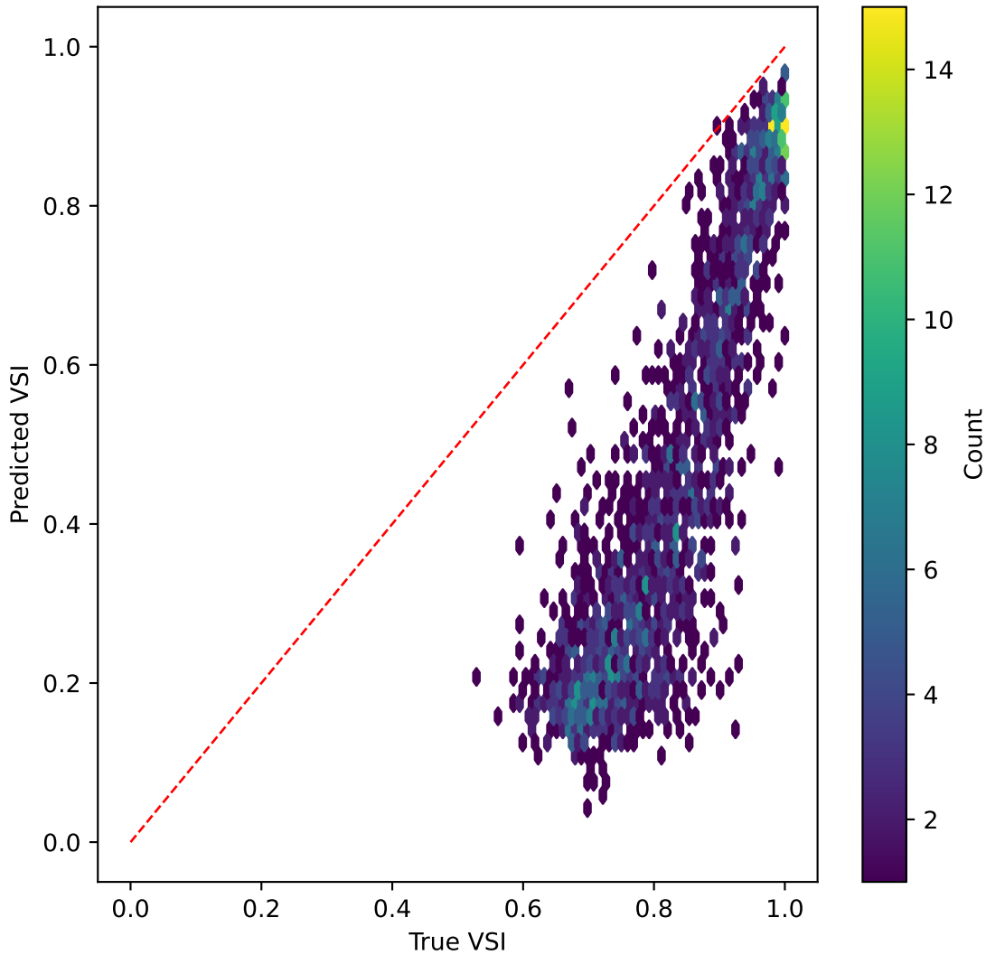
mobilenetv3 on VSI | R^2=-31.830
