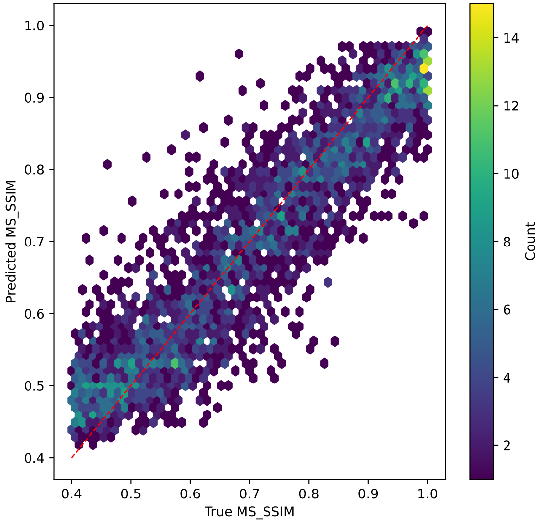
resnet50v2 on MS_SSIM | R^2=0.810
