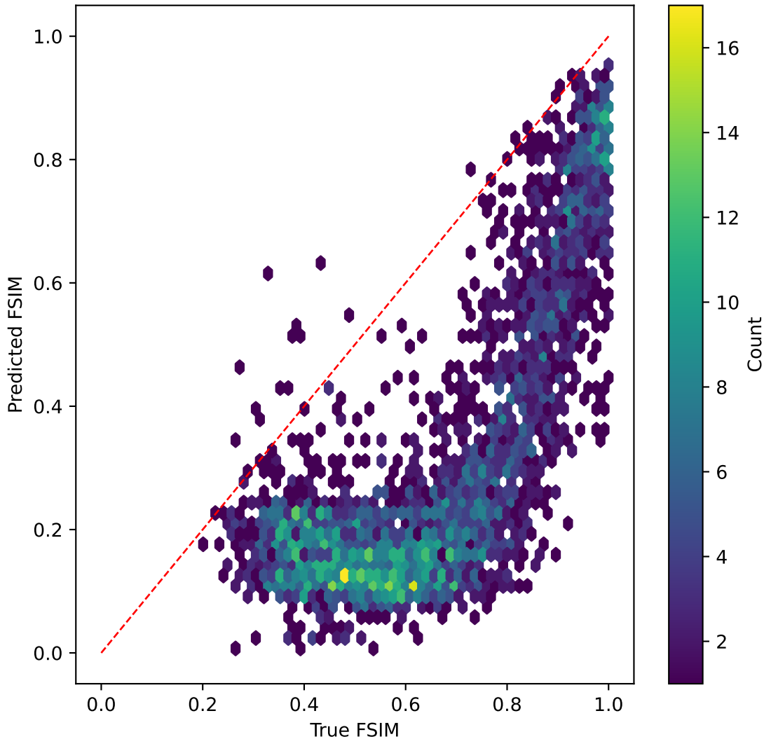
efficientnet on FSIM | R^2=-7.823
