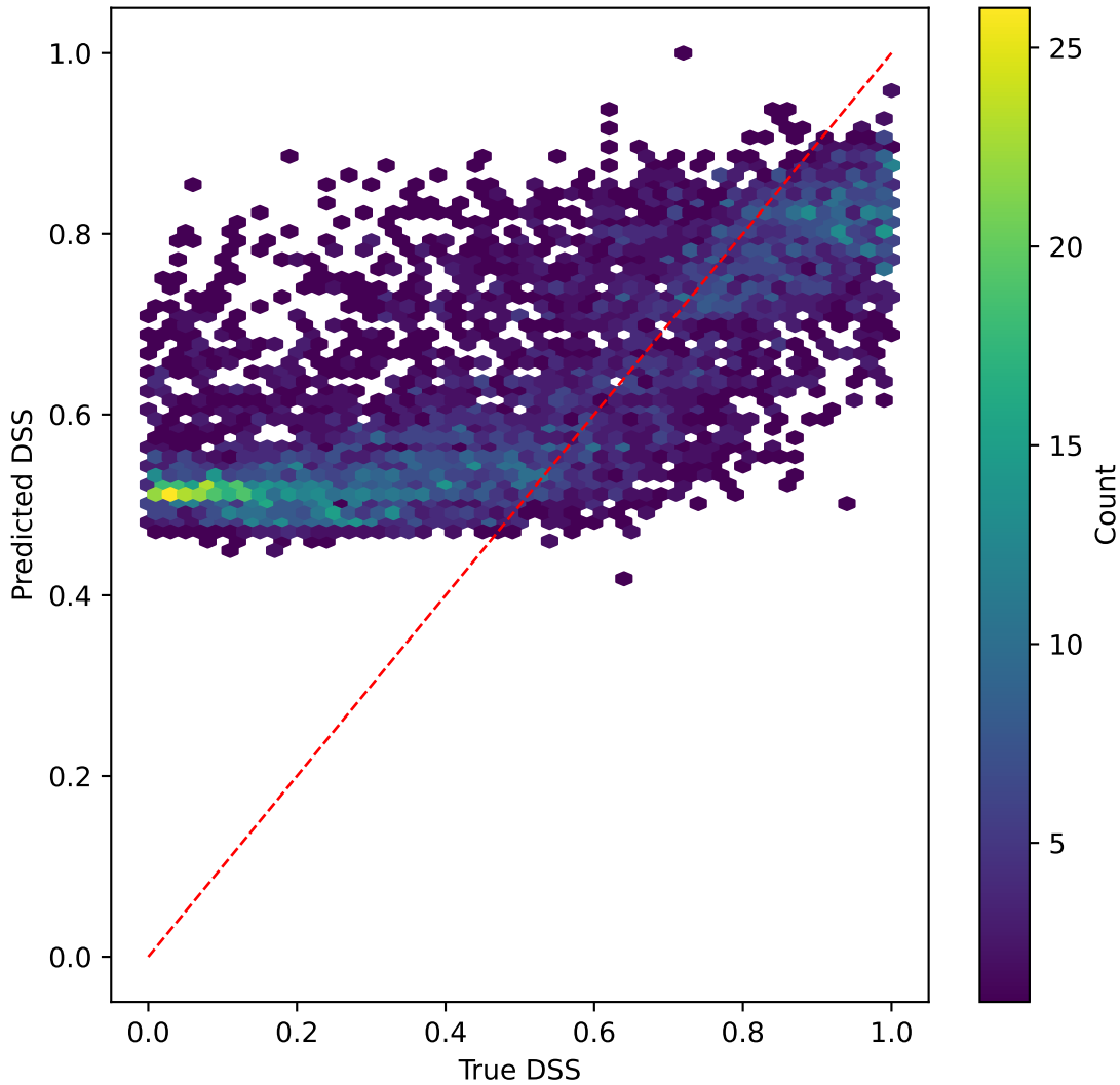
efficientnet on DSS | R^2=-1.185
