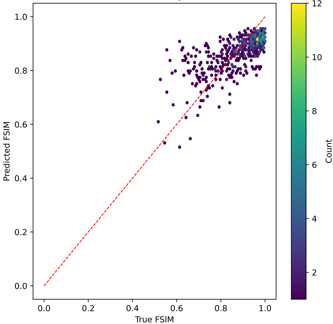
resnet50v2 on FSIM | R^2=0.383
