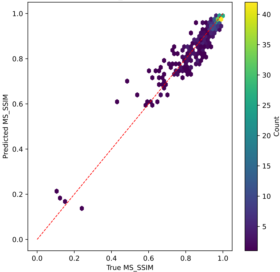
tinyvit on MS_SSIM | R^2=0.908
