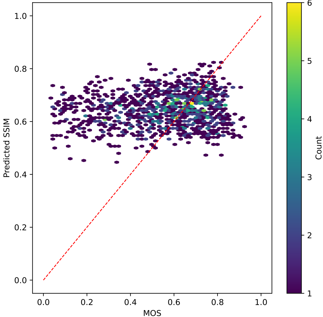
tinyvit on SSIM AGAINST MOS | R^2=-0.221
