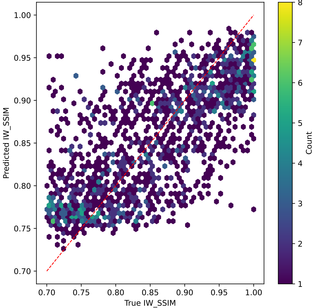
resnet50v2 on IW_SSIM | R^2=0.525
