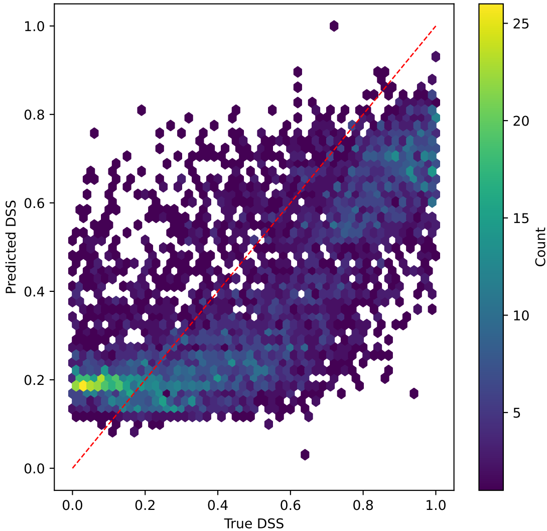
efficientnet on DSS | R^2=0.388
