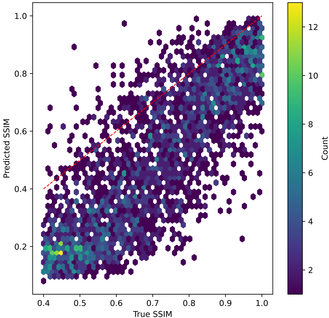
resnet50v2 on SSIM | R^2=-1.363
