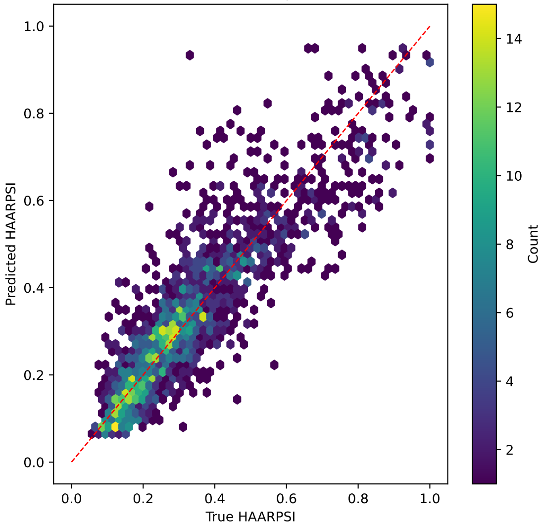
tinyvit on HAARPSI | R^2=0.762
