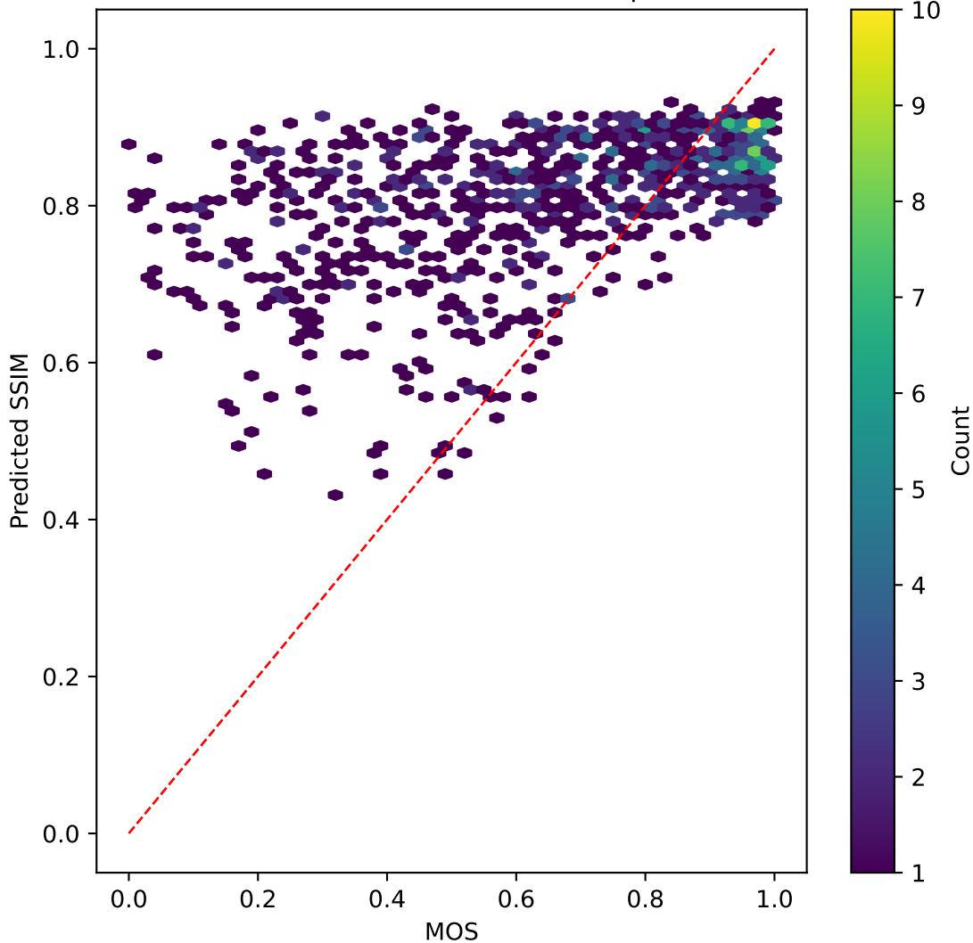
mobilenetv3 on SSIM AGAINST MOS | R^2=-0.174
