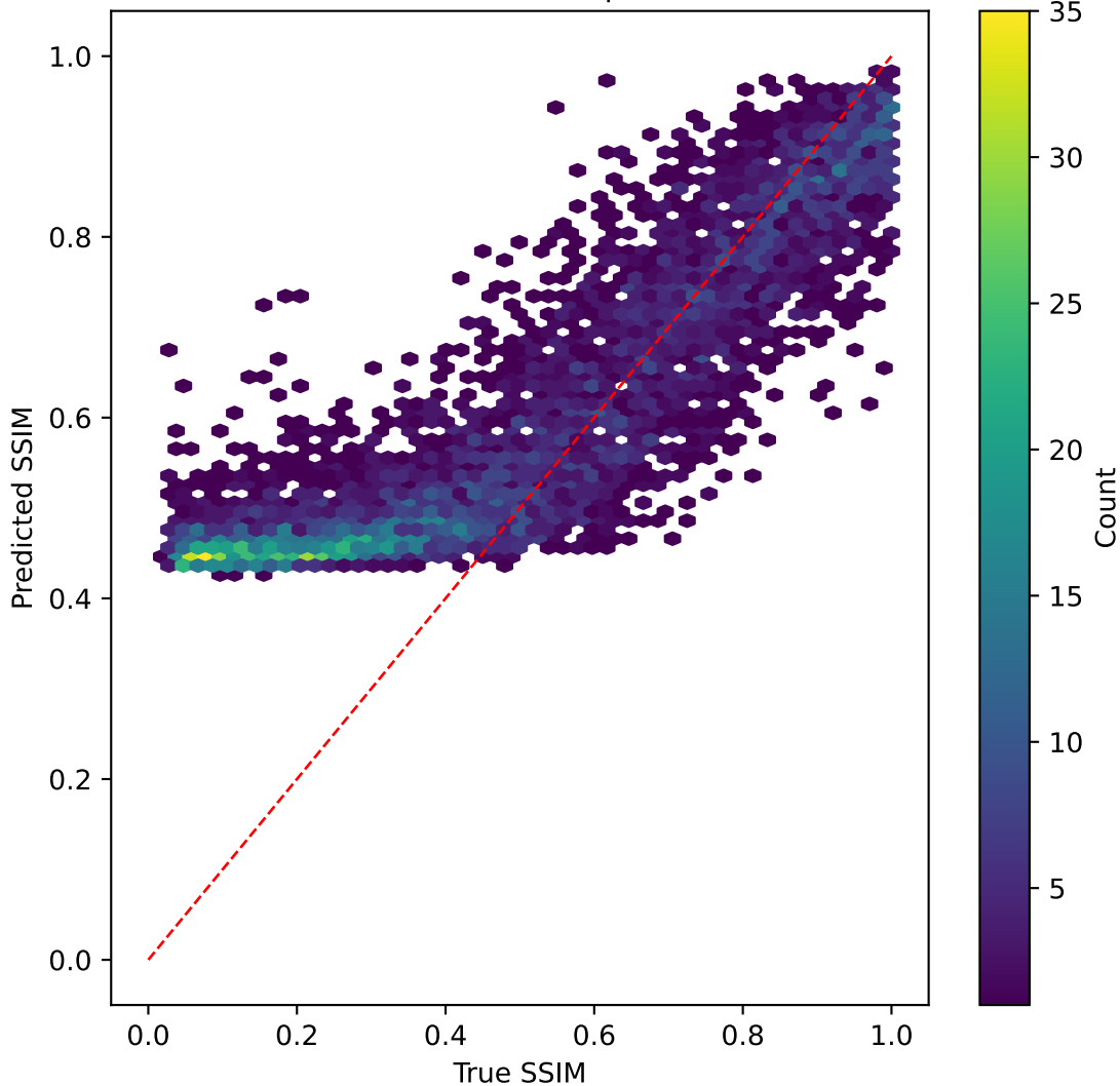
mobilevitv2 on SSIM | R^2=0.329
