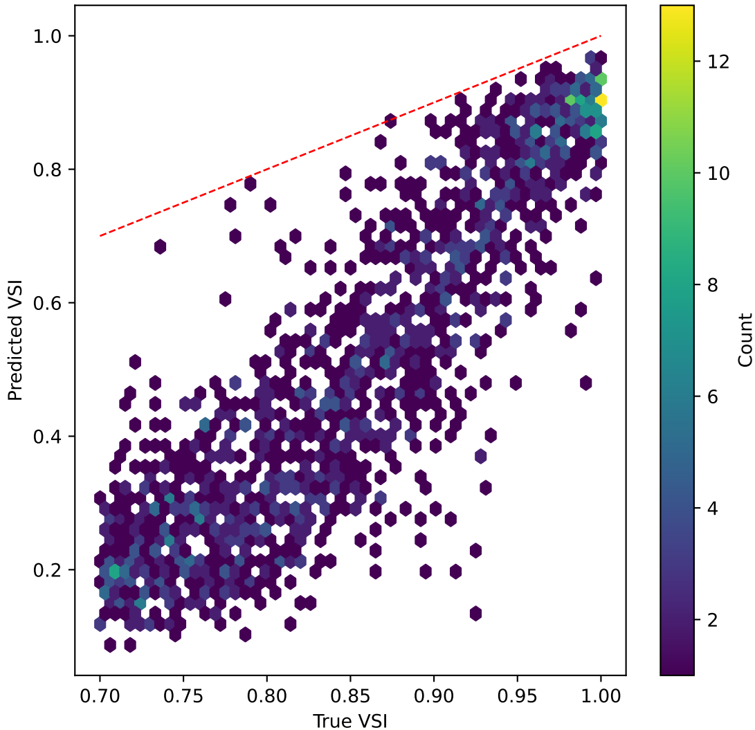
mobilenetv3 on VSI | R^2=-34.574
