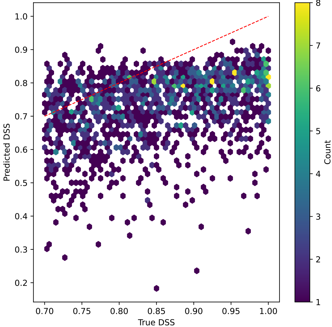
mobilenetv3 on DSS | R^2=-2.255
