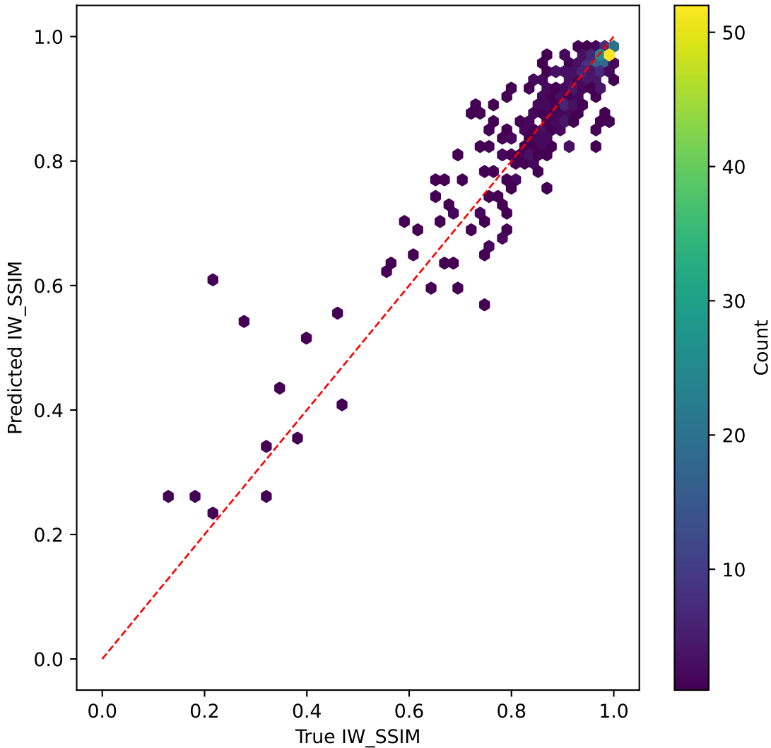
tinyvit on IW_SSIM | R^2=0.865
