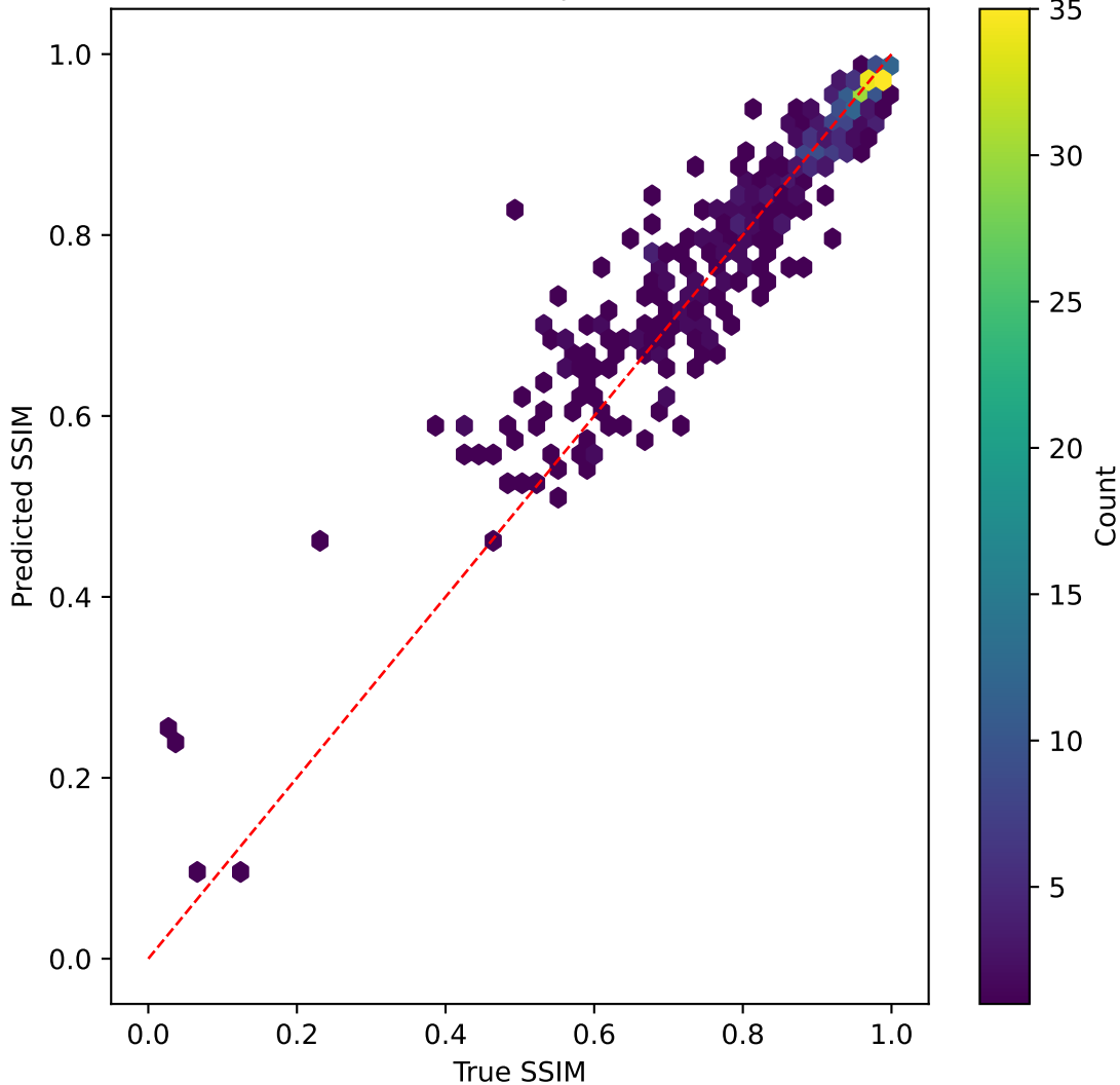
tinyvit on SSIM | R^2=0.896
