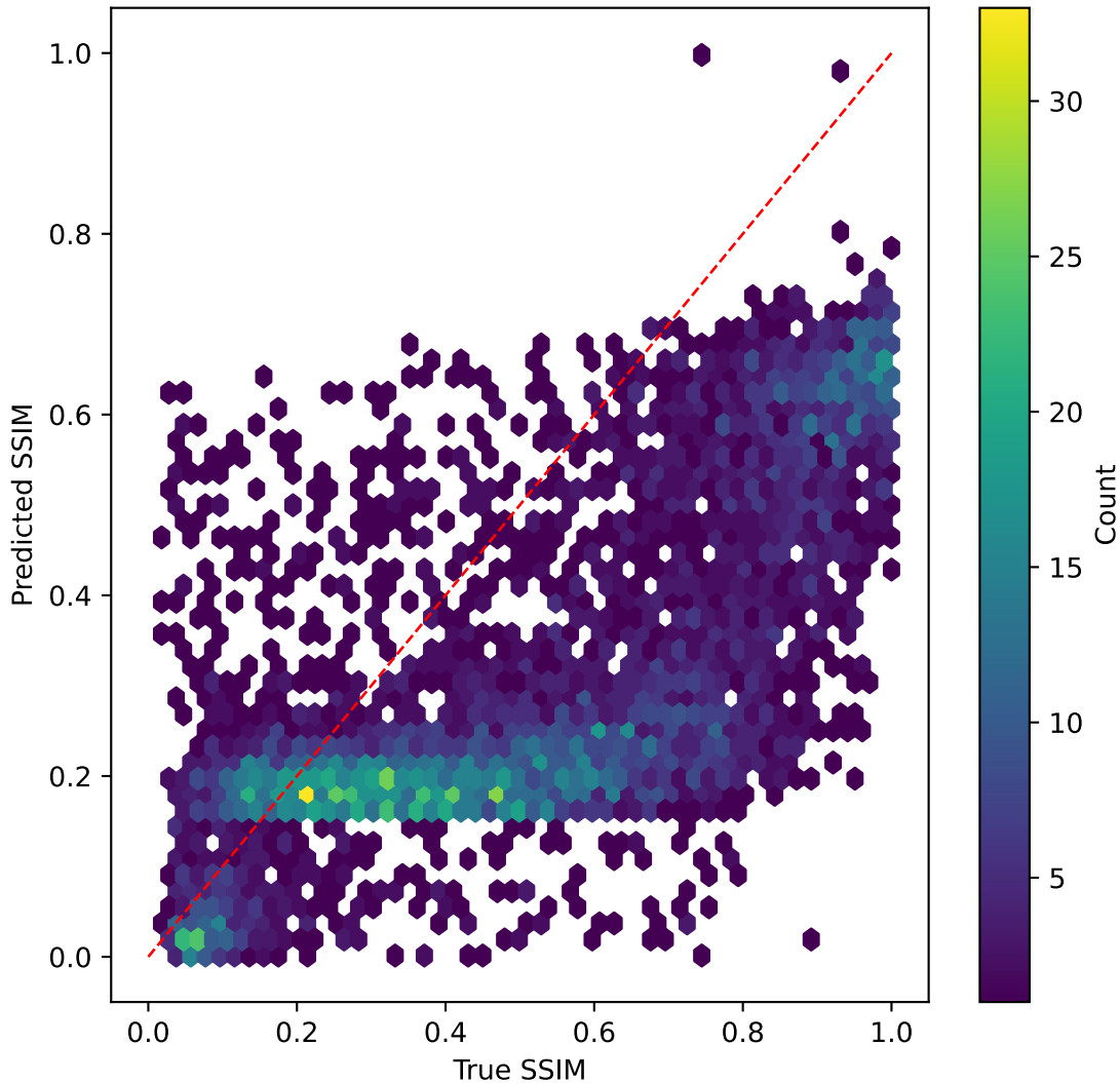
efficientnet on SSIM | R^2=-0.095
