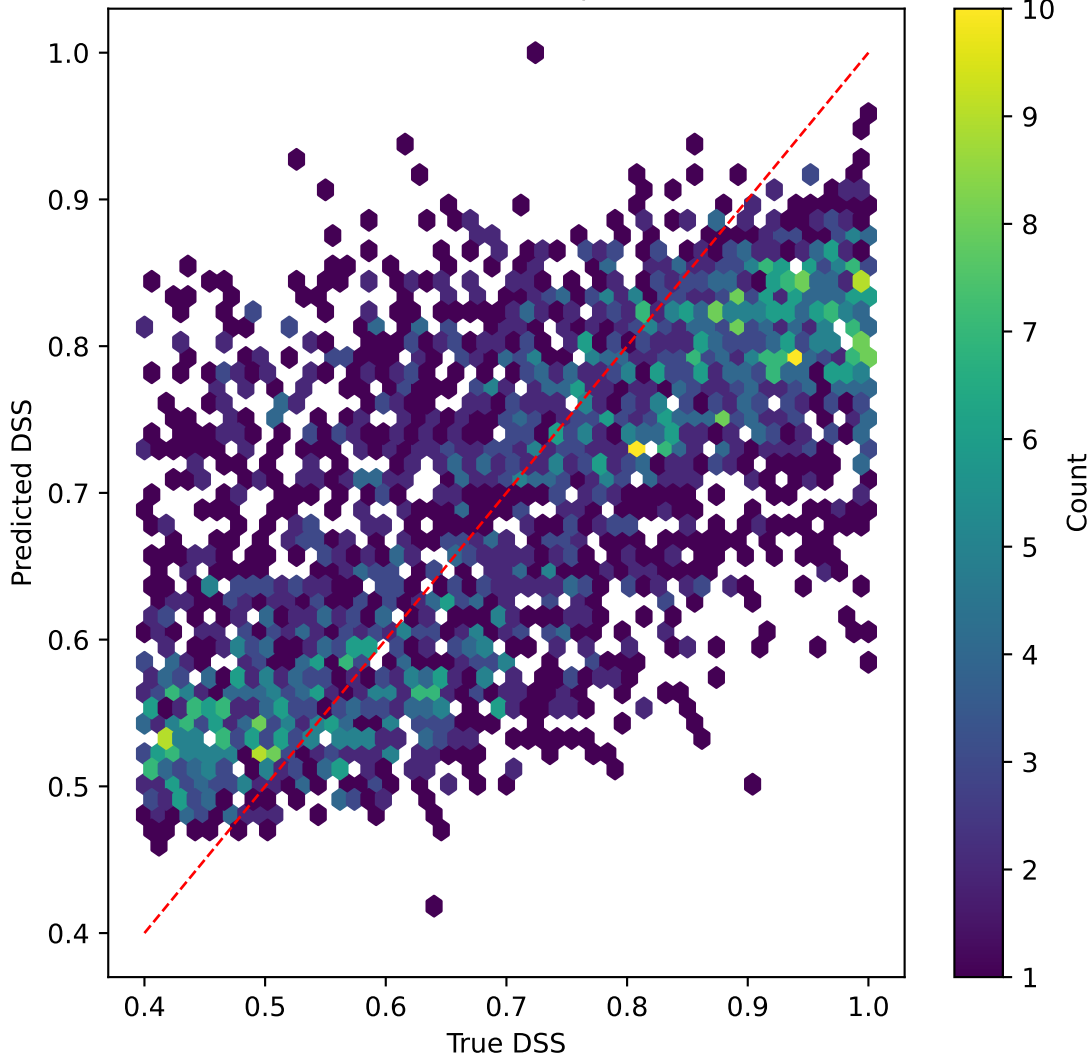
efficientnet on DSS | R^2=0.460
