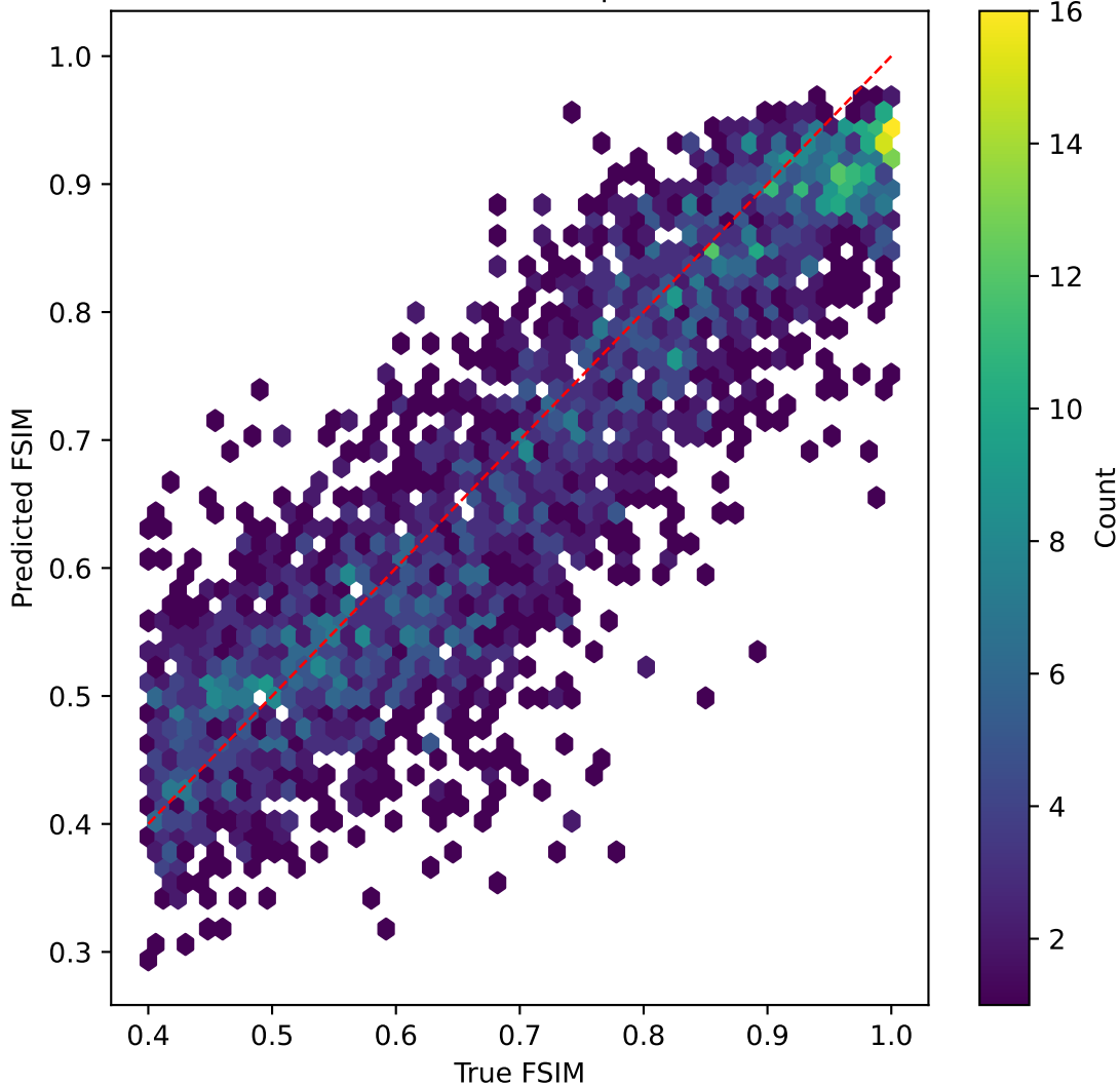
efficientnet on FSIM | R^2=0.619
