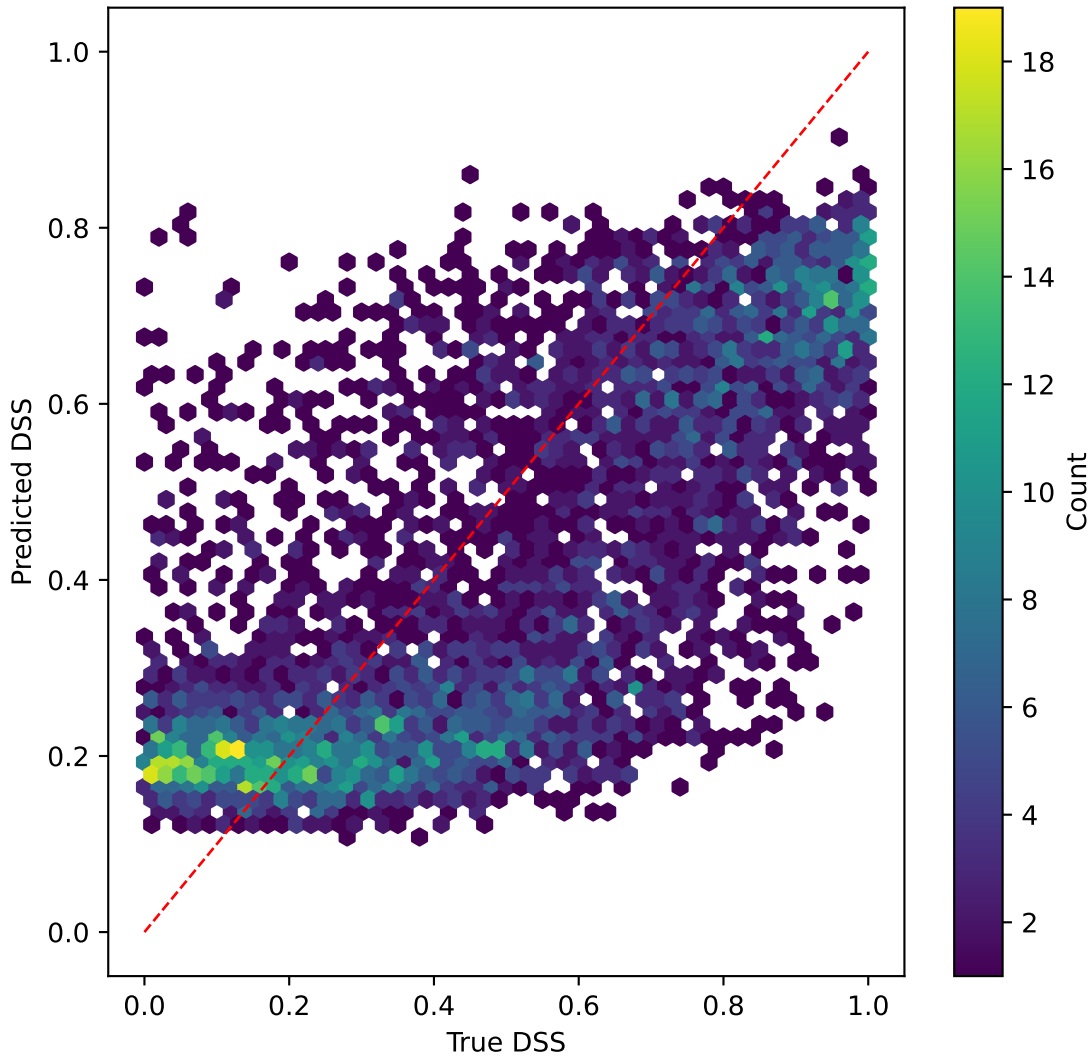
mobilenetv3 on DSS | R^2=0.402
