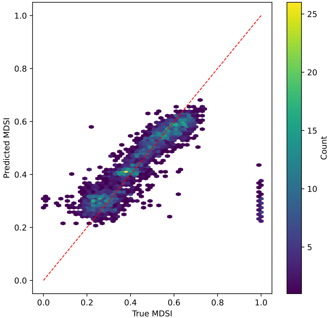
resnet50v2 on MDSI | R^2=0.239
