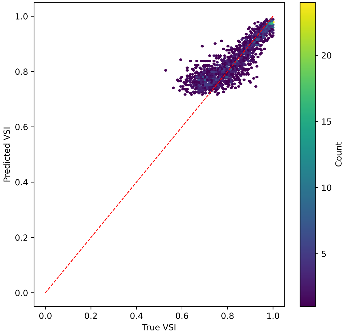
mobilevitv2 on VSI | R^2=0.698
