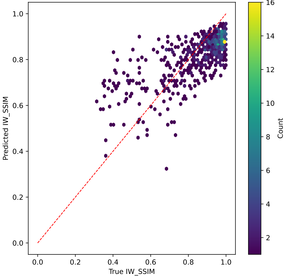
mobilenetv3 on IW_SSIM | R^2=0.378
