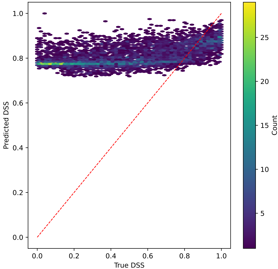
efficientnet on DSS | R^2=-4.472
