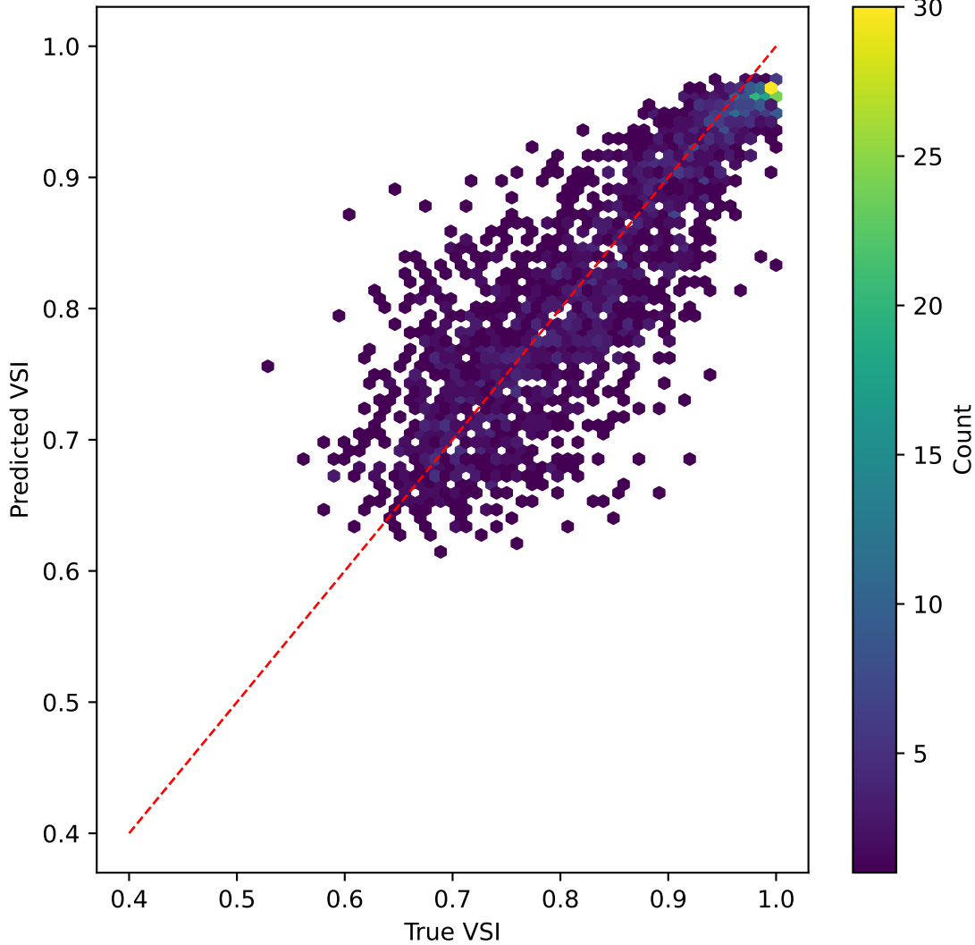
mobilevitv2 on VSI | R^2=0.363
