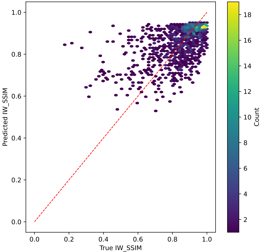
tinyvit on IW_SSIM | R^2=0.177
