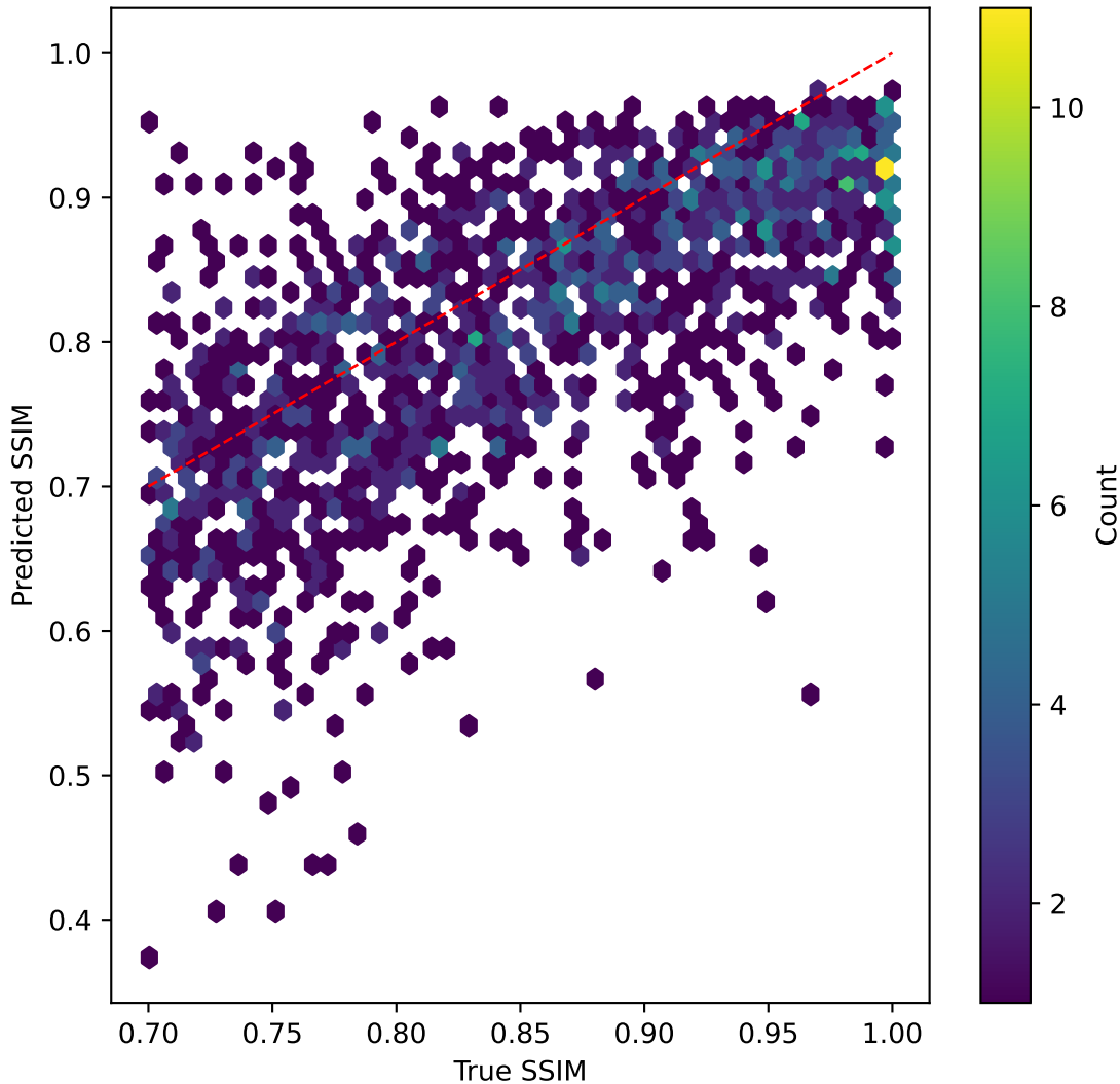
mobilevitv2 on SSIM | R^2=-0.036
