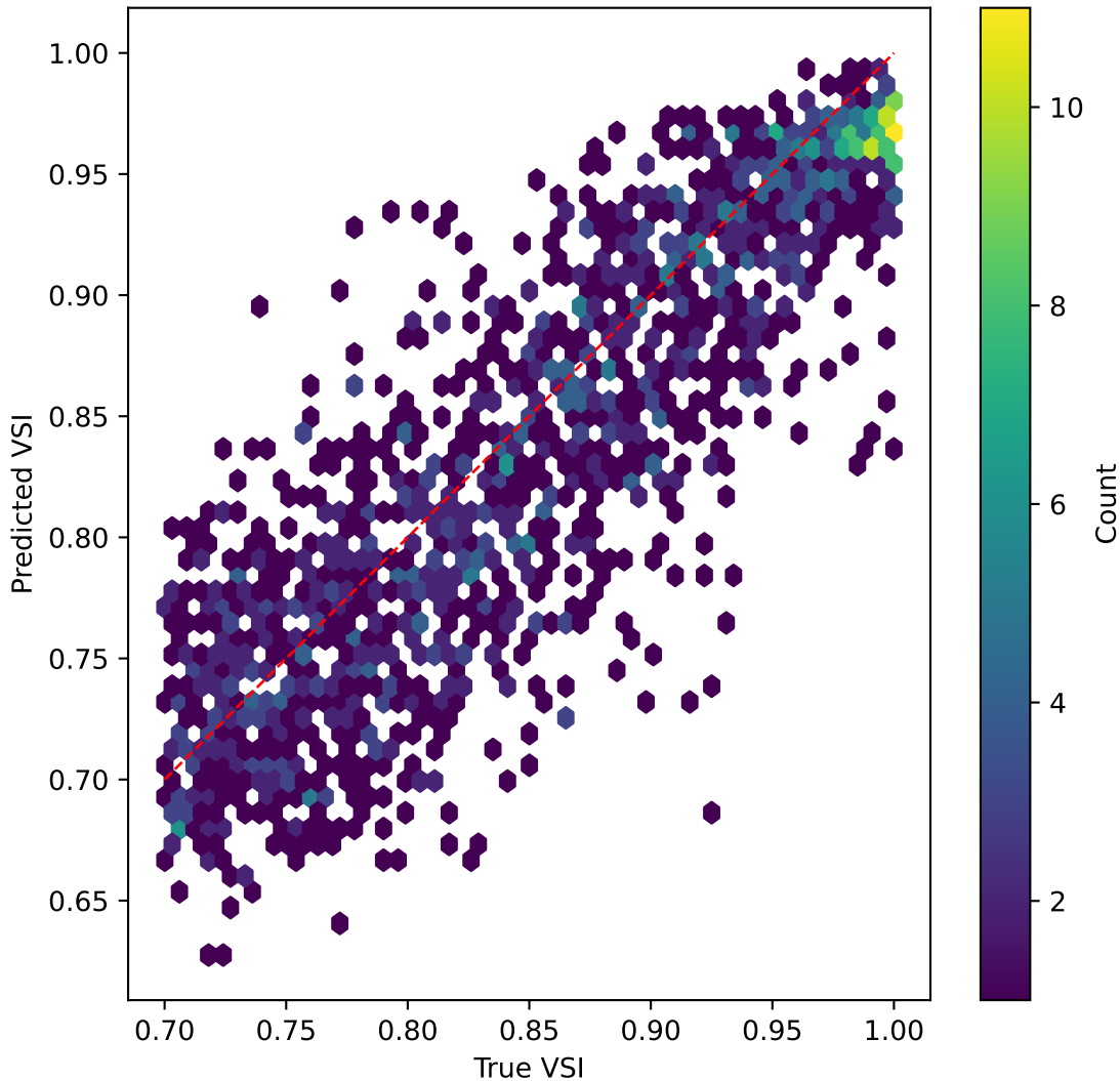
mobilenetv3 on VSI | R^2=0.270
