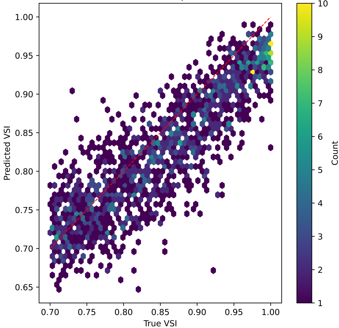
efficientnet on VSI | R^2=0.289
