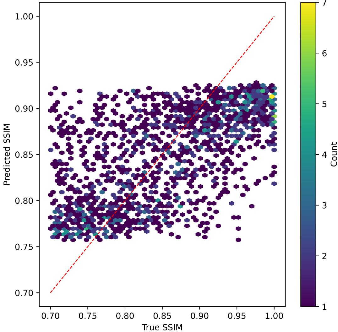
tinyvit on SSIM | R^2=0.316
