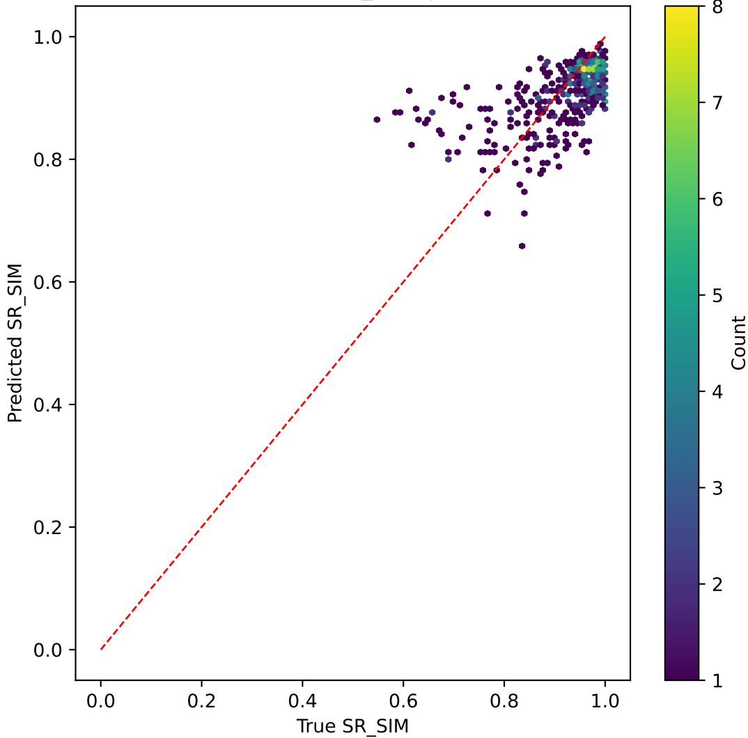
mobilenetv3 on SR_SIM | R^2=0.104
