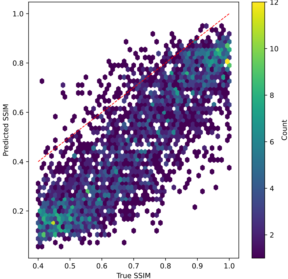
mobilenetv3 on SSIM | R^2=-1.629
