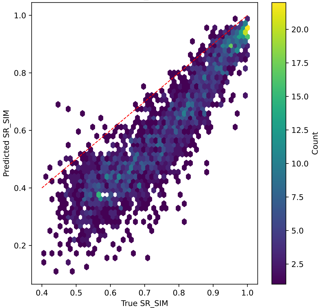
resnet50v2 on SR_SIM | R^2=-1.905
