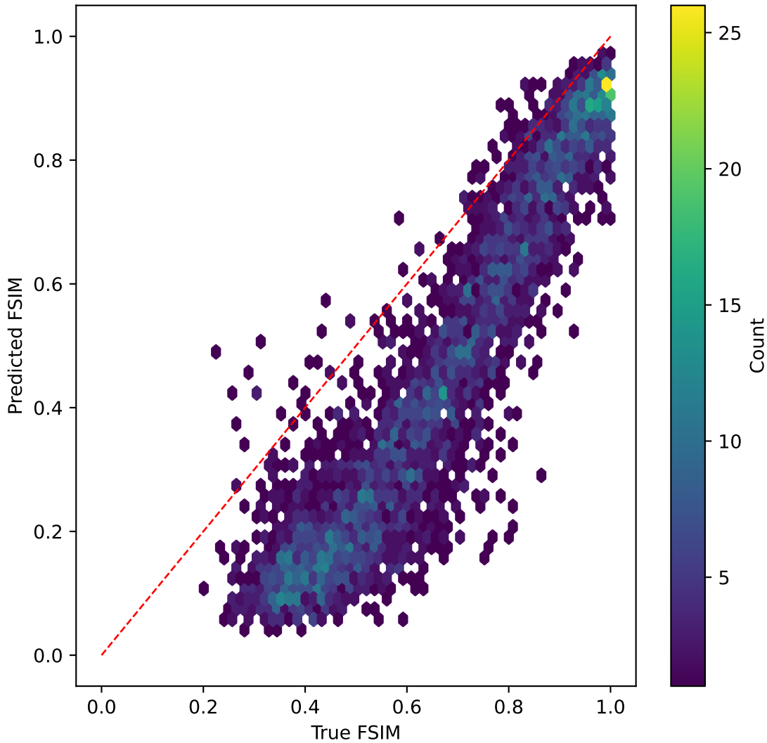
resnet50v2 on FSIM | R^2=-2.125
