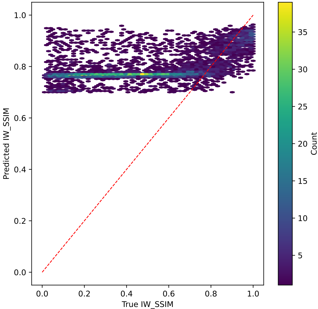
efficientnet on IW_SSIM | R^2=-1.918
