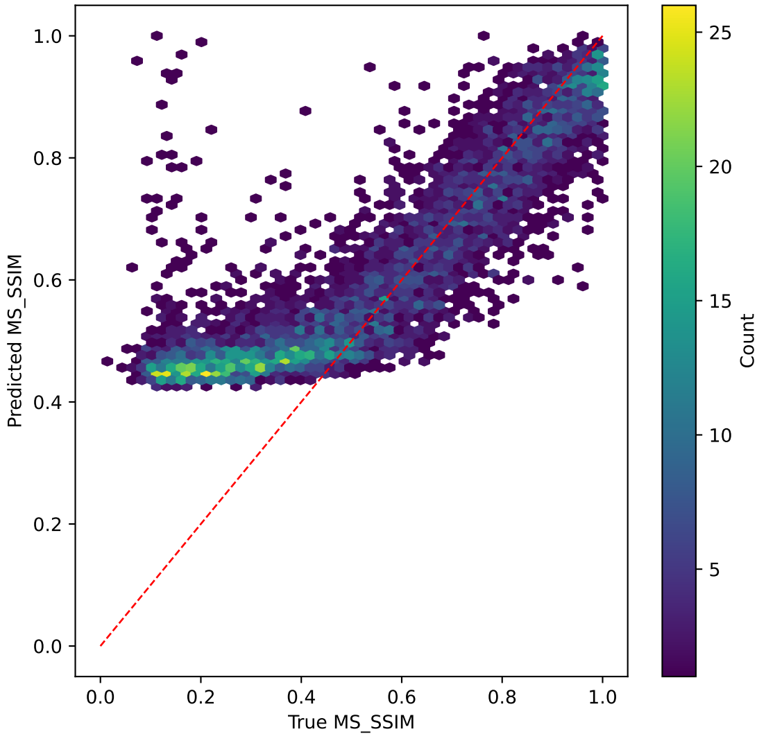
efficientnet on MS_SSIM | R^2=0.601
