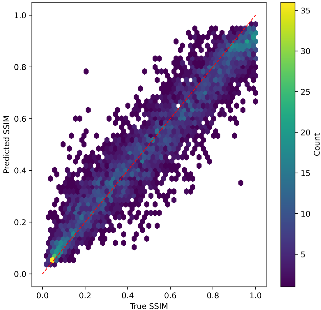
resnet50v2 on SSIM | R^2=0.848
