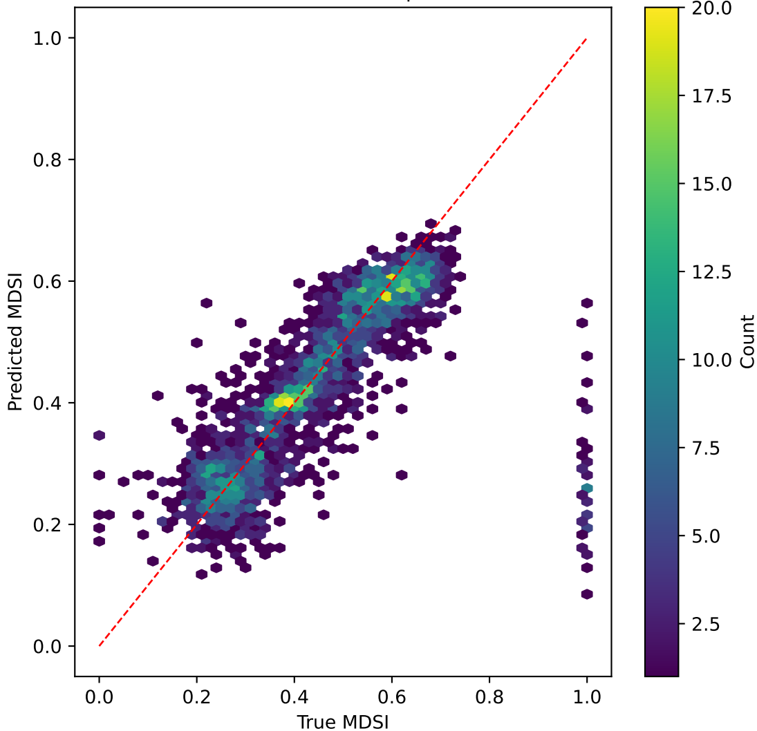
mobilenetv3 on MDSI | R^2=0.109
