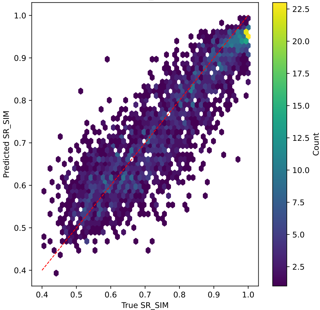
mobilenetv3 on SR_SIM | R^2=0.517
