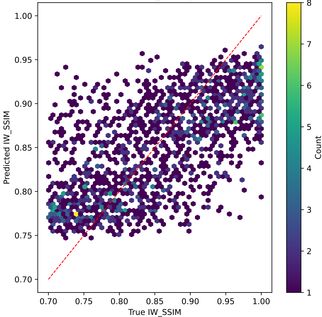
mobilenetv3 on IW_SSIM | R^2=0.433
