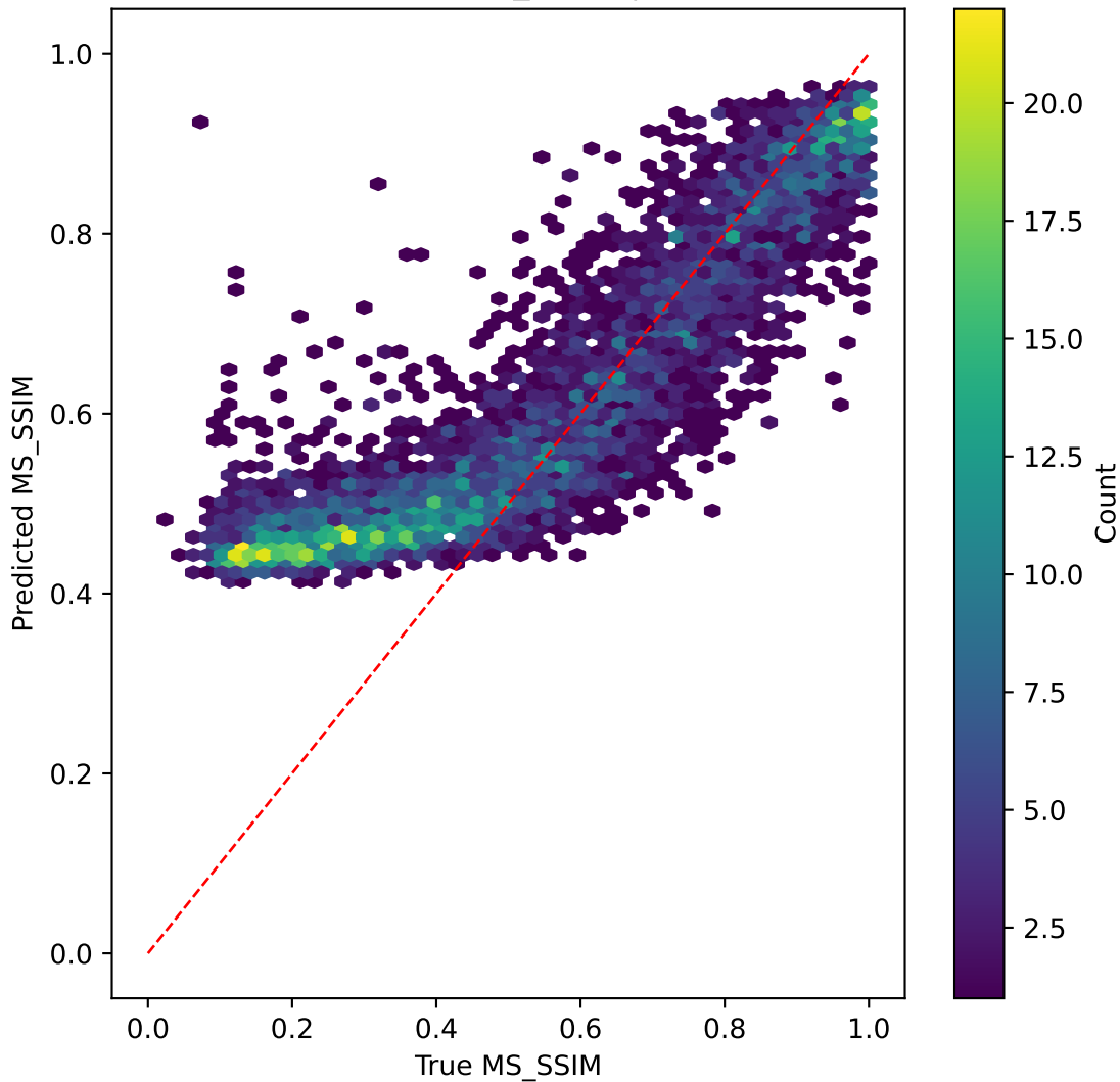
mobilenetv3 on MS_SSIM | R^2=0.614
