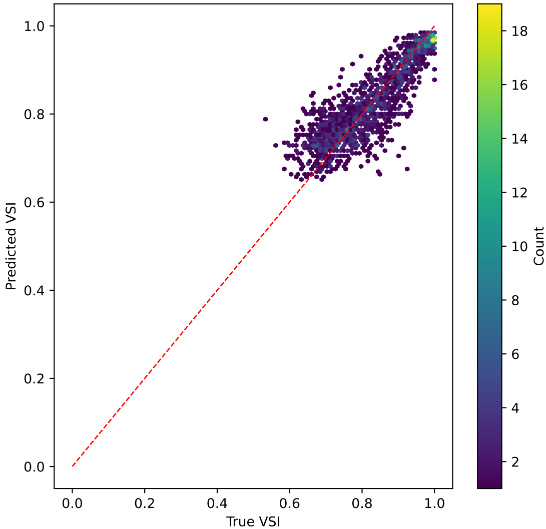
mobilevitv2 on VSI | R^2=0.528
