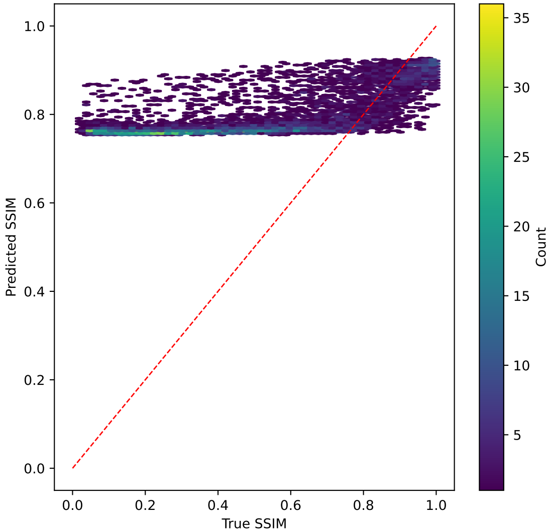
tinyvit on SSIM | R^2=-2.099
