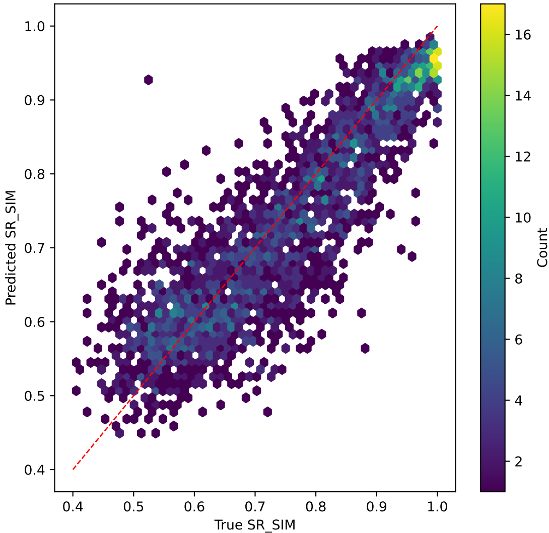
efficientnet on SR_SIM | R^2=0.562
