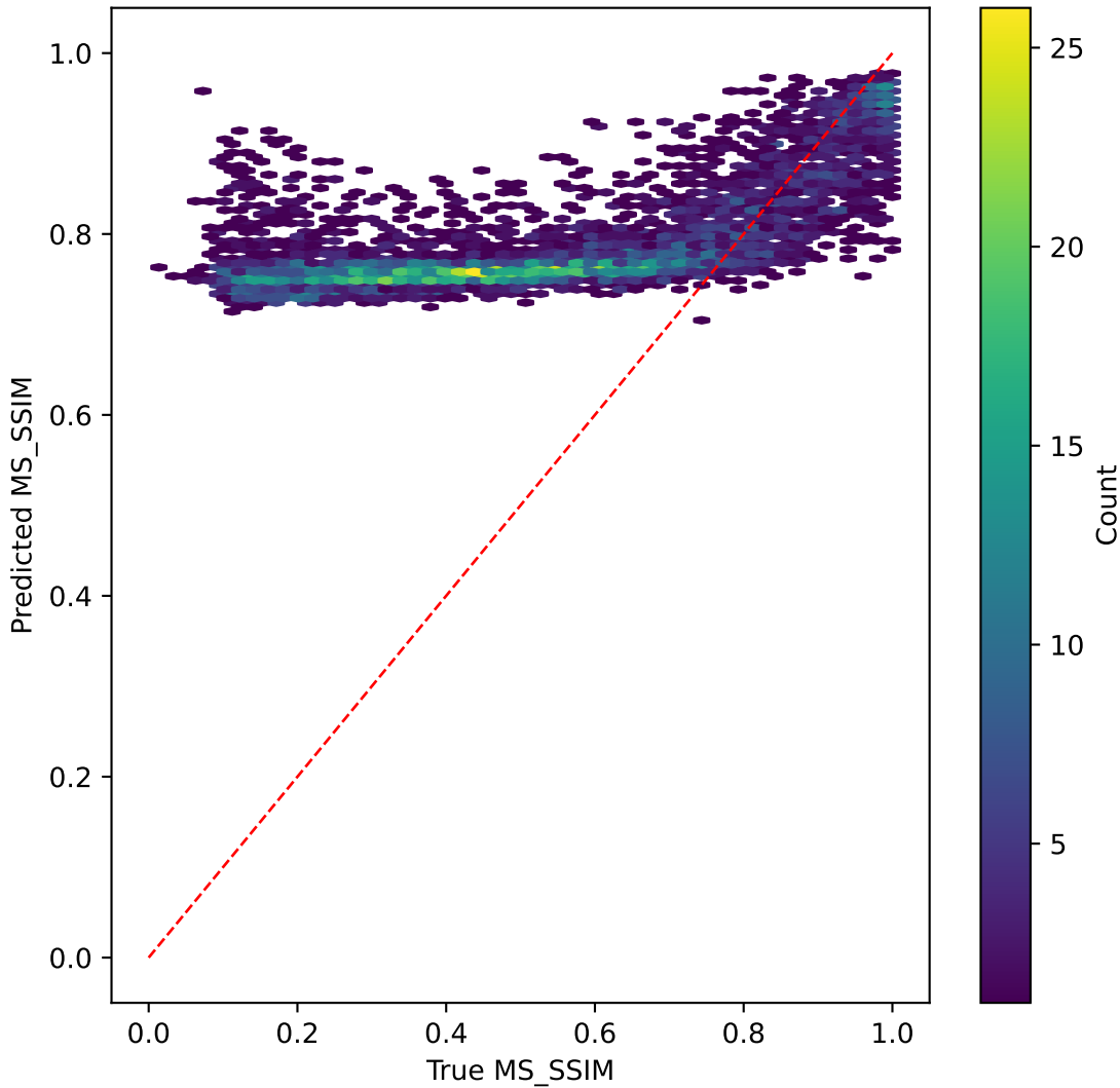
efficientnet on MS_SSIM | R^2=-1.071
