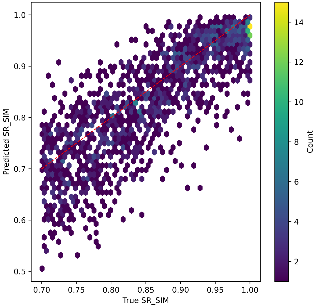
resnet50v2 on SR_SIM | R^2=0.242
