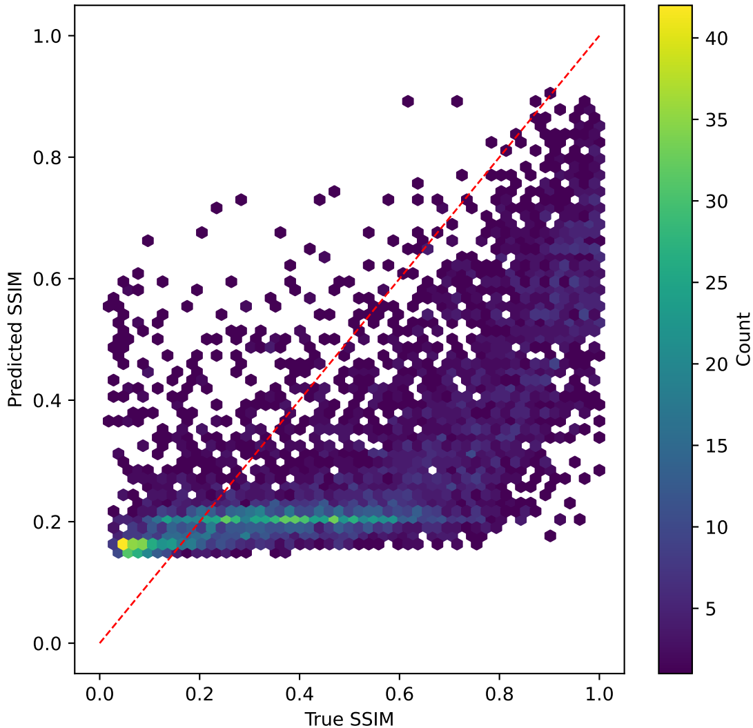
mobilevitv2 on SSIM | R^2=-0.027
