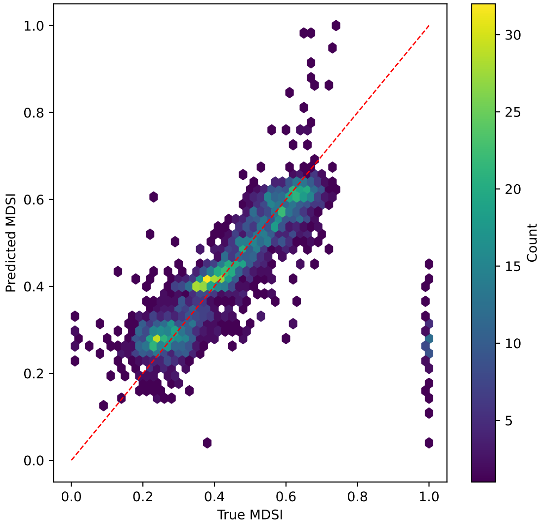
efficientnet on MDSI | R^2=0.214
