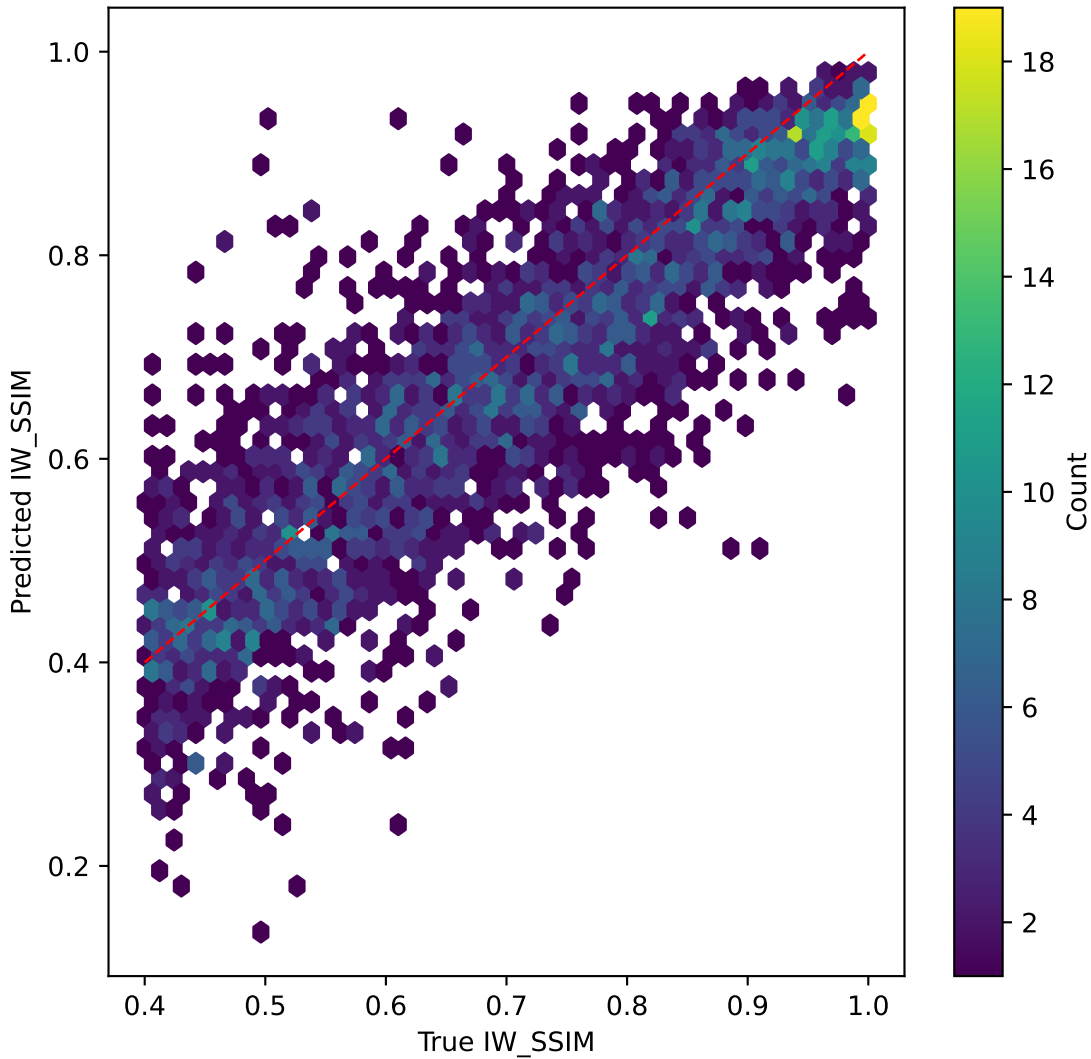
mobilevitv2 on IW_SSIM | R^2=0.772
