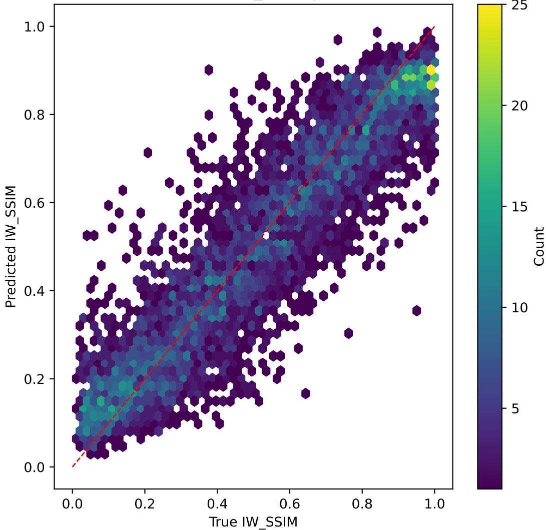
mobilenetv3 on IW_SSIM | R^2=0.812
