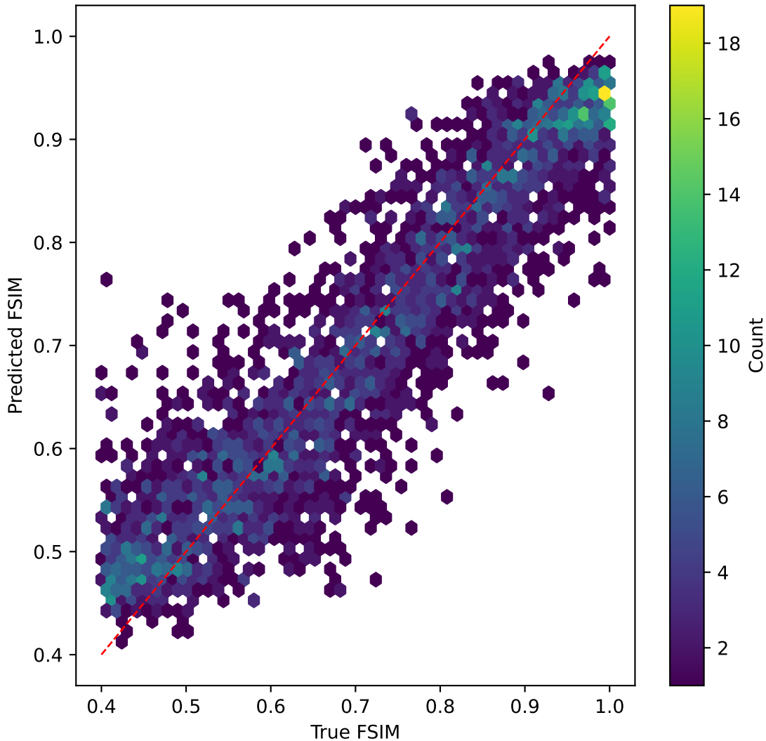
efficientnet on FSIM | R^2=0.754
