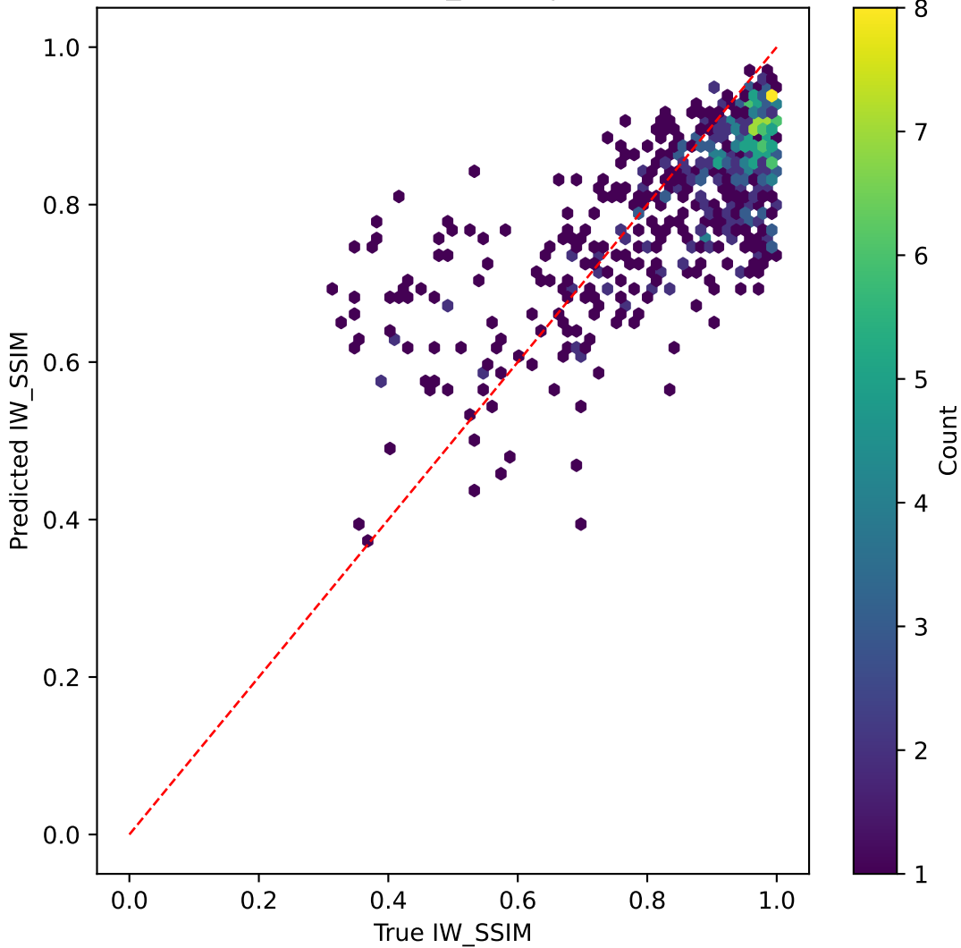
efficientnet on IW_SSIM | R^2=0.308
