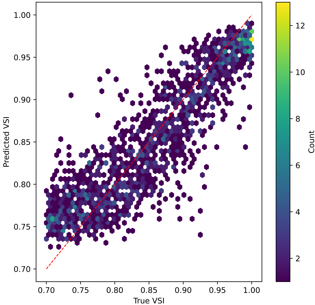
mobilenetv3 on VSI | R^2=0.602
