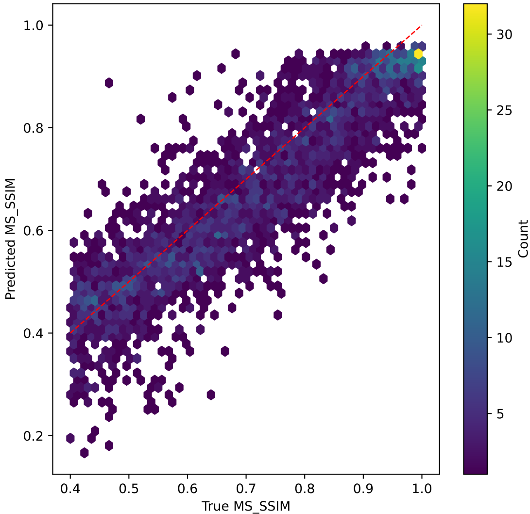
tinyvit on MS_SSIM | R^2=0.744
