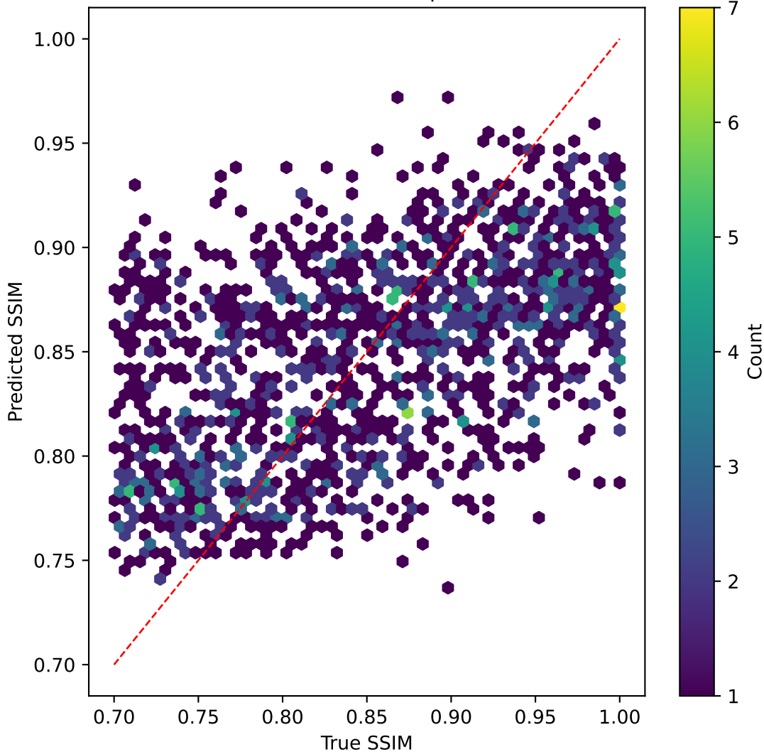
mobilenetv3 on SSIM | R^2=0.260
