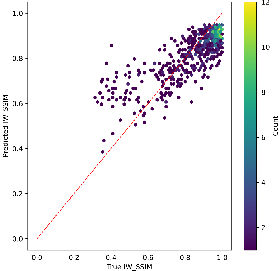
tinyvit on IW_SSIM | R^2=0.576
