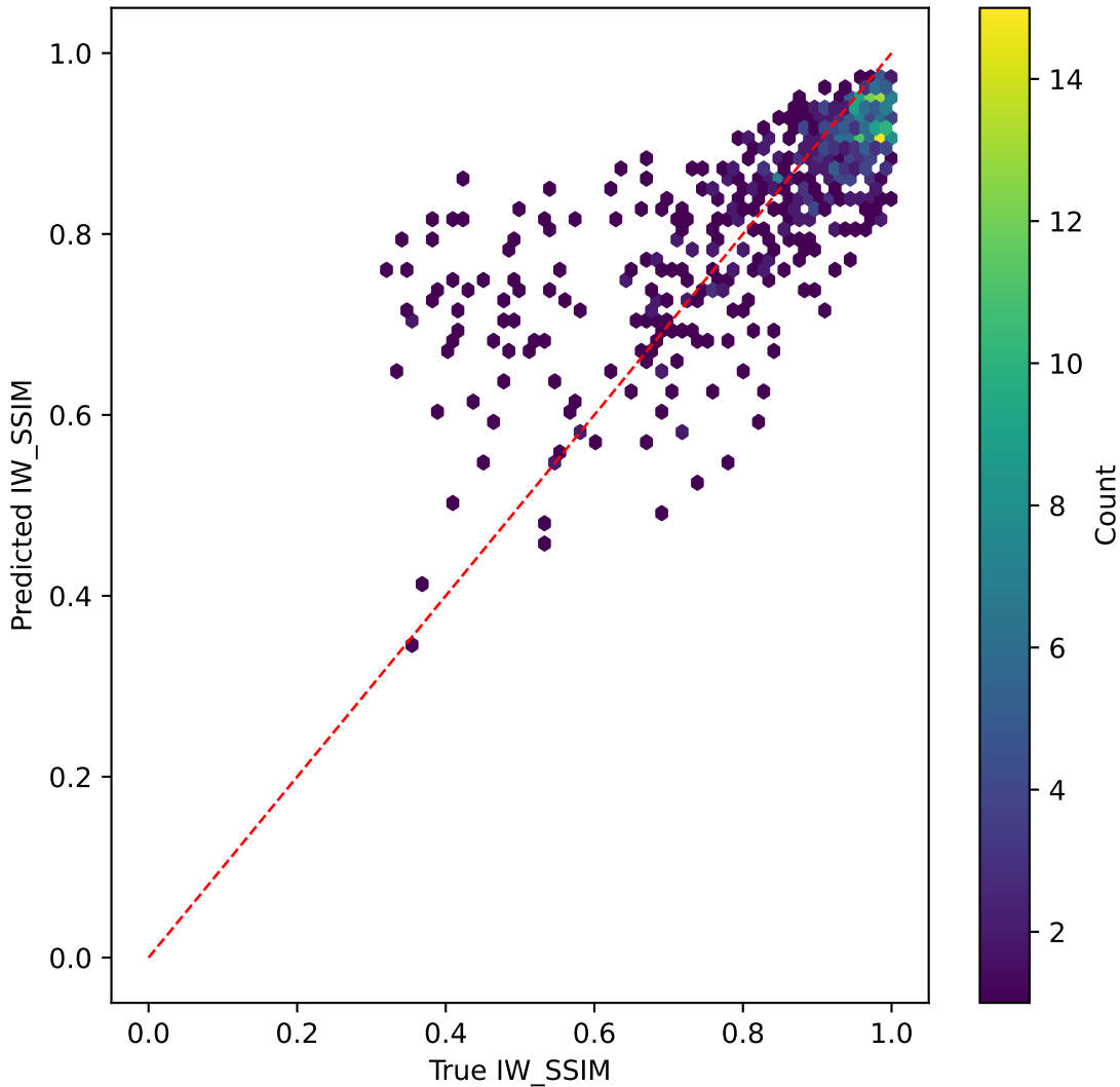
mobilevitv2 on IW_SSIM | R^2=0.578
