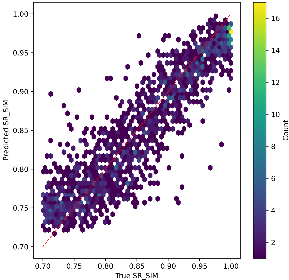
resnet50v2 on SR_SIM | R^2=0.802
