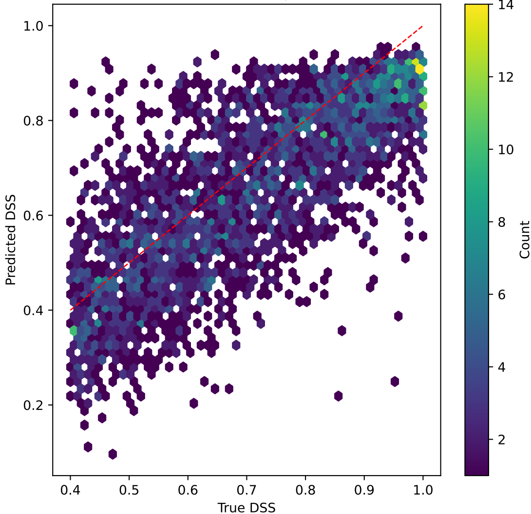
mobilevitv2 on DSS | R^2=0.483
