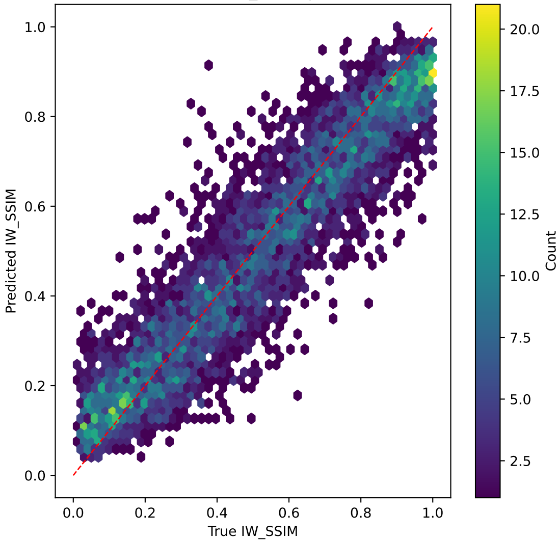
efficientnet on IW_SSIM | R^2=0.836
