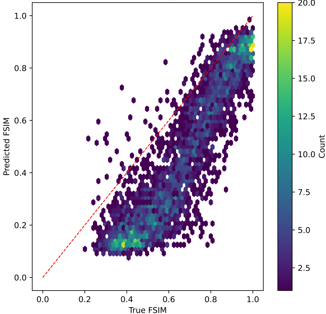
mobilenetv3 on FSIM | R^2=-2.237
