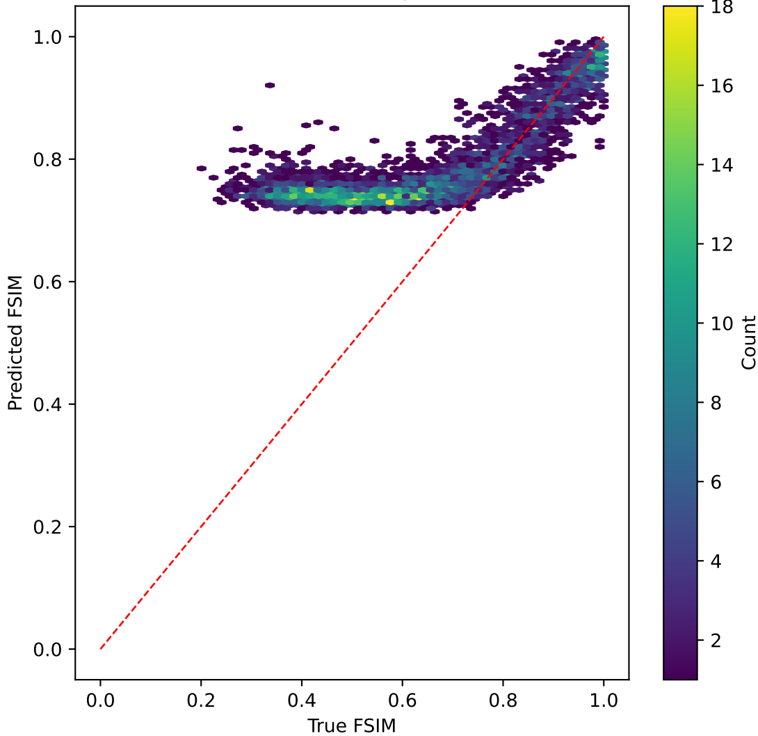
resnet50v2 on FSIM | R^2=-0.092
