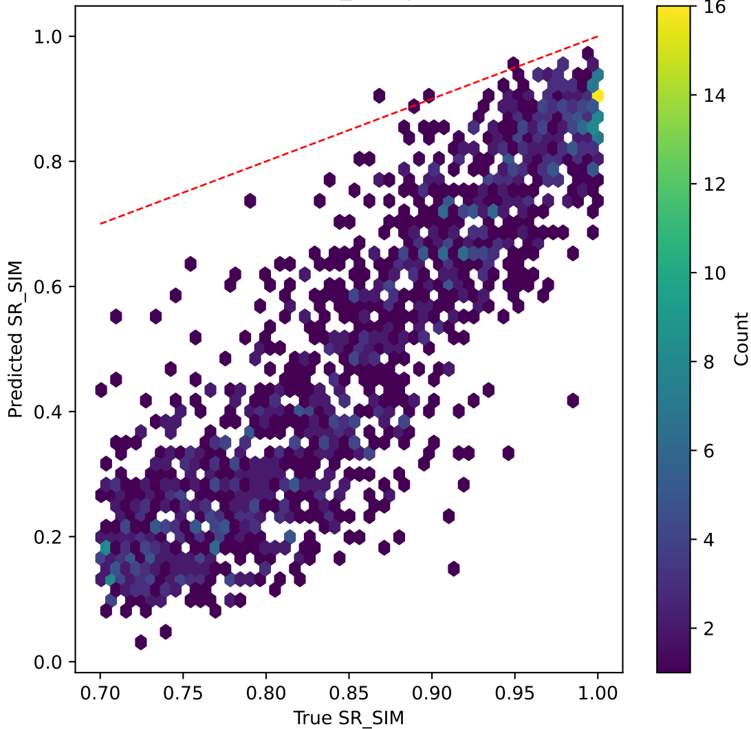
efficientnet on SR_SIM | R^2=-27.850
