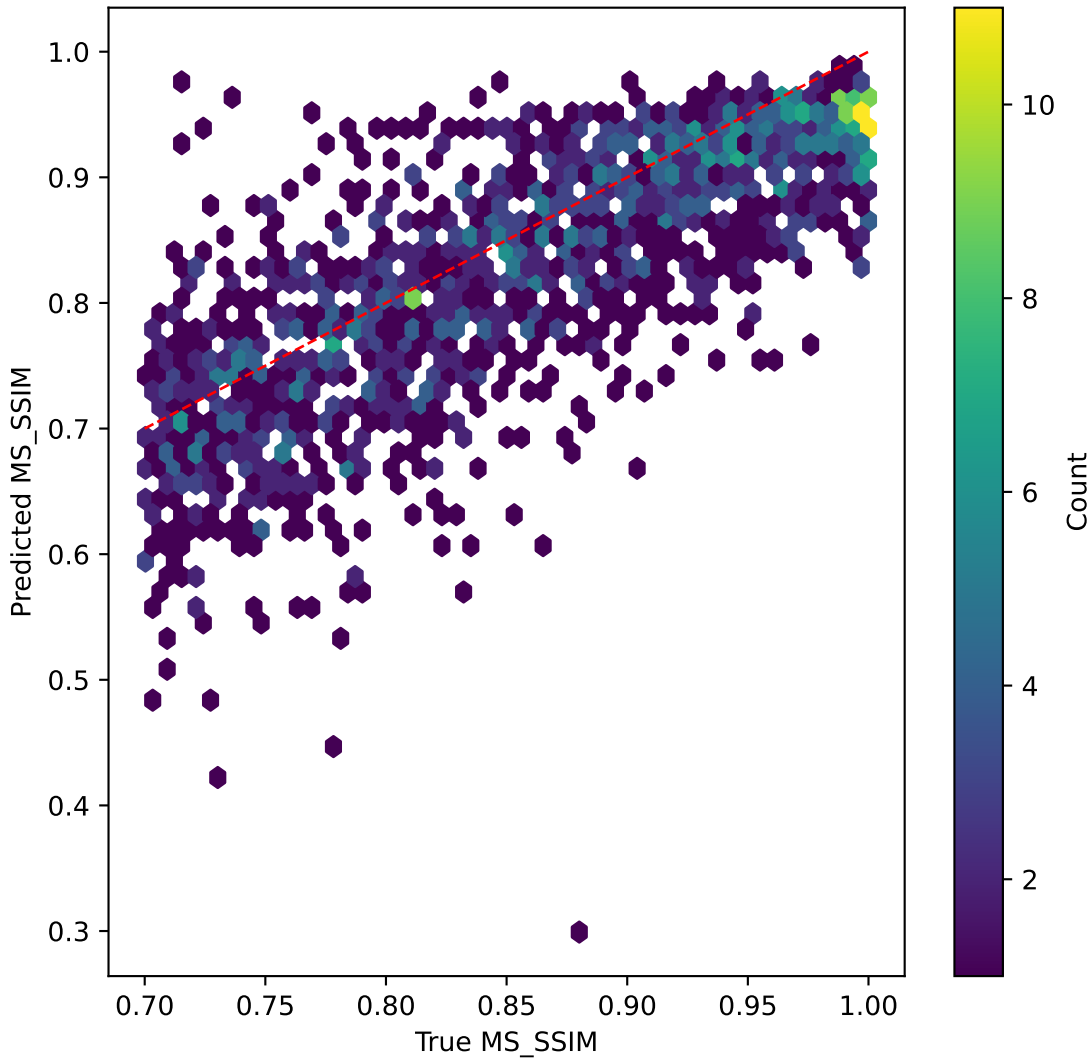
mobilevitv2 on MS_SSIM | R^2=0.295
