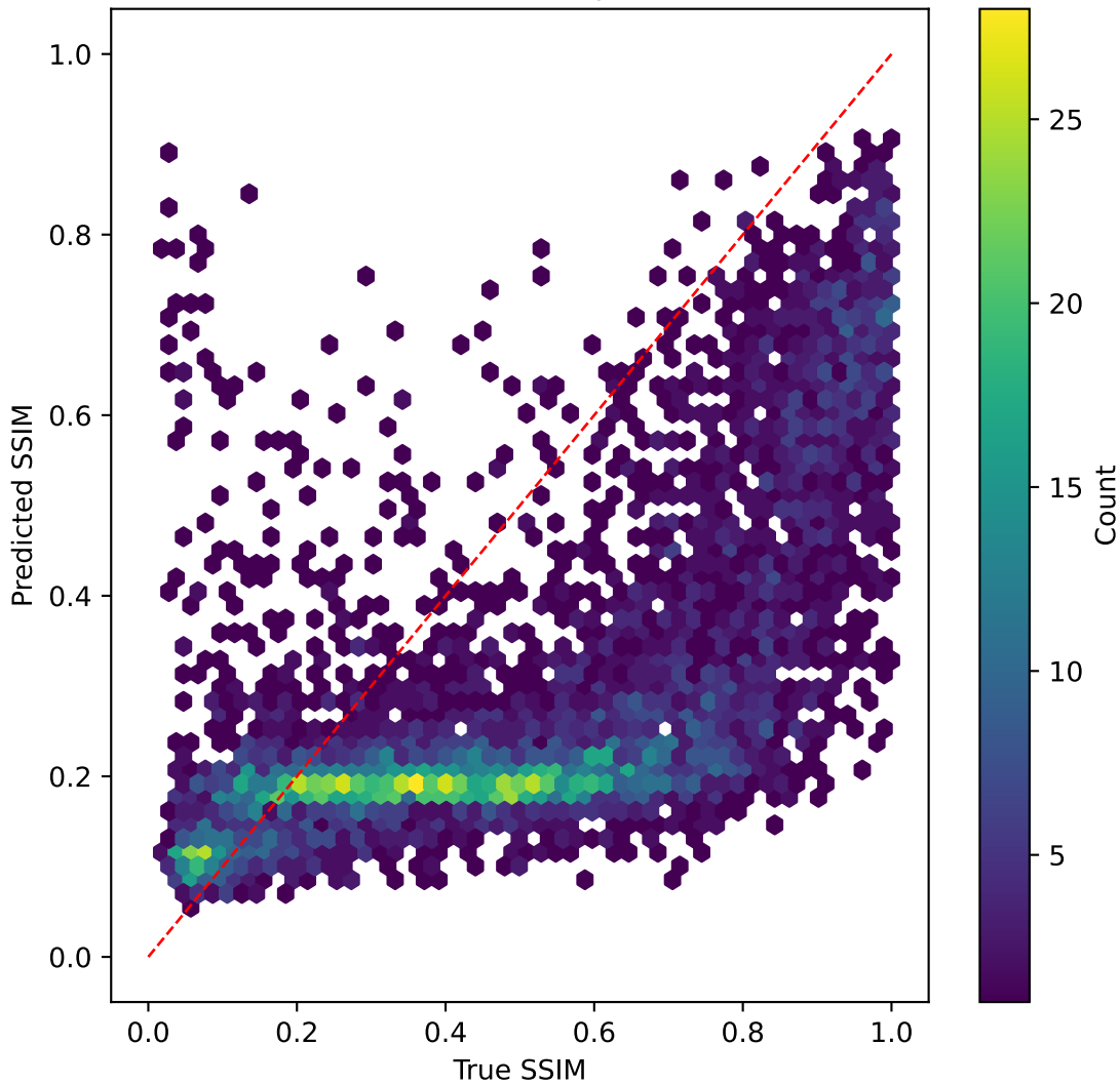
resnet50v2 on SSIM | R^2=-0.192
