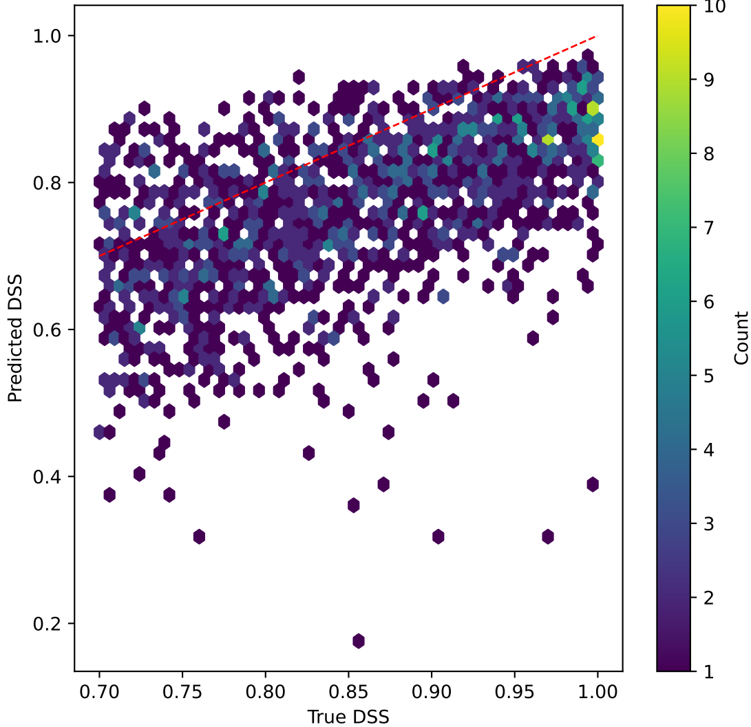
resnet50v2 on DSS | R^2=-1.023
