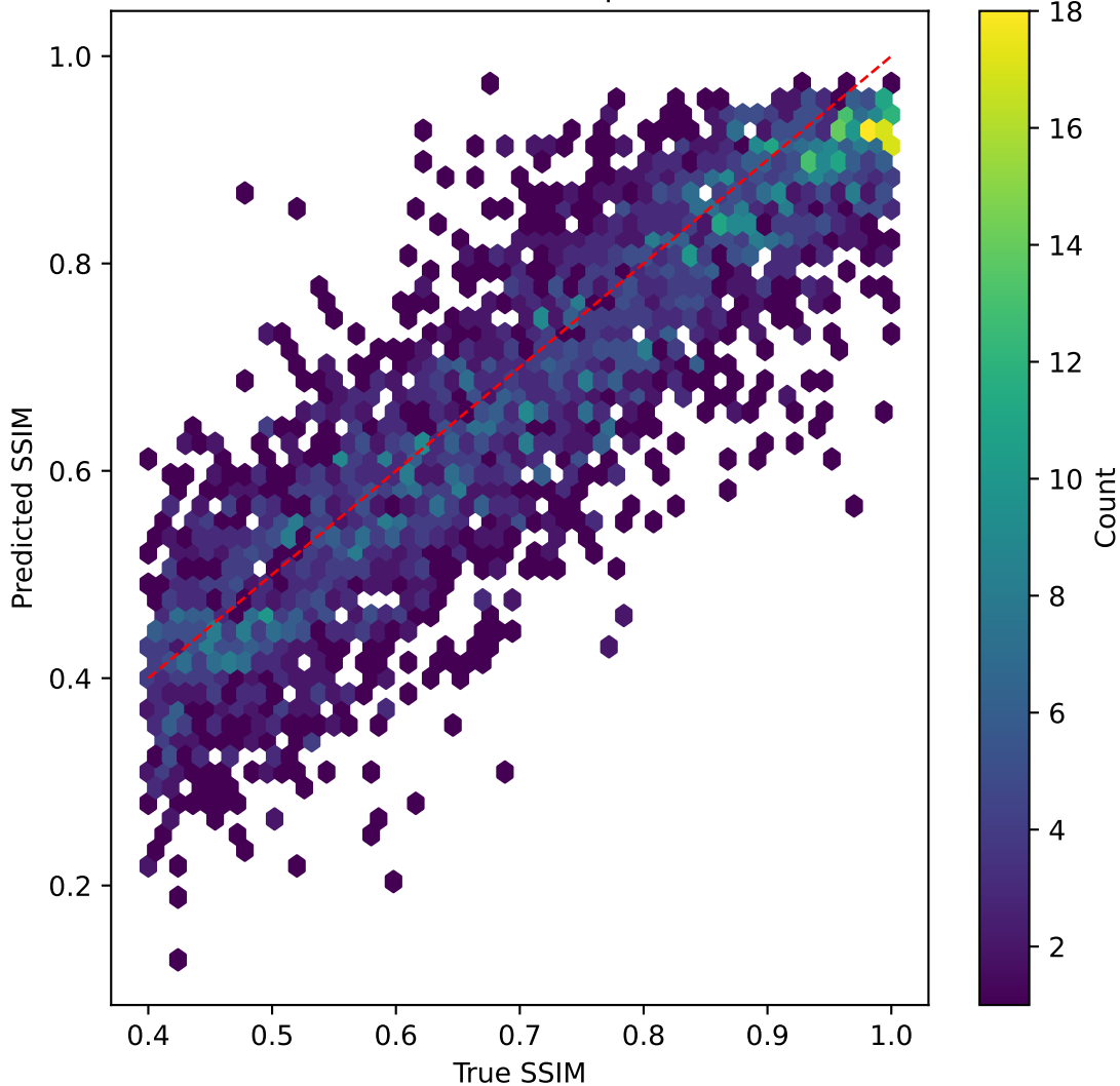
mobilevitv2 on SSIM | R^2=0.693
