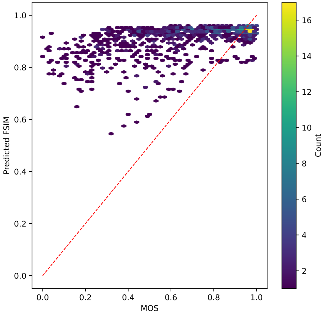
tinyvit on FSIM AGAINST MOS | R^2=-0.773
