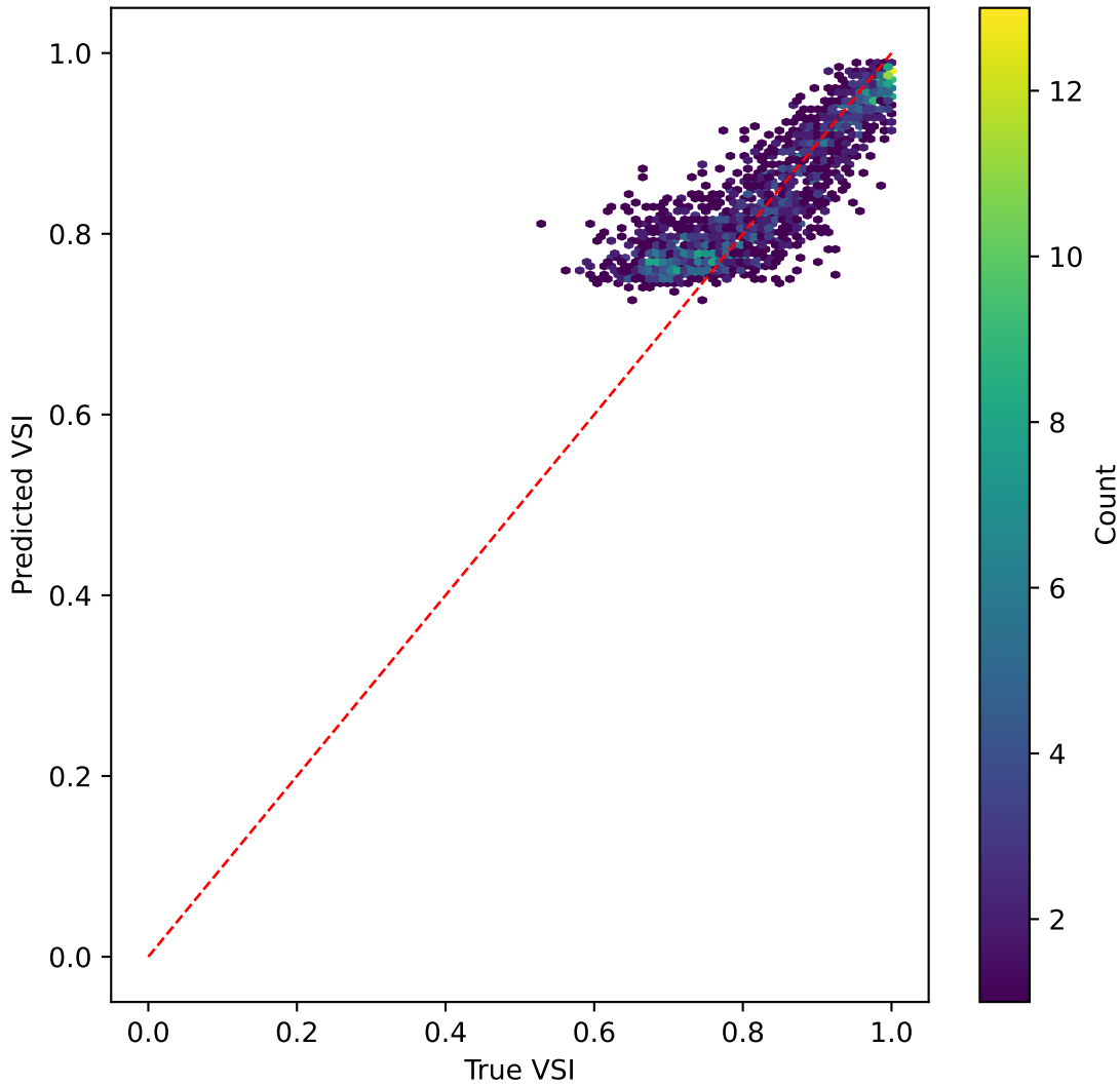
efficientnet on VSI | R^2=0.629
