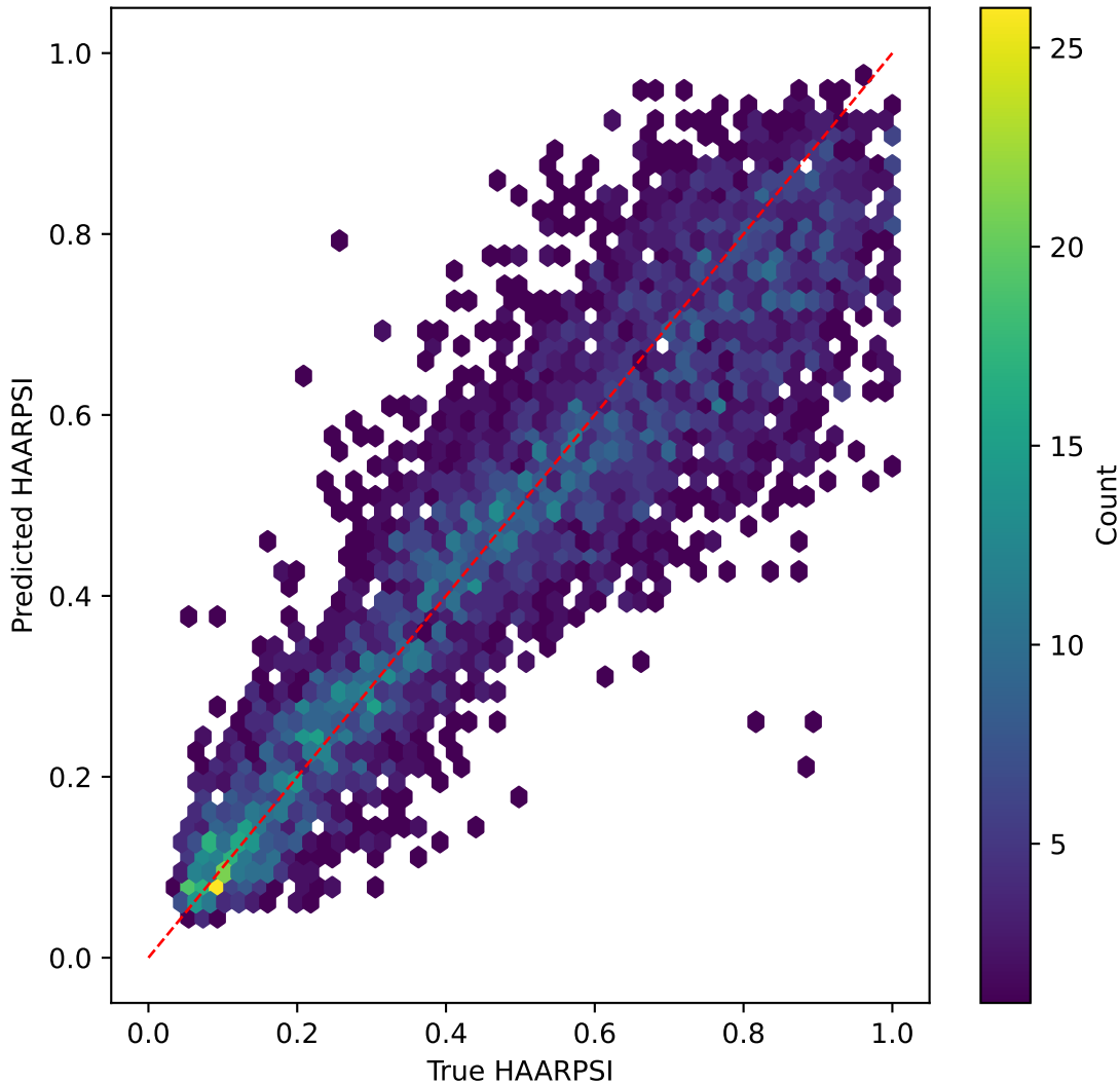
resnet50v2 on HAARPSI | R^2=0.751
