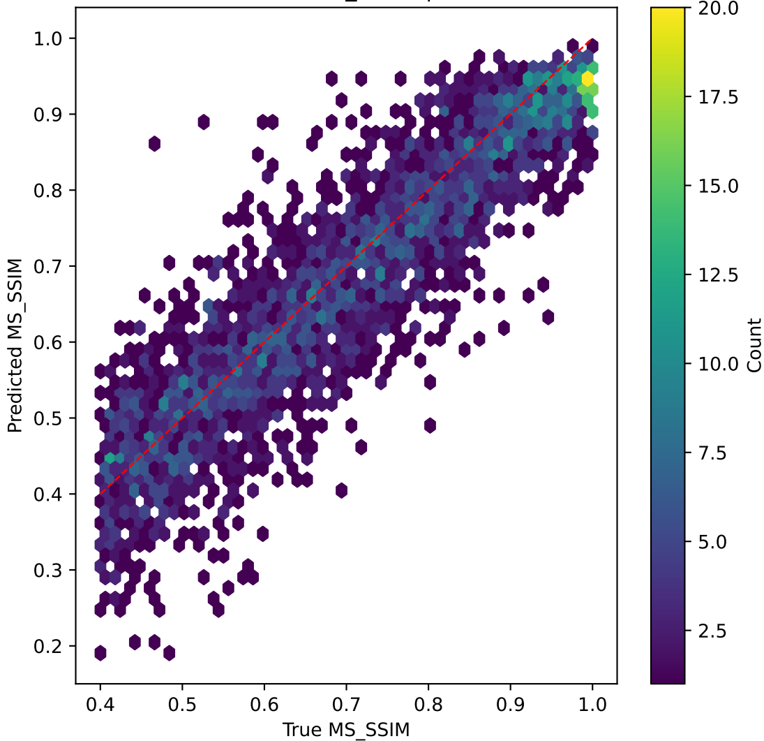
mobilevitv2 on MS_SSIM | R^2=0.776
