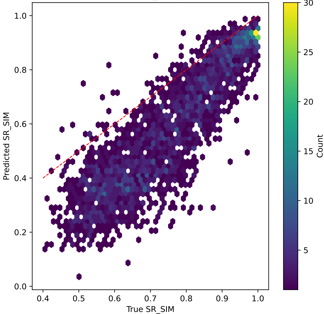
mobilenetv3 on SR_SIM | R^2=-2.761
