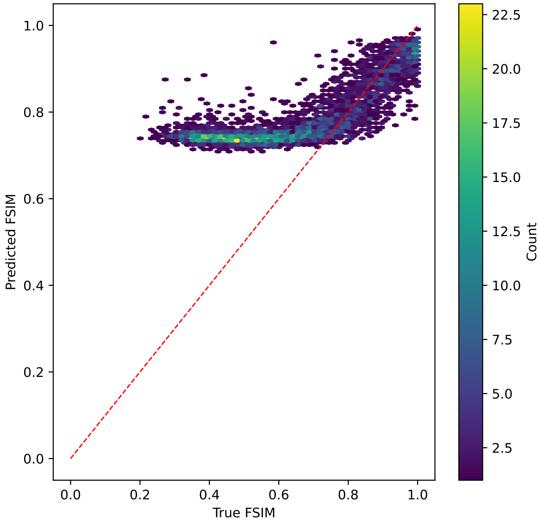
mobilenetv3 on FSIM | R^2=-0.109
