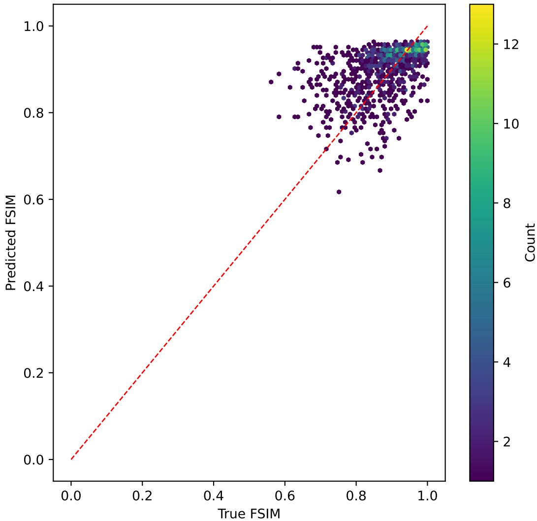
tinyvit on FSIM | R^2=0.198
