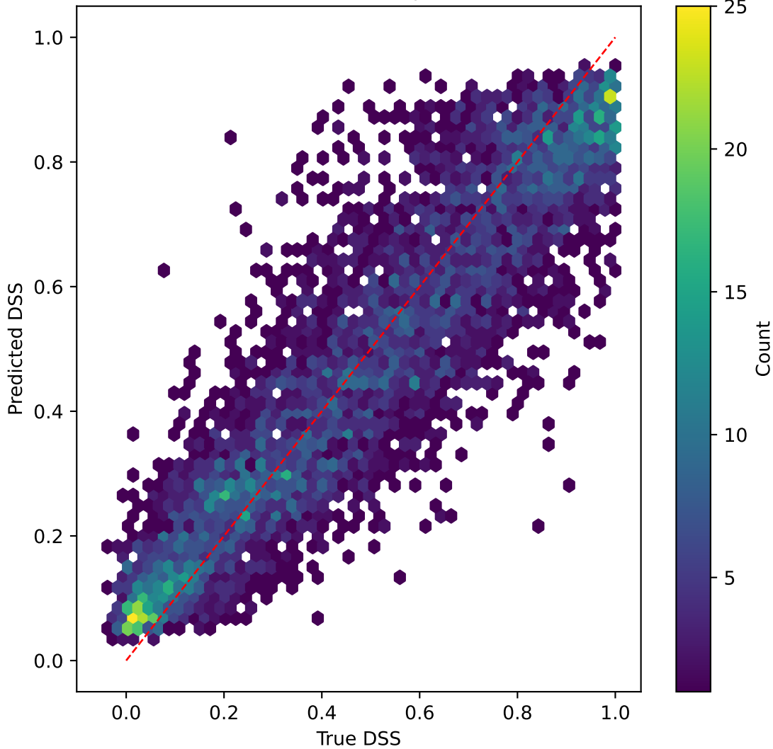
mobilevitv2 on DSS | R^2=0.796
