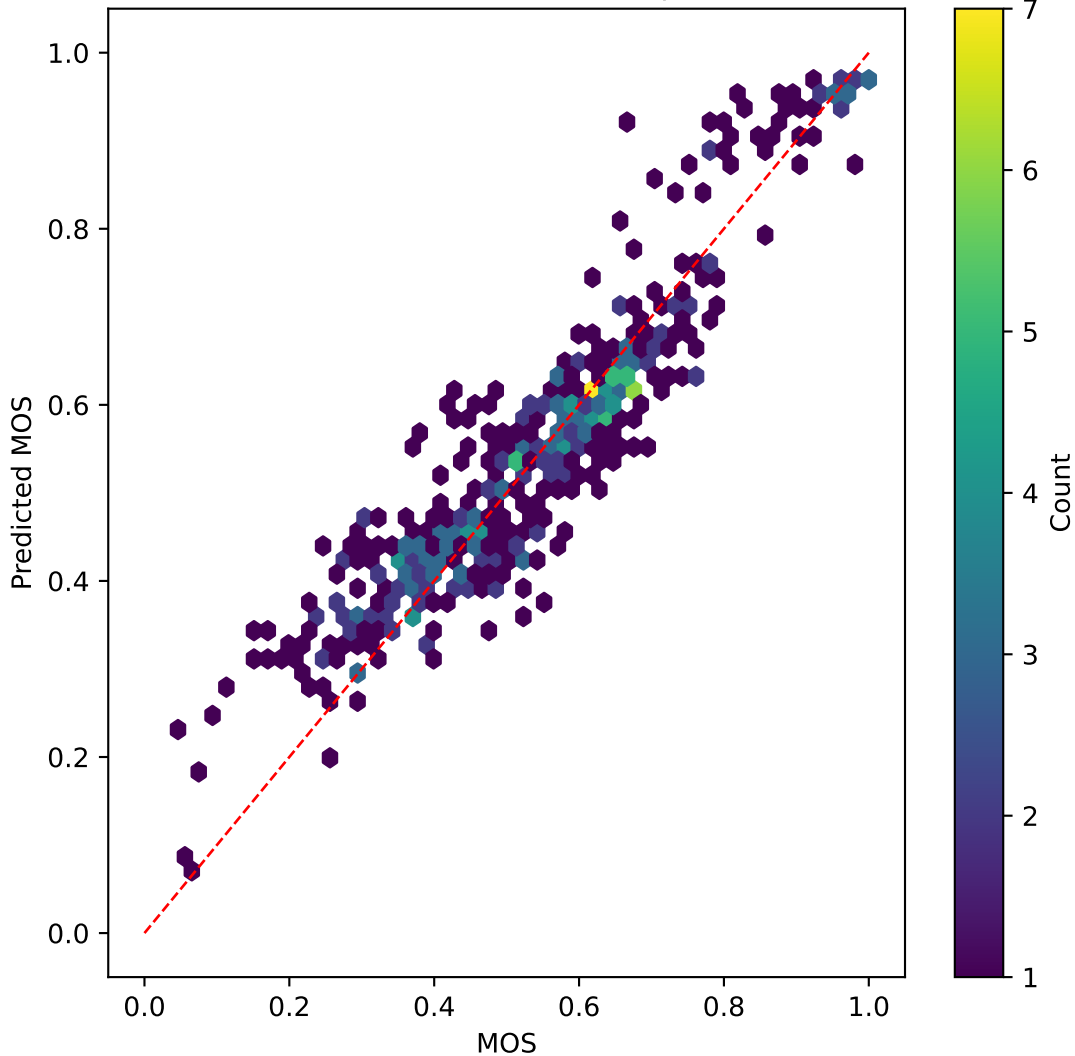
tinyvit on MOS AGAINST MOS | R^2=0.859
