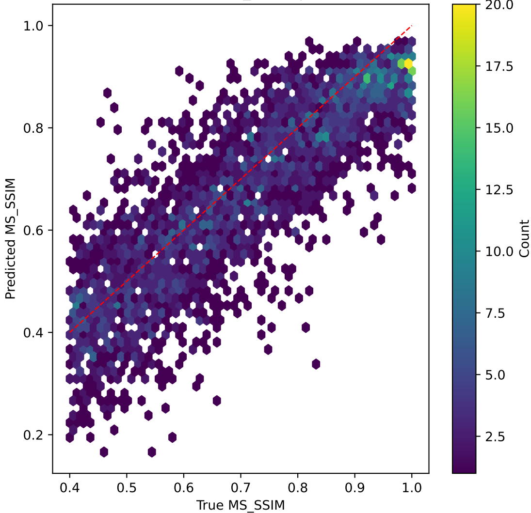
mobilenetv3 on MS_SSIM | R^2=0.619
