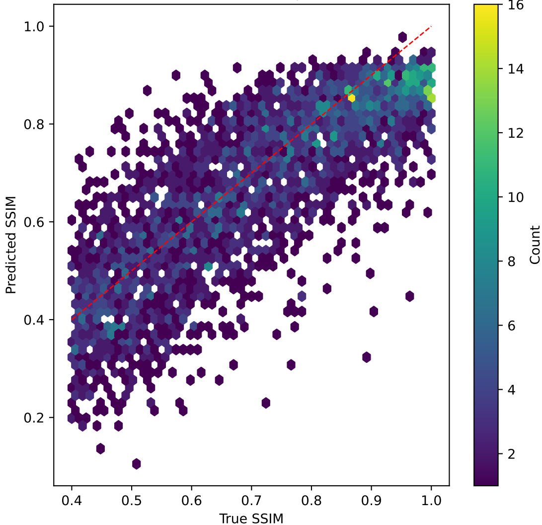
mobilenetv3 on SSIM | R^2=0.511
