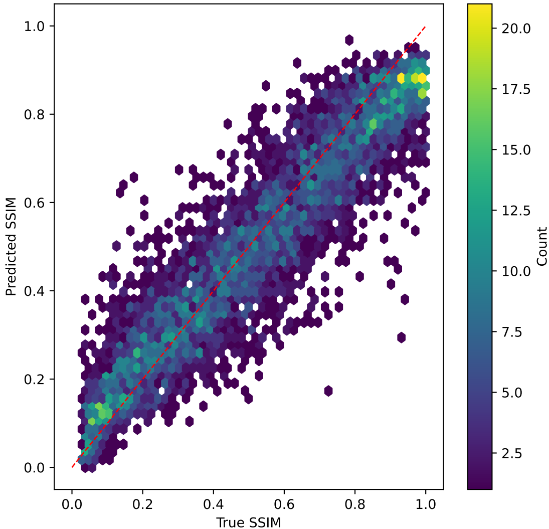
efficientnet on SSIM | R^2=0.795
