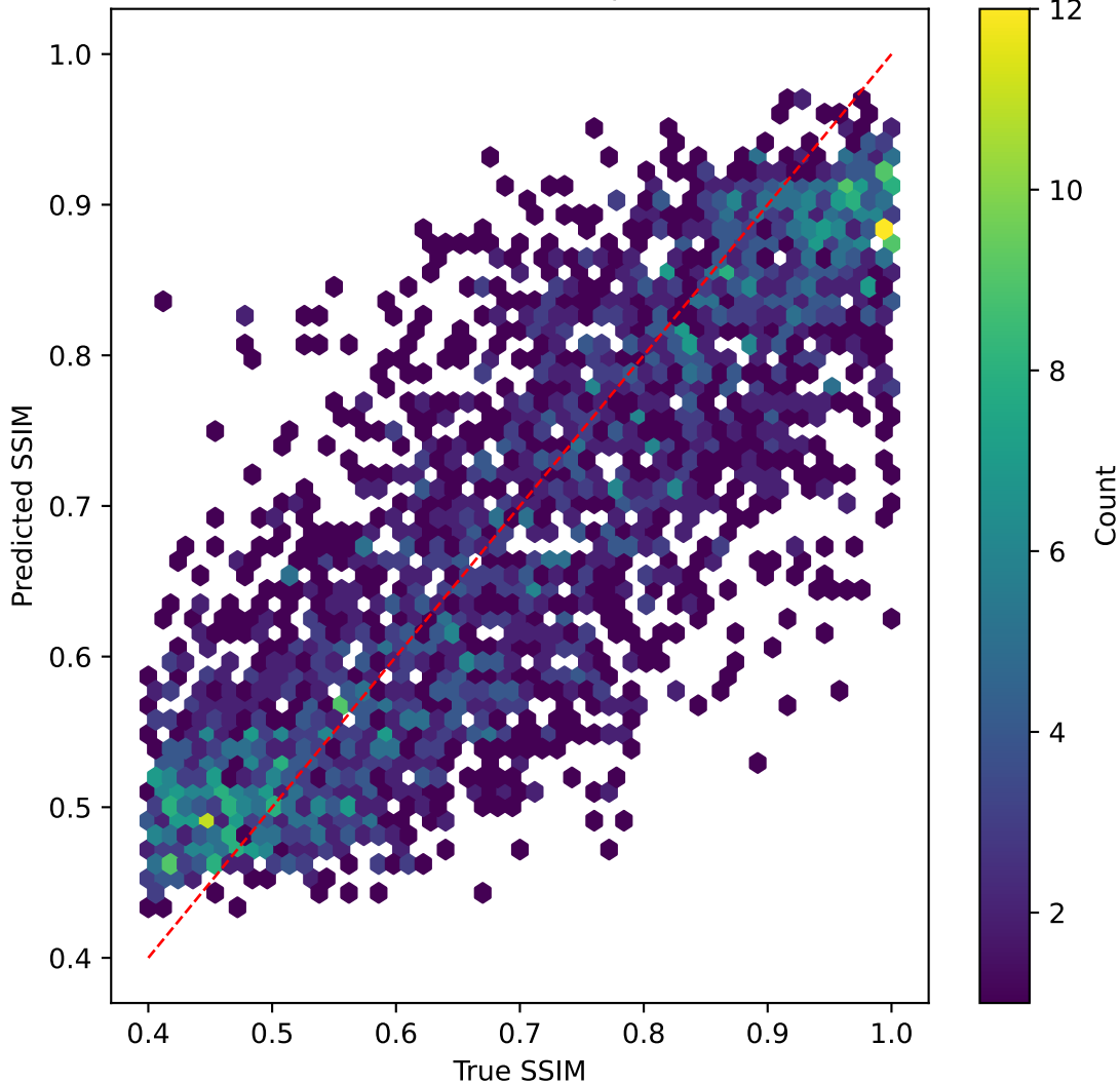
mobilenetv3 on SSIM | R^2=0.661
