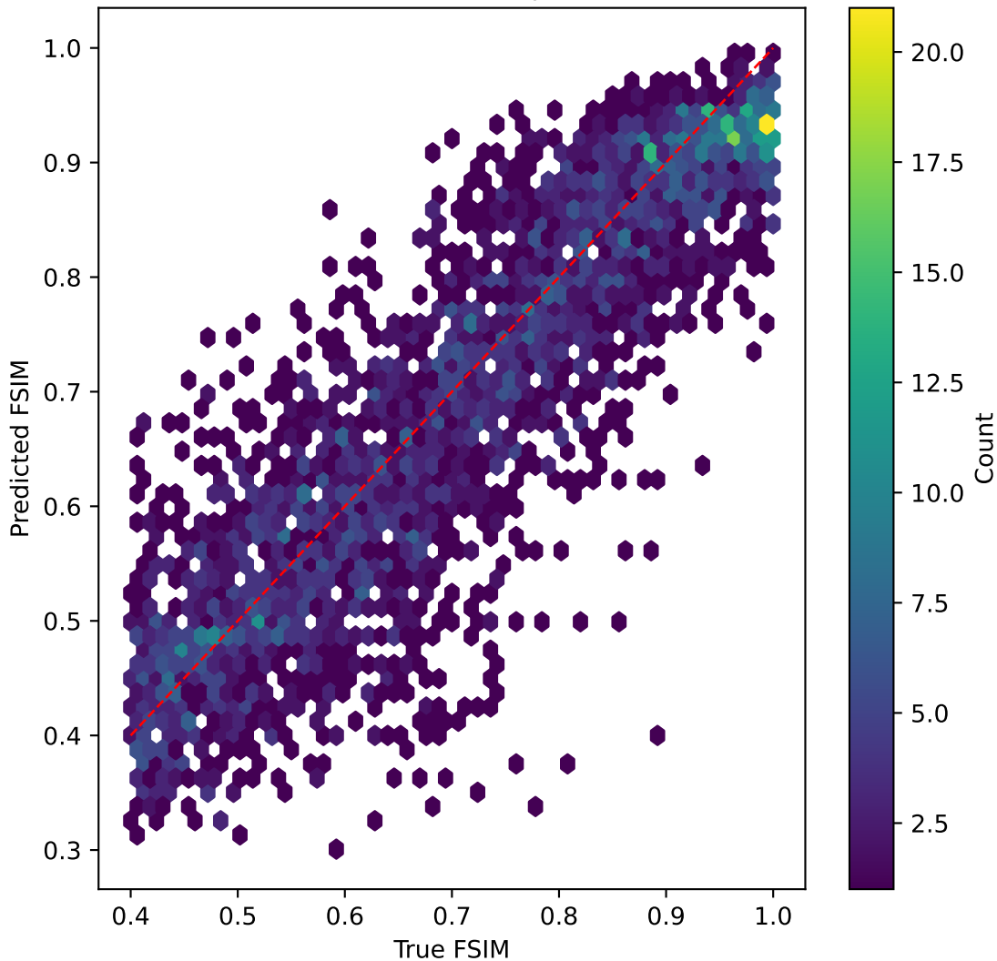
mobilenetv3 on FSIM | R^2=0.556
