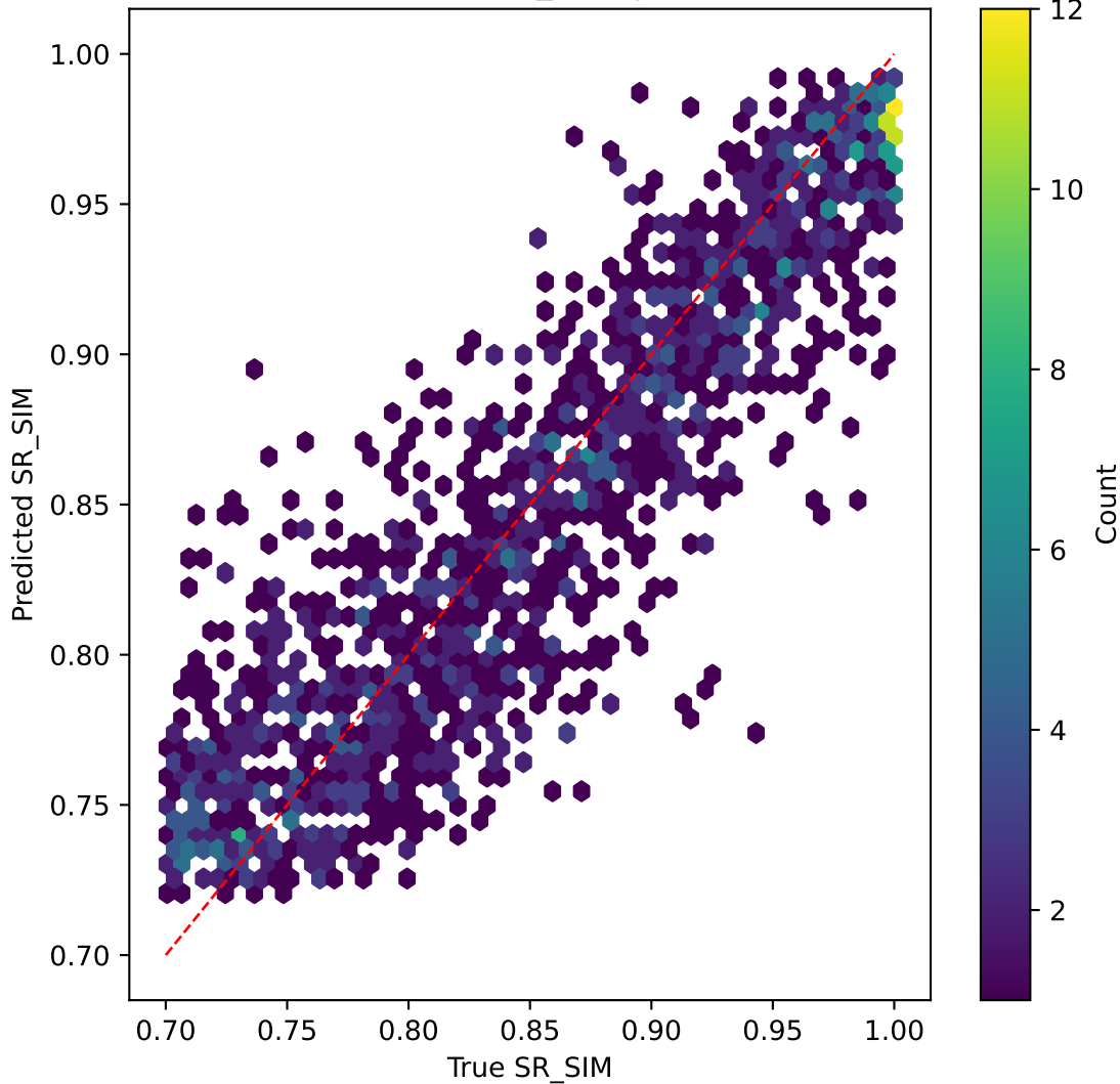
mobilevitv2 on SR_SIM | R^2=0.788
