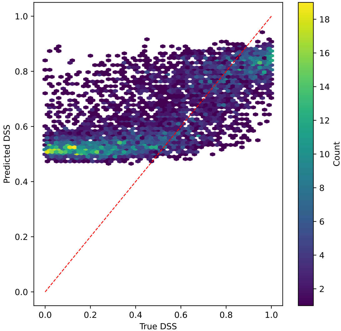
mobilenetv3 on DSS | R^2=-1.227
