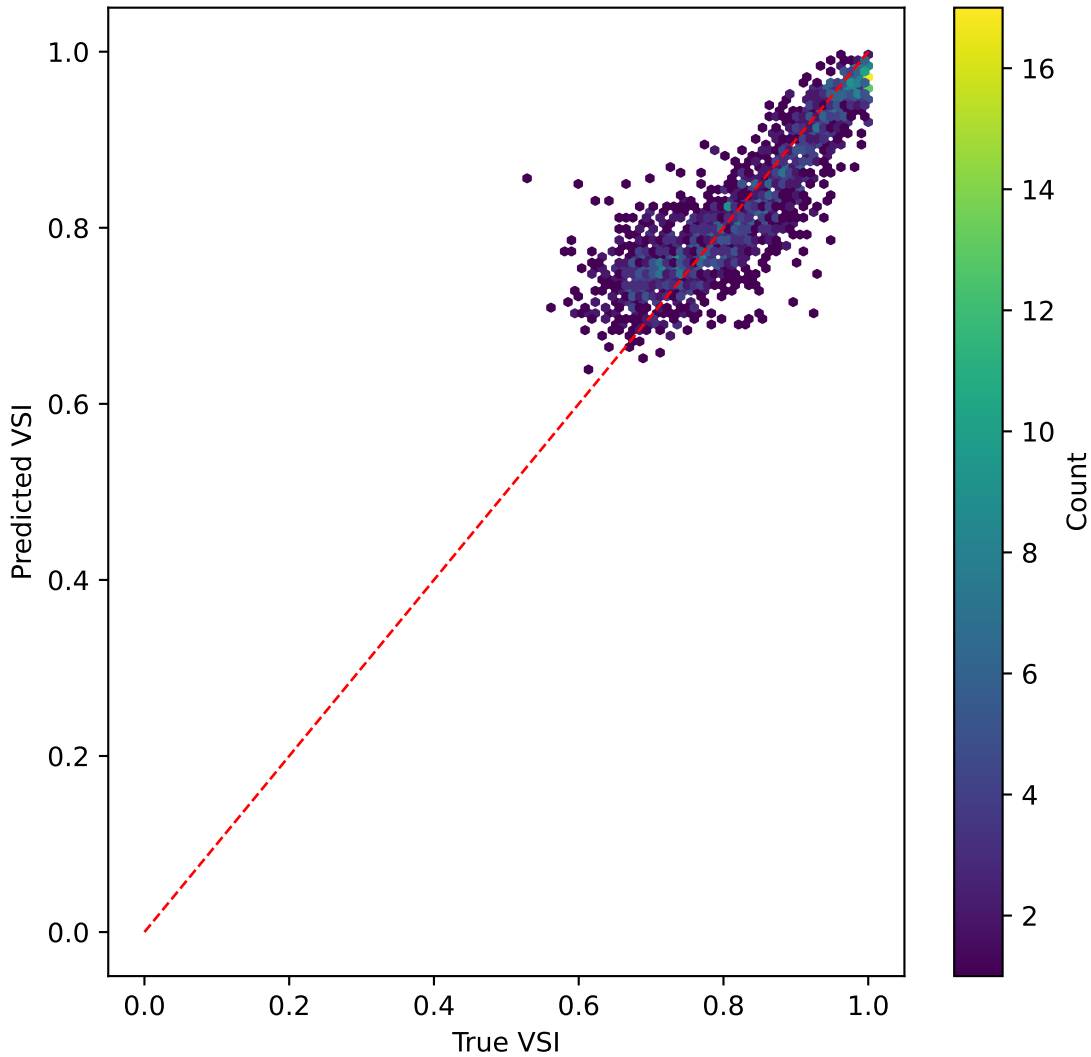
resnet50v2 on VSI | R^2=0.587
