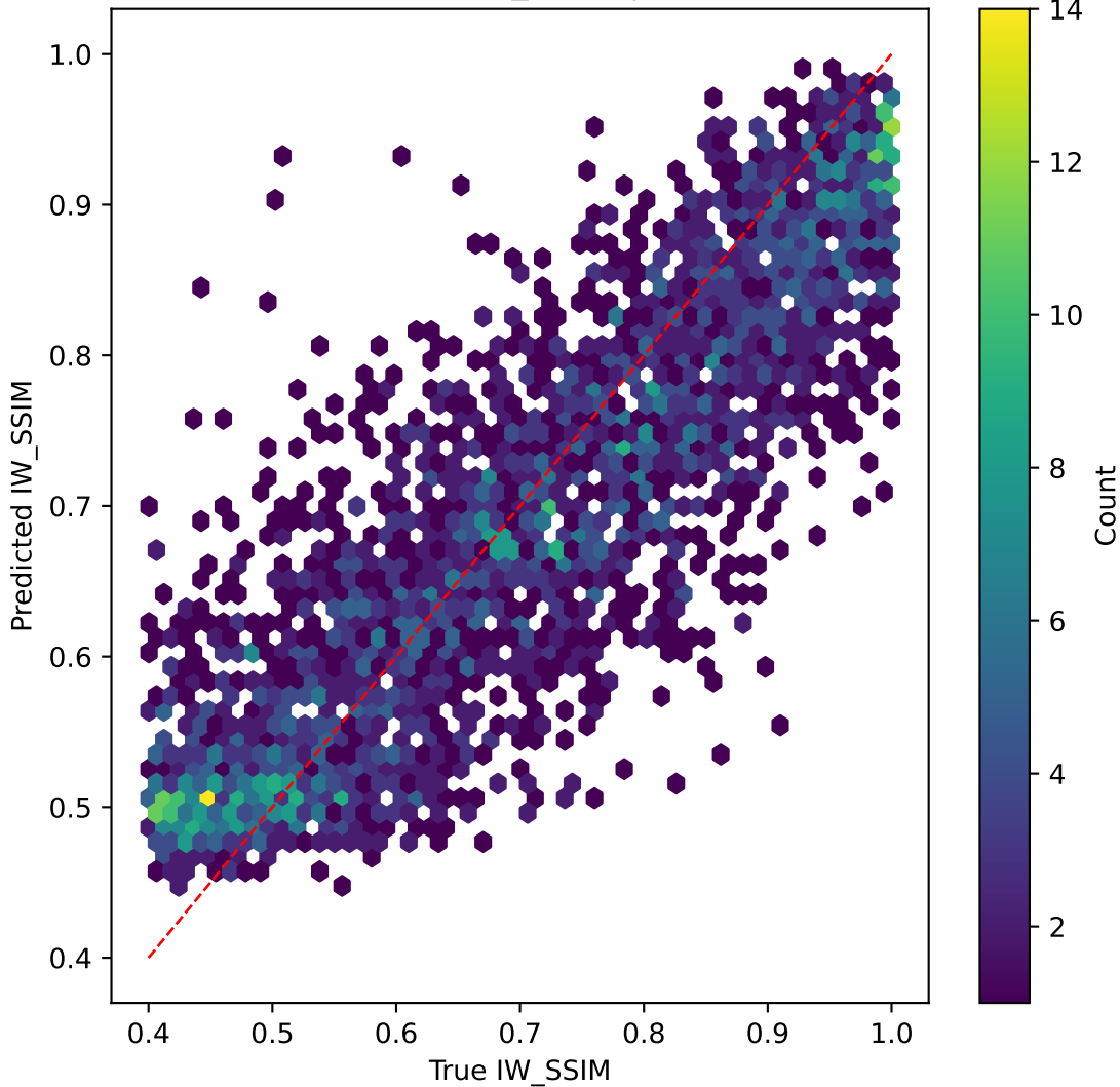
resnet50v2 on IW_SSIM | R^2=0.770
