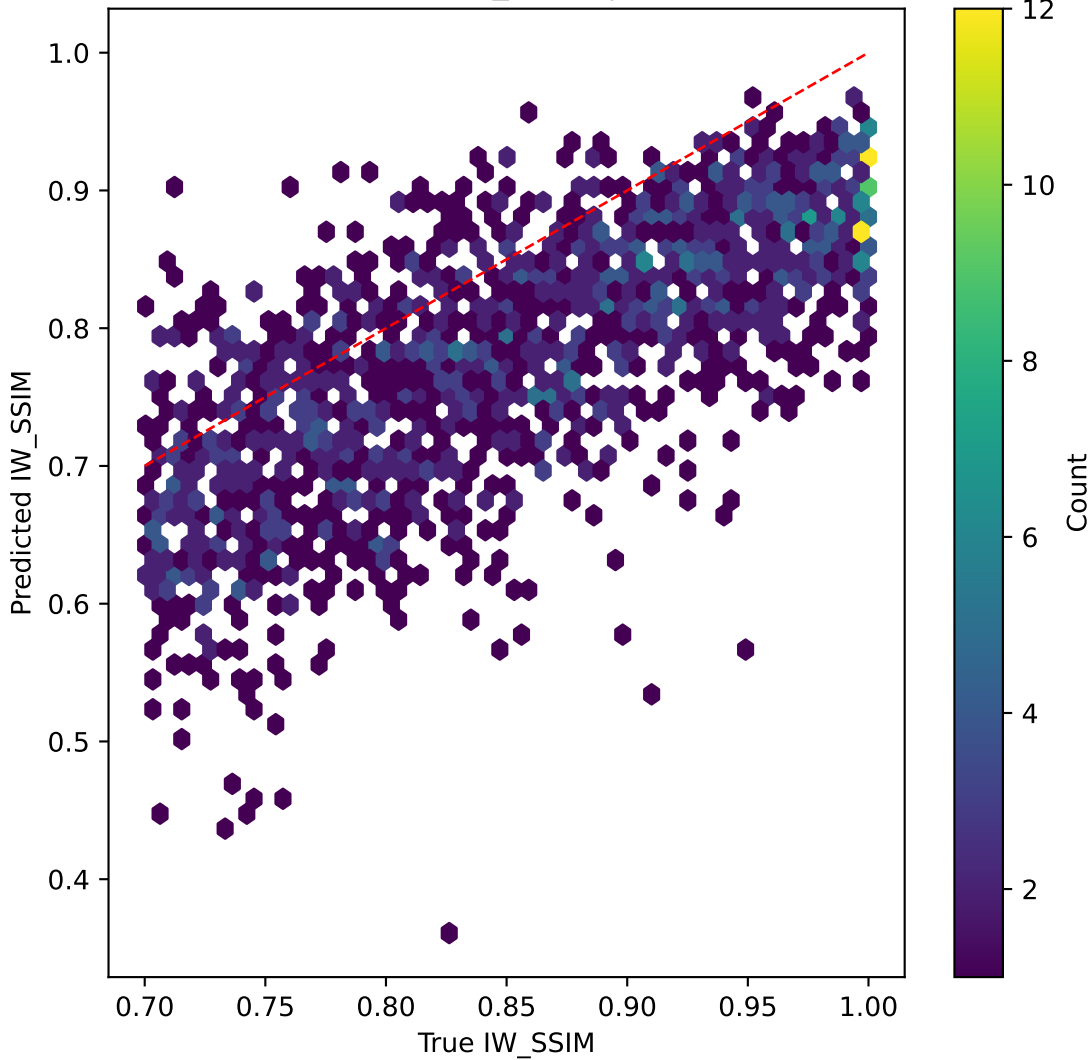
resnet50v2 on IW_SSIM | R^2=-0.250
