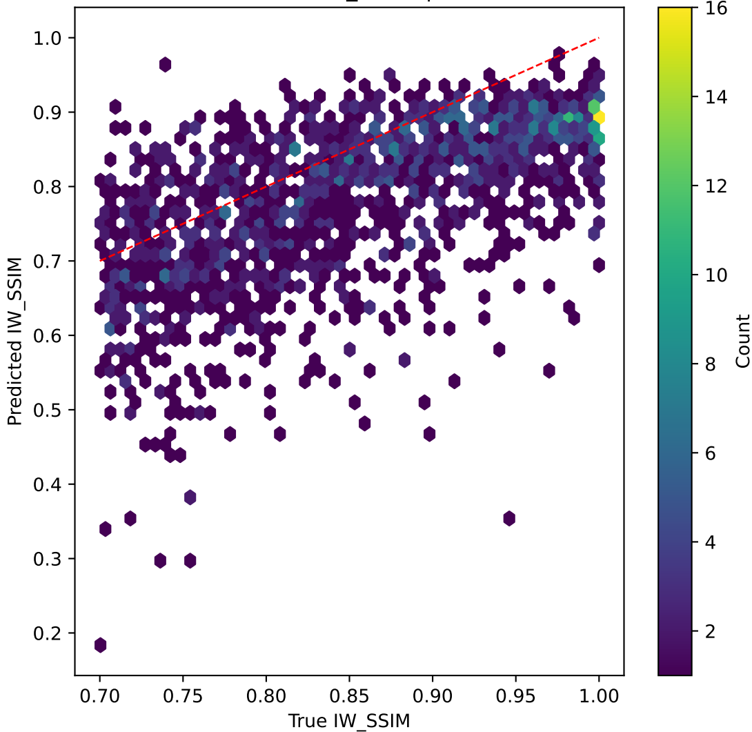
mobilenetv3 on IW_SSIM | R^2=-0.561
