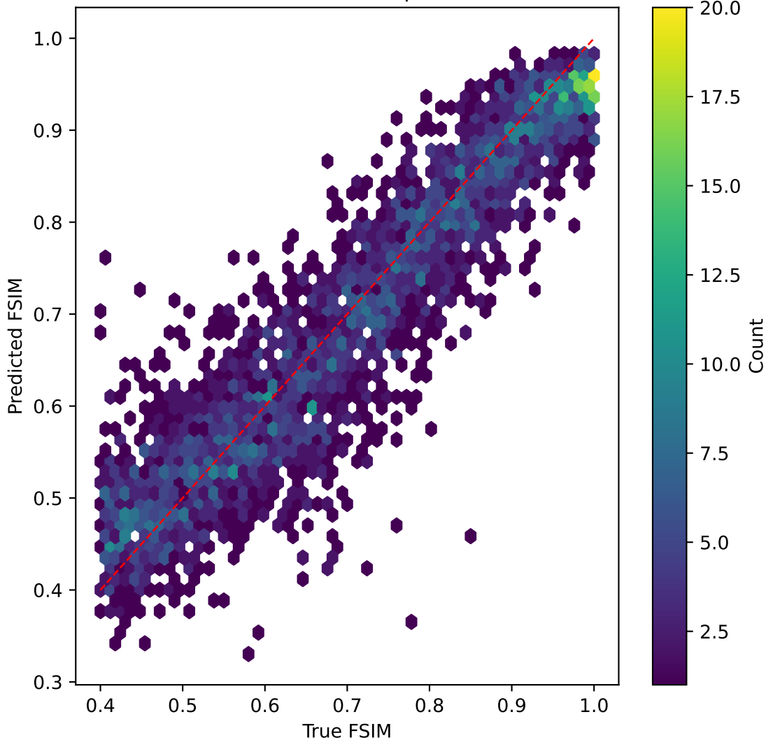
mobilevitv2 on FSIM | R^2=0.761
