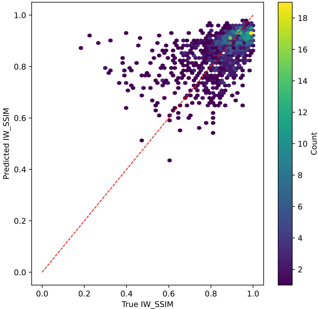
mobilevitv2 on IW_SSIM | R^2=0.191
