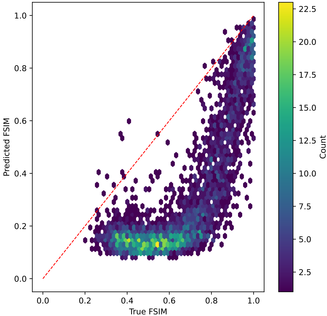
mobilevitv2 on FSIM | R^2=-7.904
