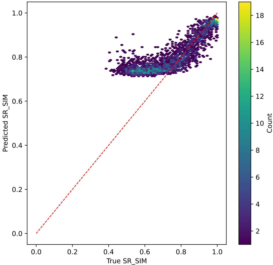
mobilenetv3 on SR_SIM | R^2=0.643
