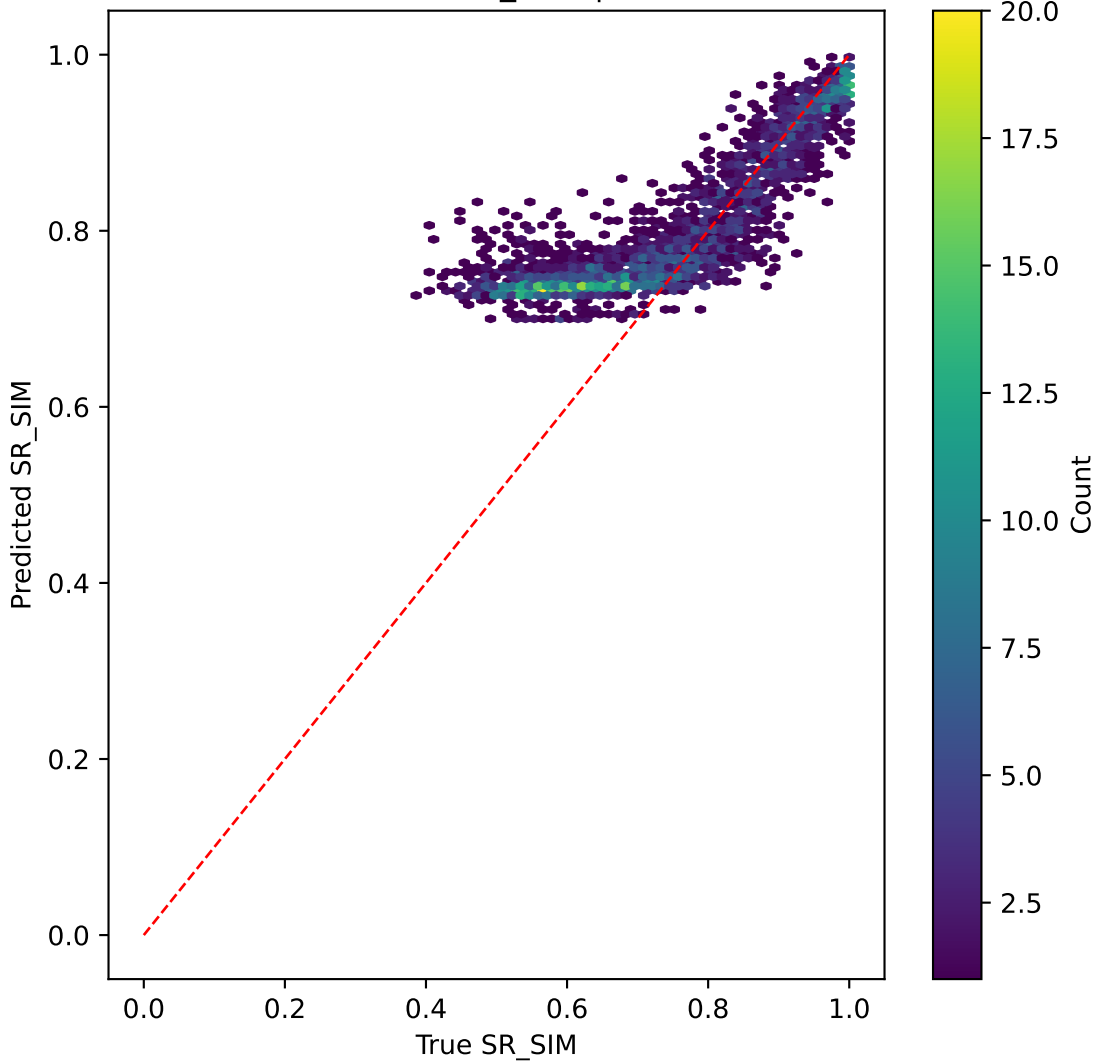
efficientnet on SR_SIM | R^2=0.669
