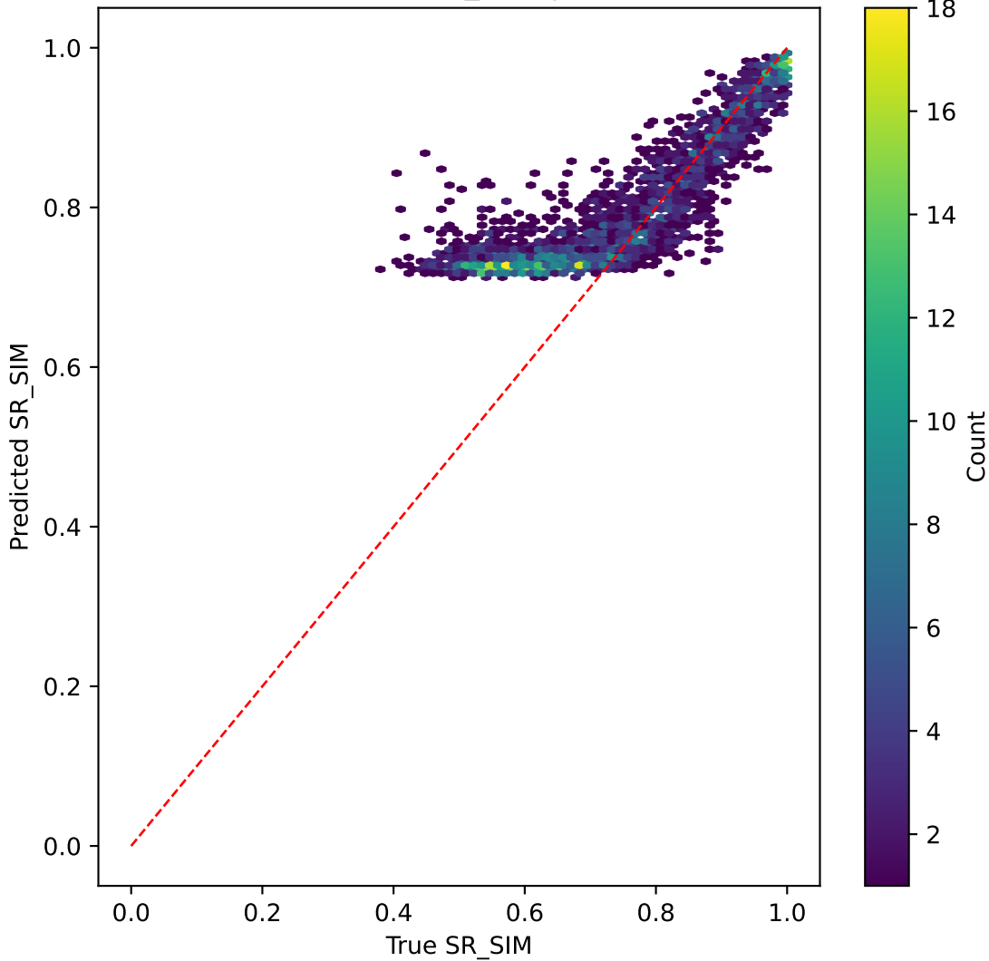
mobilevitv2 on SR_SIM | R^2=0.693
