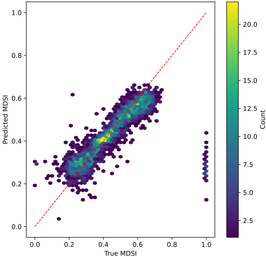
mobilevitv2 on MDSI | R^2=0.317
