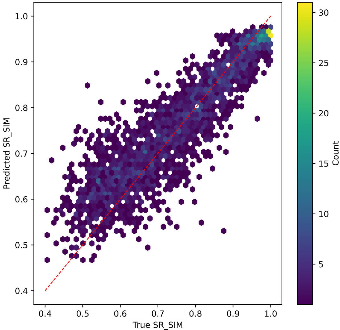
mobilevitv2 on SR_SIM | R^2=0.728
