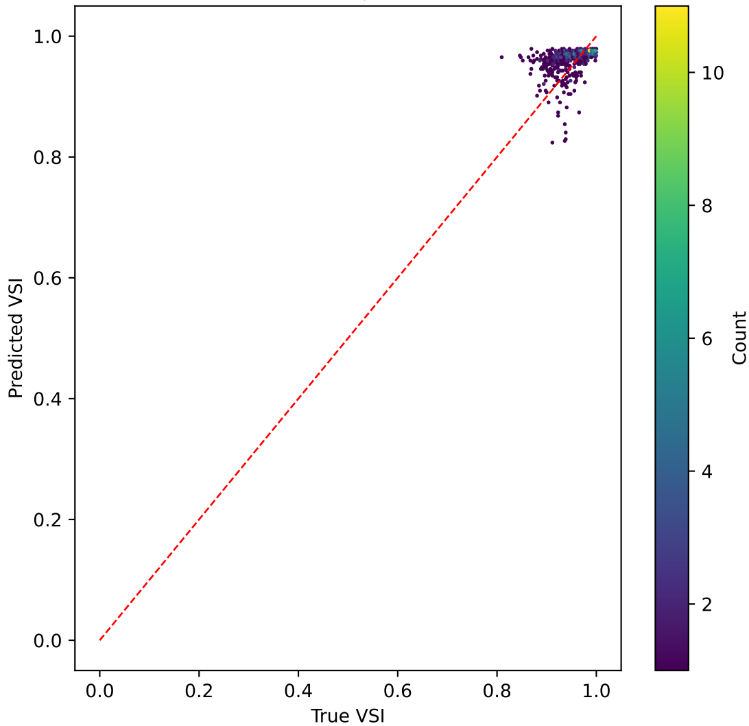
tinyvit on VSI | R^2=-0.012
