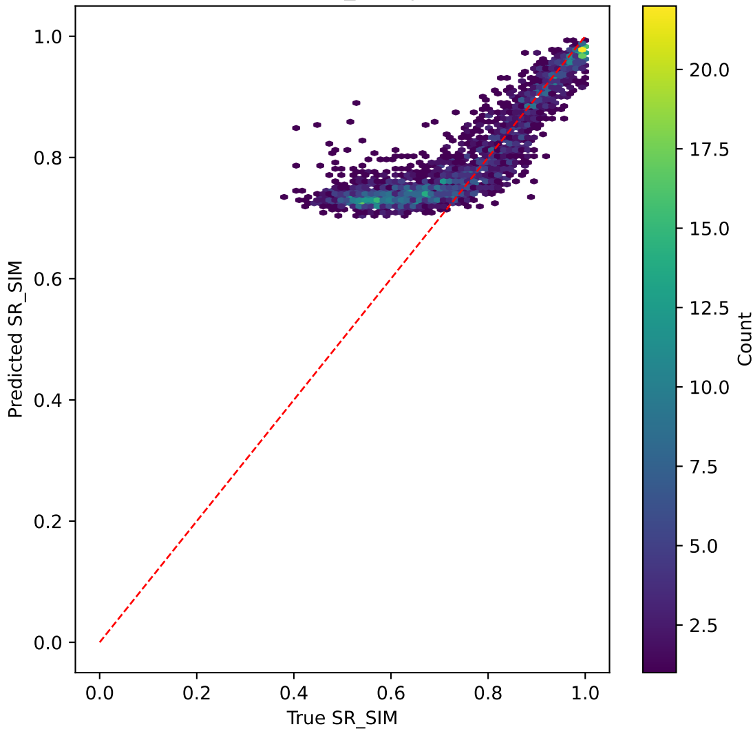
resnet50v2 on SR_SIM | R^2=0.696
