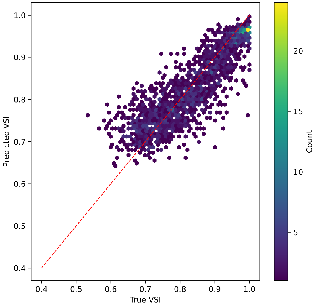
mobilenetv3 on VSI | R^2=0.452
