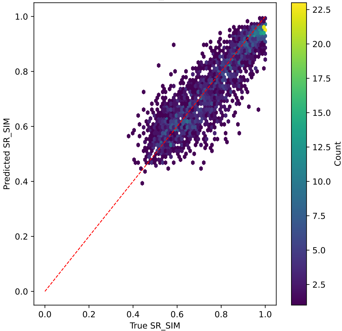
mobilenetv3 on SR_SIM | R^2=0.518
