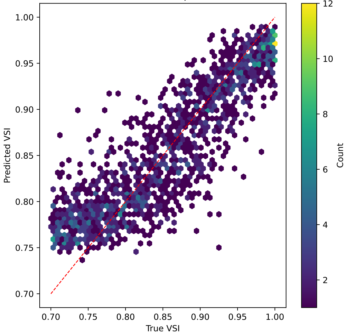
efficientnet on VSI | R^2=0.623
