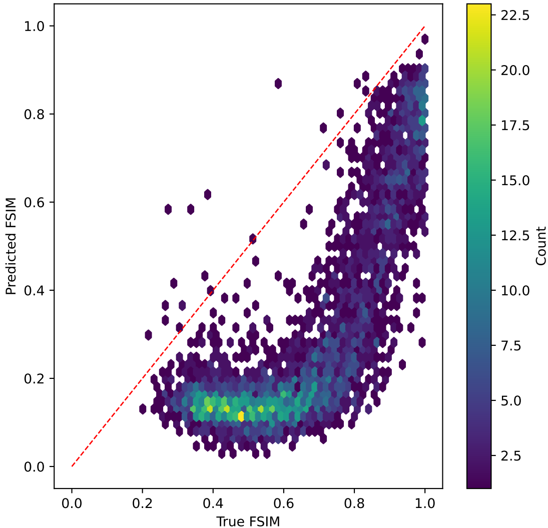
mobilenetv3 on FSIM | R^2=-8.117
