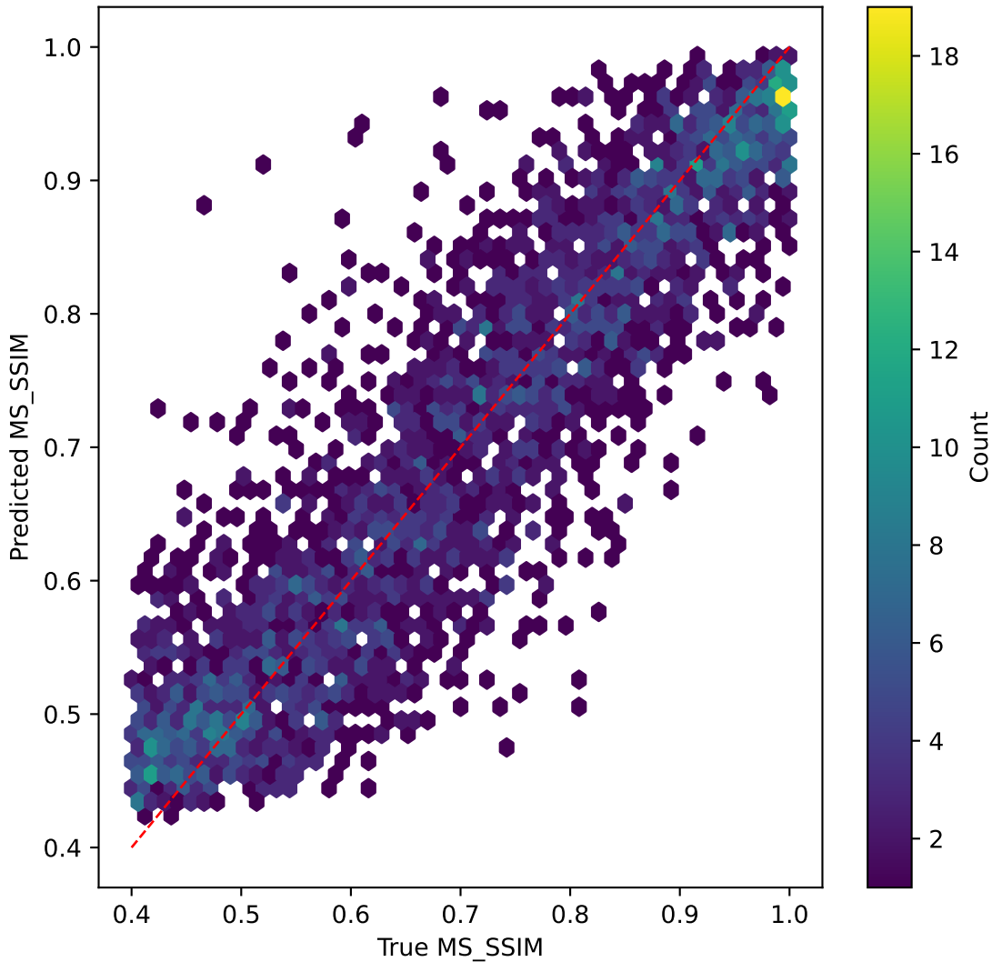
mobilevitv2 on MS_SSIM | R^2=0.792
