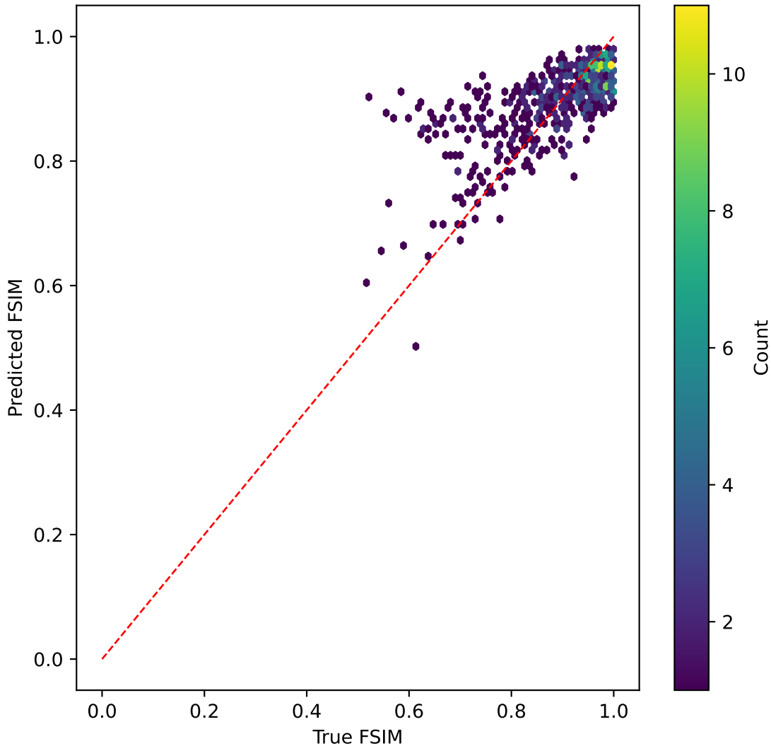
mobilevitv2 on FSIM | R^2=0.484
