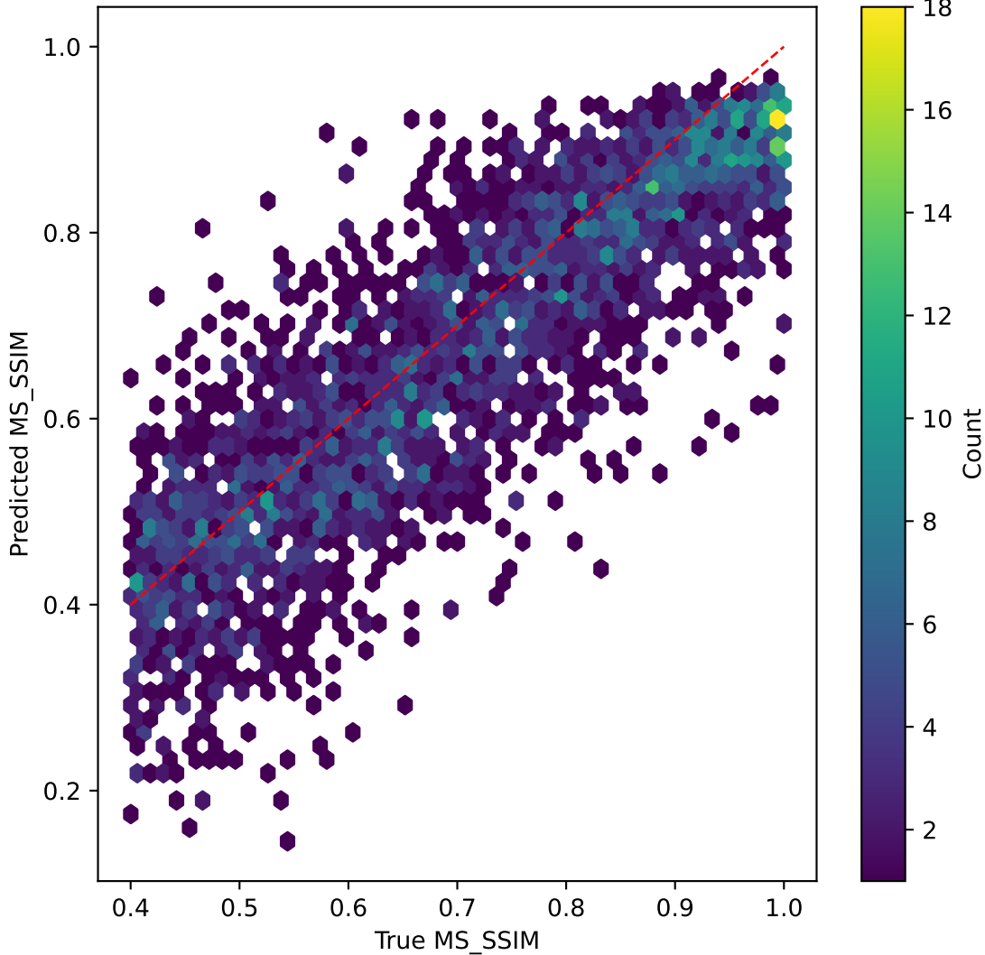
efficientnet on MS_SSIM | R^2=0.660
