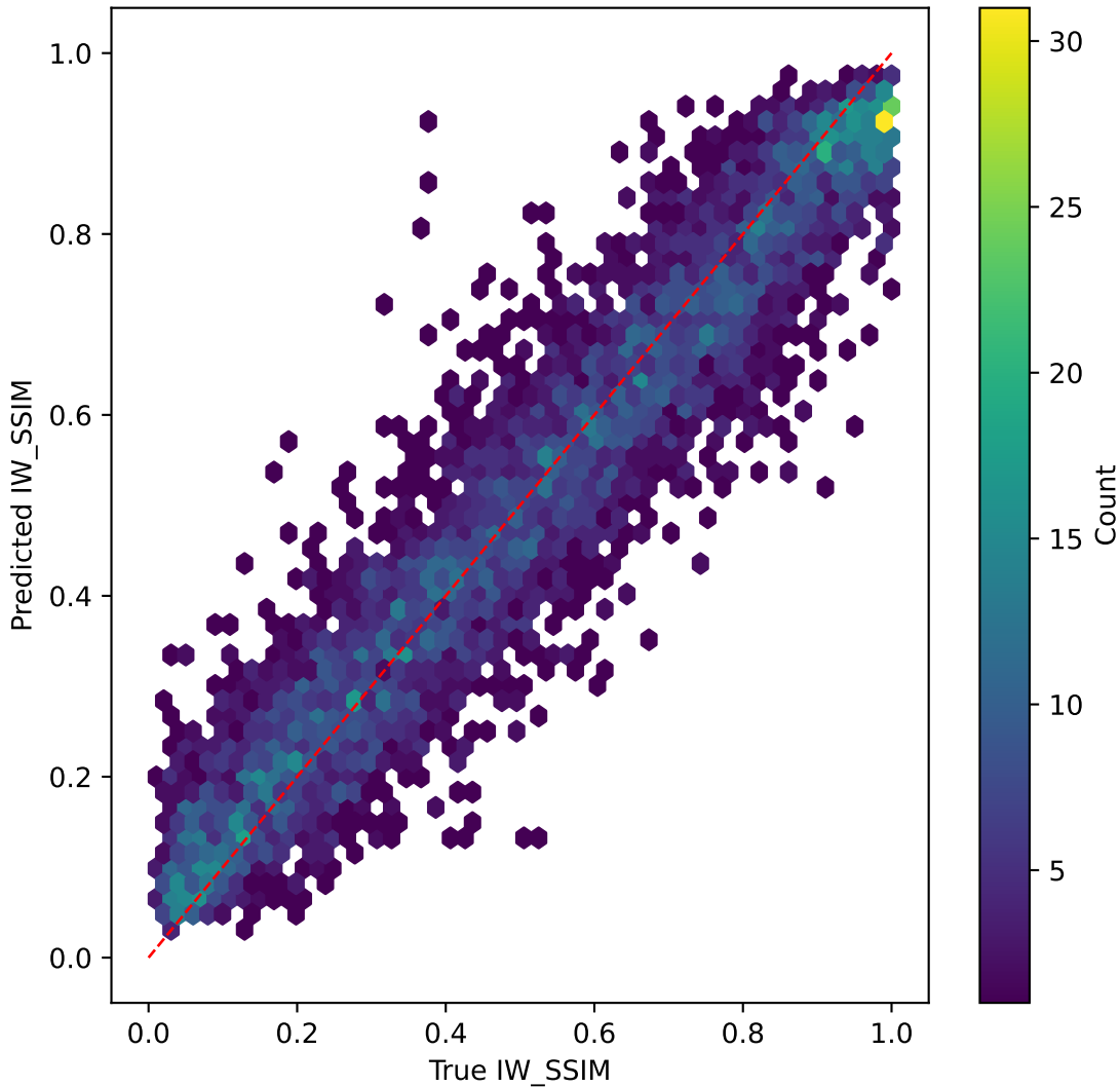
mobilevitv2 on IW_SSIM | R^2=0.888
