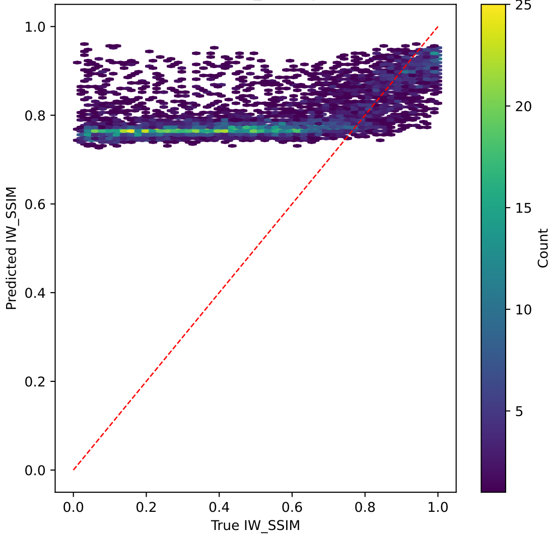
mobilenetv3 on IW_SSIM | R^2=-1.942
