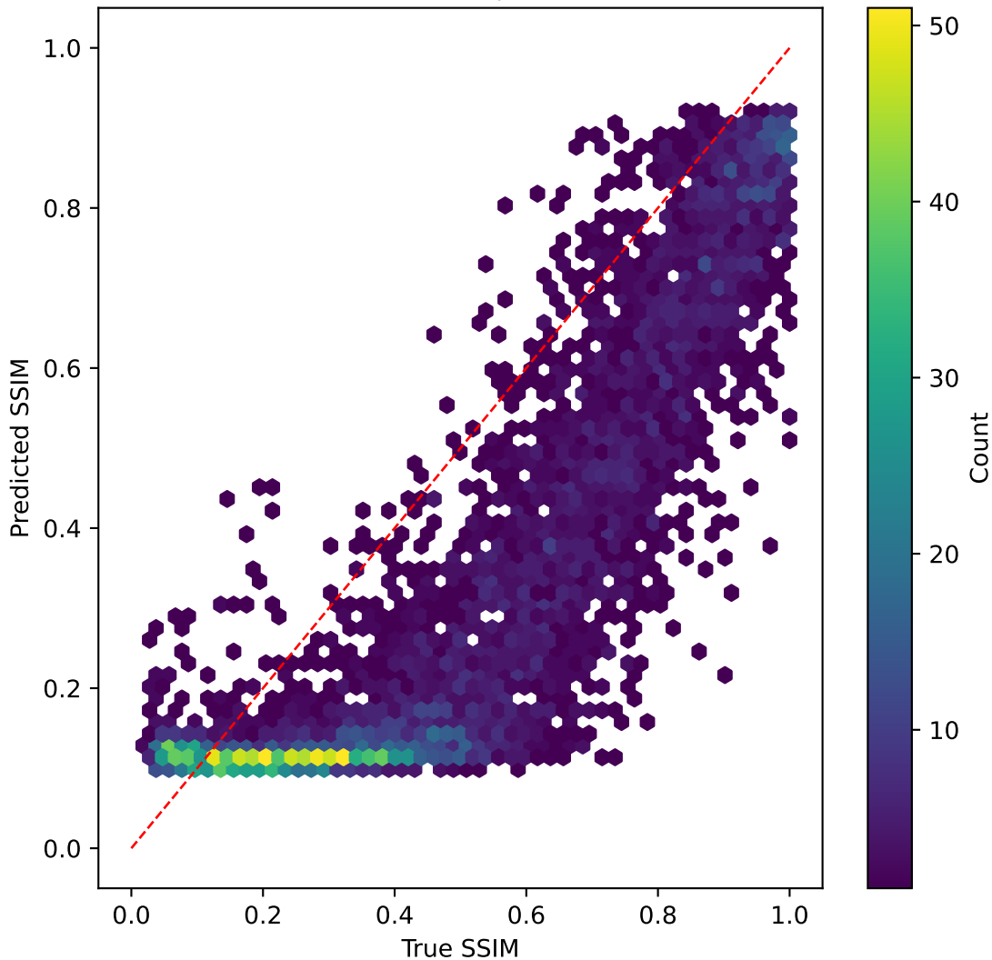
tinyvit on SSIM | R^2=0.147
