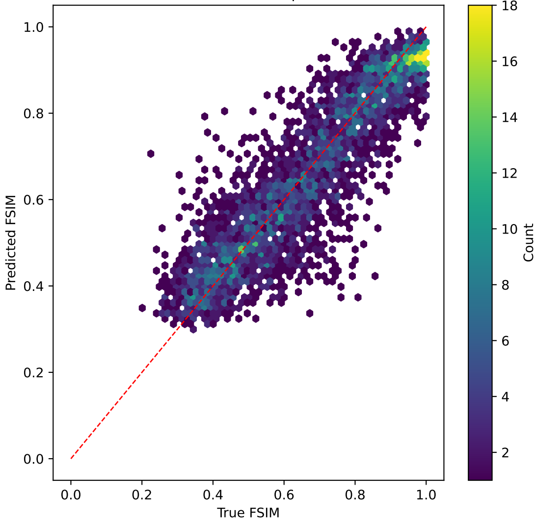
mobilenetv3 on FSIM | R^2=0.587
