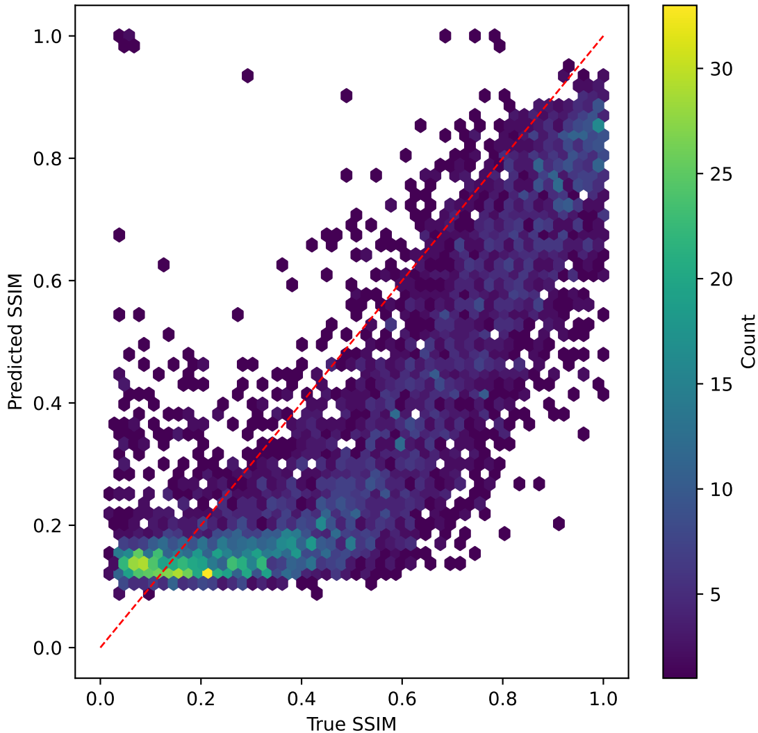
efficientnet on SSIM | R^2=0.306
