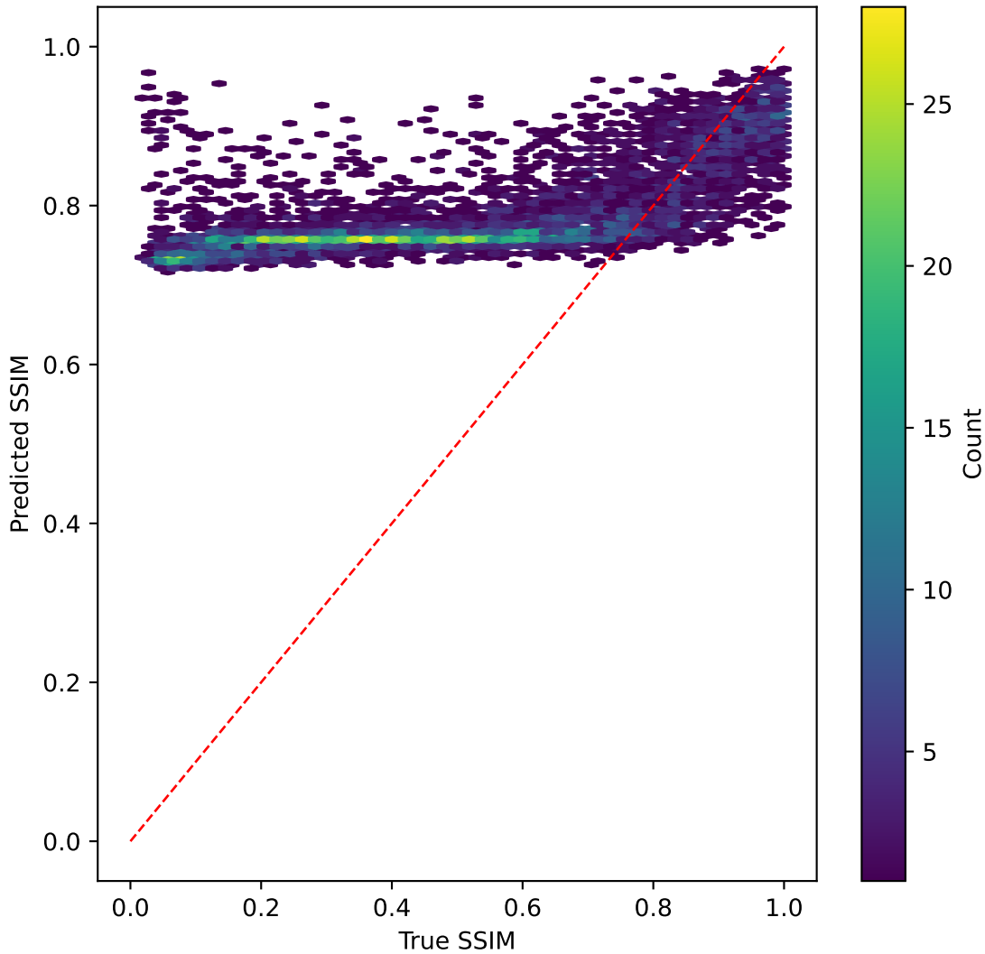
resnet50v2 on SSIM | R^2=-1.984
