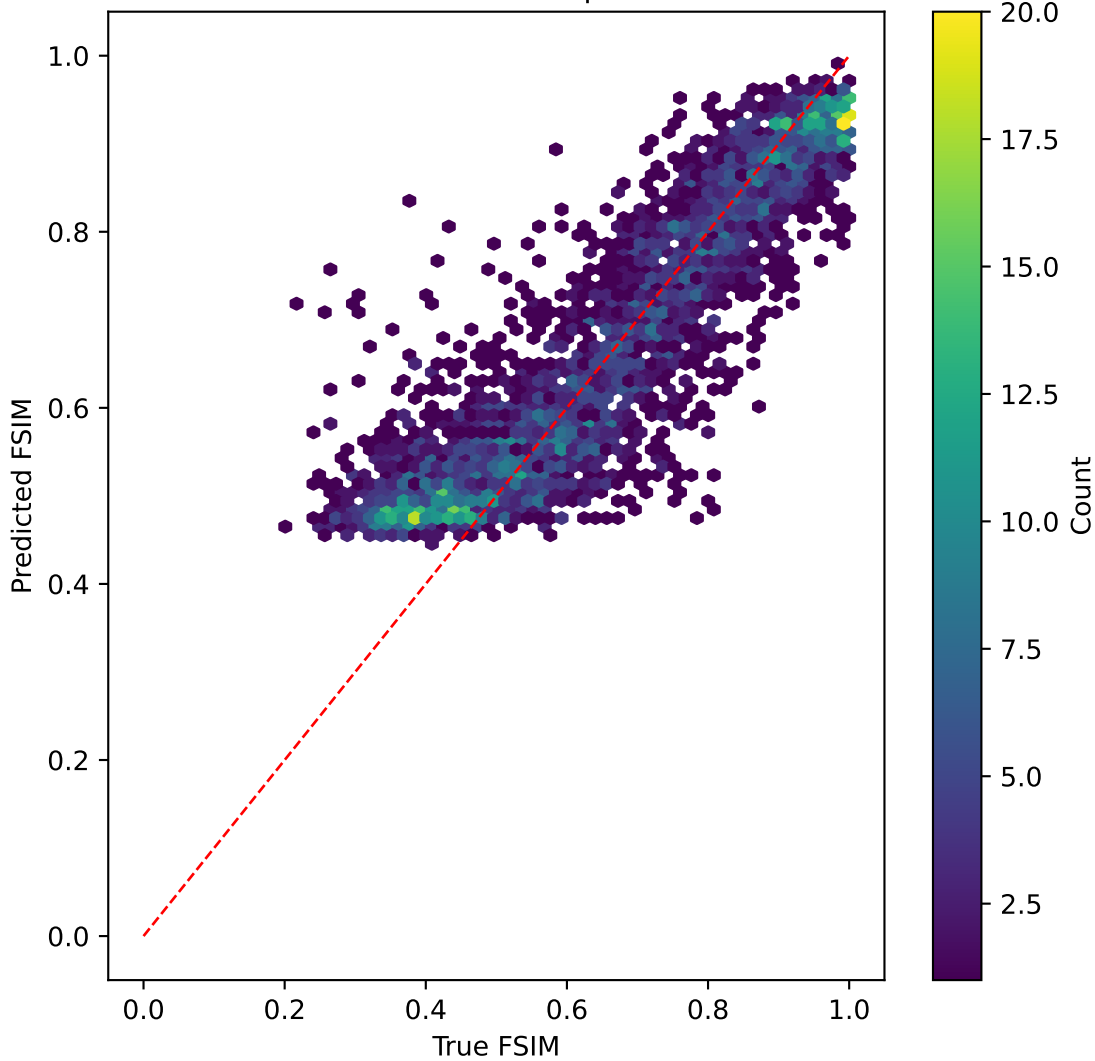
mobilenetv3 on FSIM | R^2=0.723
