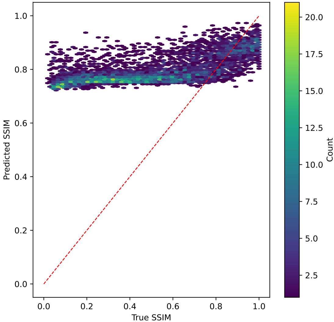
mobilenetv3 on SSIM | R^2=-2.116
