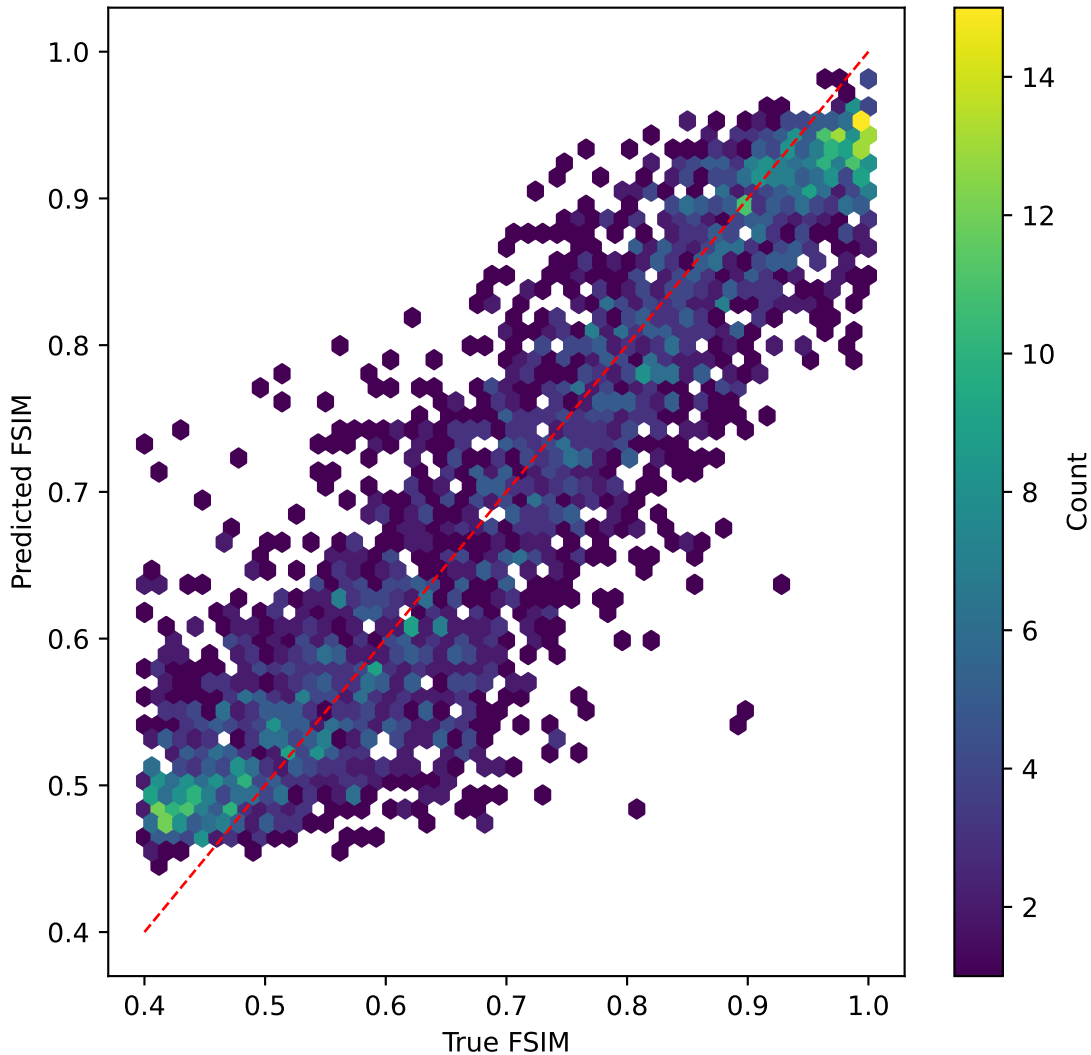
mobilenetv3 on FSIM | R^2=0.720
