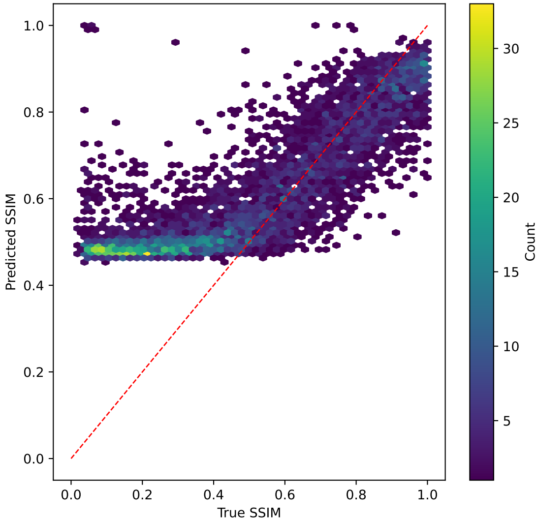
efficientnet on SSIM | R^2=0.169
