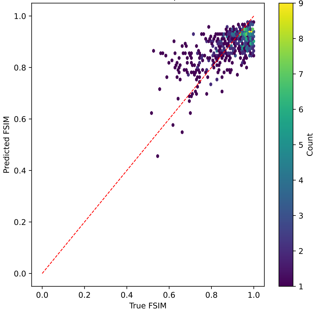
mobilenetv3 on FSIM | R^2=0.336
