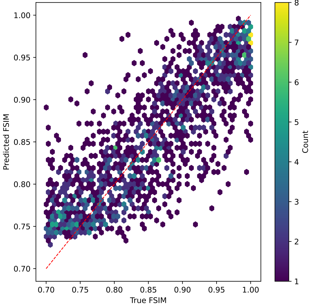
mobilevitv2 on FSIM | R^2=0.679
