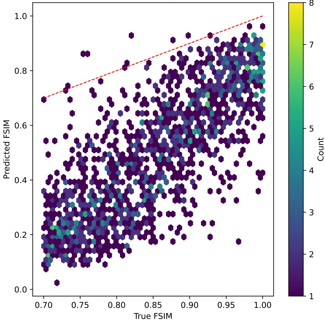
efficientnet on FSIM | R^2=-22.561
