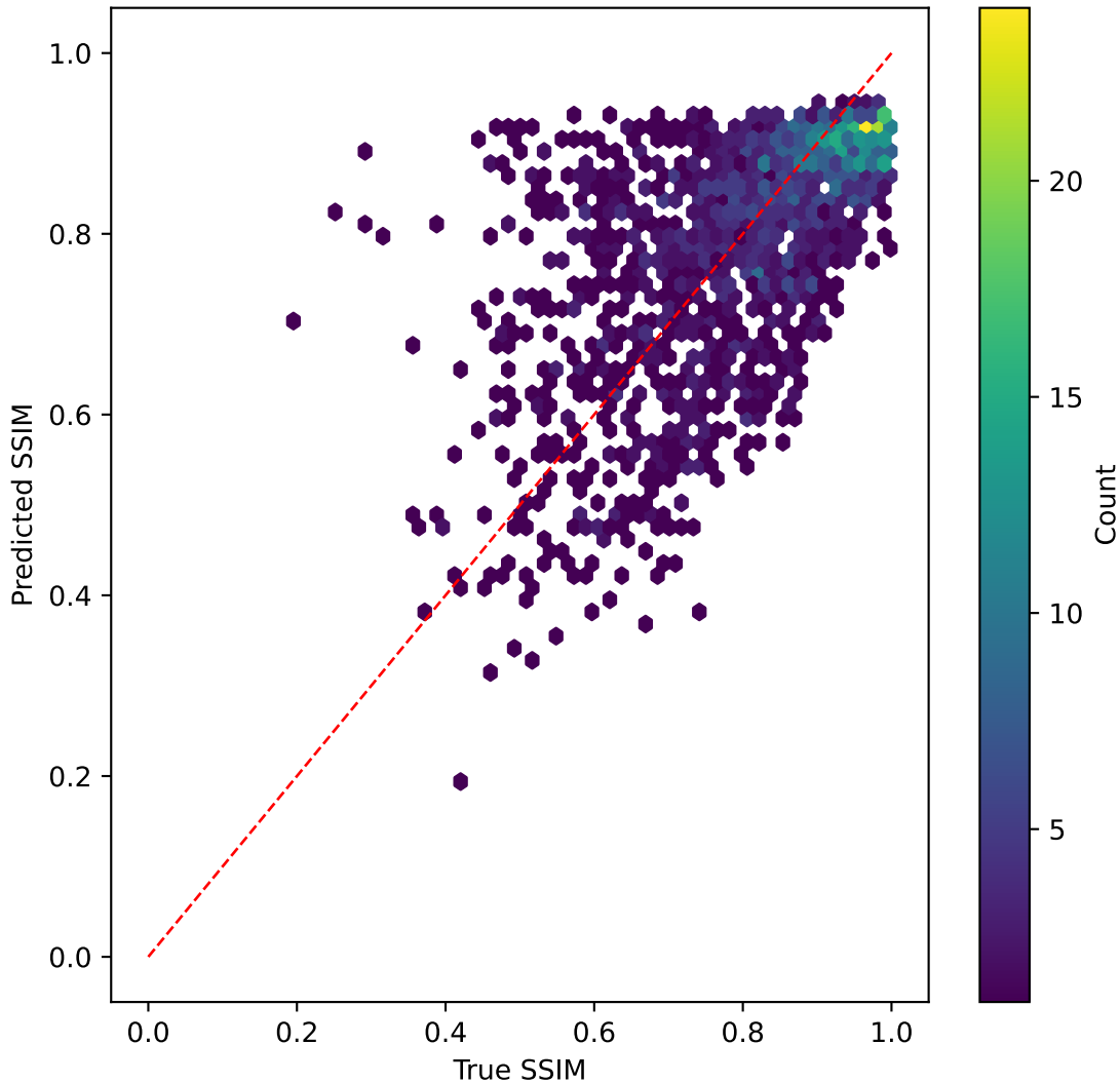
tinyvit on SSIM | R^2=0.365
