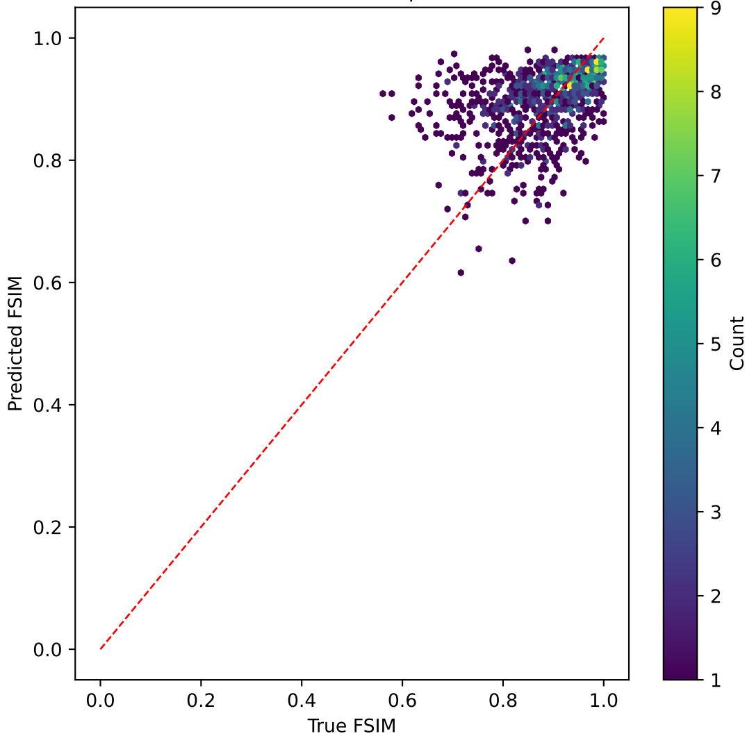
mobilevitv2 on FSIM | R^2=0.085
