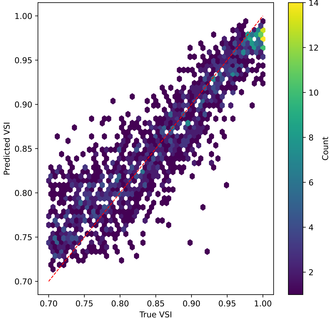
resnet50v2 on VSI | R^2=0.695
