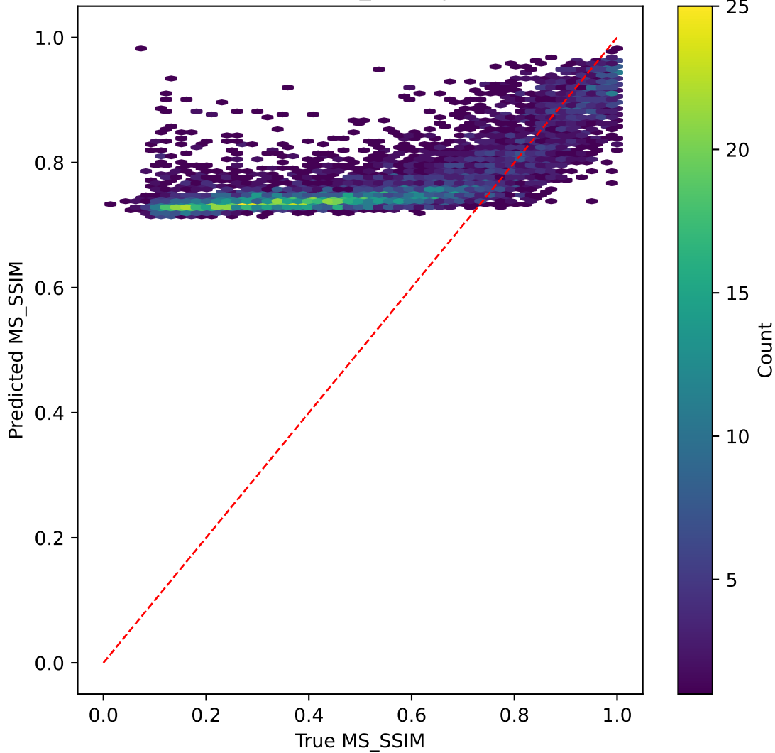
mobilenetv3 on MS_SSIM | R^2=-0.923
