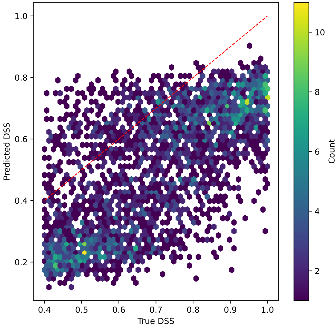
mobilenetv3 on DSS | R^2=-0.677
