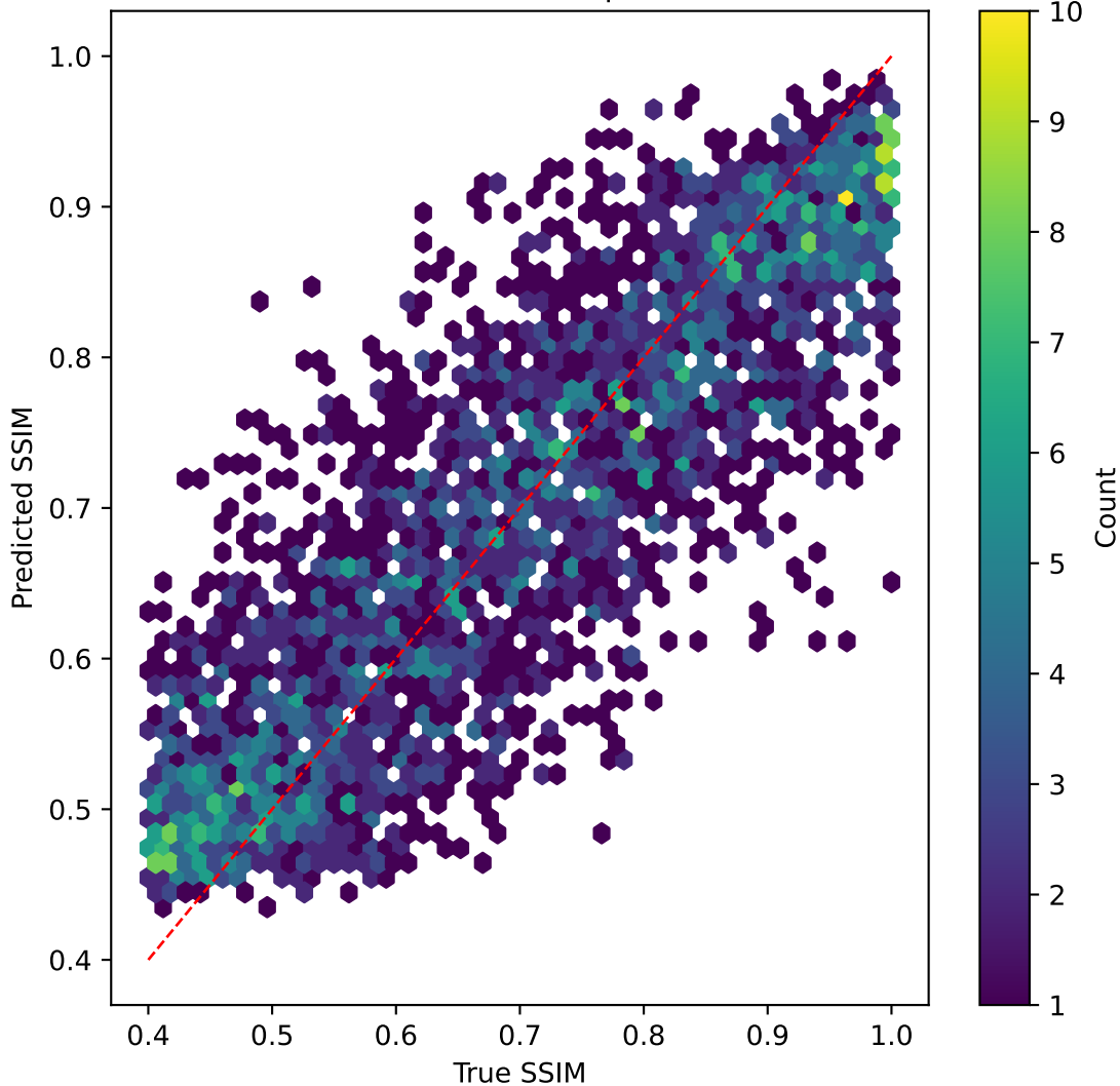
mobilevitv2 on SSIM | R^2=0.698
