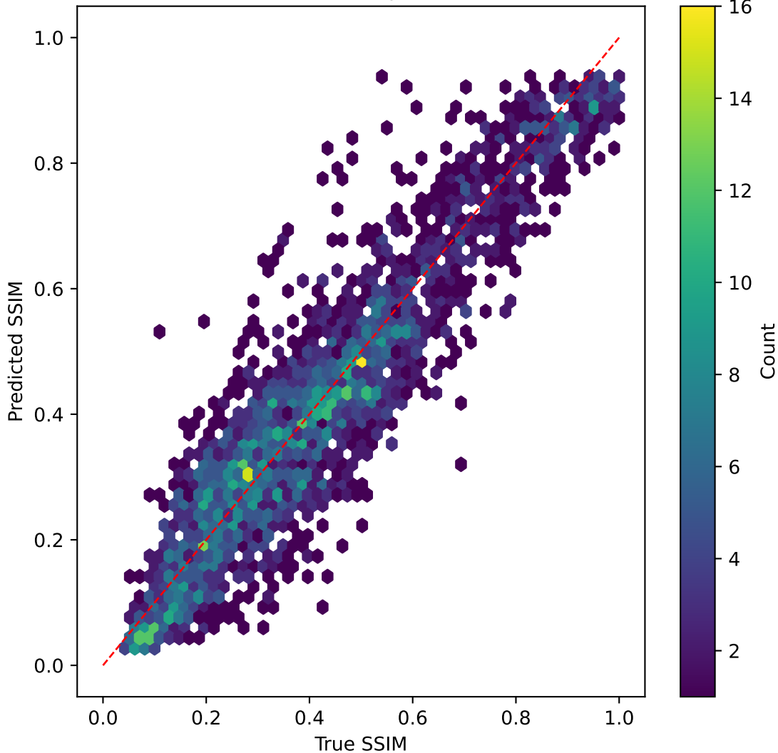
tinyvit on SSIM | R^2=0.852
