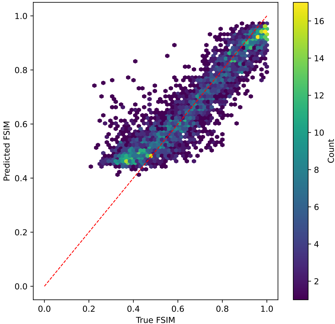
efficientnet on FSIM | R^2=0.755
