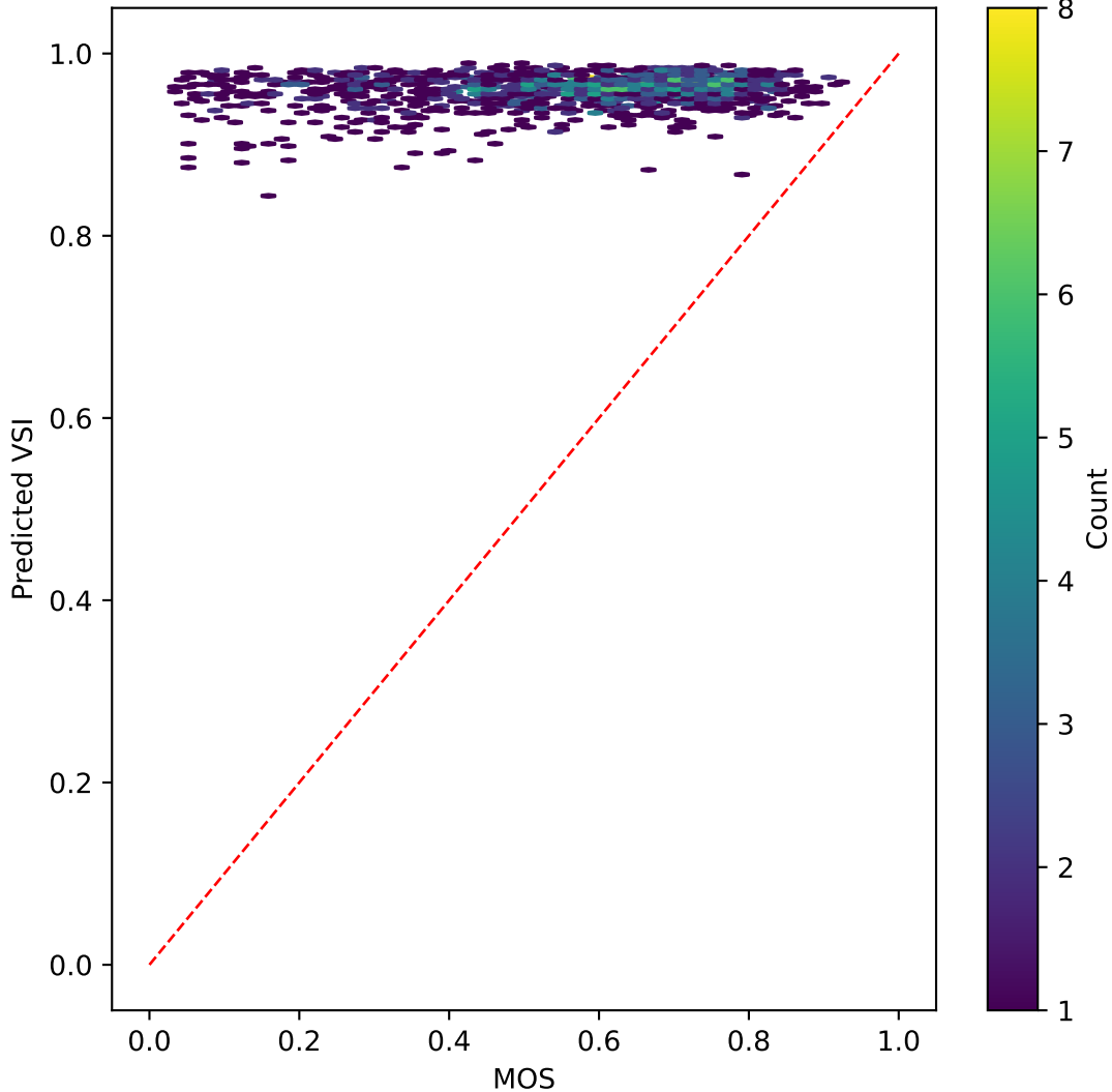
tinyvit on VSI AGAINST MOS | R^2=-3.962
