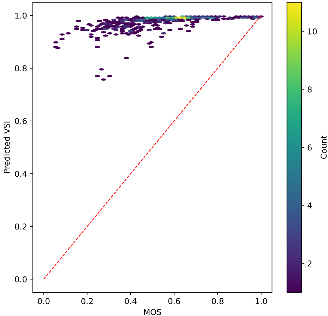
tinyvit on VSI AGAINST MOS | R^2=-5.346
