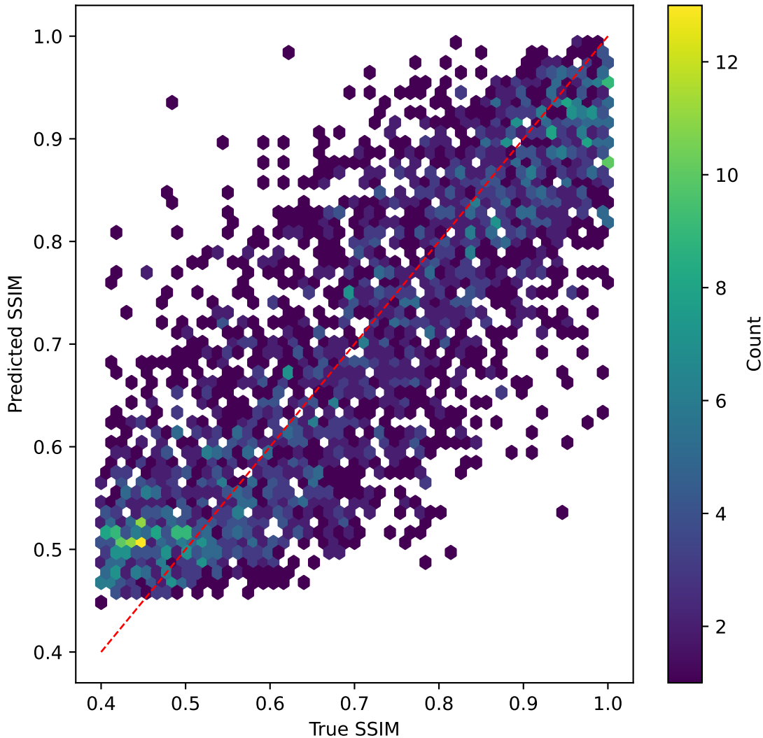
resnet50v2 on SSIM | R^2=0.643
