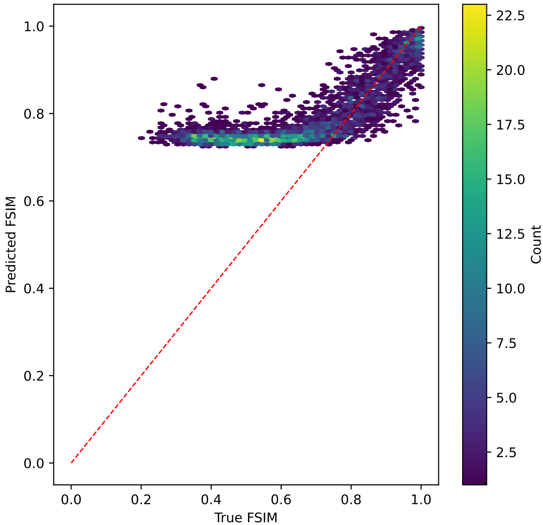
mobilevitv2 on FSIM | R^2=-0.107
