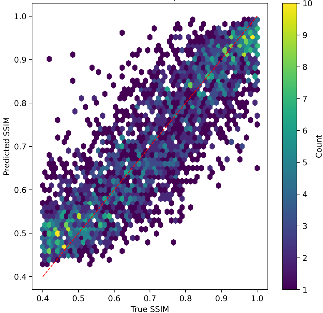
resnet50v2 on SSIM | R^2=0.700
