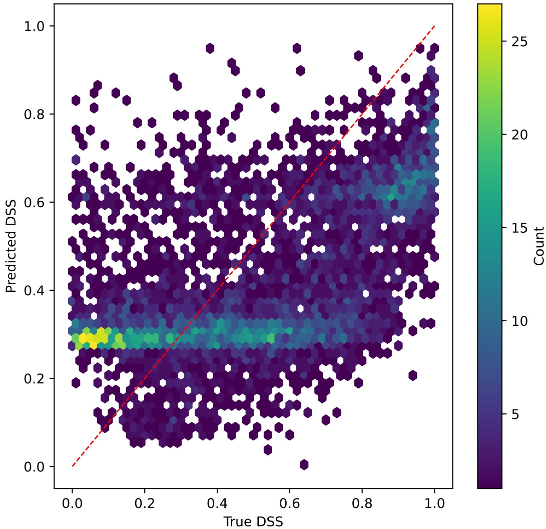
resnet50v2 on DSS | R^2=-0.010
