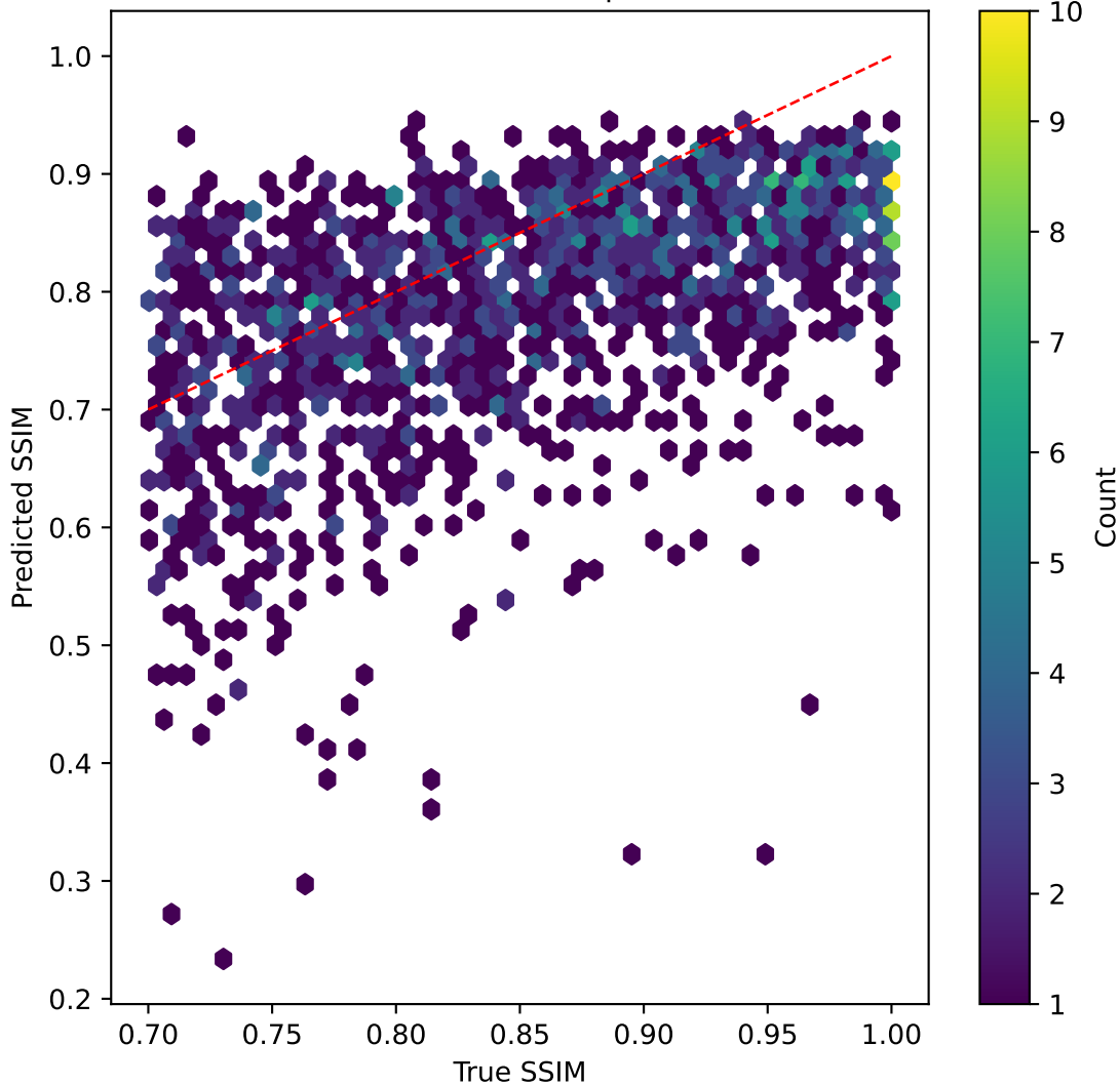
mobilenetv3 on SSIM | R^2=-0.614
