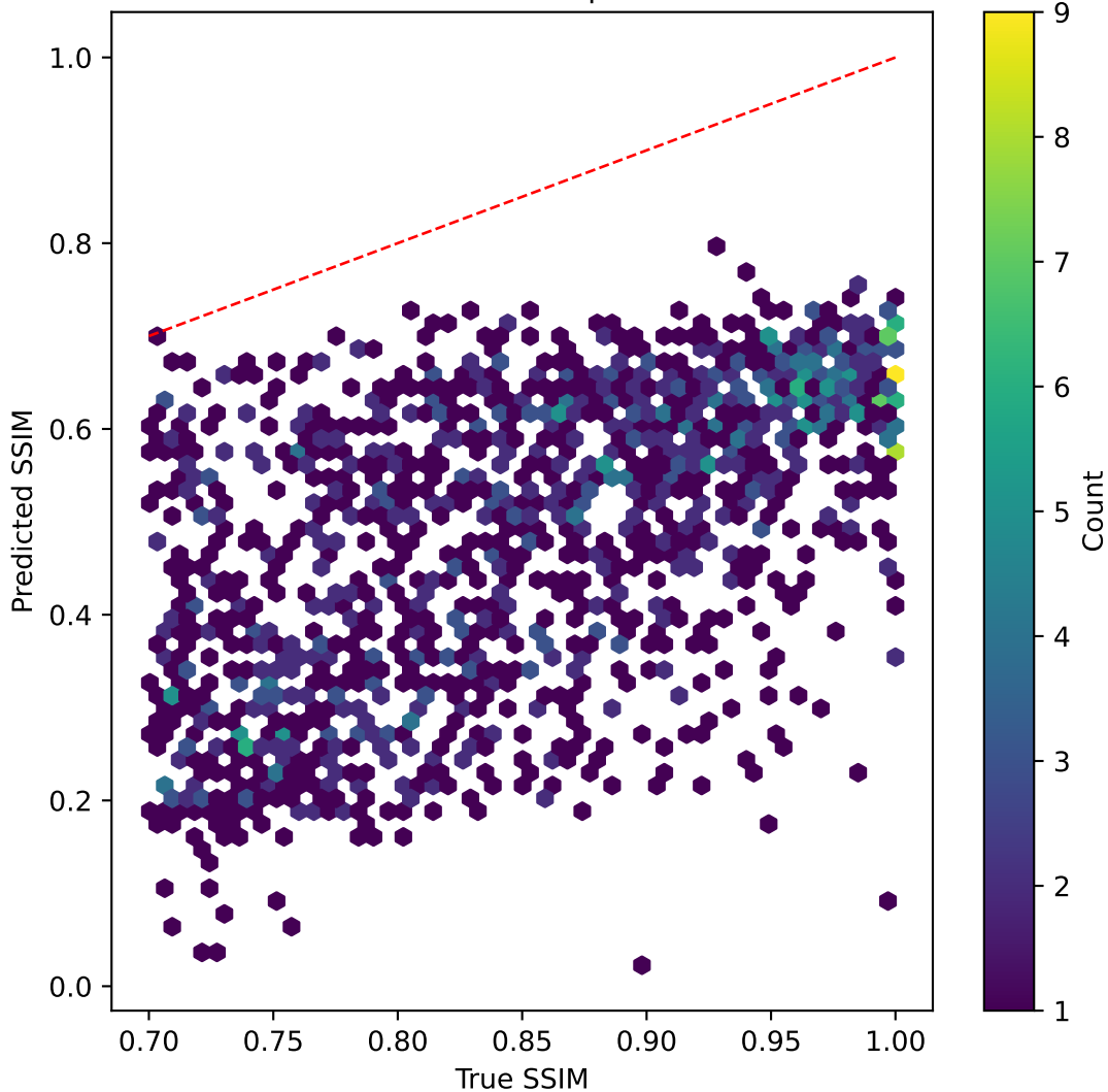
efficientnet on SSIM | R^2=-19.226
