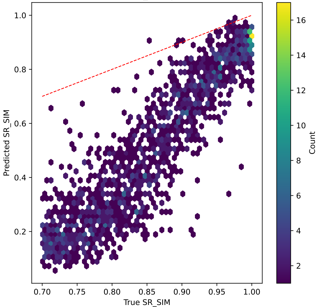
resnet50v2 on SR_SIM | R^2=-27.155
