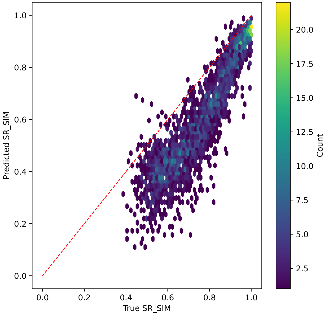
resnet50v2 on SR_SIM | R^2=-1.902
