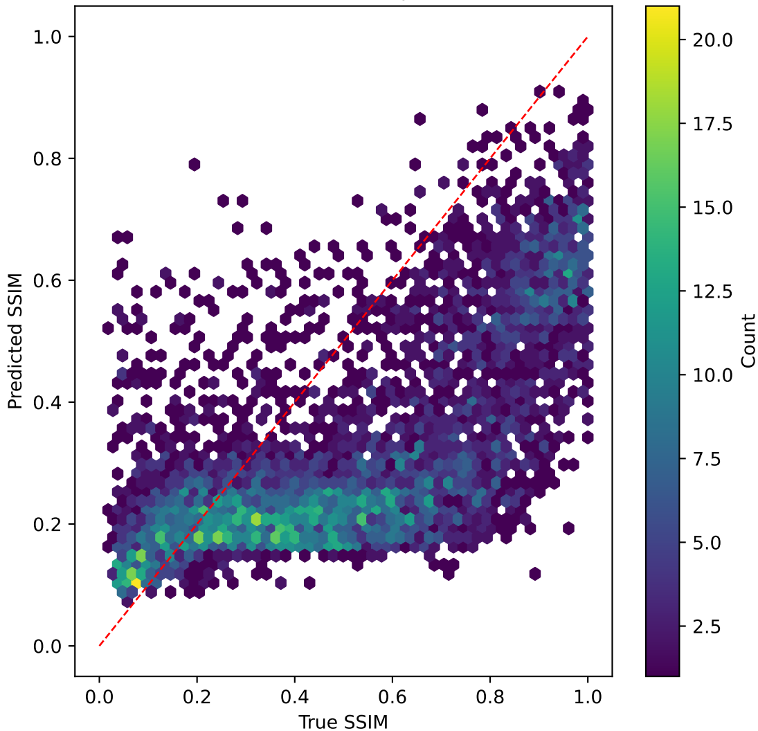
mobilenetv3 on SSIM | R^2=-0.020
