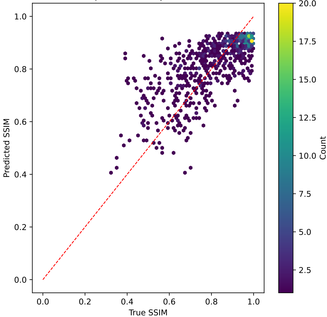
tinyvit on SSIM | R^2=0.550
