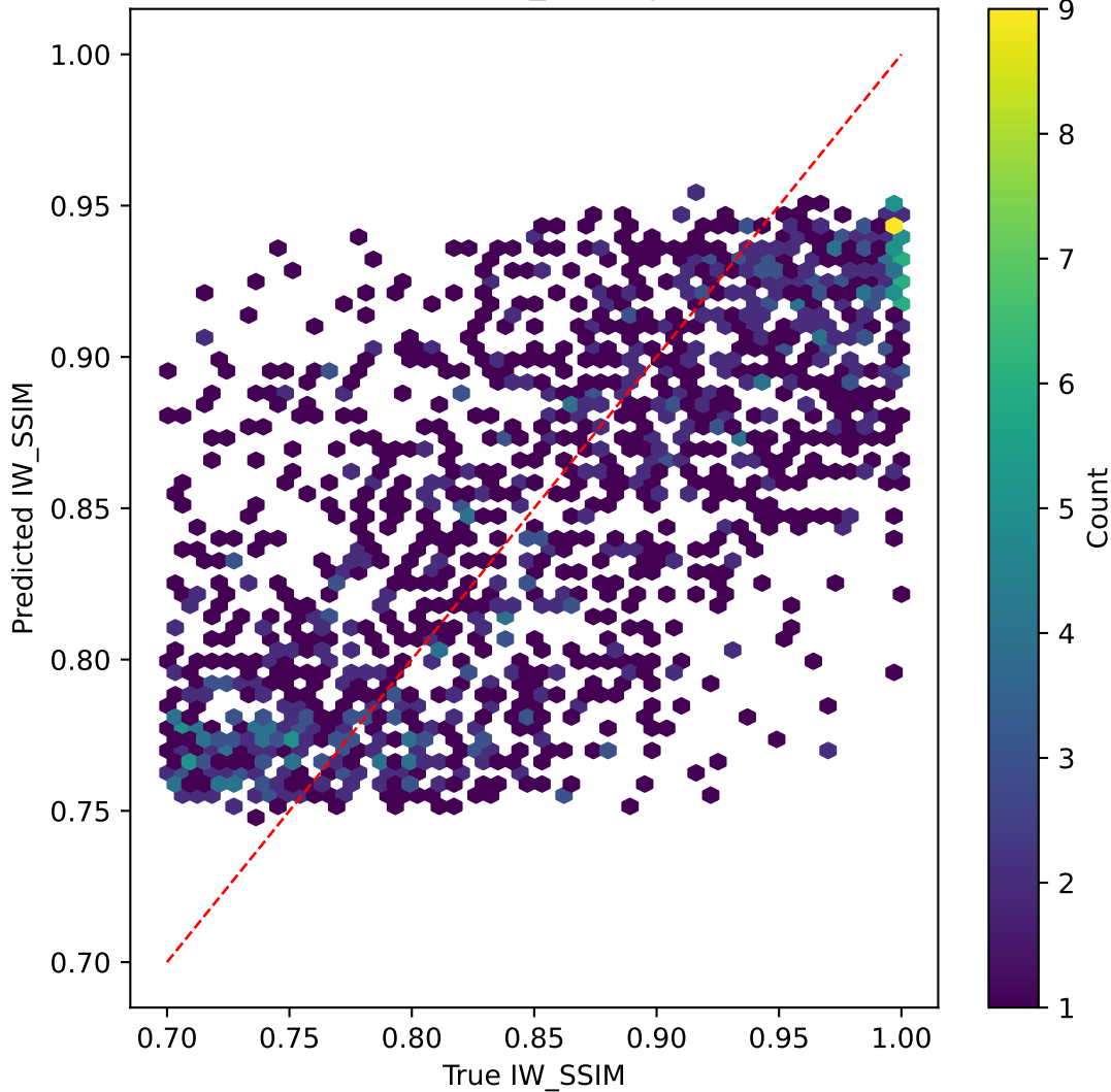
mobilevitv2 on IW_SSIM | R^2=0.481
