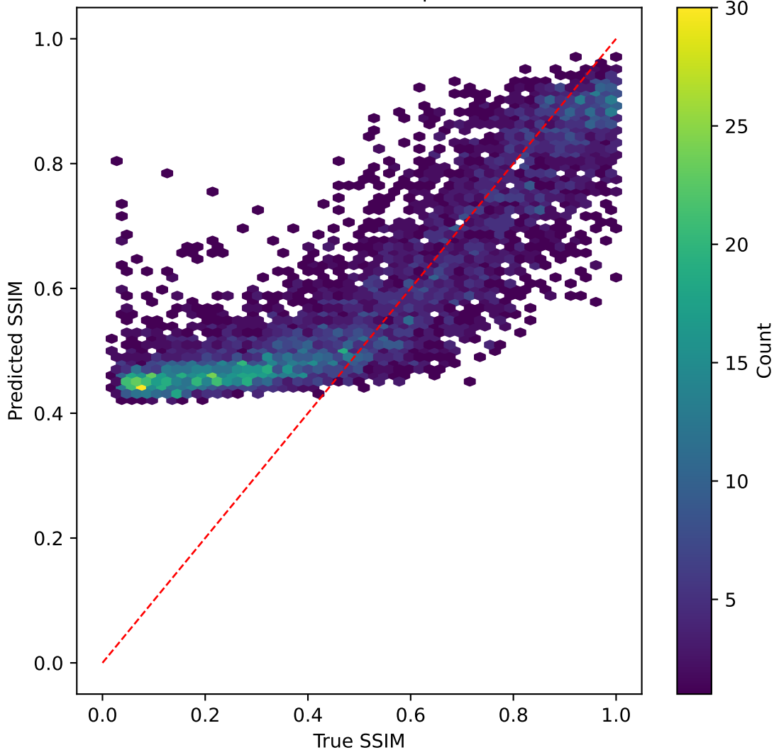
mobilenetv3 on SSIM | R^2=0.304
