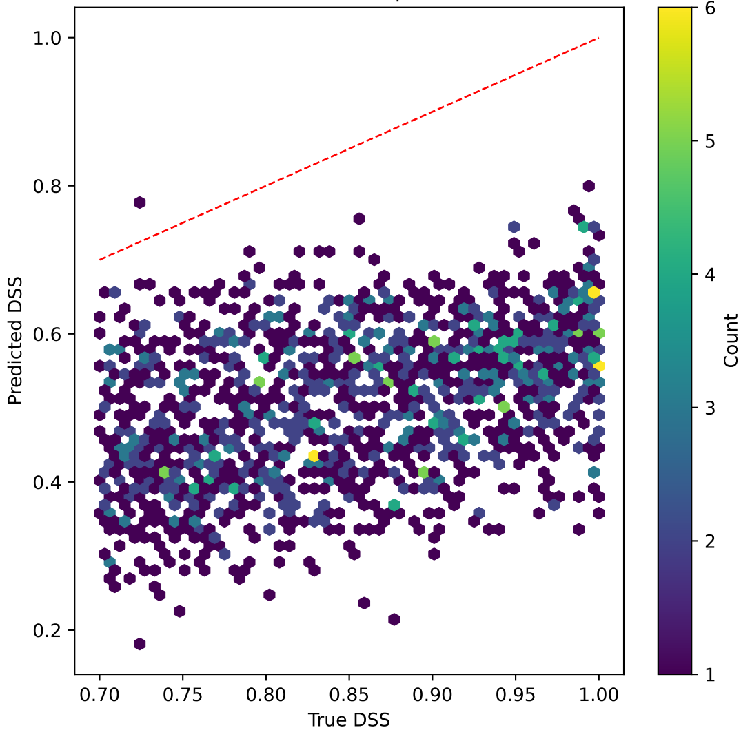
mobilenetv3 on DSS | R^2=-14.684
