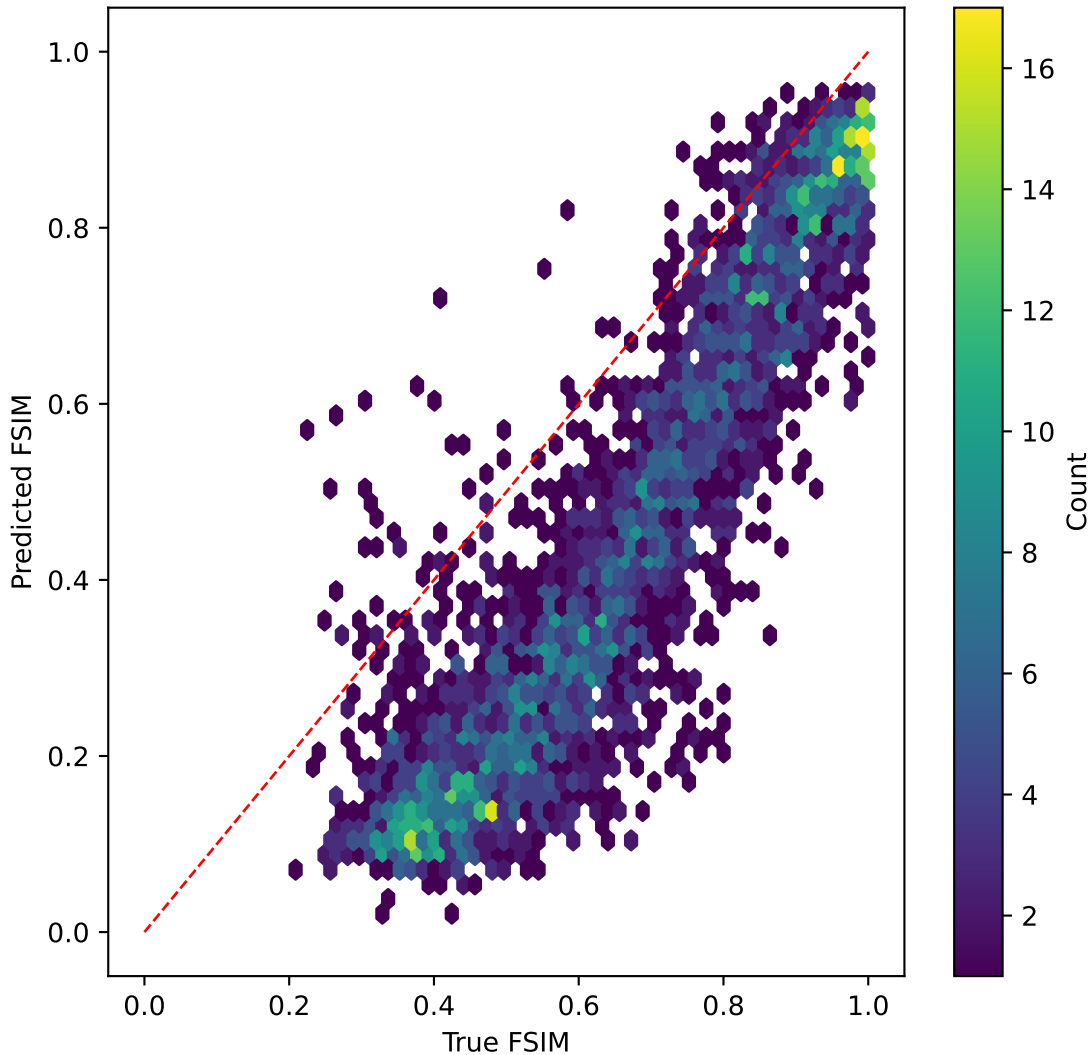
efficientnet on FSIM | R^2=-2.253
