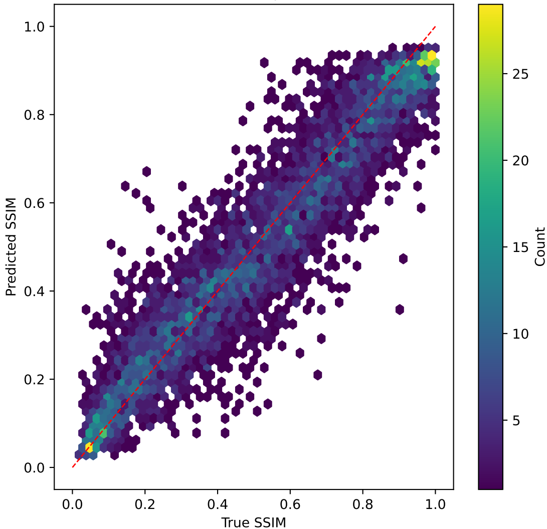
tinyvit on SSIM | R^2=0.834
