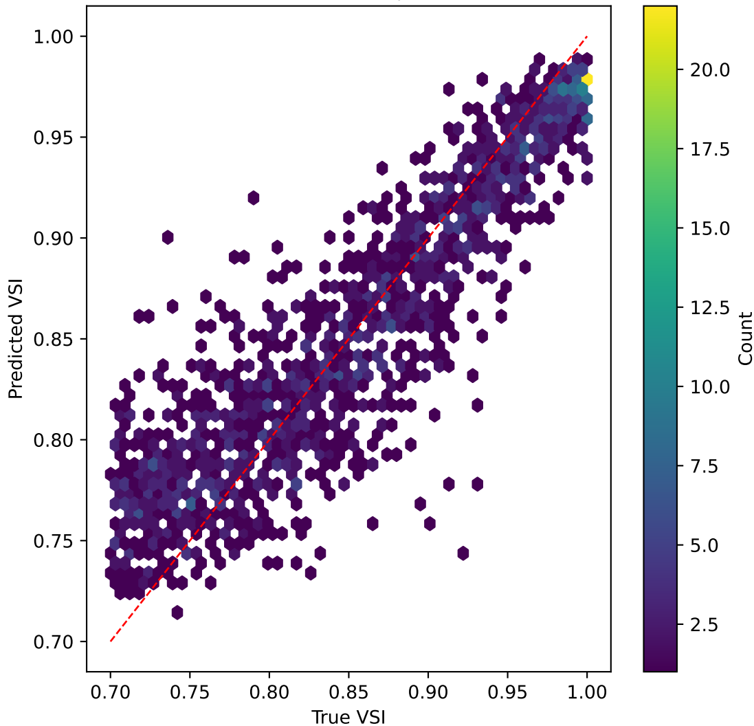
mobilevitv2 on VSI | R^2=0.695
