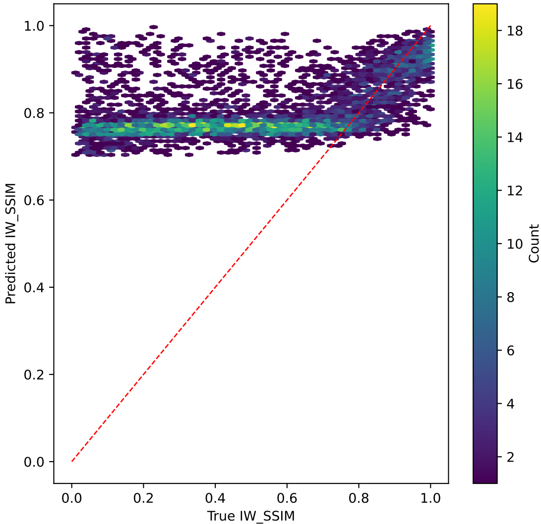
resnet50v2 on IW_SSIM | R^2=-2.000
