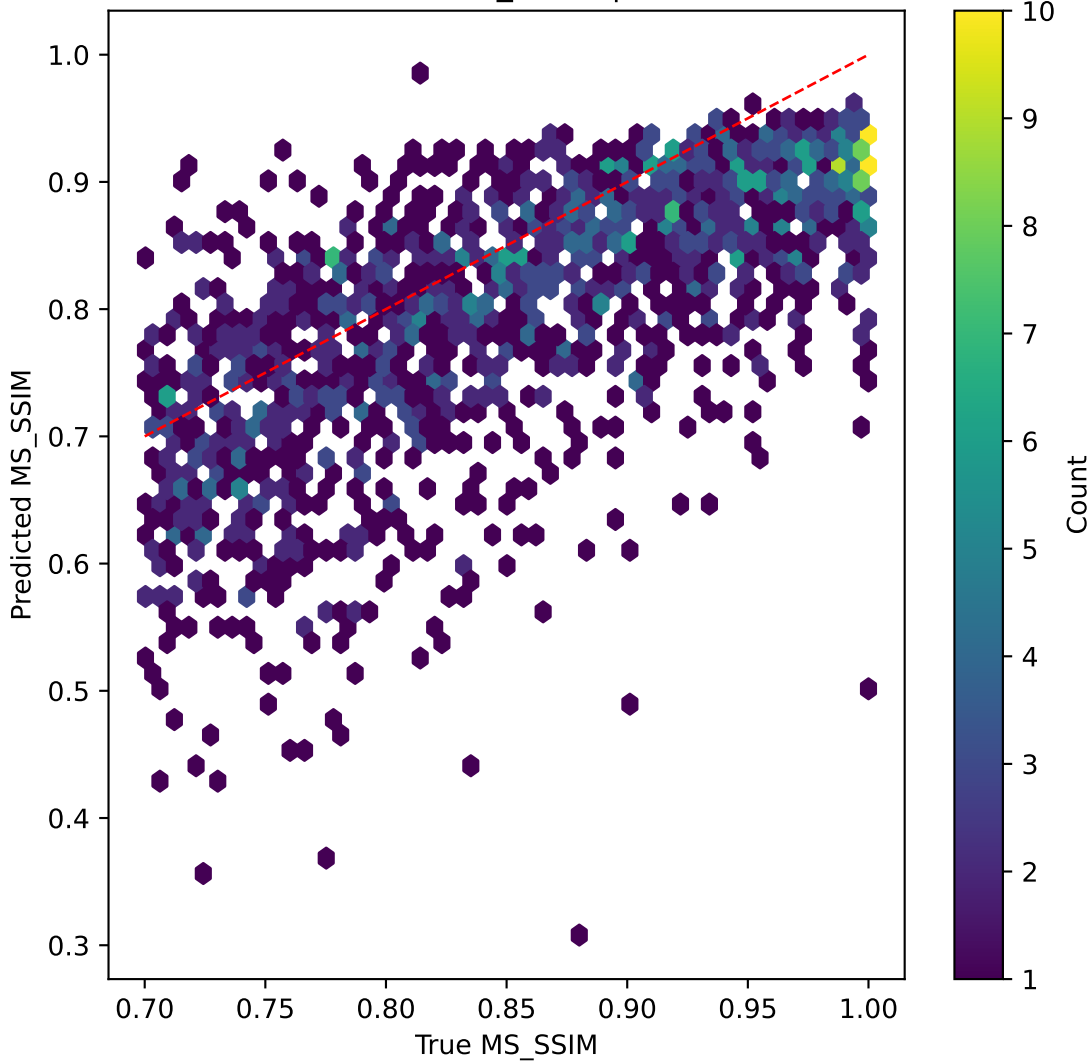
efficientnet on MS_SSIM | R^2=-0.224
