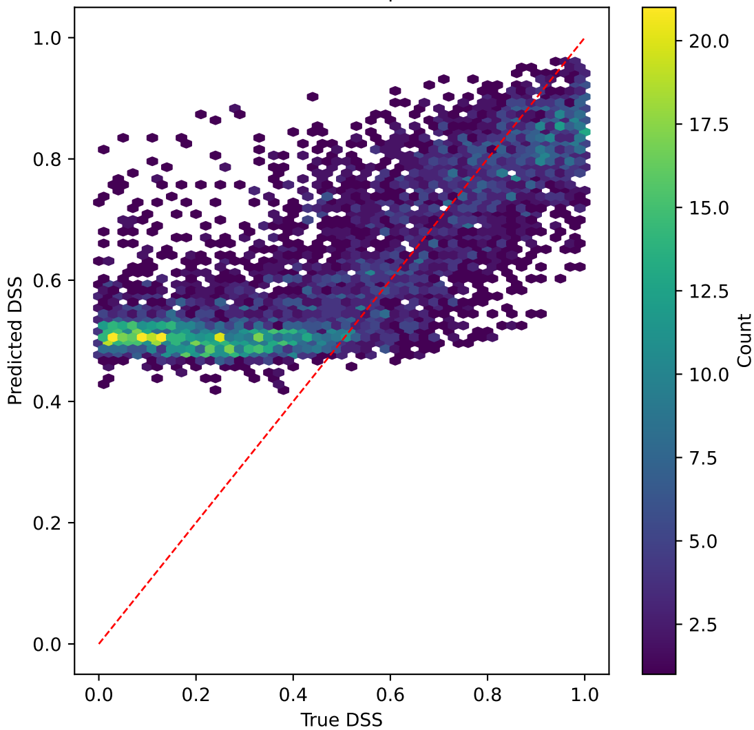
resnet50v2 on DSS | R^2=-0.966
