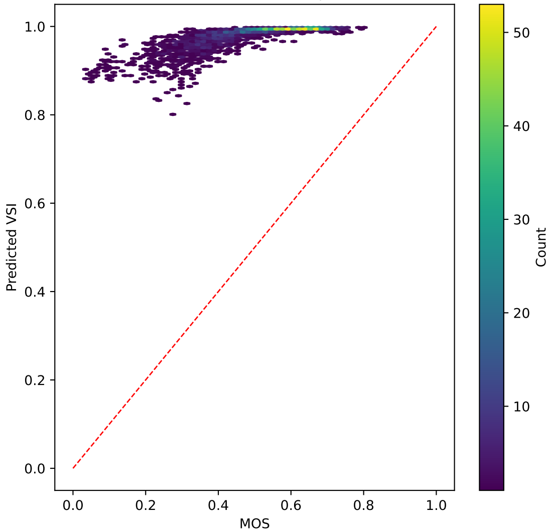
tinyvit on VSI AGAINST MOS | R^2=-12.055
