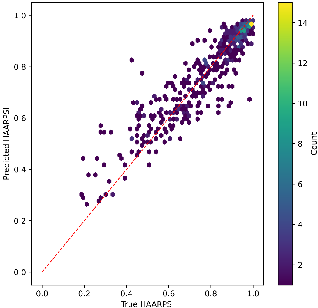
tinyvit on HAARPSI | R^2=0.842
