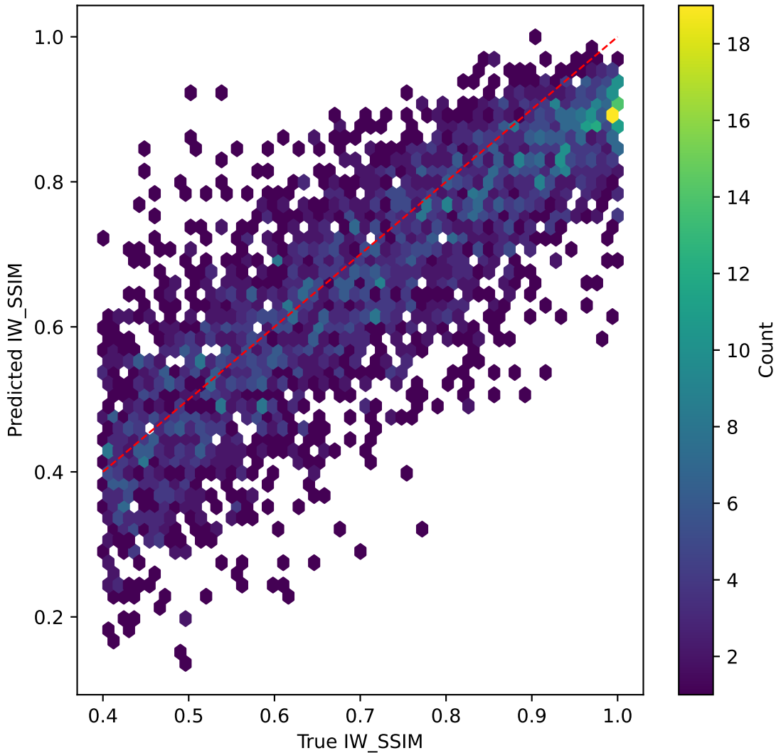
efficientnet on IW_SSIM | R^2=0.638
