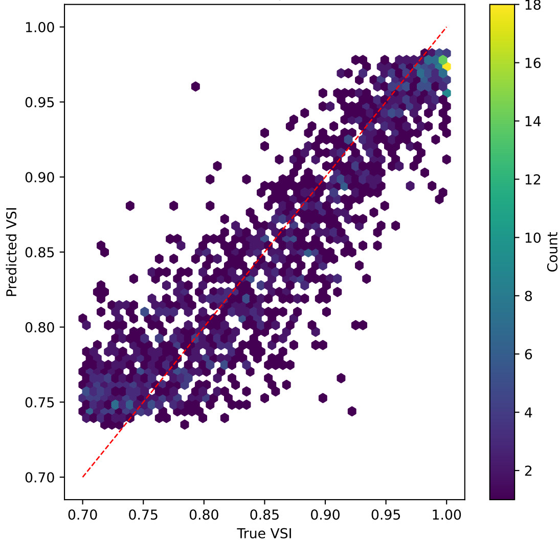
tinyvit on VSI | R^2=0.633
