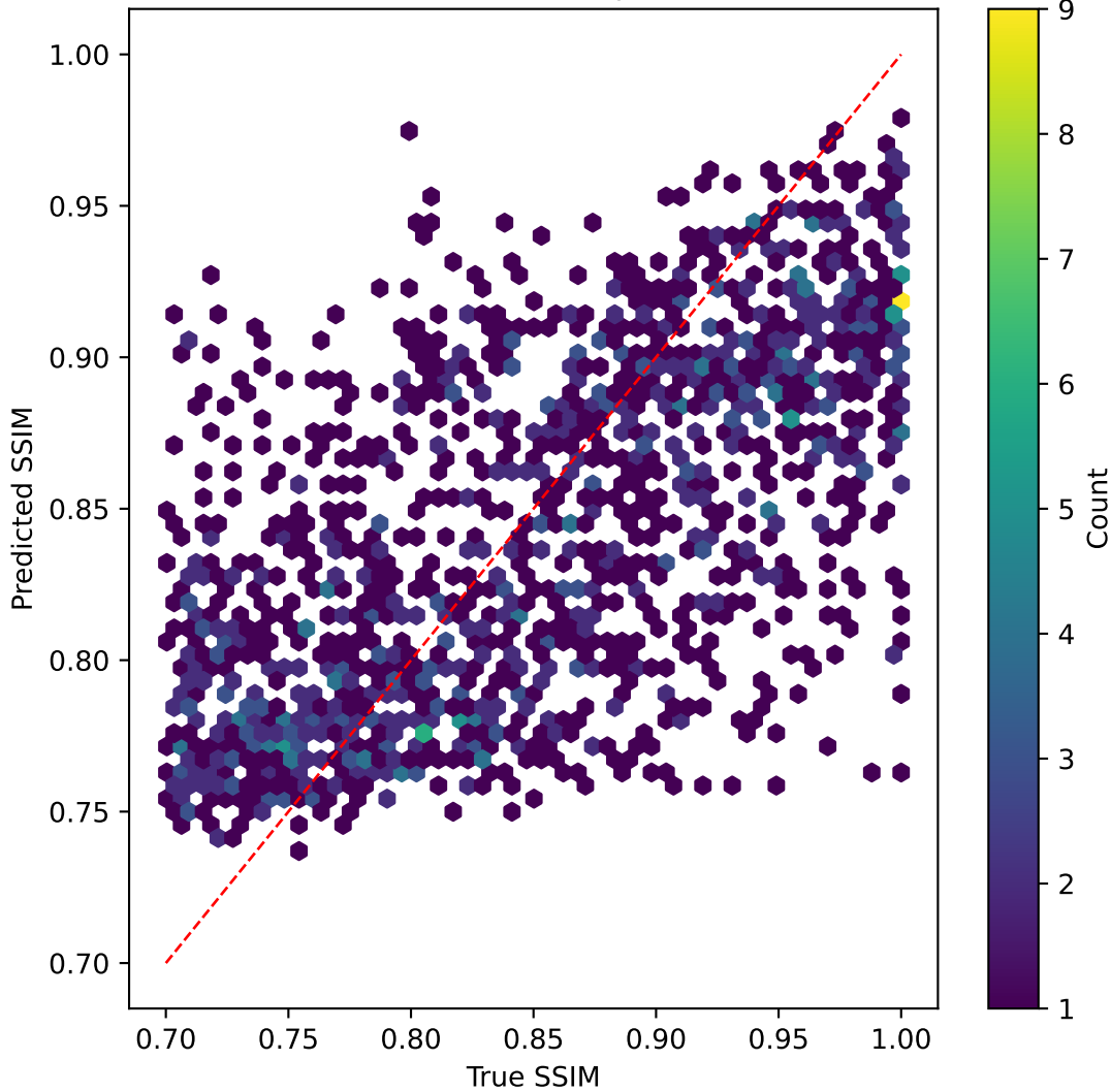
resnet50v2 on SSIM | R^2=0.364
