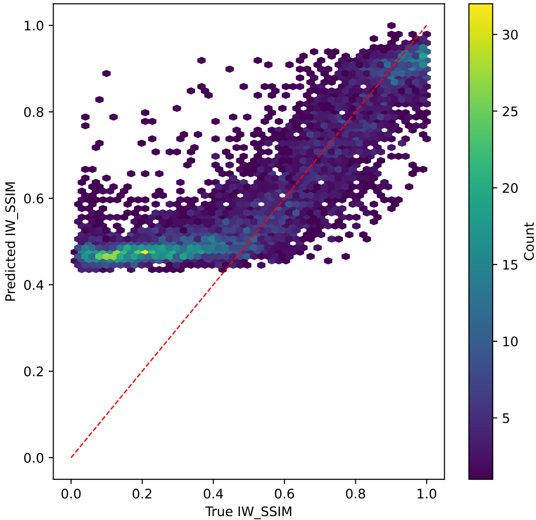
efficientnet on IW_SSIM | R^2=0.264
