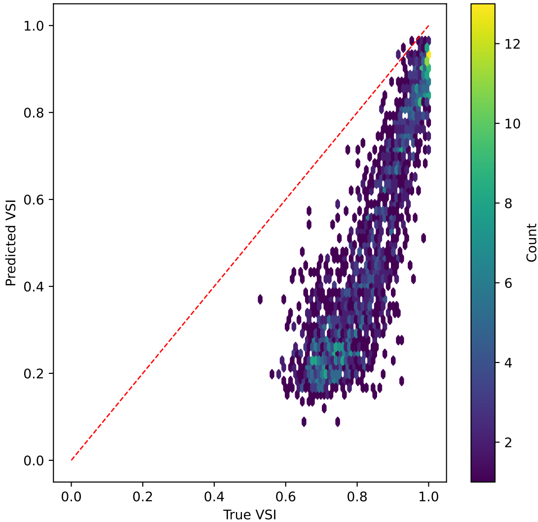
efficientnet on VSI | R^2=-29.839
