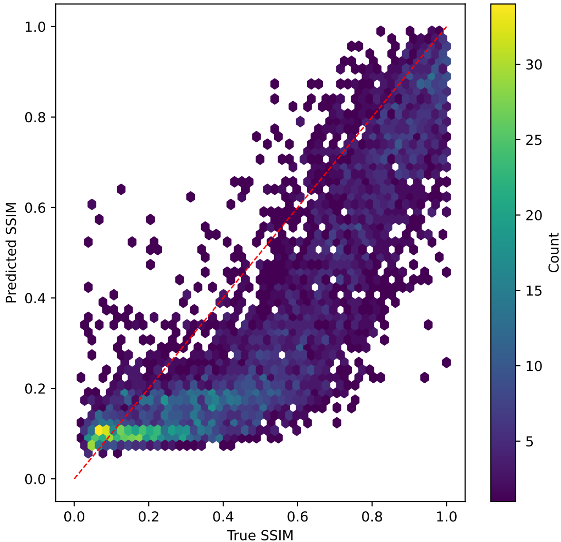
resnet50v2 on SSIM | R^2=0.255
