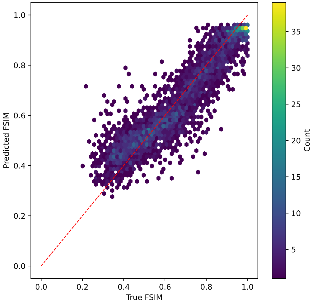
tinyvit on FSIM | R^2=0.731
