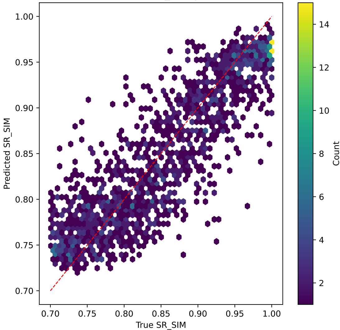
mobilenetv3 on SR_SIM | R^2=0.748
