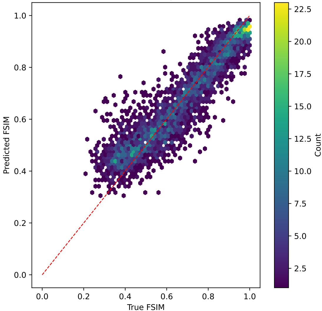
mobilevitv2 on FSIM | R^2=0.769
