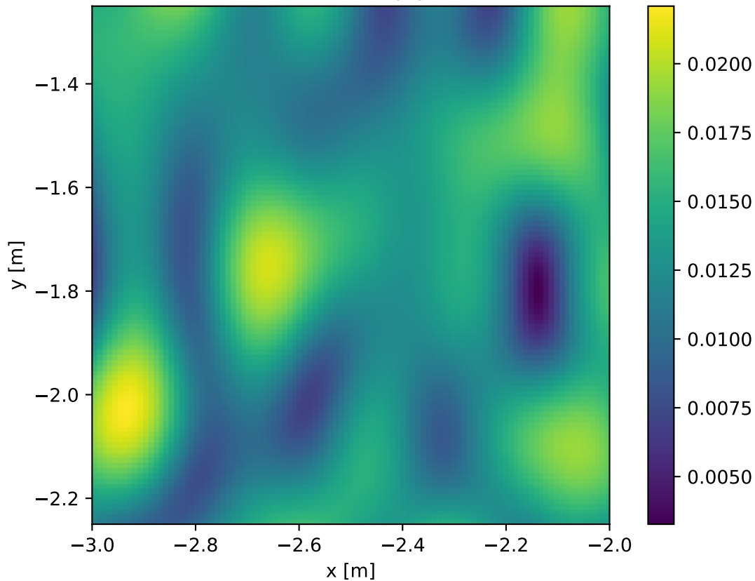
pcnk field ( |p| )
