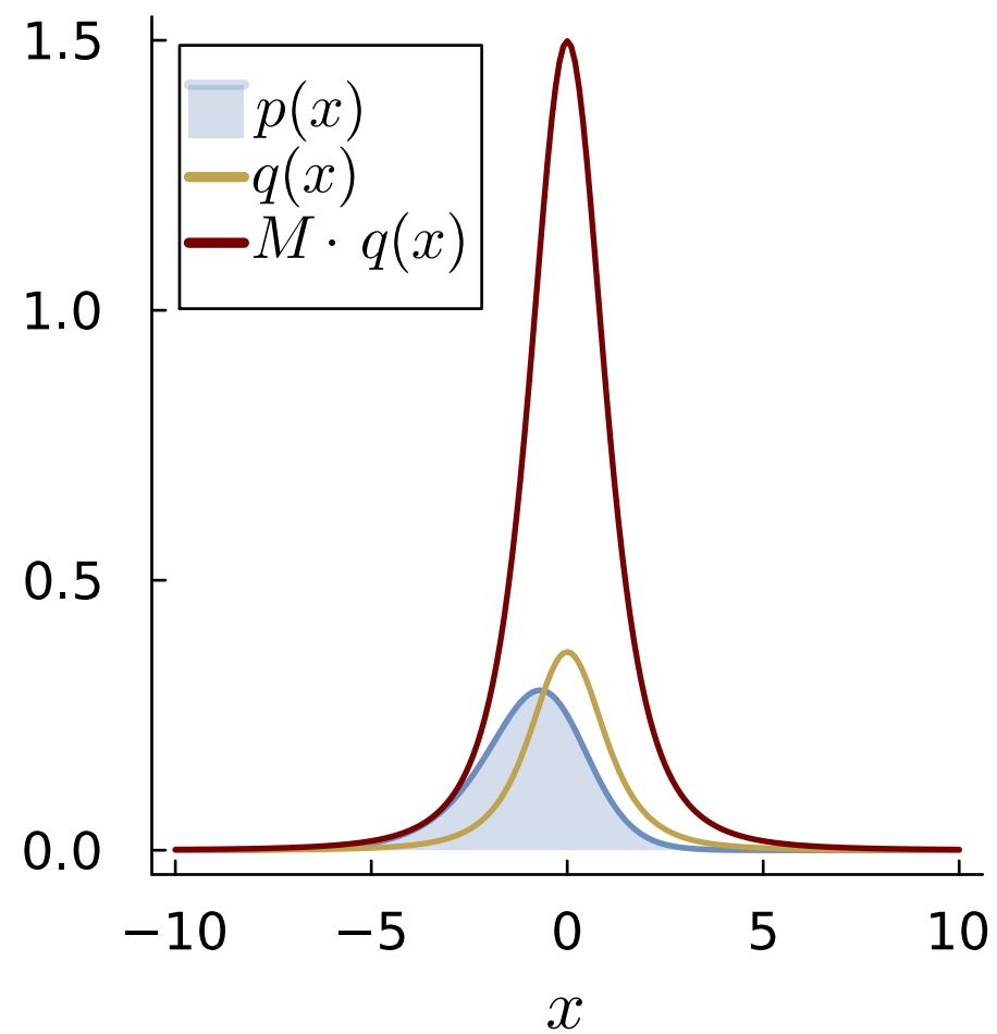
t(0, 1, 3) proposal
