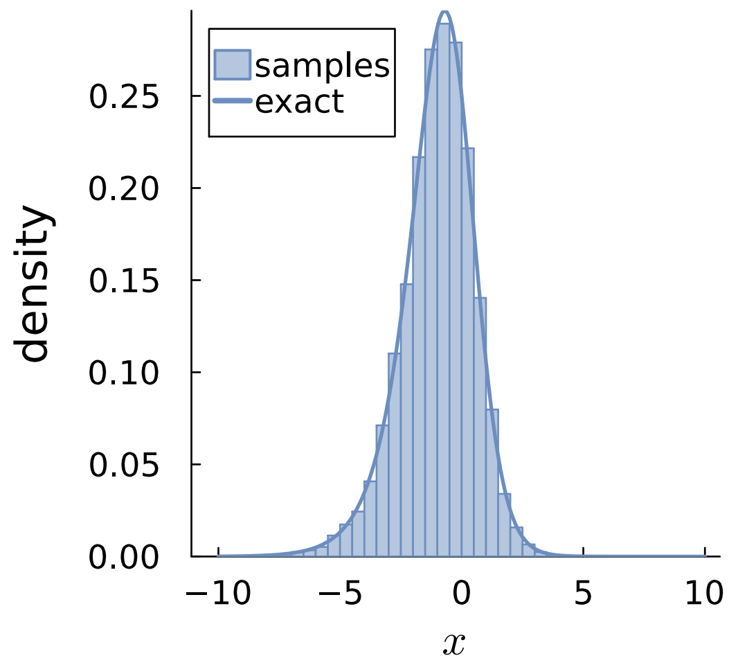
M = 4.078 , acc. rate = 0.243
