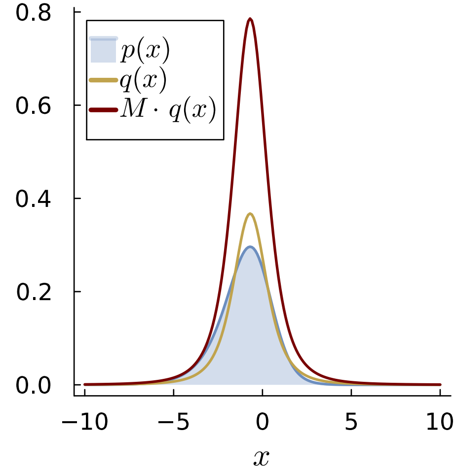
t(x_{\text{mode}}, 1, 3) proposal
