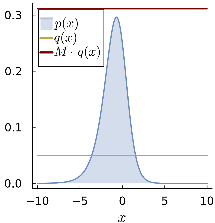
Uniform( -10, 10 ) proposal
