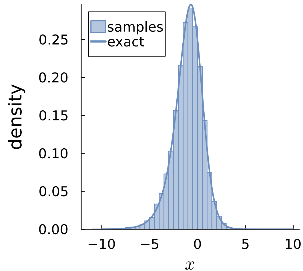
M = 2.138 , acc. rate = 0.466
