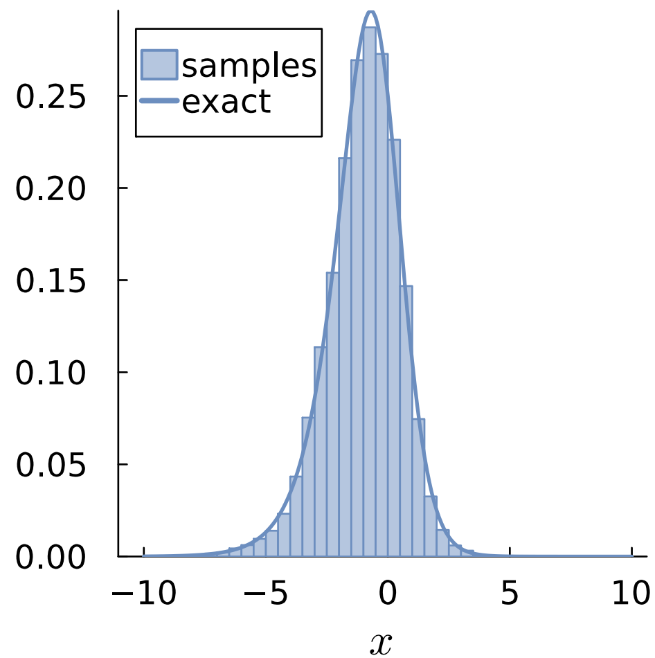
M = 6.222 , acc. rate = 0.159
