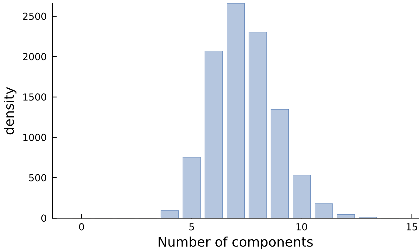
Posterior distribution for number of components
