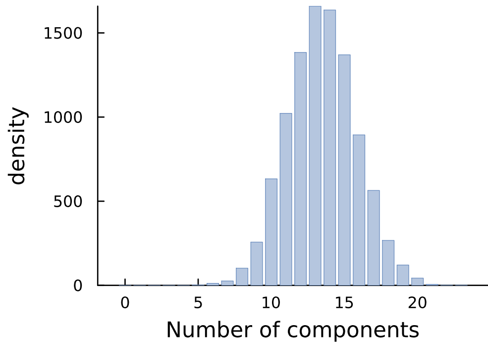
Posterior distribution for number of compon
