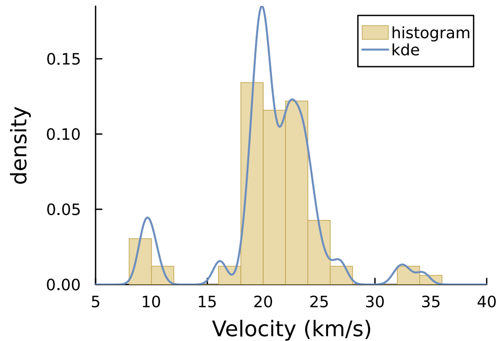
Kernel density estimate
