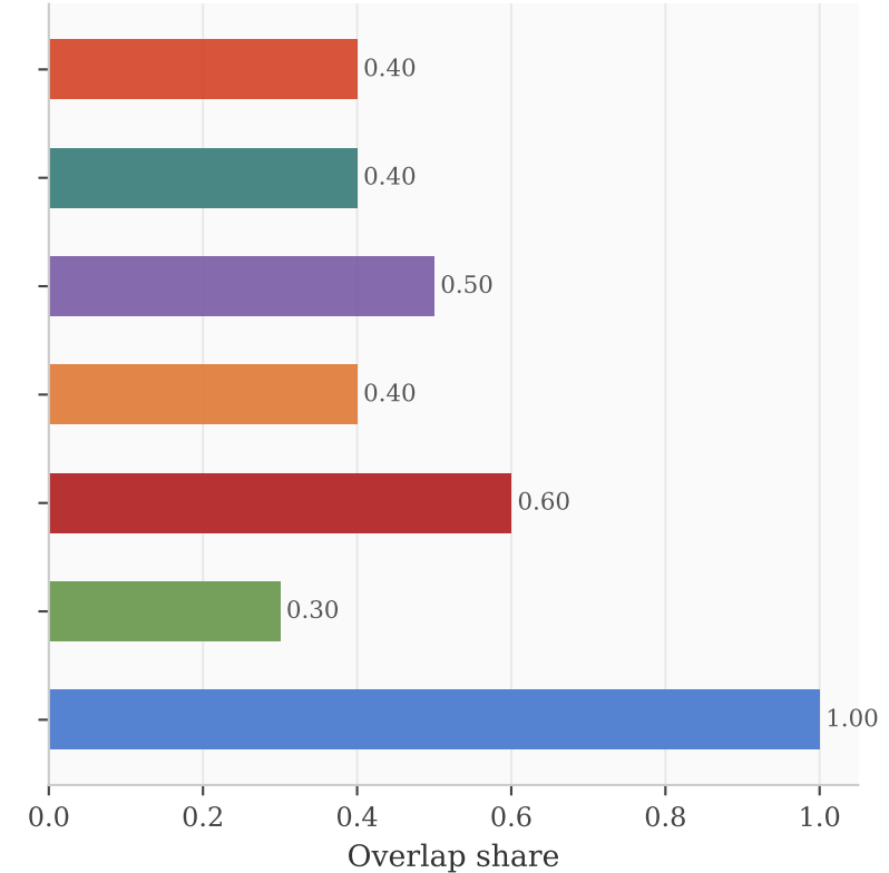
Top-K Overlap
