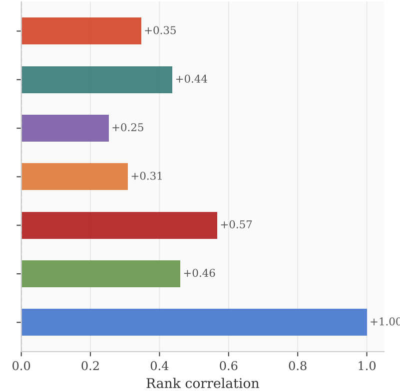
Spearman \rho
