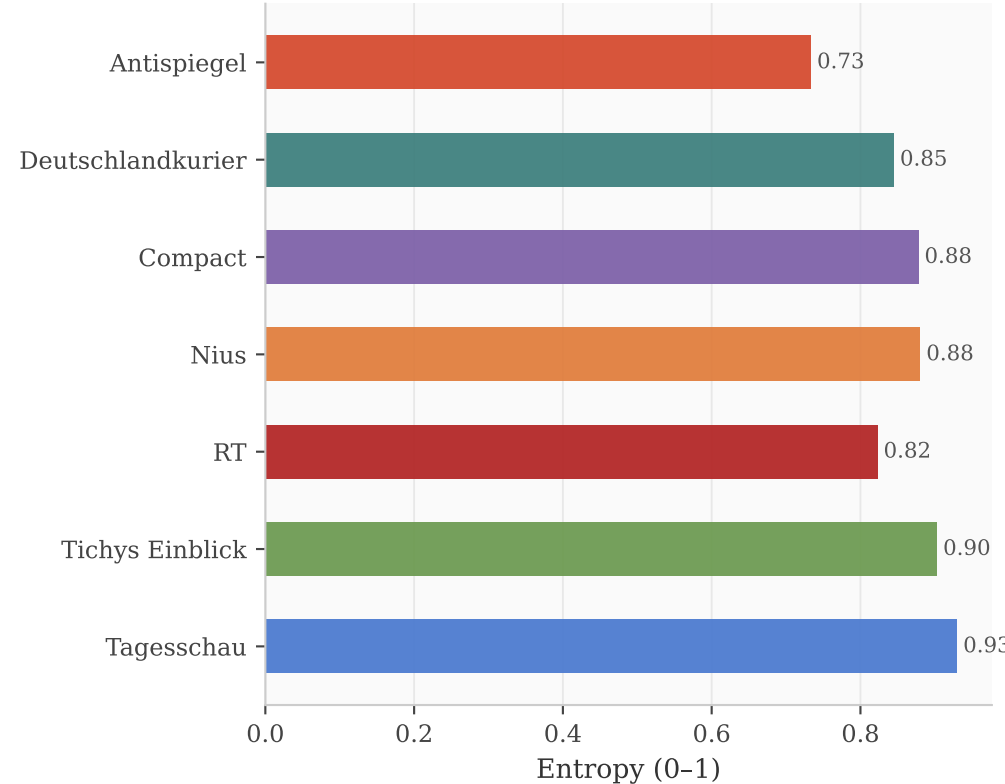
Topic Entropy
