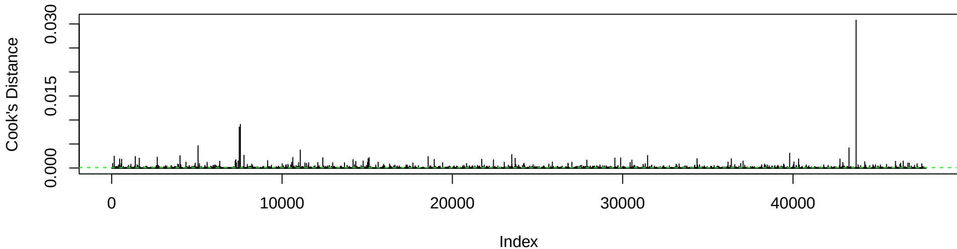
Cook's Distance by Observation Index
