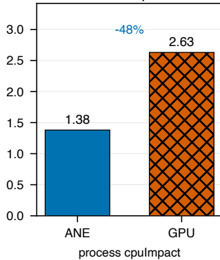
CPU impact
